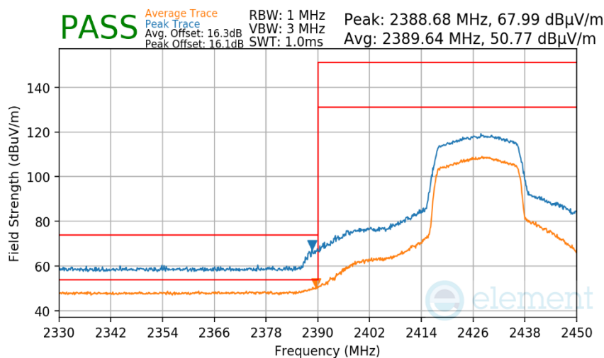
Plot 7-516 Radiated Restricted Lower Band Edge Measurement Antenna 3a
