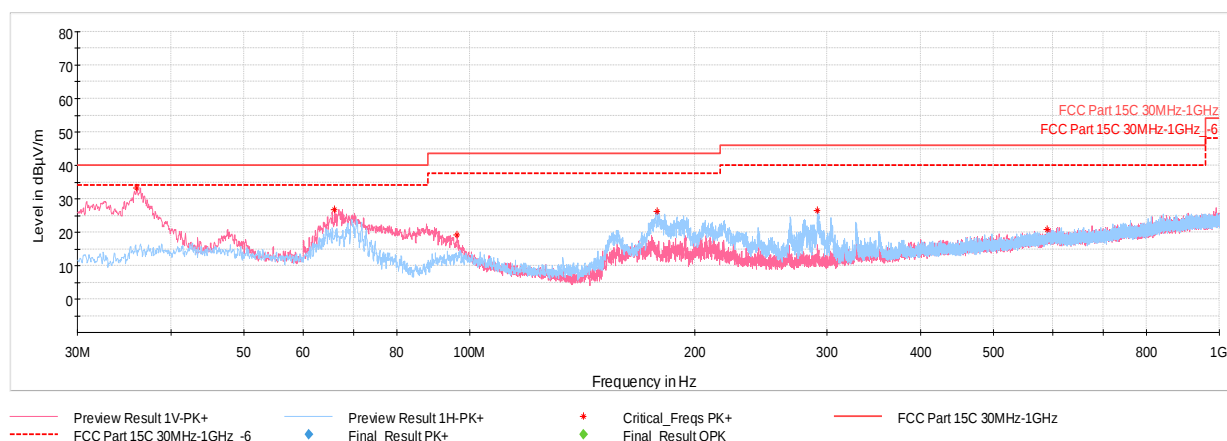
Plot 7-197. Radiated Spurious Emissions below 1GHz CDD Ch.6 (RU26), with AC/DC Adapter and USB-C Cable
