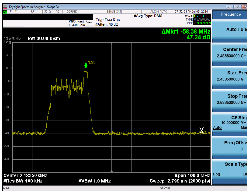
Plot 7-90. Band Edge Antenna 1a (802.11ax OFDMA – RU26 Index 8 – Ch. 11)
