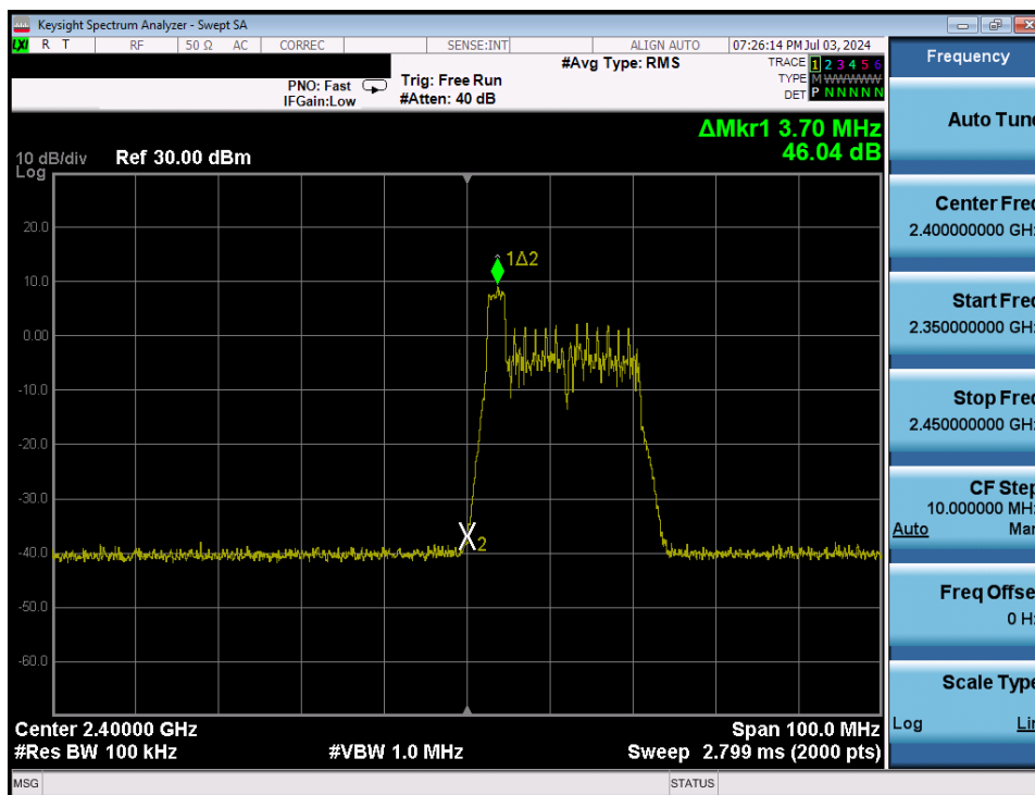
Plot 7-89. Band Edge Antenna 1a (802.11ax OFDMA – RU26 Index 0 – Ch. 1)
