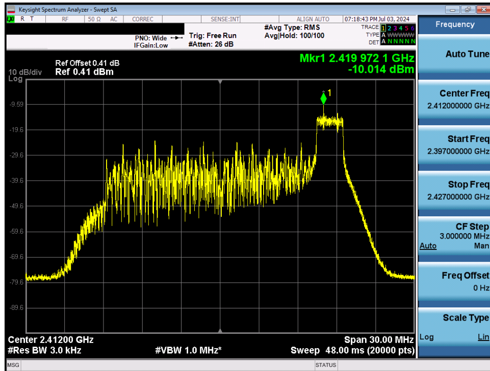
Plot 7-39. Power Spectral Density Plot Antenna 1a (802.11ax OFDMA – RU26 Index 8 – Ch. 1)
