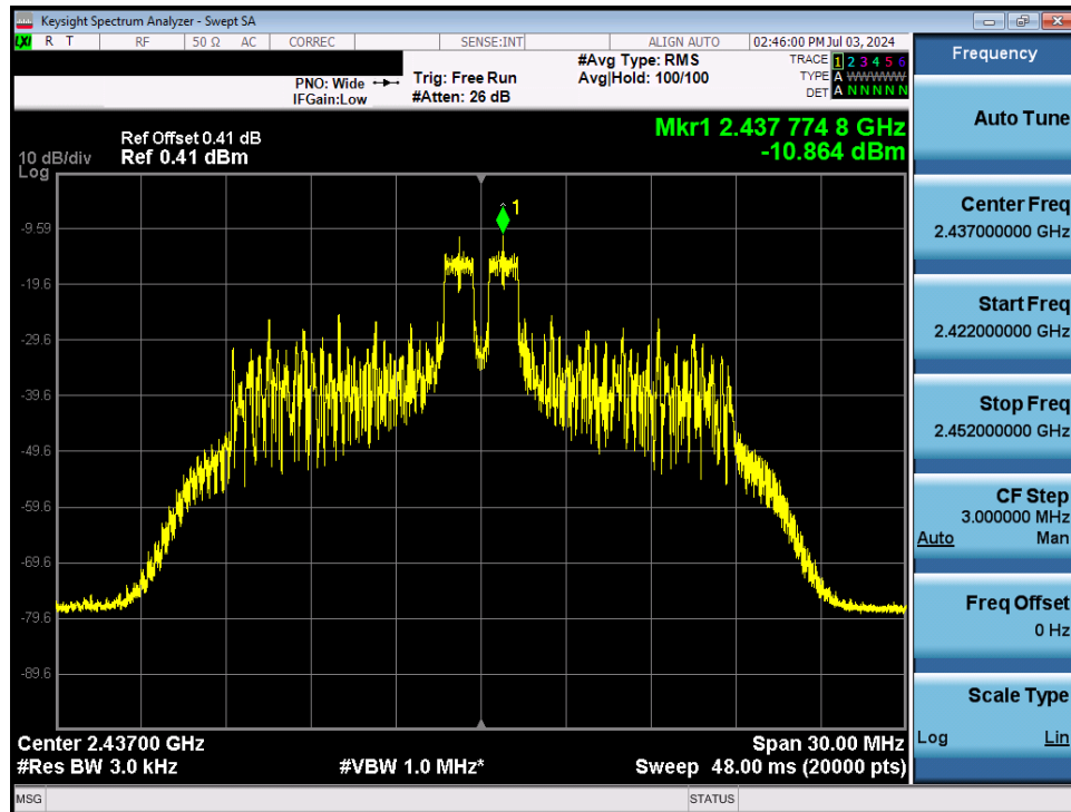
Plot 7-29. Power Spectral Density Plot Antenna 3a (802.11ax OFDMA – RU26 Index 4 – Ch. 6)
