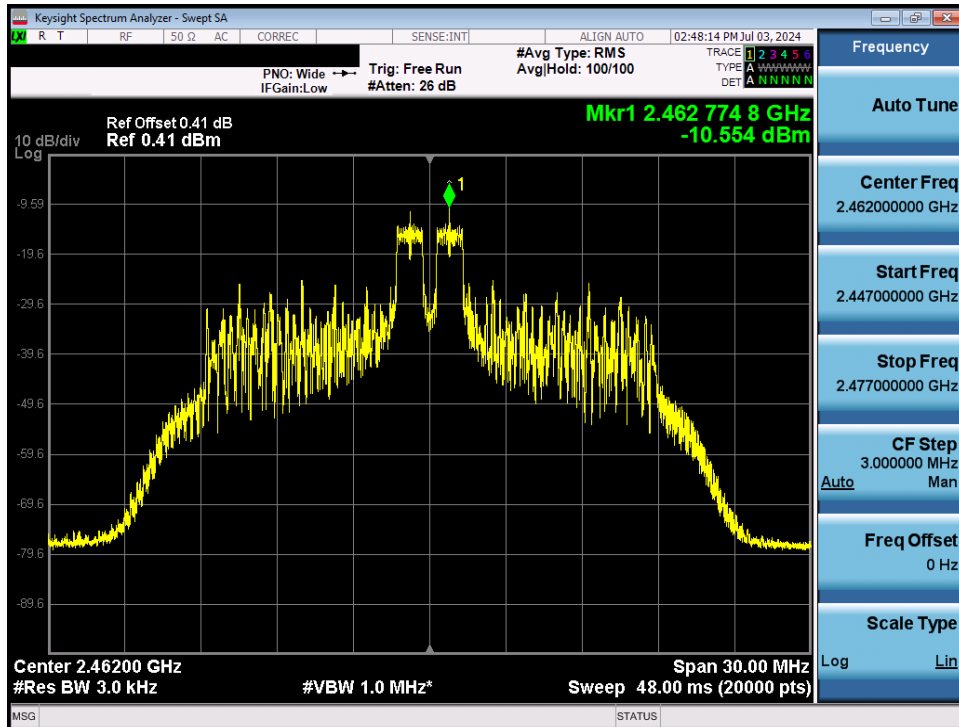
Plot 7-32. Power Spectral Density Plot Antenna 3a (802.11ax OFDMA – RU26 Index 4 – Ch. 11)
