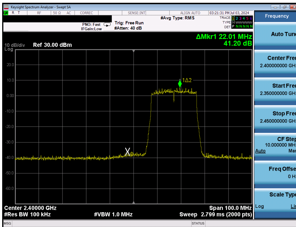
Plot 7-77. Band Edge Antenna 3a (802.11ax OFDMA – RU242 – Ch. 2)
