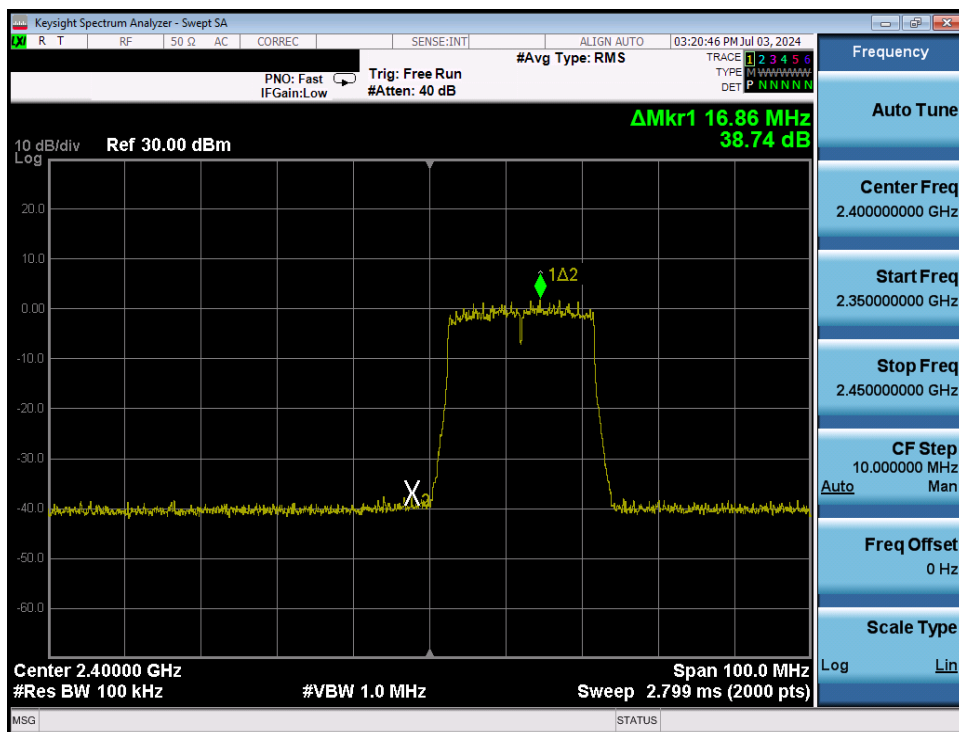
Plot 7-76. Band Edge Antenna 3a (802.11ax OFDMA – RU242 – Ch. 1)
