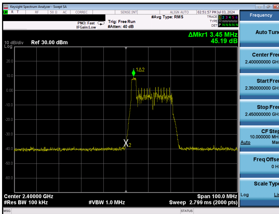
Plot 7-73. Band Edge Antenna 3a (802.11ax OFDMA – RU26 Index 0 – Ch. 1)
