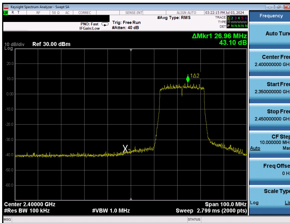
Plot 7-78. Band Edge Antenna 3a (802.11ax OFDMA – RU242 – Ch. 3)
