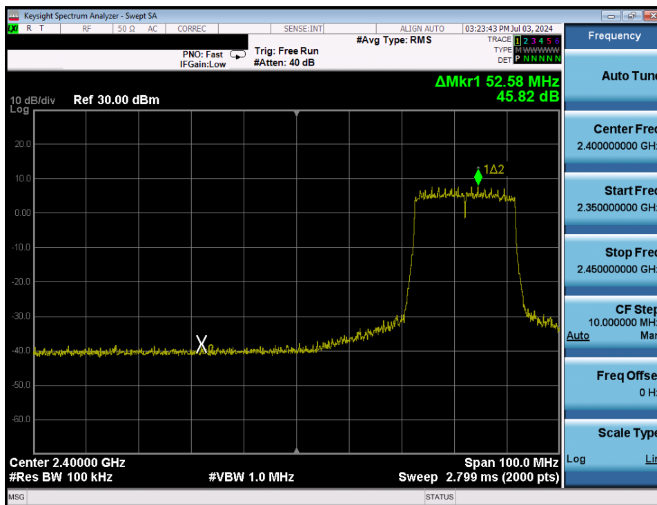
Plot 7-80. Band Edge Antenna 3a (802.11ax OFDMA – RU242 – Ch. 5)
