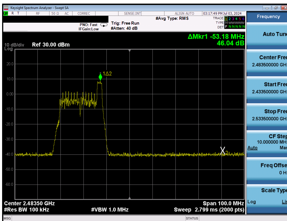
Plot 7-74. Band Edge Antenna 3a (802.11ax OFDMA – RU26 Index 8 – Ch. 11)
