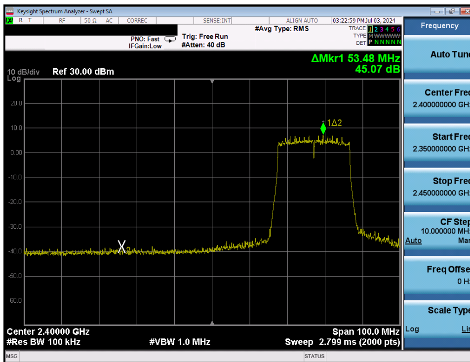
Plot 7-79. Band Edge Antenna 3a (802.11ax OFDMA – RU242 – Ch. 4)
