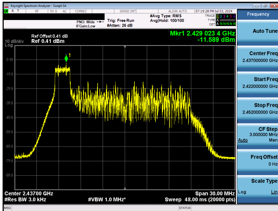
Plot 7-40. Power Spectral Density Plot Antenna 1a (802.11ax OFDMA – RU26 Index 0 – Ch. 6)
