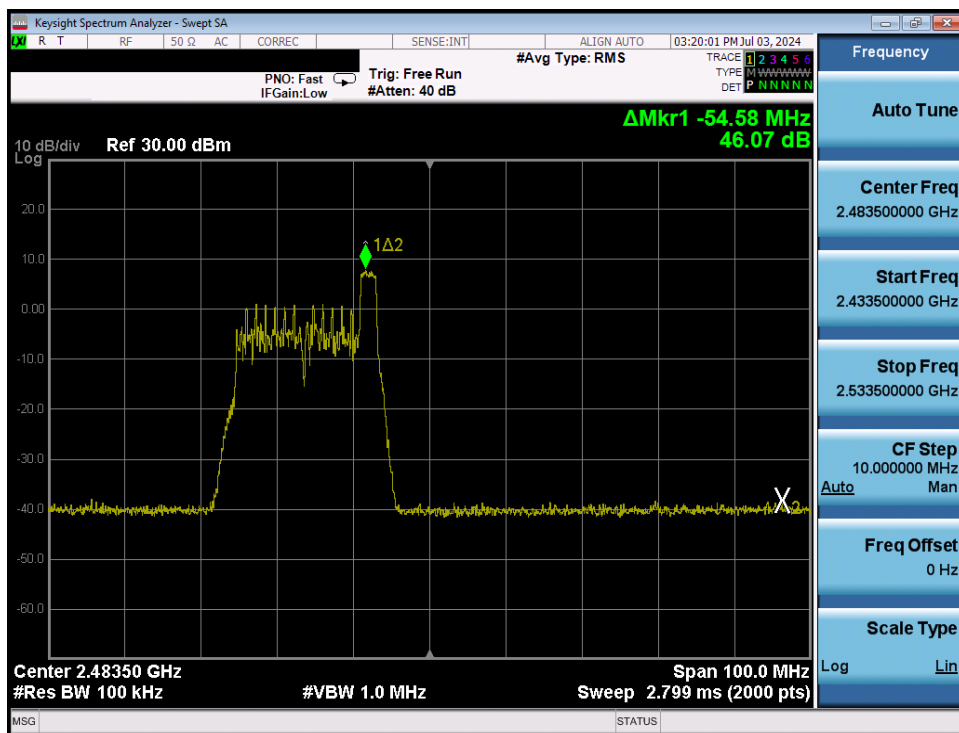
Plot 7-75. Band Edge Antenna 3a (802.11ax OFDMA – RU26 Index 8 – Ch. 12)
