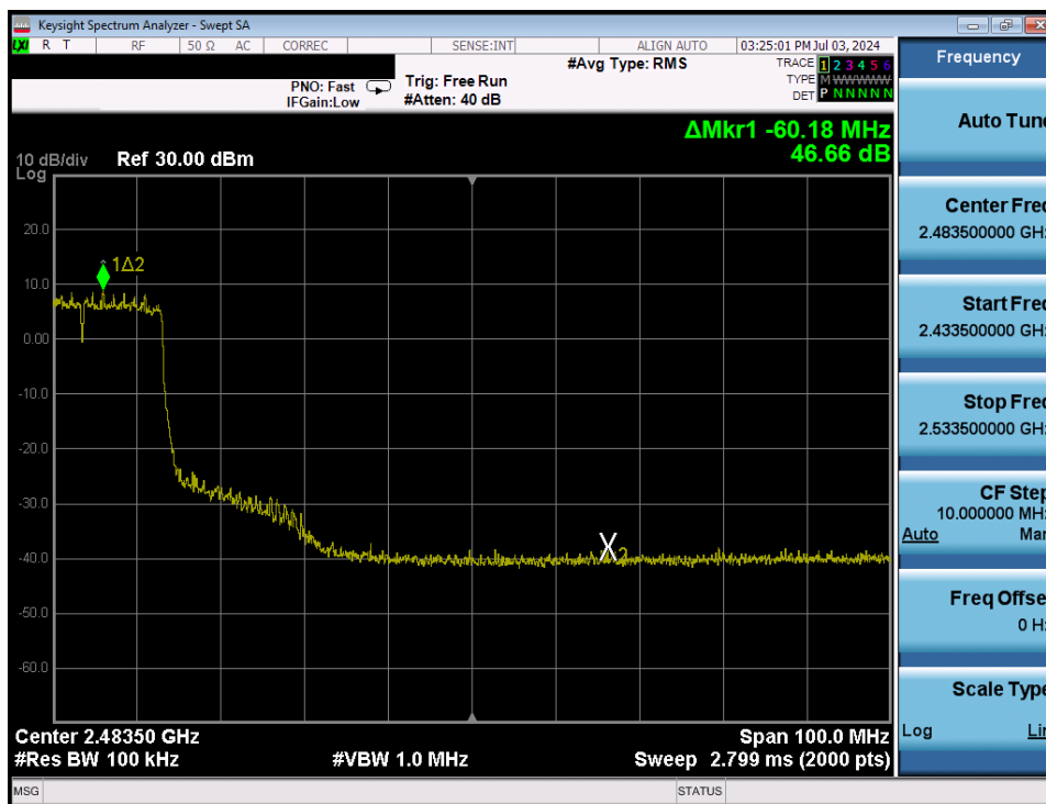
Plot 7-82. Band Edge Antenna 3a (802.11ax OFDMA – RU242 – Ch. 6 High)
