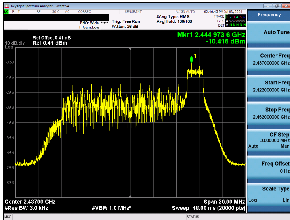
Plot 7-30. Power Spectral Density Plot Antenna 3a (802.11ax OFDMA – RU26 Index 8 – Ch. 6)
