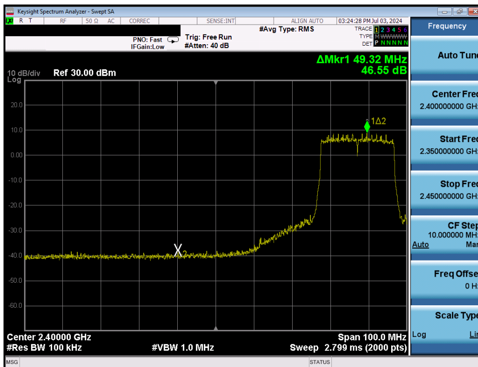
Plot 7-81. Band Edge Antenna 3a (802.11ax OFDMA – RU242 – Ch. 6 Low)
