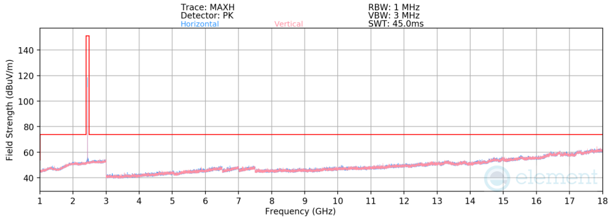
Plot 7-104. Radiated Spurious Emissions 1-18GHz Antenna 3a (1Mbps, ePA – Ch. 19)
