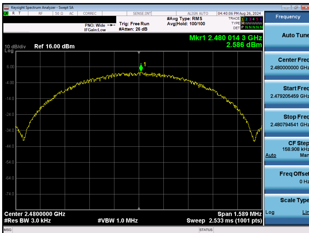
Plot 7-54. Power Spectral Density Plot Antenna 1a (Bluetooth (LE), 1Mbps, ePA – Ch. 39)
