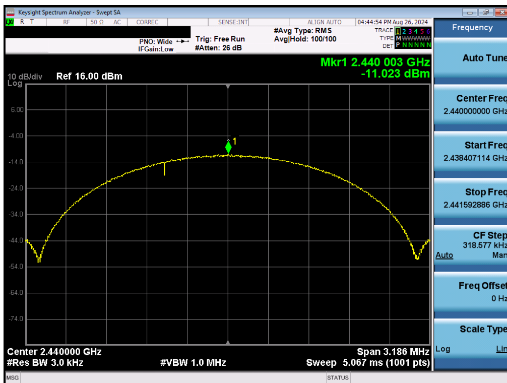
Plot 7-70. Power Spectral Density Plot Antenna 1a (Bluetooth (LE), 2Mbps, iPA – Ch. 19)
