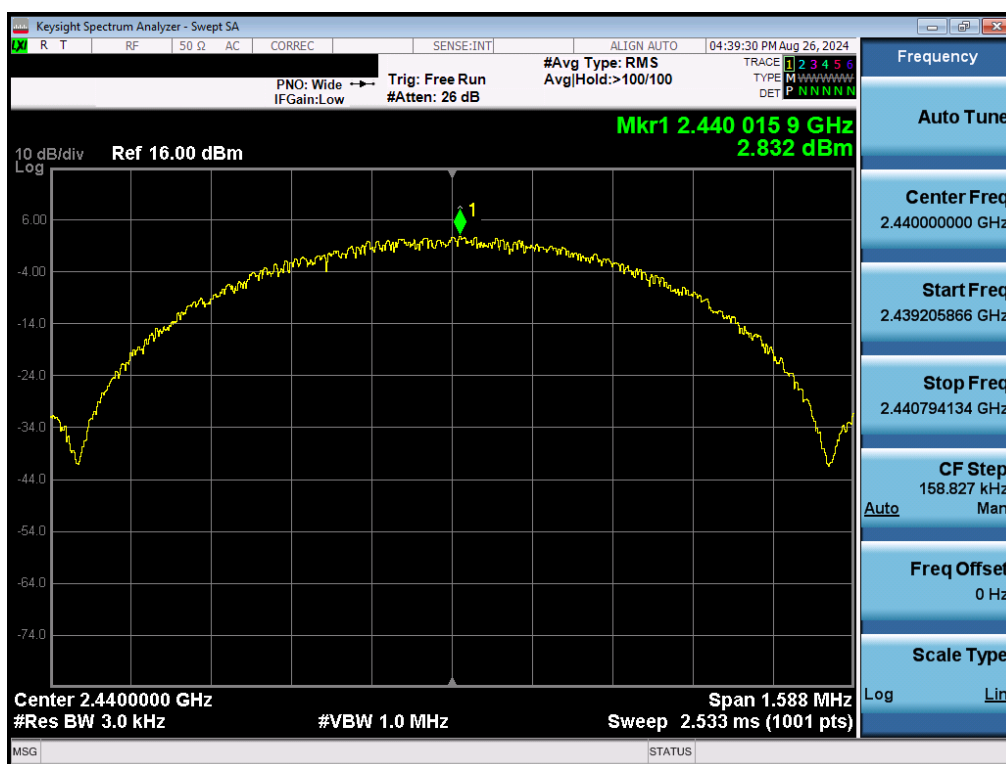
Plot 7-52. Power Spectral Density Plot Antenna 1a (Bluetooth (LE), 1Mbps, ePA – Ch. 19)
