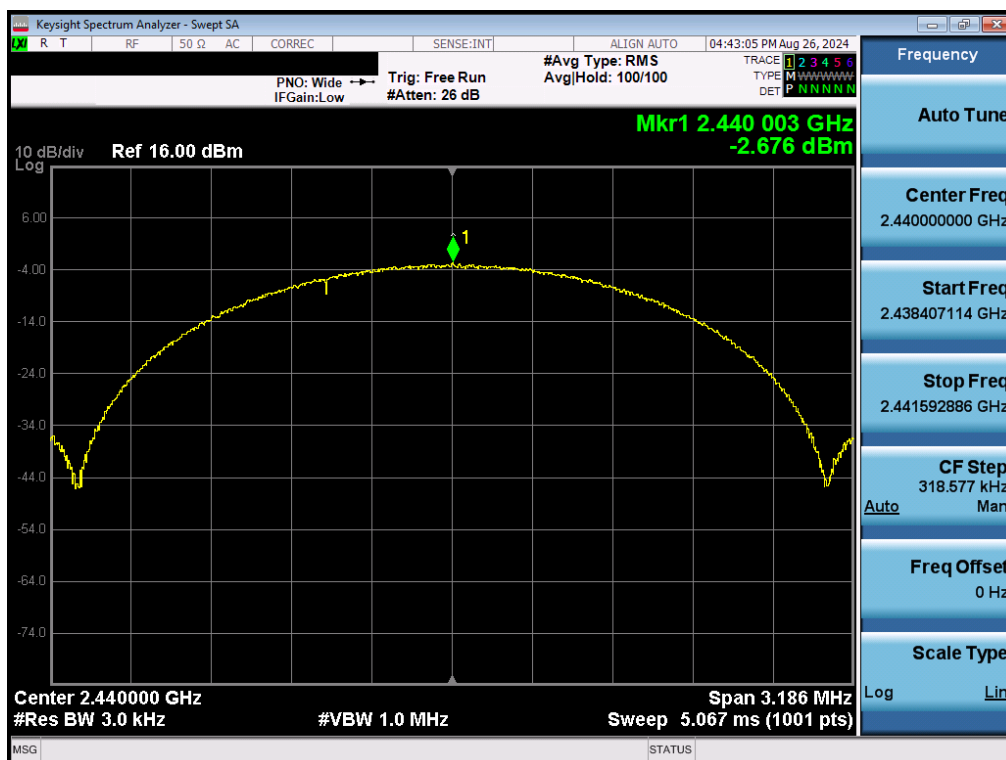
Plot 7-64. Power Spectral Density Plot Antenna 1a (Bluetooth (LE), 2Mbps, ePA – Ch. 19)
