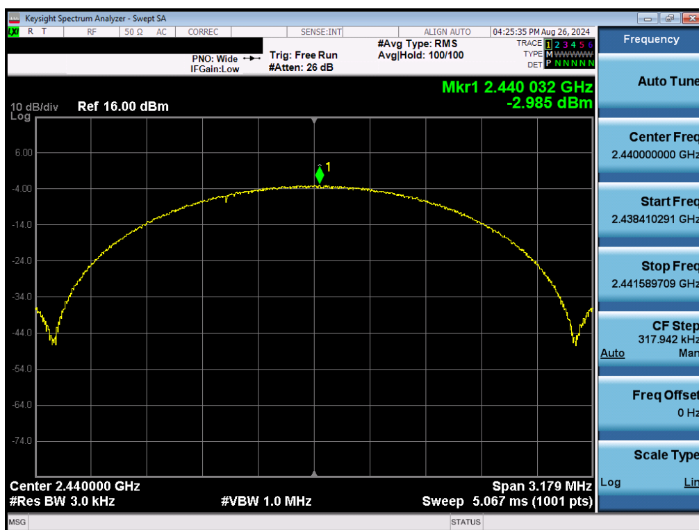
Plot 7-63. Power Spectral Density Plot Antenna 3a (Bluetooth (LE), 2Mbps, ePA – Ch. 19)
