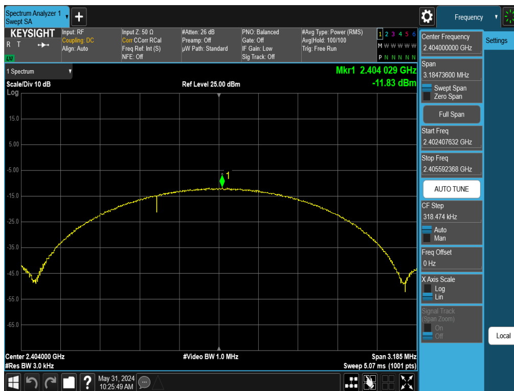
Plot 7-28. Power Spectral Density Plot Antenna 3a (Bluetooth (LE), 2Mbps, iPA – Ch. 1)
