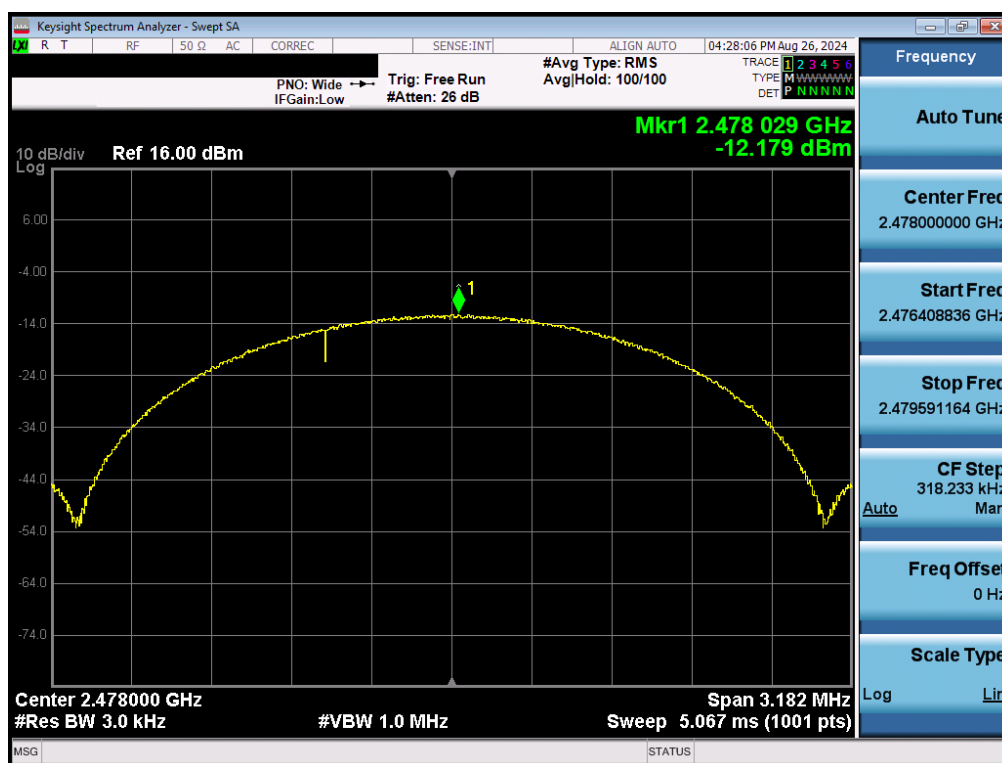
Plot 7-71. Power Spectral Density Plot Antenna 3a (Bluetooth (LE), 2Mbps, iPA – Ch. 38)
