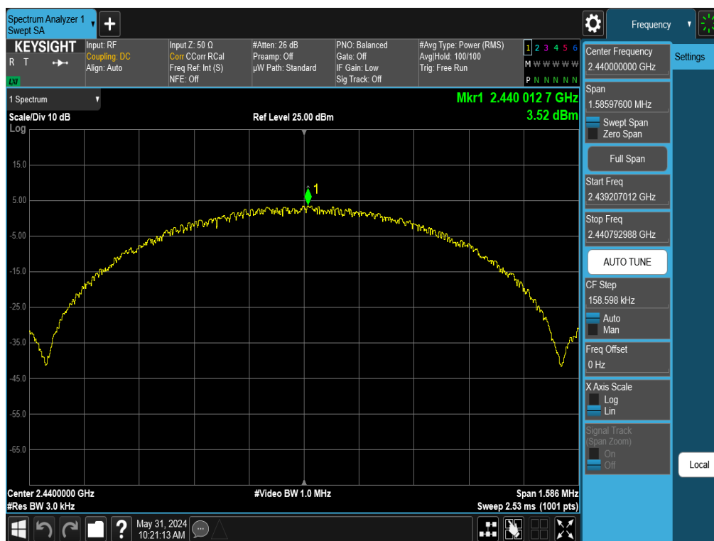
Plot 7-20. Power Spectral Density Plot Antenna 3a (Bluetooth (LE), 1Mbps, ePA – Ch. 19)
