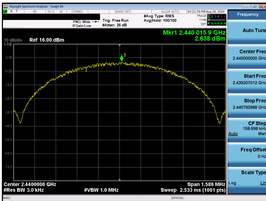
Plot 7-51. Power Spectral Density Plot Antenna 3a (Bluetooth (LE), 1Mbps, ePA – Ch. 19)
