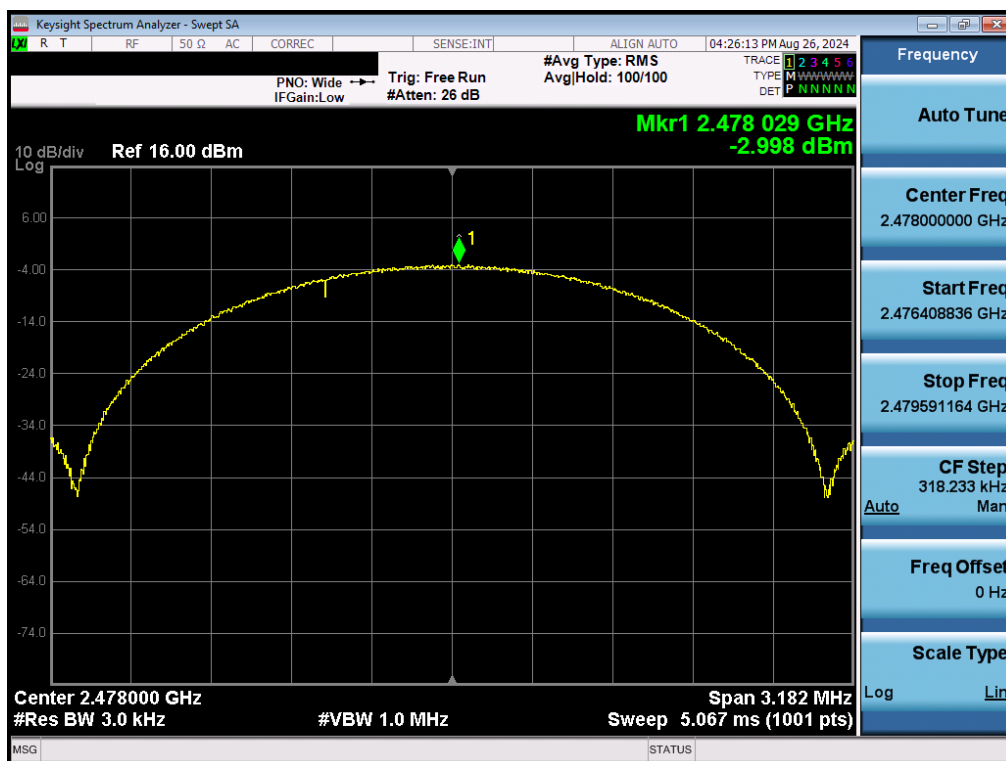
Plot 7-65. Power Spectral Density Plot Antenna 3a (Bluetooth (LE), 2Mbps, ePA – Ch. 38)
