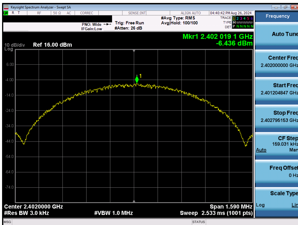
Plot 7-56. Power Spectral Density Plot Antenna 1a (Bluetooth (LE), 1Mbps, iPA – Ch. 0)
