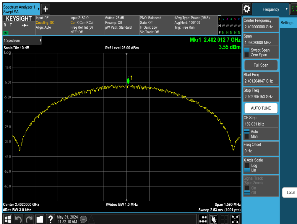
Plot 7-31. Power Spectral Density Plot Antenna 1a (Bluetooth (LE), 1Mbps, ePA – Ch. 0)
