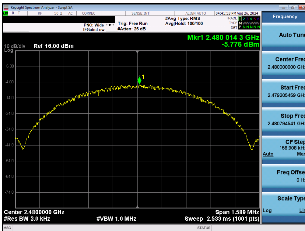
Plot 7-60. Power Spectral Density Plot Antenna 1a (Bluetooth (LE), 1Mbps, iPA – Ch. 39)
