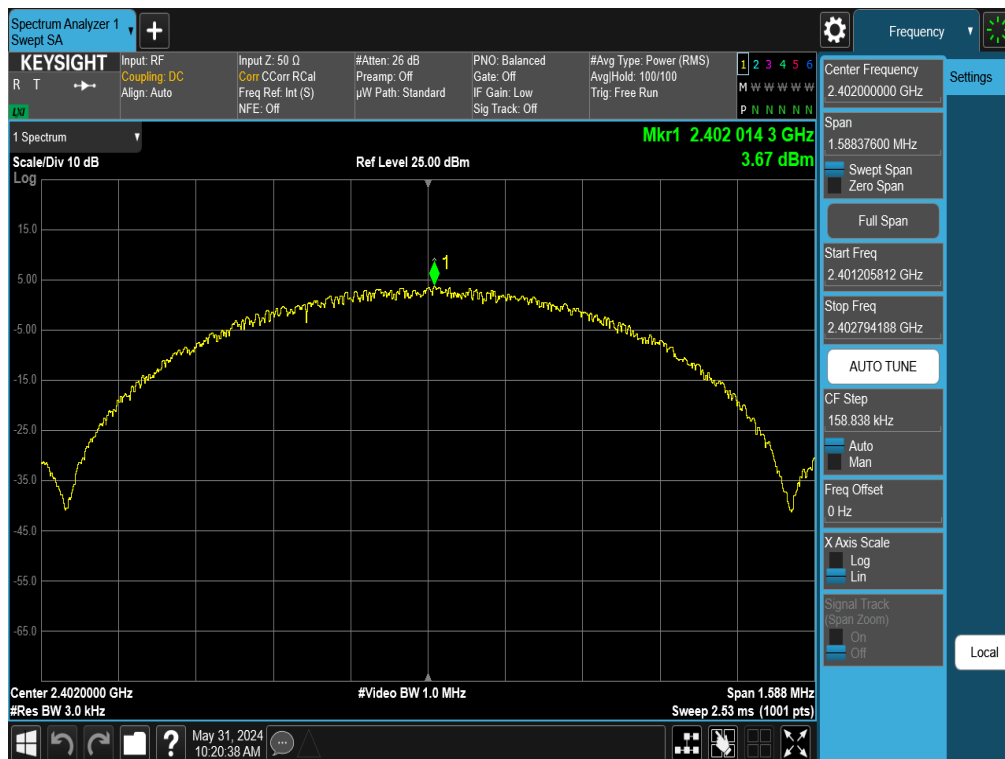
Plot 7-19. Power Spectral Density Plot Antenna 3a (Bluetooth (LE), 1Mbps, ePA – Ch. 0)
