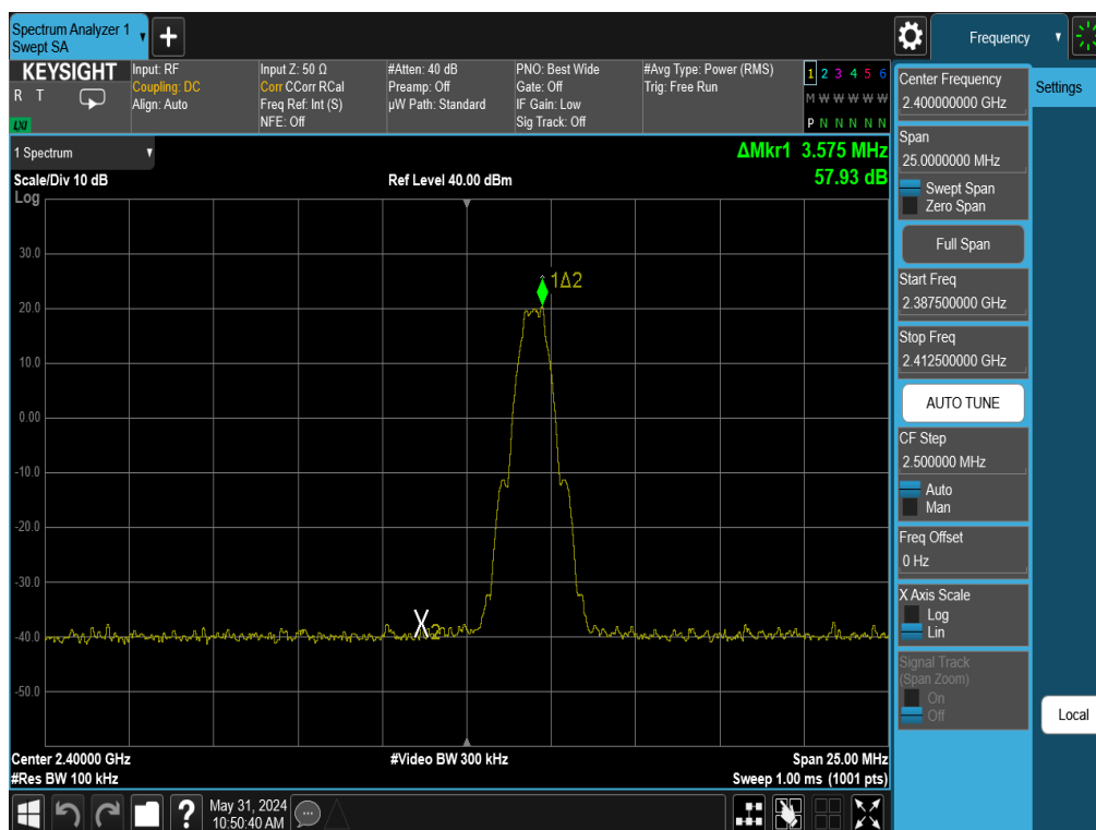
Plot 7-73. Band Edge Plot Antenna 3a (Bluetooth (LE), 1Mbps, ePA – Ch.0)
