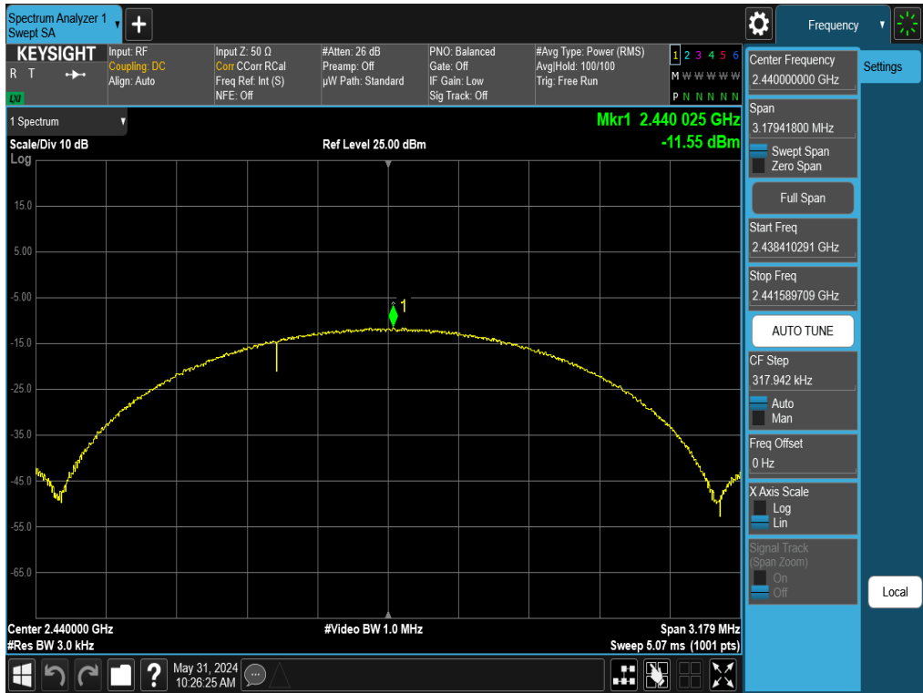
Plot 7-29. Power Spectral Density Plot Antenna 3a (Bluetooth (LE), 2Mbps, iPA – Ch. 19)
