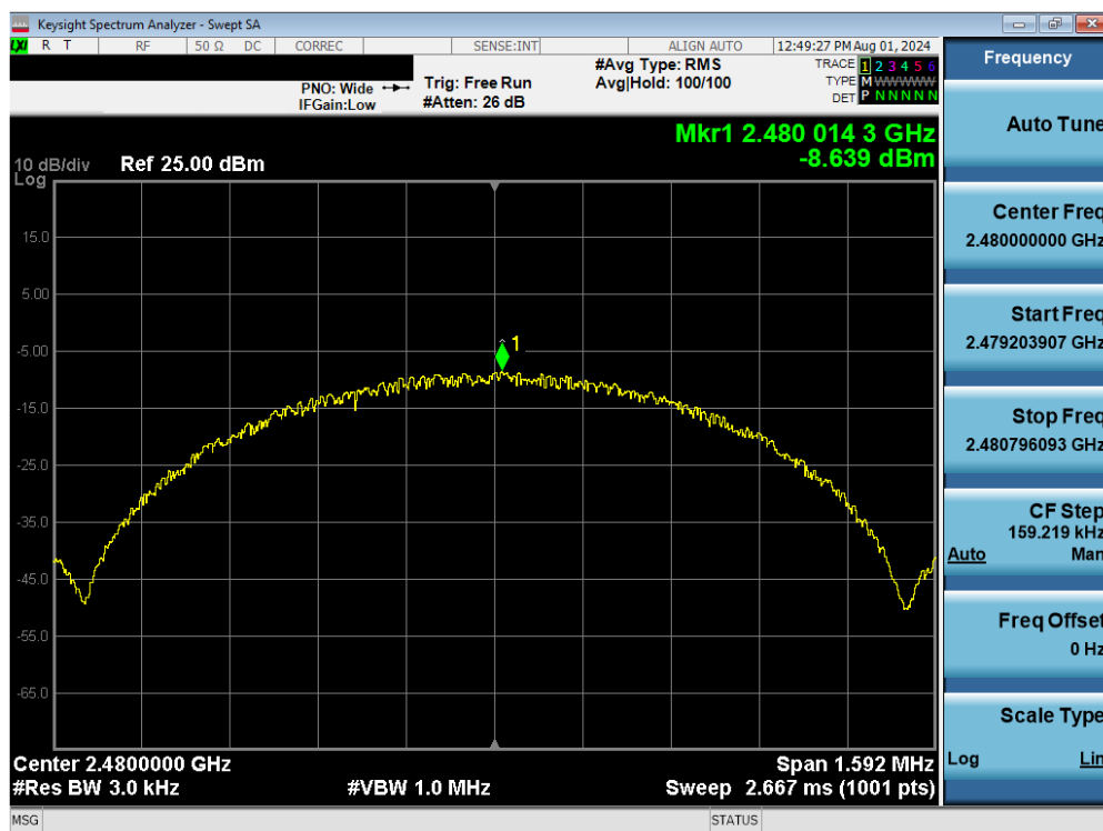
Plot 7-45. Power Spectral Density Plot Antenna 4 (Bluetooth (LE), 1Mbps, iPA – Ch. 39)
