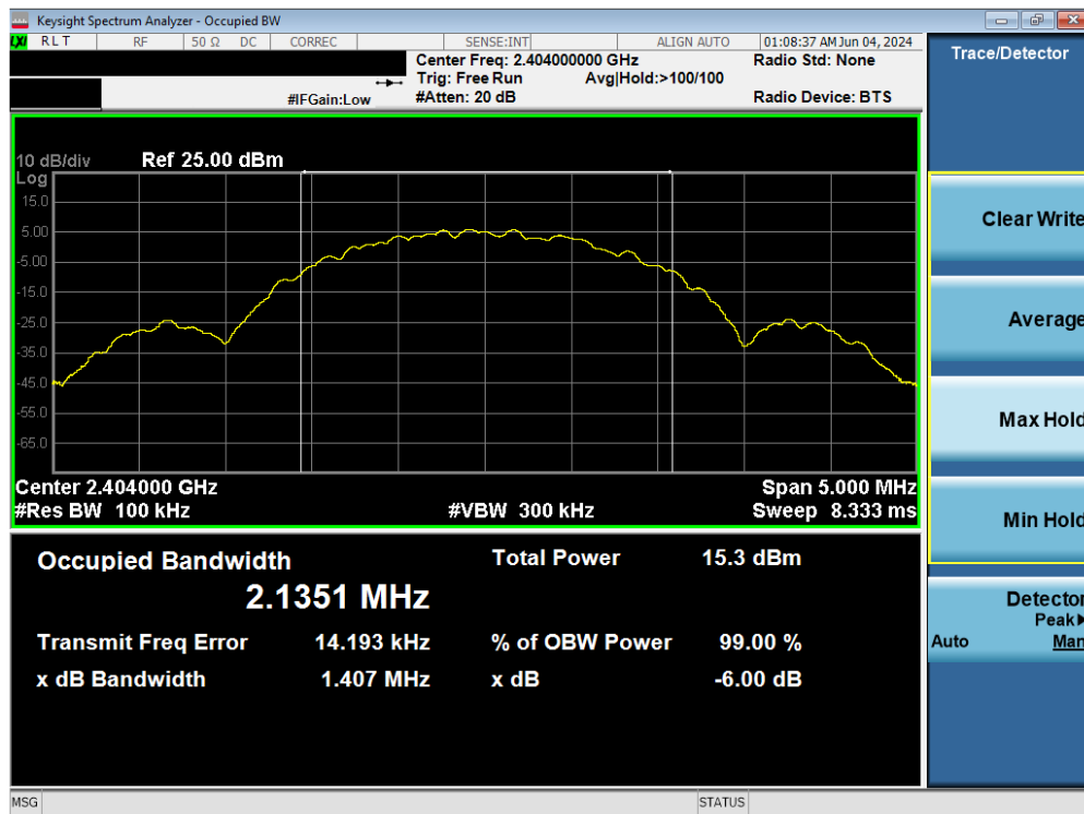
Plot 7-16. 6dB BW & 99% OBW Plot Antenna 4 (Bluetooth (LE), 2Mbps, iPA – Ch. 1)
