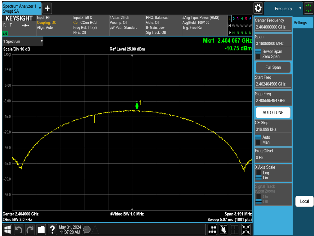
Plot 7-40. Power Spectral Density Plot Antenna 1a (Bluetooth (LE), 2Mbps, iPA – Ch. 1)
