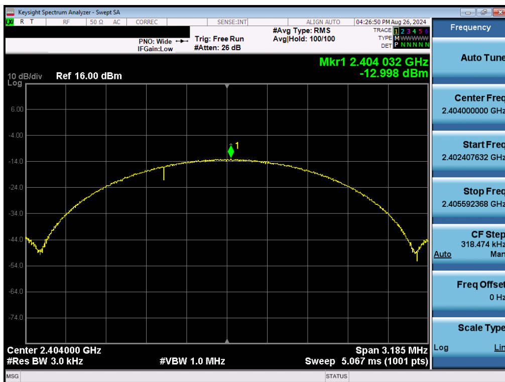
Plot 7-67. Power Spectral Density Plot Antenna 3a (Bluetooth (LE), 2Mbps, iPA – Ch. 1)
