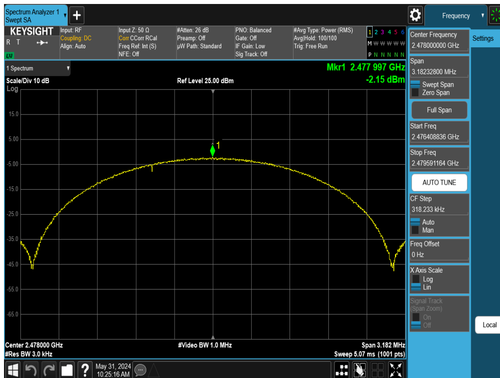
Plot 7-27. Power Spectral Density Plot Antenna 3a (Bluetooth (LE), 2Mbps, ePA – Ch. 38)
