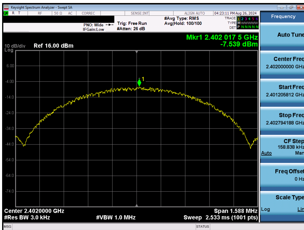
Plot 7-55. Power Spectral Density Plot Antenna 3a (Bluetooth (LE), 1Mbps, iPA – Ch. 0)
