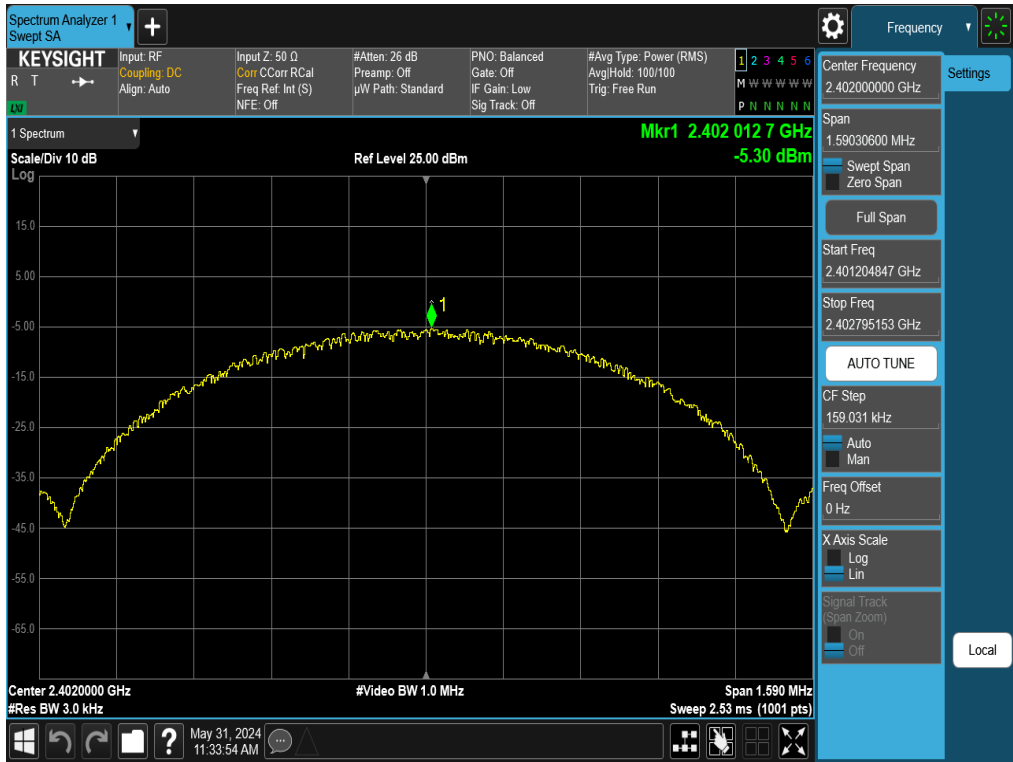
Plot 7-34. Power Spectral Density Plot Antenna 1a (Bluetooth (LE), 1Mbps, iPA – Ch. 0)
