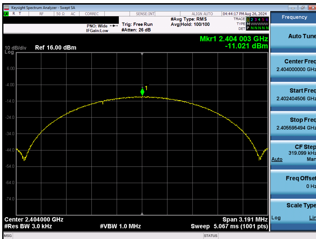
Plot 7-68. Power Spectral Density Plot Antenna 1a (Bluetooth (LE), 2Mbps, iPA – Ch. 1)
