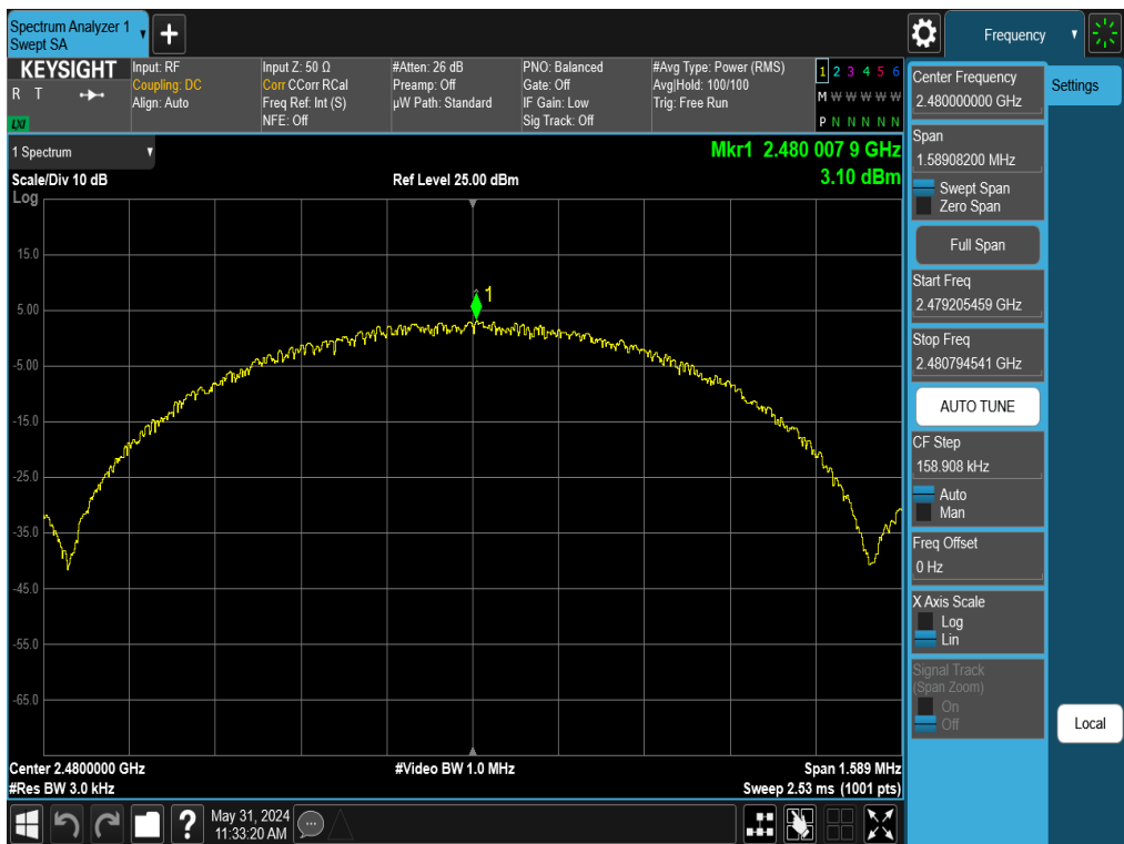
Plot 7-33. Power Spectral Density Plot Antenna 1a (Bluetooth (LE), 1Mbps, ePA – Ch. 39)
