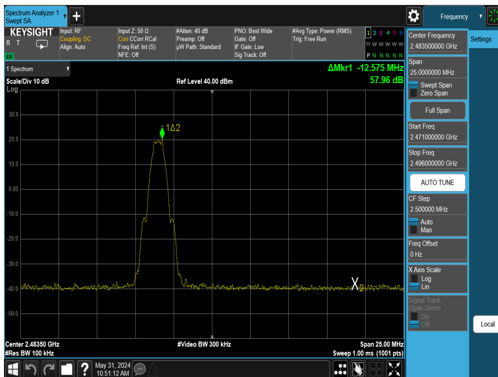
Plot 7-74. Band Edge Plot Antenna 3a (Bluetooth (LE), 1Mbps, ePA – Ch. 39)
