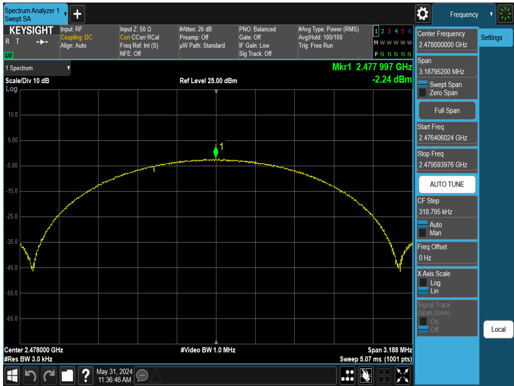
Plot 7-39. Power Spectral Density Plot Antenna 1a (Bluetooth (LE), 2Mbps, ePA – Ch. 38)
