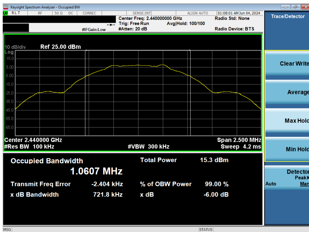
Plot 7-14. 6dB BW & 99% OBW Plot Antenna 4 (Bluetooth (LE), 1Mbps, iPA – Ch. 19)
