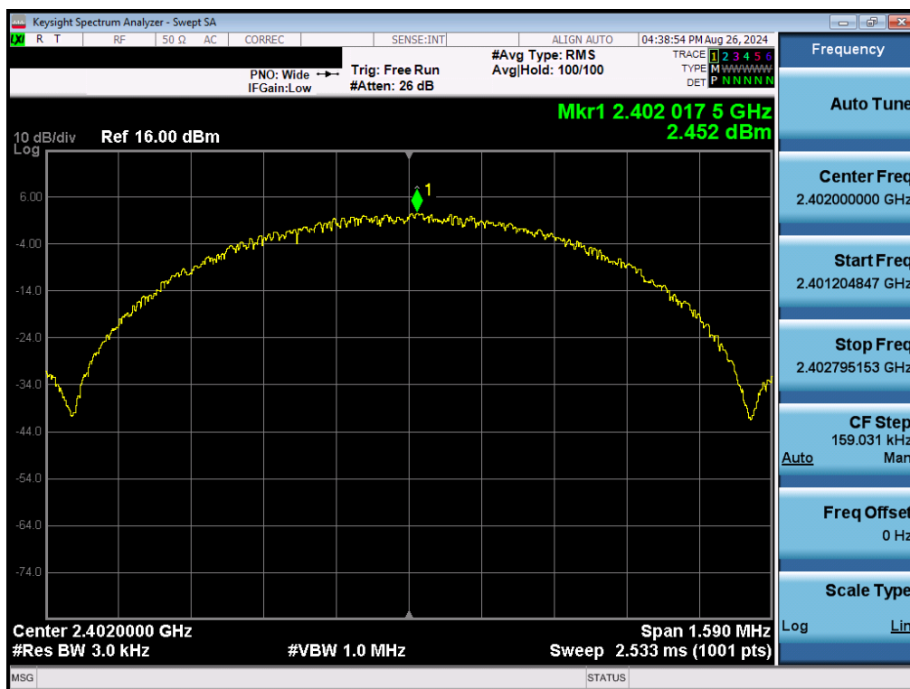
Plot 7-50. Power Spectral Density Plot Antenna 1a (Bluetooth (LE), 1Mbps, ePA – Ch. 0)
