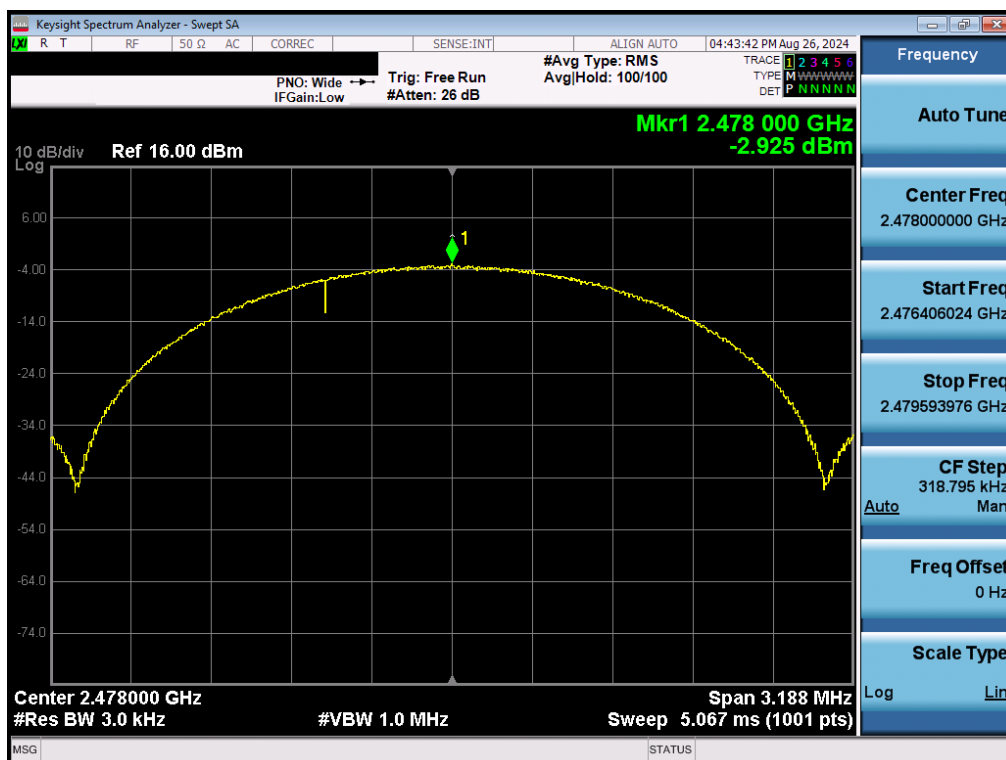
Plot 7-66. Power Spectral Density Plot Antenna 1a (Bluetooth (LE), 2Mbps, ePA – Ch. 38)
