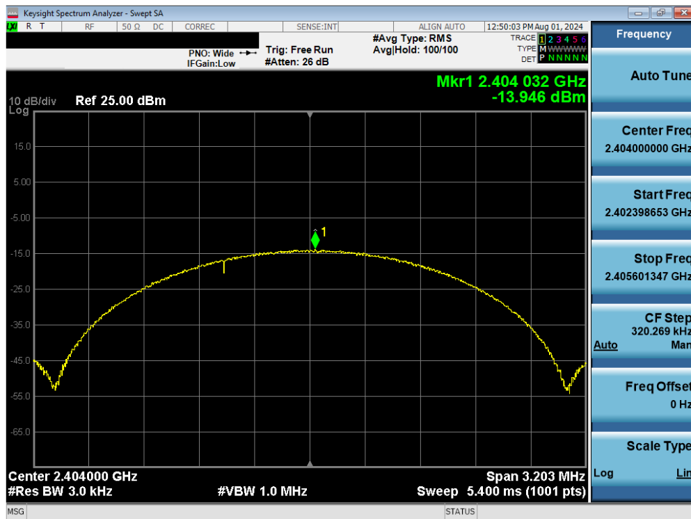
Plot 7-46. Power Spectral Density Plot Antenna 4 (Bluetooth (LE), 2Mbps, iPA – Ch. 1)
