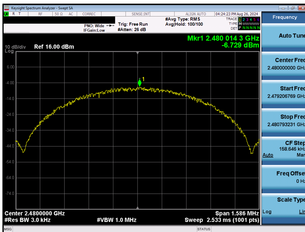
Plot 7-59. Power Spectral Density Plot Antenna 3a (Bluetooth (LE), 1Mbps, iPA – Ch. 39)
