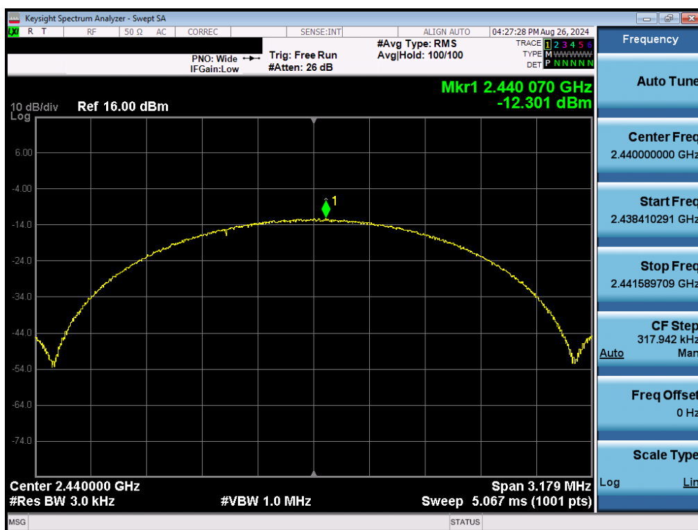
Plot 7-69. Power Spectral Density Plot Antenna 3a (Bluetooth (LE), 2Mbps, iPA – Ch. 19)
