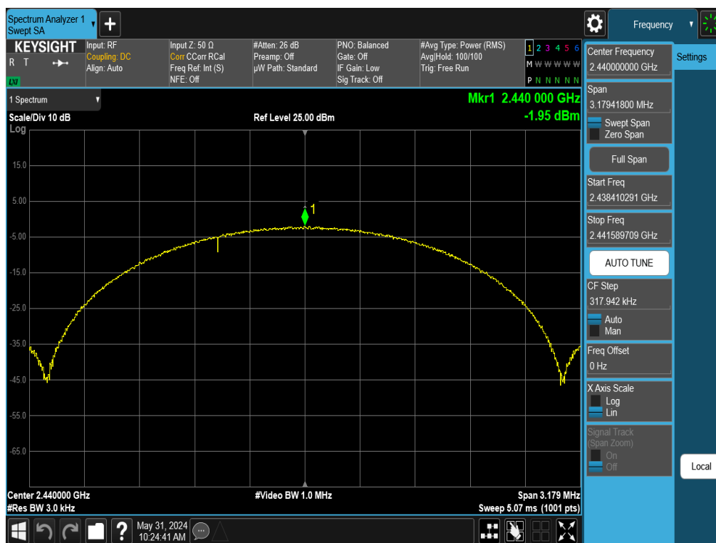
Plot 7-26. Power Spectral Density Plot Antenna 3a (Bluetooth (LE), 2Mbps, ePA – Ch. 19)
