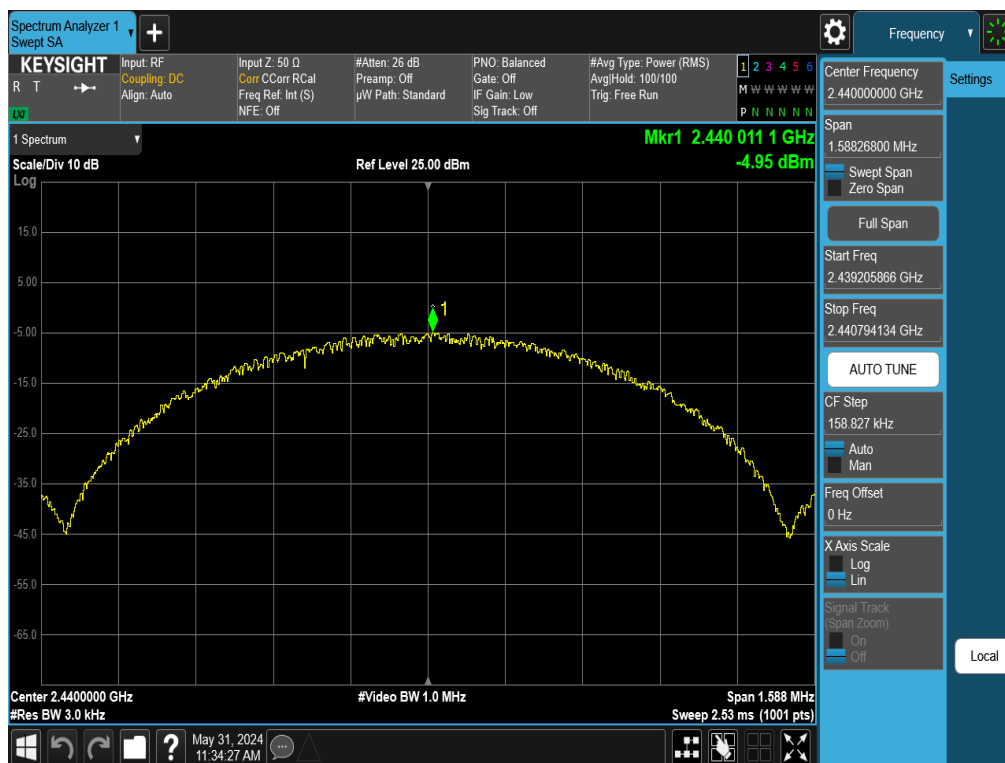
Plot 7-35. Power Spectral Density Plot Antenna 1a (Bluetooth (LE), 1Mbps, iPA – Ch. 19)
