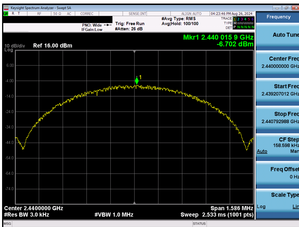
Plot 7-57. Power Spectral Density Plot Antenna 3a (Bluetooth (LE), 1Mbps, iPA – Ch. 19)
