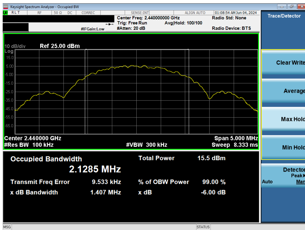
Plot 7-17. 6dB BW & 99% OBW Plot Antenna 4 (Bluetooth (LE), 2Mbps, iPA – Ch. 19)
