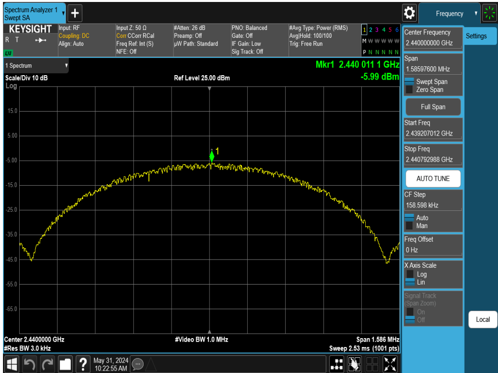
Plot 7-23. Power Spectral Density Plot Antenna 3a (Bluetooth (LE), 1Mbps, iPA – Ch. 19)
