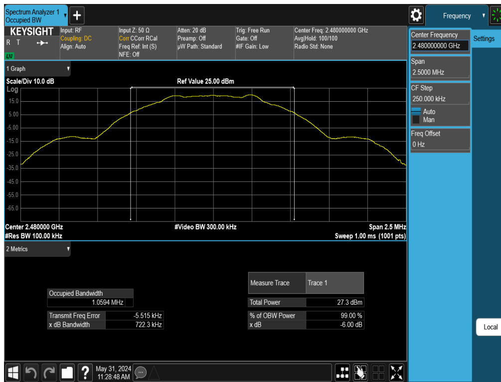
Plot 7-9. 6dB BW & 99% OBW Plot Antenna 1a (Bluetooth (LE), 1Mbps, ePA – Ch. 39)
