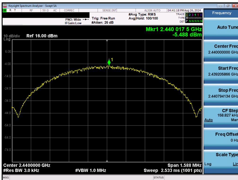
Plot 7-58. Power Spectral Density Plot Antenna 1a (Bluetooth (LE), 1Mbps, iPA – Ch. 19)
