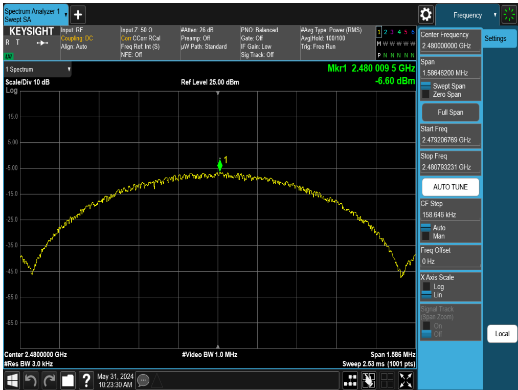
Plot 7-24. Power Spectral Density Plot Antenna 3a (Bluetooth (LE), 1Mbps, iPA – Ch. 39)
