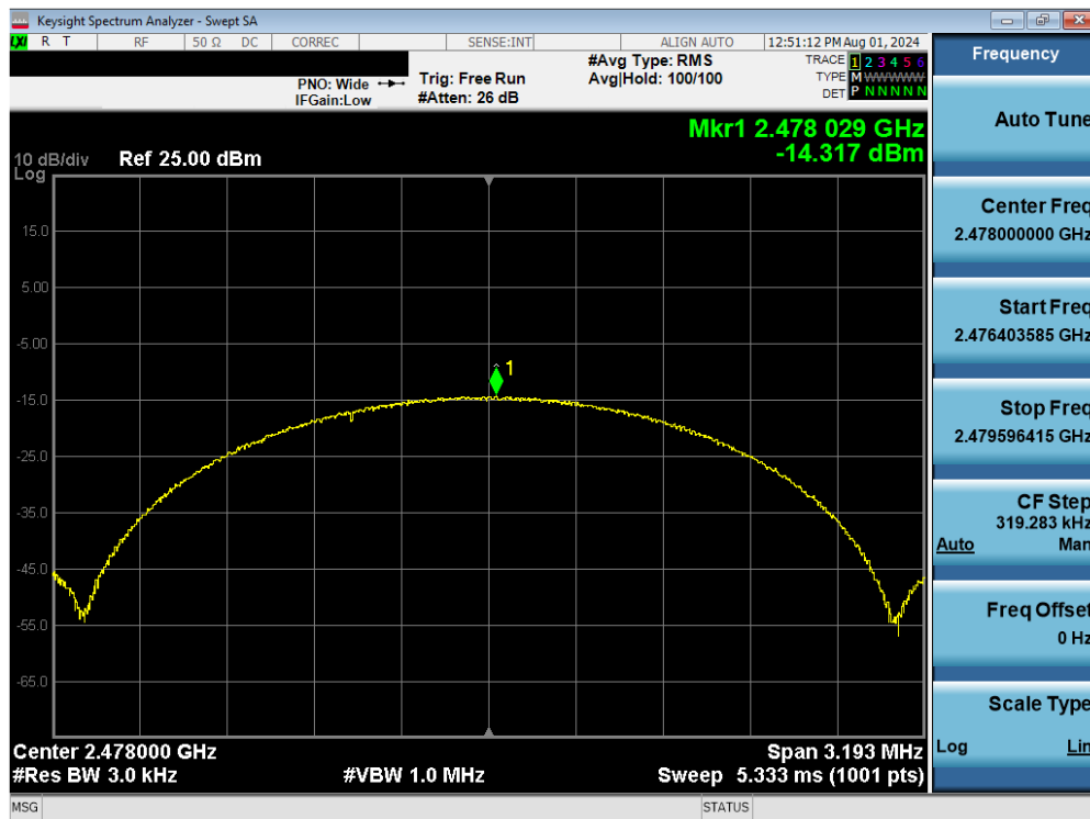
Plot 7-48. Power Spectral Density Plot Antenna 4 (Bluetooth (LE), 2Mbps, iPA – Ch. 38)
