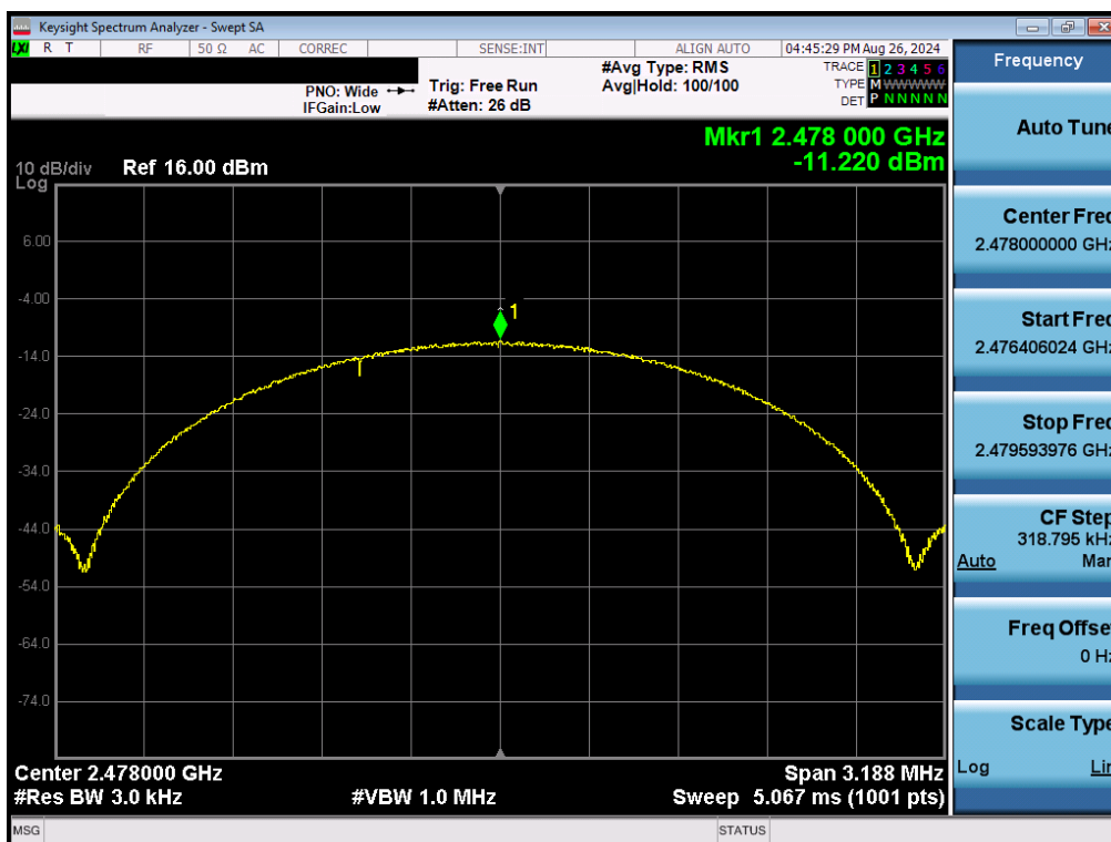
Plot 7-72. Power Spectral Density Plot Antenna 1a (Bluetooth (LE), 2Mbps, iPA – Ch. 38)
