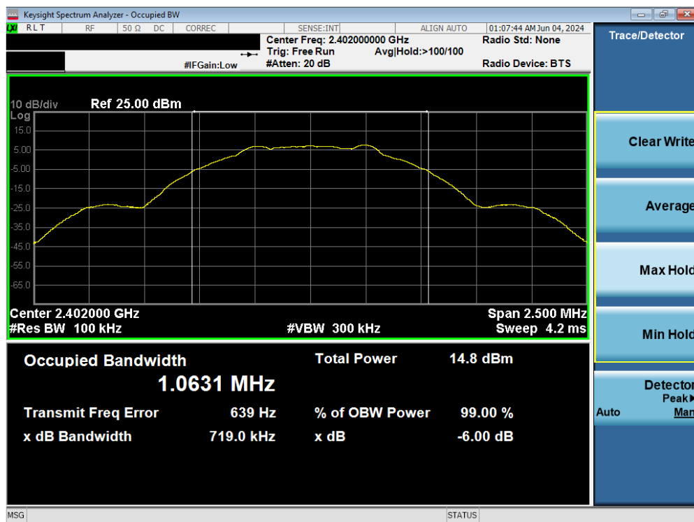
Plot 7-13. 6dB BW & 99% OBW Plot Antenna 4 (Bluetooth (LE), 1Mbps, iPA – Ch. 0)
