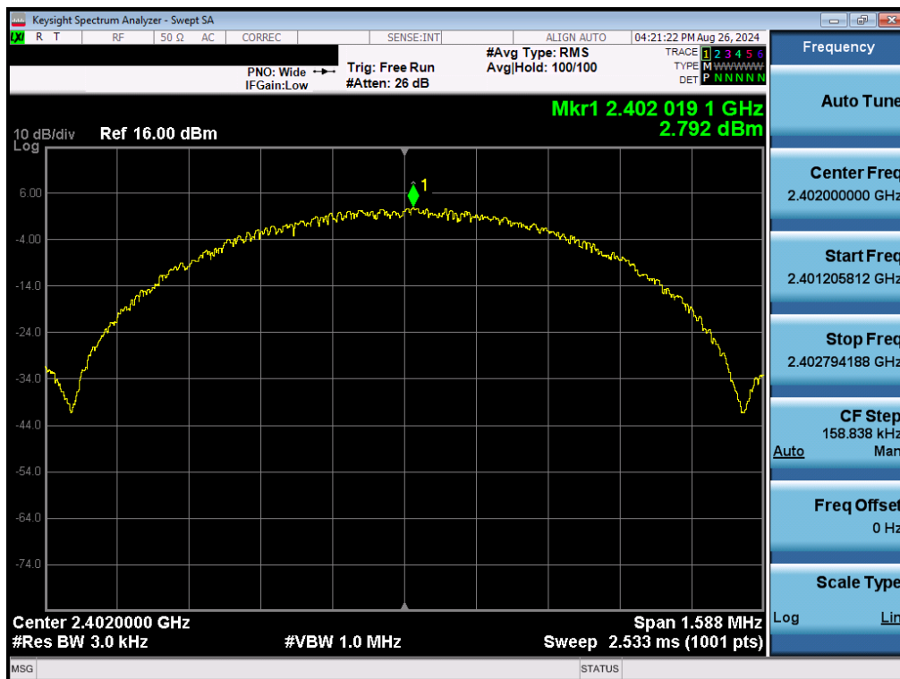
Plot 7-49. Power Spectral Density Plot Antenna 3a (Bluetooth (LE), 1Mbps, ePA – Ch. 0)
