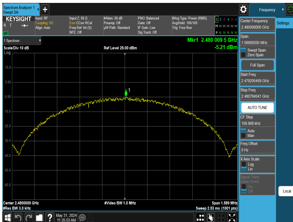
Plot 7-36. Power Spectral Density Plot Antenna 1a (Bluetooth (LE), 1Mbps, iPA – Ch. 39)
