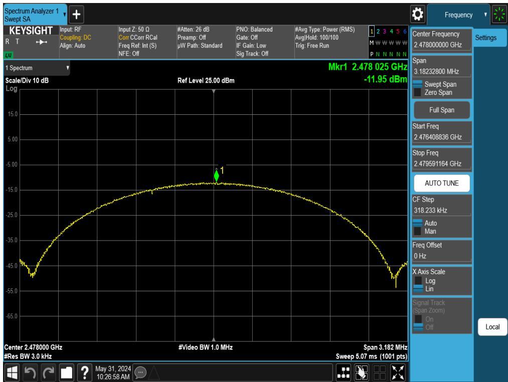
Plot 7-30. Power Spectral Density Plot Antenna 3a (Bluetooth (LE), 2Mbps, iPA – Ch. 38)
