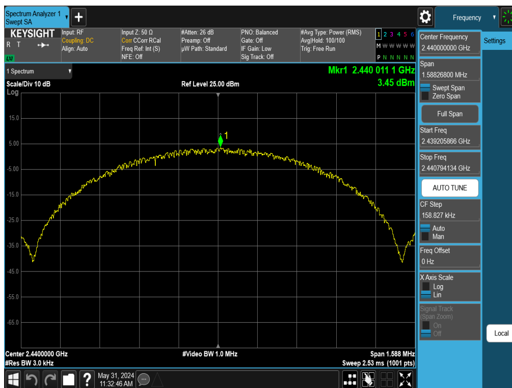
Plot 7-32. Power Spectral Density Plot Antenna 1a (Bluetooth (LE), 1Mbps, ePA – Ch. 19)
