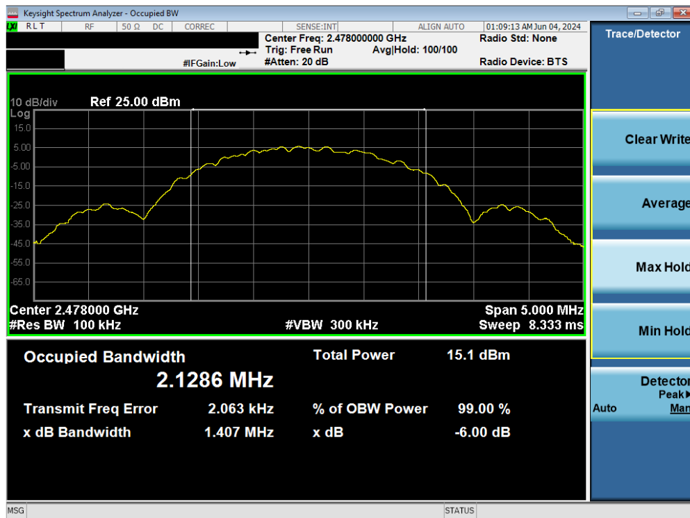
Plot 7-18. 6dB BW & 99% OBW Plot Antenna 4 (Bluetooth (LE), 2Mbps, iPA – Ch. 38)
