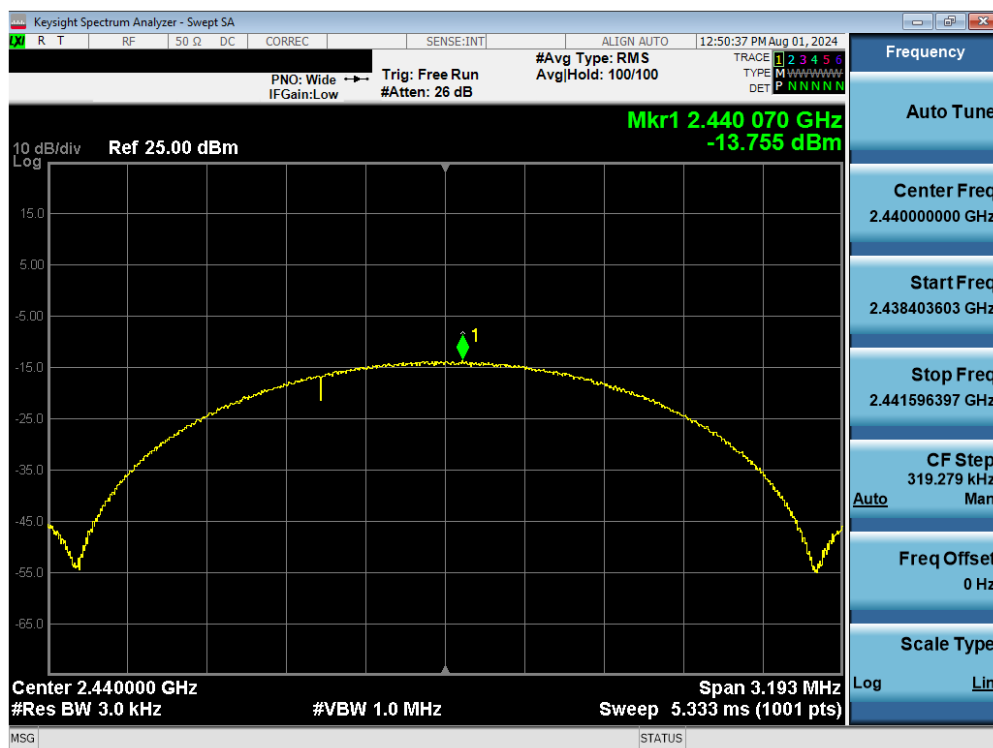
Plot 7-47. Power Spectral Density Plot Antenna 4 (Bluetooth (LE), 2Mbps, iPA – Ch. 19)
