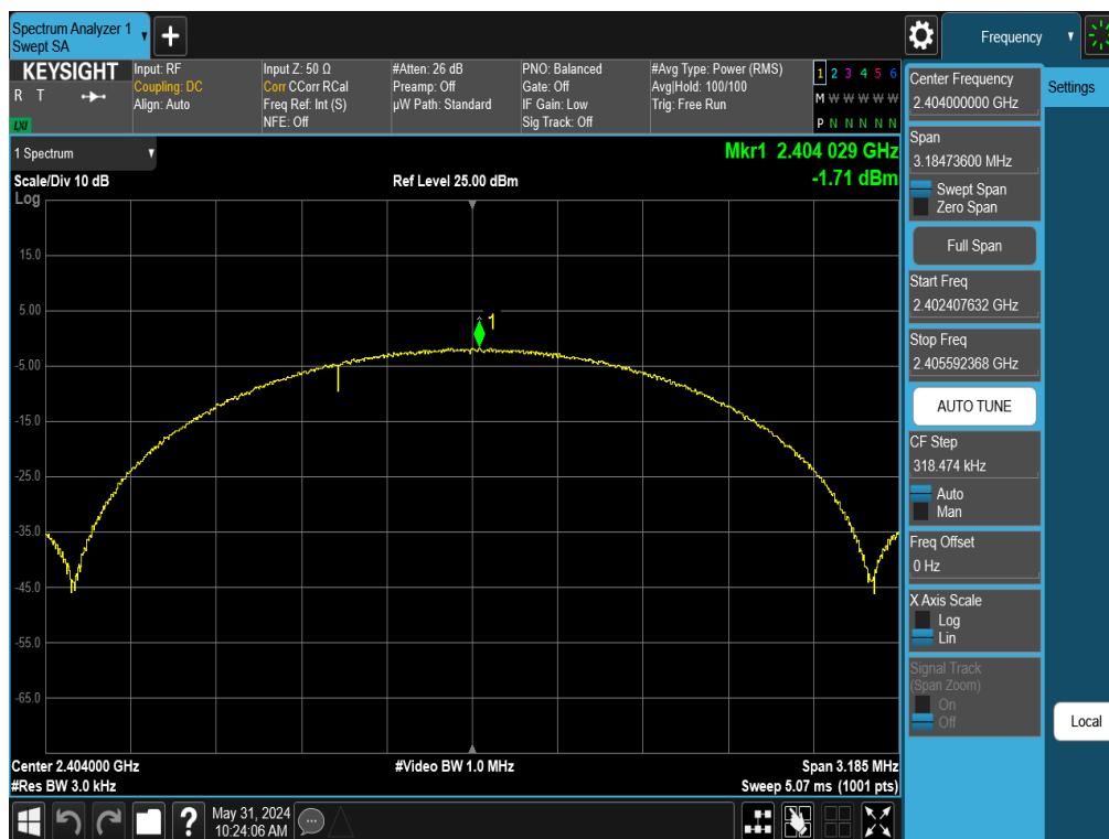
Plot 7-25. Power Spectral Density Plot Antenna 3a (Bluetooth (LE), 2Mbps, ePA – Ch. 1)
