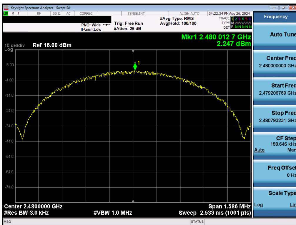
Plot 7-53. Power Spectral Density Plot Antenna 3a (Bluetooth (LE), 1Mbps, ePA – Ch. 39)
