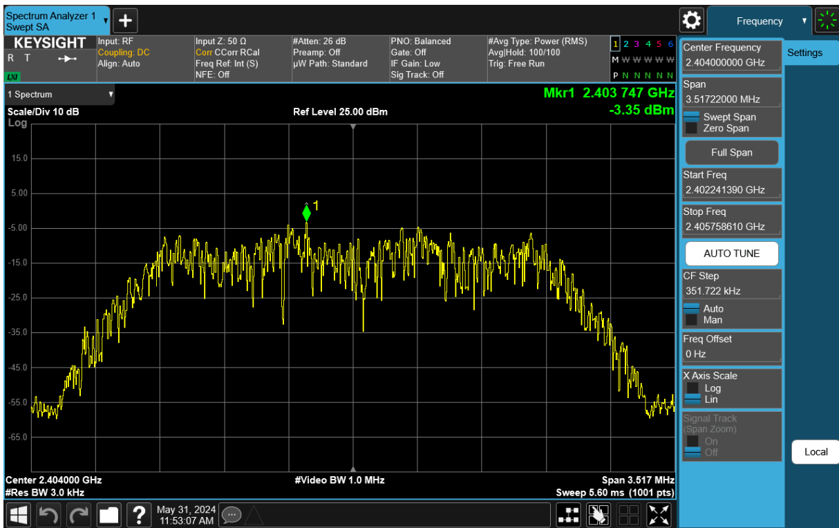
Plot 7-50. Power Spectral Density Plot Tx BF Antenna 1a (Bluetooth (HDR4), 4Mbps, ePA – Ch. 1)
