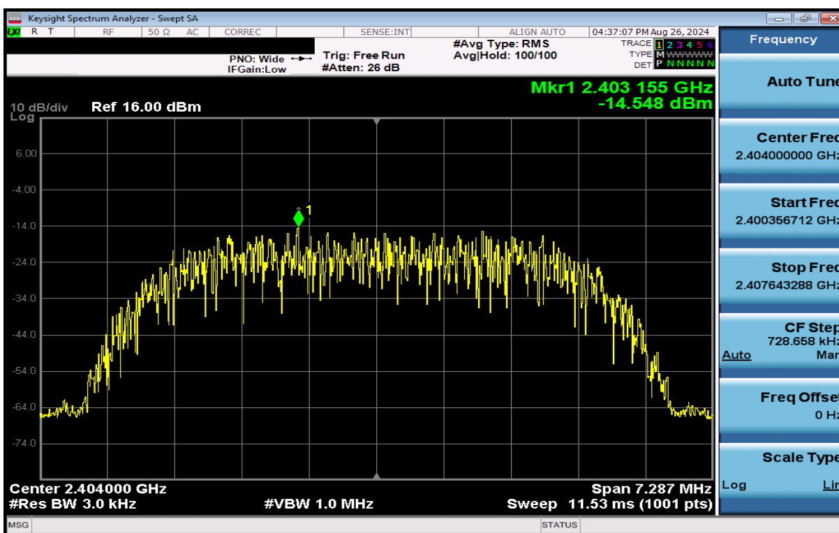
Plot 7-40. Power Spectral Density Plot Antenna 1a (Bluetooth (HDR8), 8Mbps, iPA – Ch. 1)
