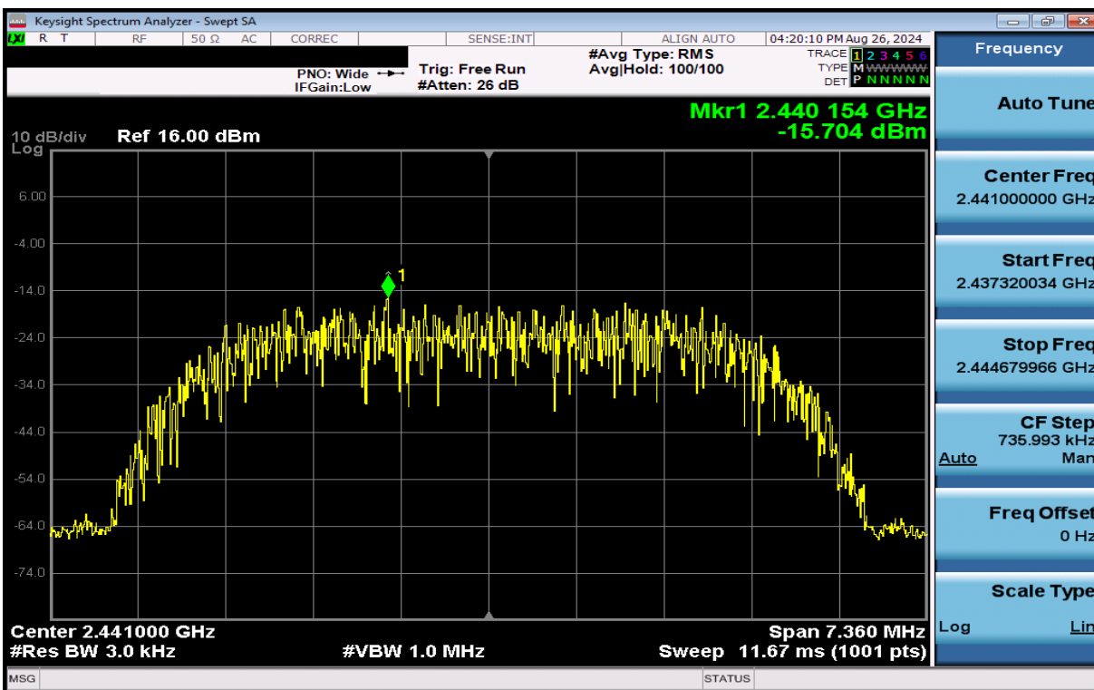
Plot 7-29. Power Spectral Density Plot Antenna 3a (Bluetooth (HDR8), 8Mbps, iPA – Ch. 38)
