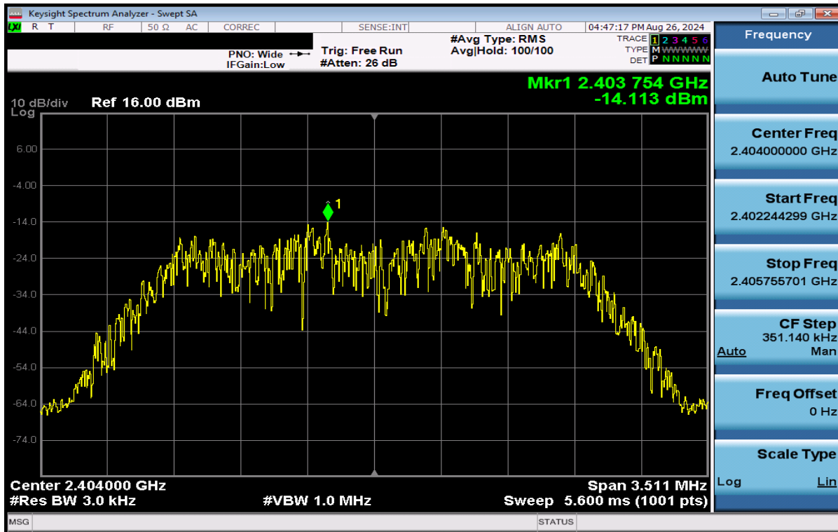
Plot 7-43. Power Spectral Density Plot Antenna 4 (Bluetooth (HDR4), 4Mbps, iPA – Ch. 1)
