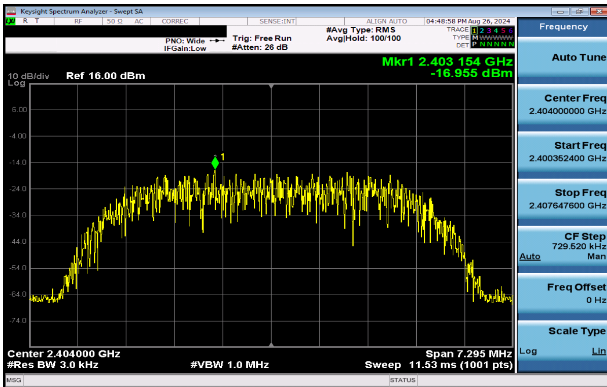
Plot 7-46. Power Spectral Density Plot Antenna 4 (Bluetooth (HDR8), 8Mbps, iPA – Ch. 1)
