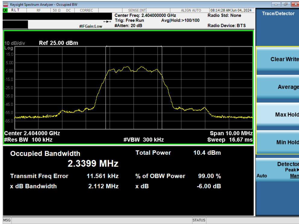
Plot 7-13. 6dB BW & 99% OBW Plot Antenna 4 (Bluetooth (HDR4), 4Mbps, iPA – Ch. 1)
