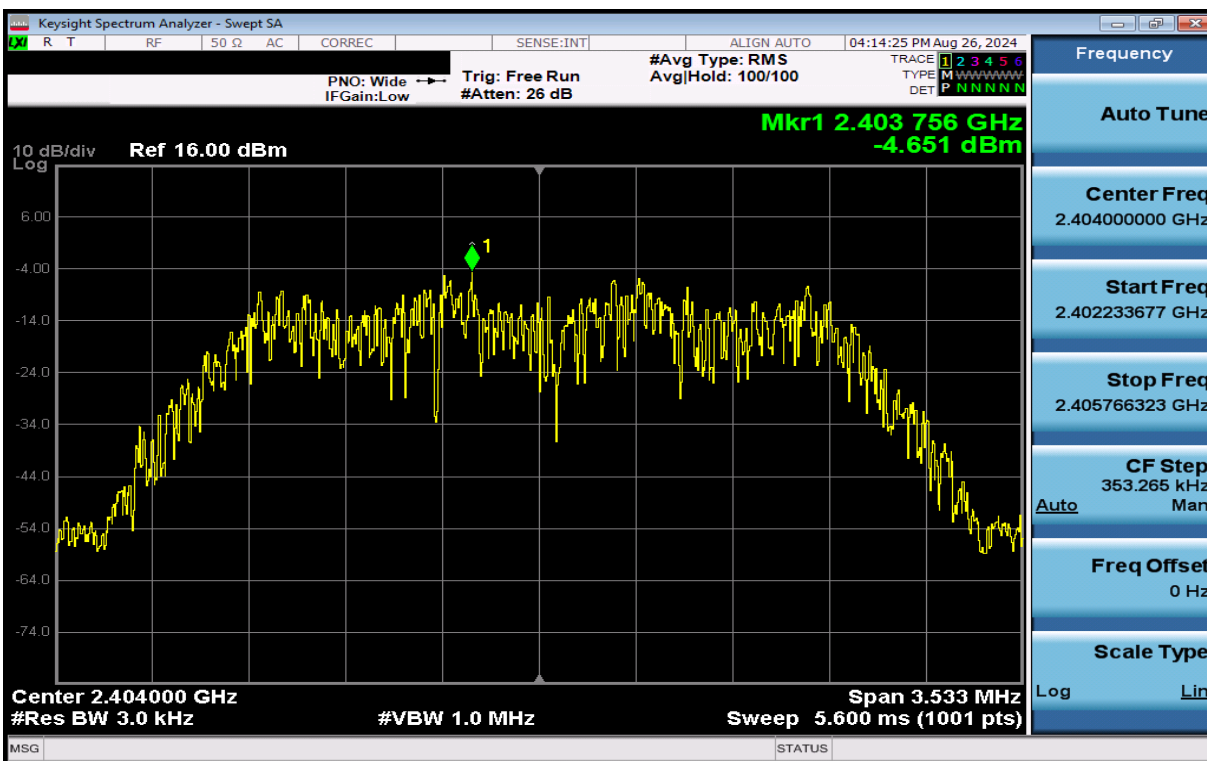
Plot 7-19. Power Spectral Density Plot Antenna 3a (Bluetooth (HDR4), 4Mbps, ePA – Ch. 1)
