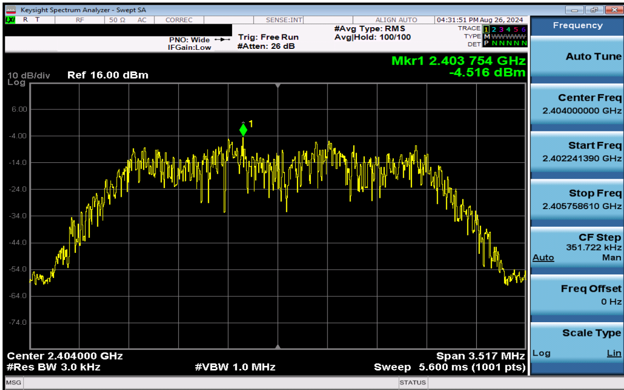
Plot 7-31. Power Spectral Density Plot Antenna 1a (Bluetooth (HDR4), 4Mbps, ePA – Ch. 1)
