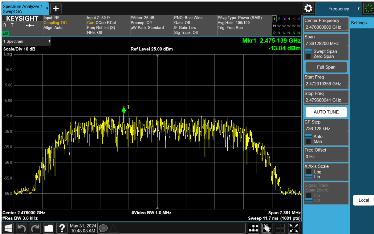
Plot 7-71. Power Spectral Density Plot TxBF Antenna 3a (Bluetooth (HDR8), 8Mbps, iPA – Ch. 73)
