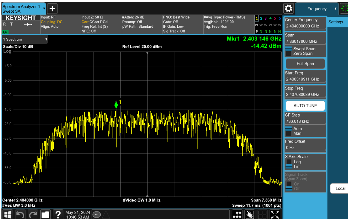
Plot 7-67. Power Spectral Density Plot Tx BF Antenna 3a (Bluetooth (HDR8), 8Mbps, iPA – Ch. 1)
