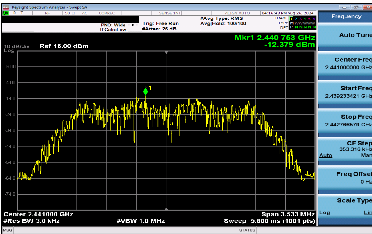
Plot 7-23. Power Spectral Density Plot Antenna 3a (Bluetooth (HDR4), 4Mbps, iPA – Ch. 38)
