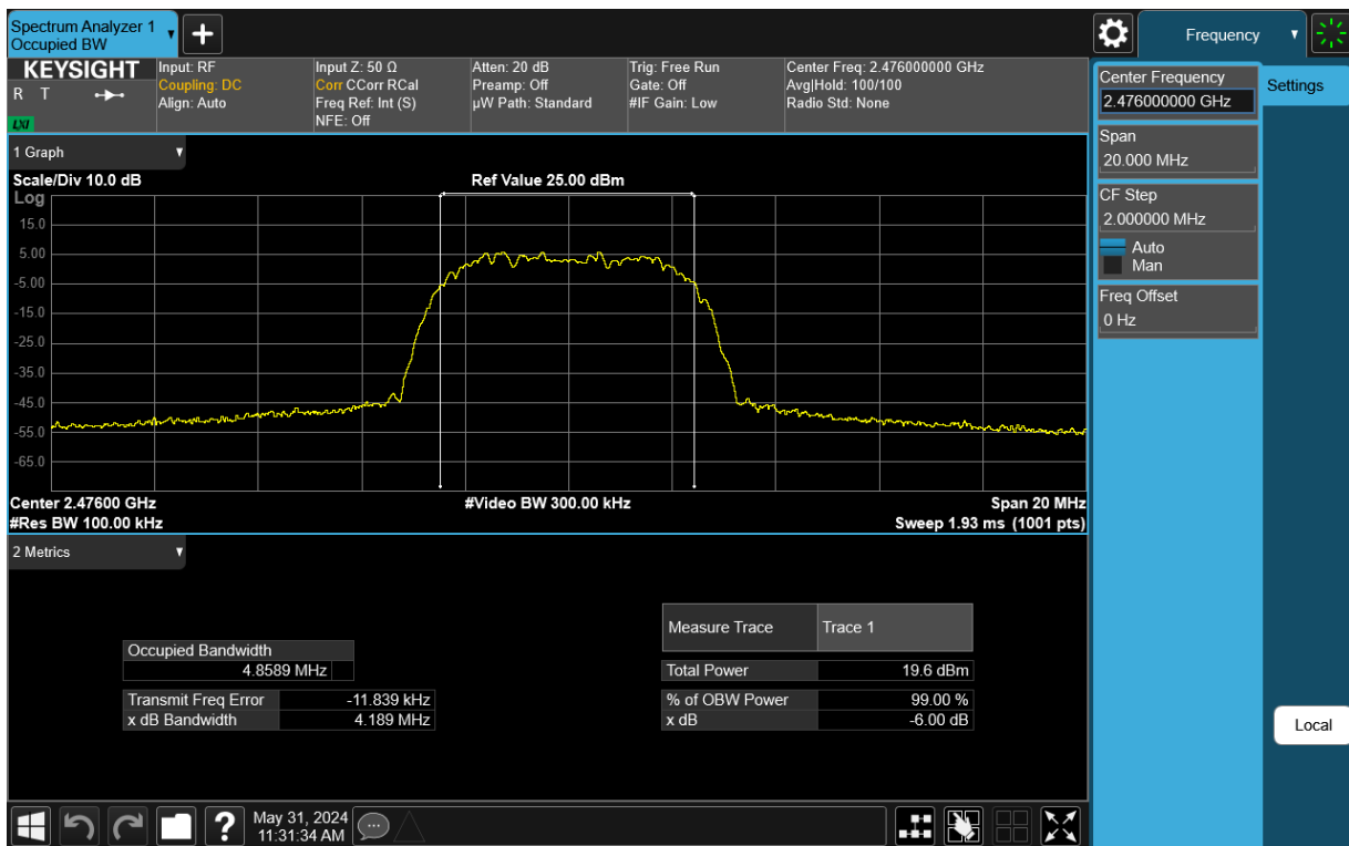
Plot 7-12. 6dB BW & 99% OBW Plot Antenna 1a (Bluetooth (HDR8), 8Mbps, ePA – Ch. 73)
