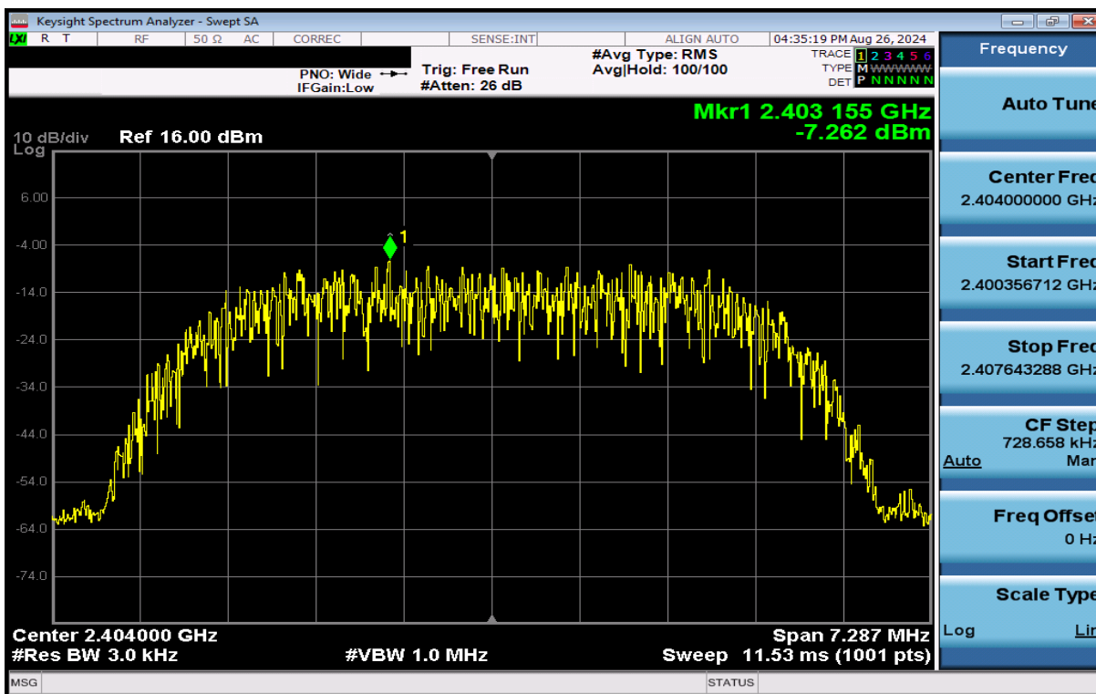
Plot 7-37. Power Spectral Density Plot Antenna 1a (Bluetooth (HDR8), 8Mbps, ePA – Ch. 1)
