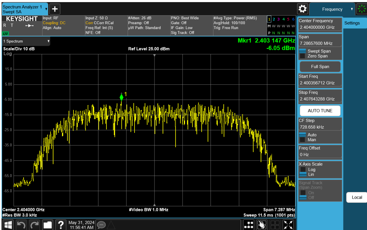
Plot 7-62. Power Spectral Density Plot TxBF Antenna 1a (Bluetooth (HDR8), 8Mbps, ePA – Ch. 1)
