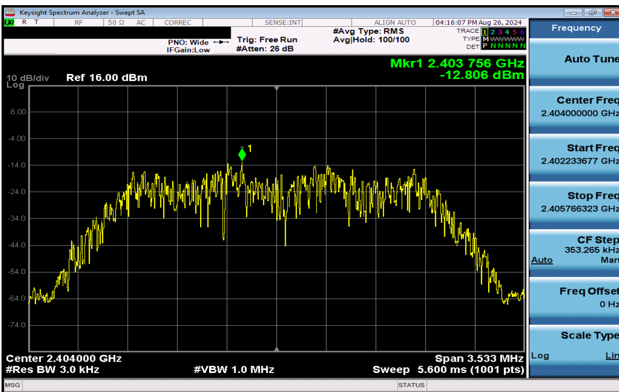
Plot 7-22. Power Spectral Density Plot Antenna 3a (Bluetooth (HDR4), 4Mbps, iPA – Ch. 1)
