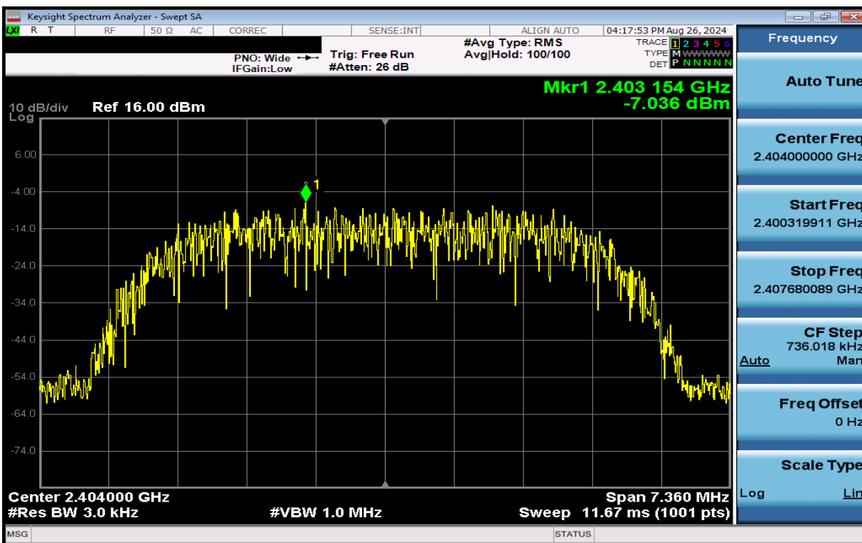
Plot 7-25. Power Spectral Density Plot Antenna 3a (Bluetooth (HDR8), 8Mbps, ePA – Ch. 1)
