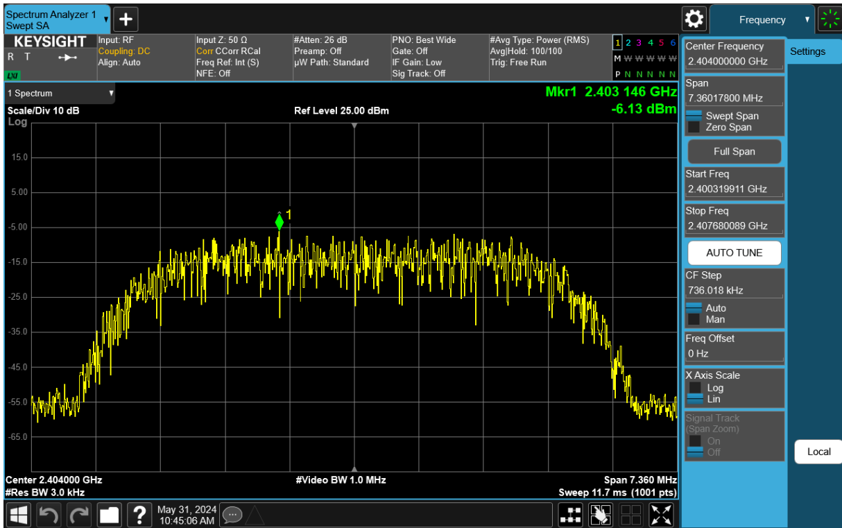
Plot 7-61. Power Spectral Density Plot TxBF Antenna 3a (Bluetooth (HDR8), 8Mbps, ePA – Ch. 1)
