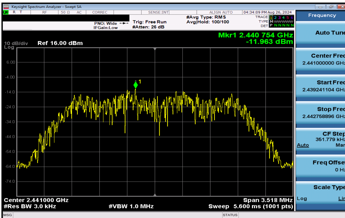
Plot 7-35. Power Spectral Density Plot Antenna 1a (Bluetooth (HDR4), 4Mbps, iPA – Ch. 38)
