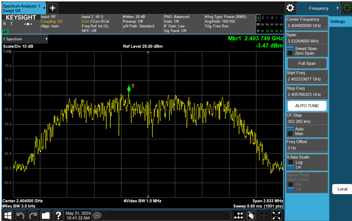
Plot 7-49. Power Spectral Density Plot Tx BF Antenna 3a (Bluetooth (HDR4), 4Mbps, ePA – Ch. 1)
