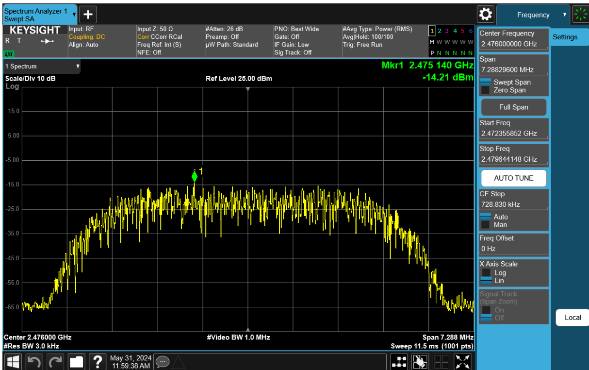
Plot 7-72. Power Spectral Density Plot TxBF Antenna 1a (Bluetooth (HDR8), 8Mbps, iPA – Ch. 73)
