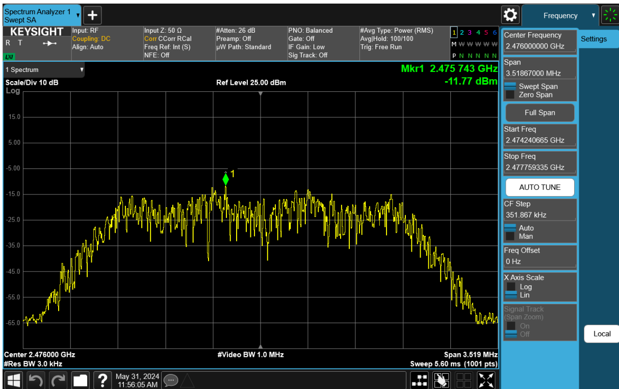
Plot 7-60. Power Spectral Density Plot TxBF Antenna 1a (Bluetooth (HDR4), 4Mbps, iPA – Ch. 73)
