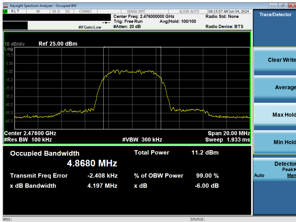
Plot 7-18. 6dB BW & 99% OBW Plot Antenna 4 (Bluetooth (HDR8), 8Mbps, iPA – Ch. 73)
