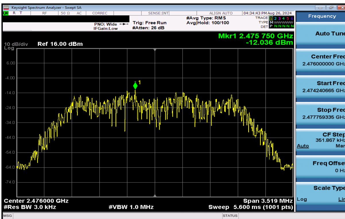
Plot 7-36. Power Spectral Density Plot Antenna 1a (Bluetooth (HDR4), 4Mbps, iPA – Ch. 73)
