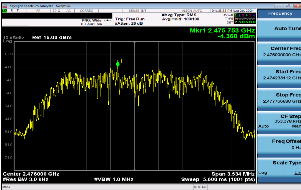
Plot 7-21. Power Spectral Density Plot Antenna 3a (Bluetooth (HDR4), 4Mbps, ePA – Ch. 73)
