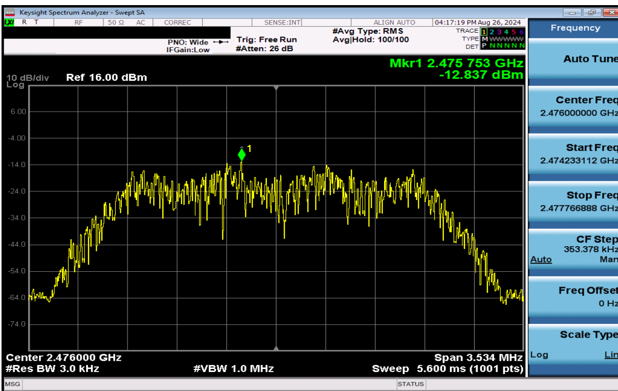
Plot 7-24. Power Spectral Density Plot Antenna 3a (Bluetooth (HDR4), 4Mbps, iPA – Ch. 73)
