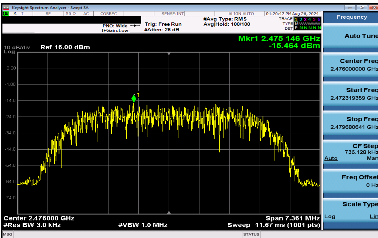
Plot 7-30. Power Spectral Density Plot Antenna 3a (Bluetooth (HDR8), 8Mbps, iPA – Ch. 73)
