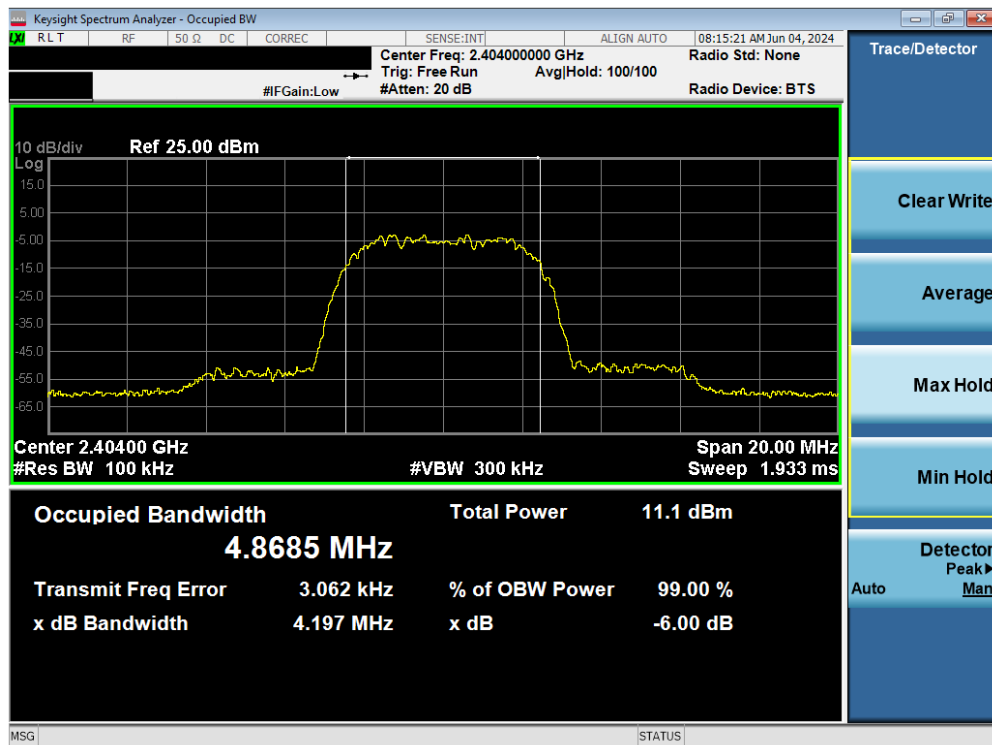
Plot 7-16. 6dB BW & 99% OBW Plot Antenna 4 (Bluetooth (HDR8), 8Mbps, iPA – Ch. 1)
