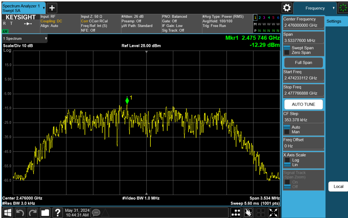
Plot 7-59. Power Spectral Density Plot TxBF Antenna 3a (Bluetooth (HDR4), 4Mbps, iPA – Ch. 73)
