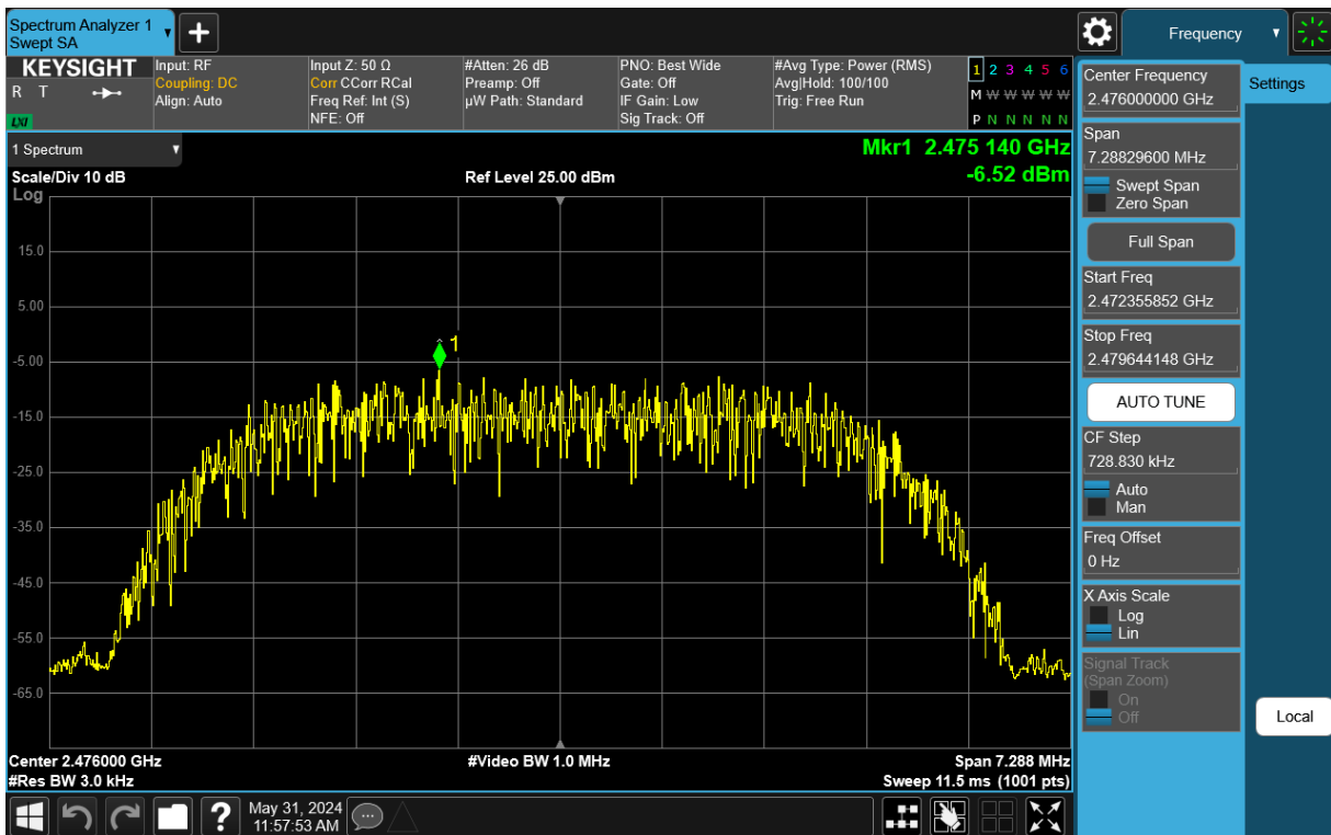
Plot 7-66. Power Spectral Density Plot TxBF Antenna 1a (Bluetooth (HDR8), 8Mbps, ePA – Ch. 73)
