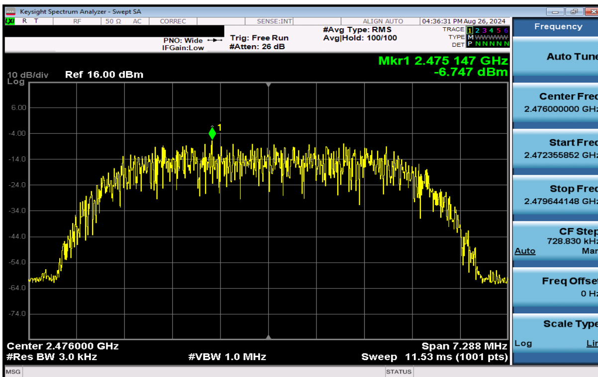
Plot 7-39. Power Spectral Density Plot Antenna 1a (Bluetooth (HDR8), 8Mbps, ePA – Ch. 73)
