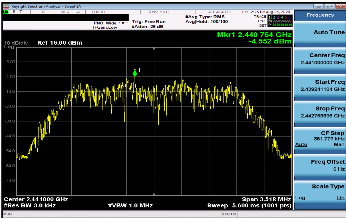
Plot 7-32. Power Spectral Density Plot Antenna 1a (Bluetooth (HDR4), 4Mbps, ePA – Ch. 38)
