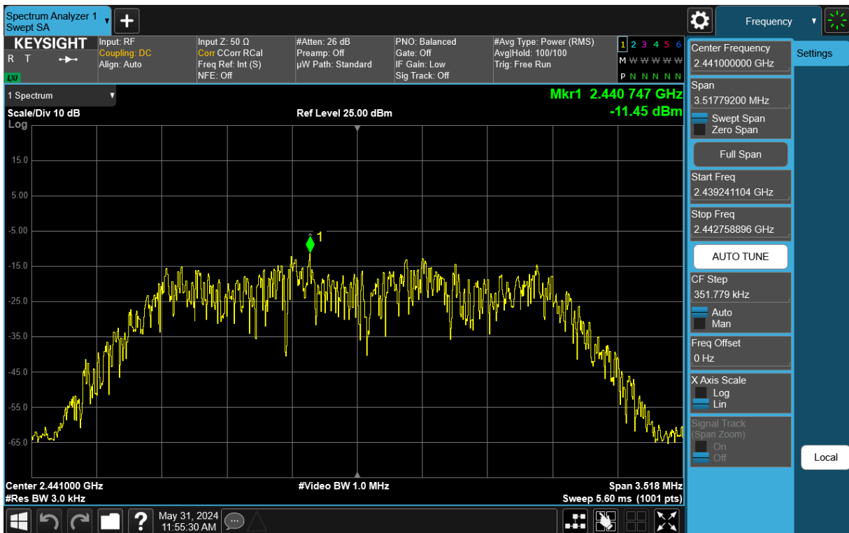
Plot 7-58. Power Spectral Density Plot TxBF Antenna 1a (Bluetooth (HDR4), 4Mbps, iPA – Ch. 38)
