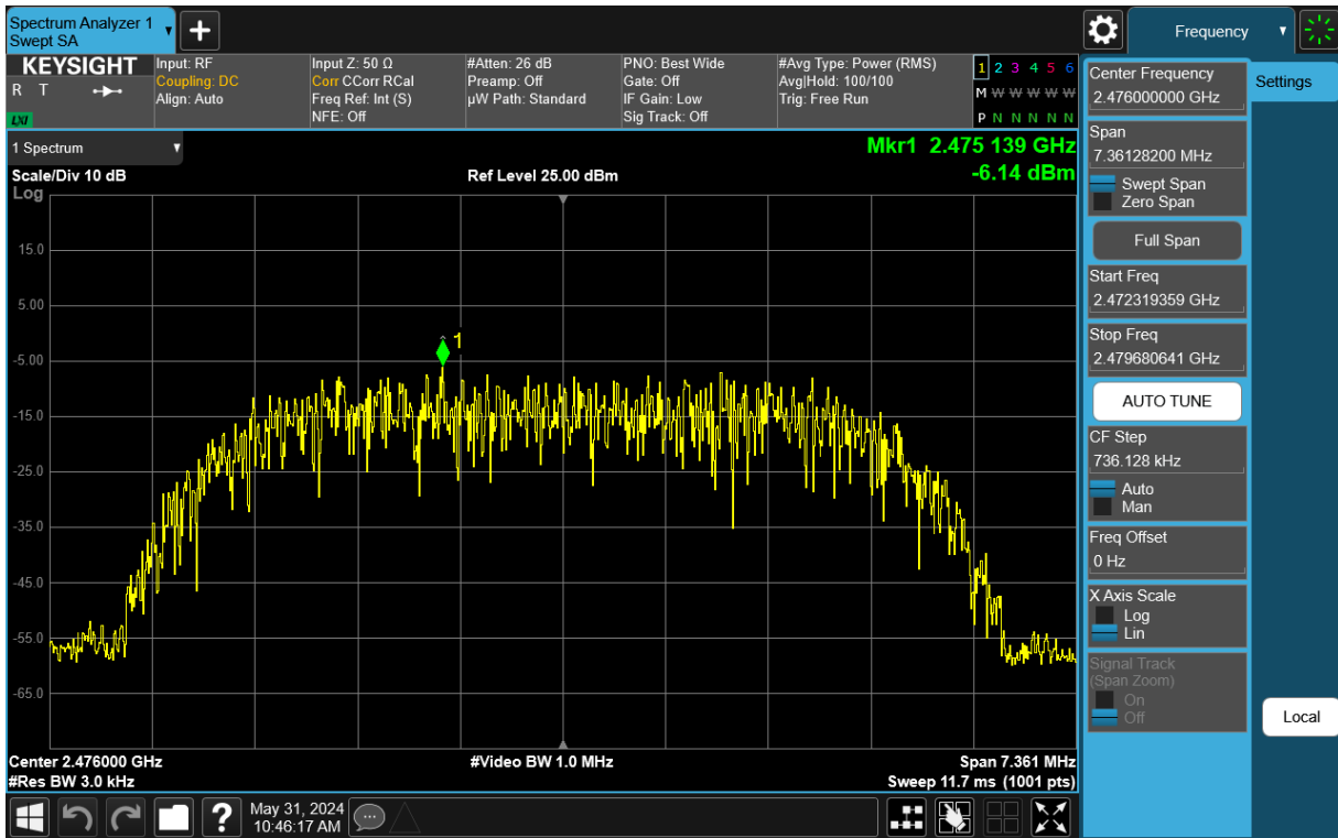
Plot 7-65. Power Spectral Density Plot TxBF Antenna 3a (Bluetooth (HDR8), 8Mbps, ePA – Ch. 73)
