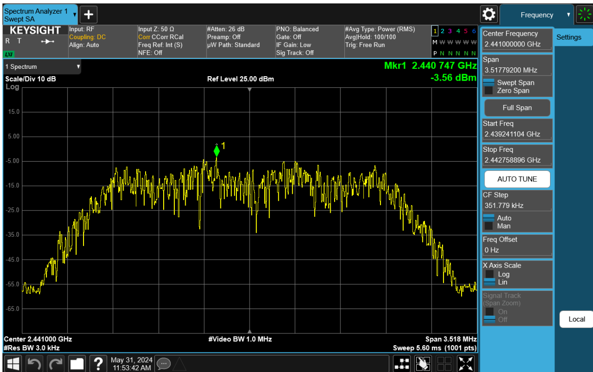
Plot 7-52. Power Spectral Density Plot TxBF Antenna 1a (Bluetooth (HDR4), 4Mbps, ePA – Ch. 38)
