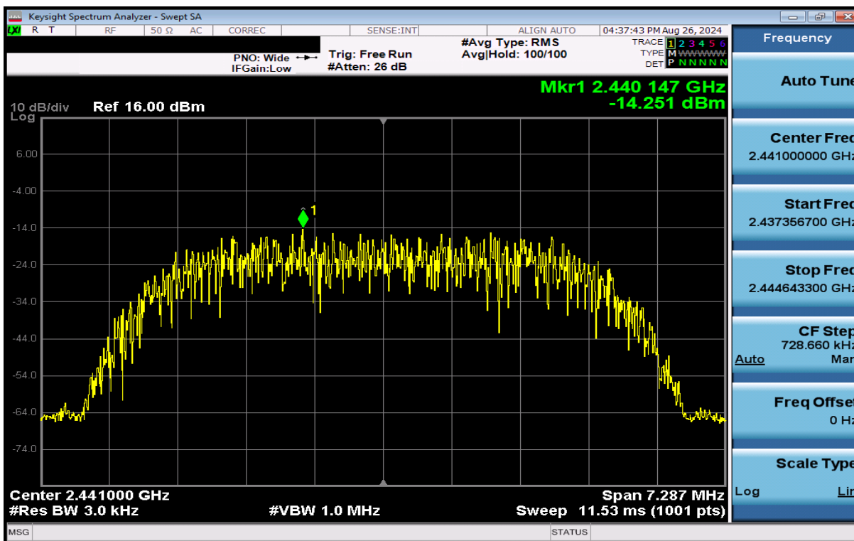
Plot 7-41. Power Spectral Density Plot Antenna 1a (Bluetooth (HDR8), 8Mbps, iPA – Ch. 38)
