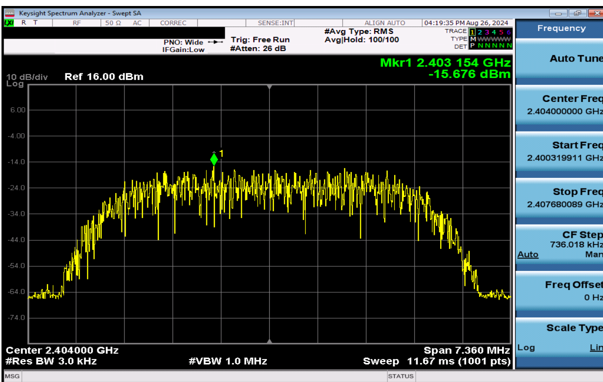
Plot 7-28. Power Spectral Density Plot Antenna 3a (Bluetooth (HDR8), 8Mbps, iPA – Ch. 1)
