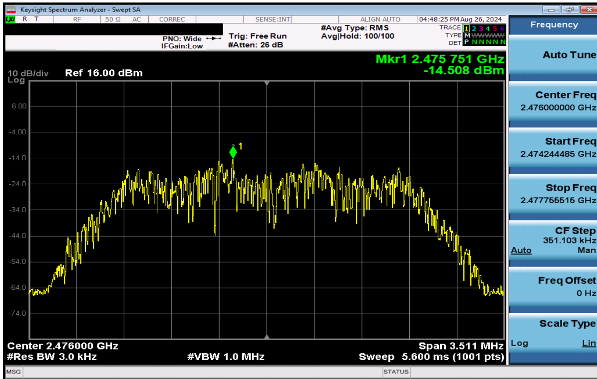
Plot 7-45. Power Spectral Density Plot Antenna 4 (Bluetooth (HDR4), 4Mbps, iPA – Ch. 73)
