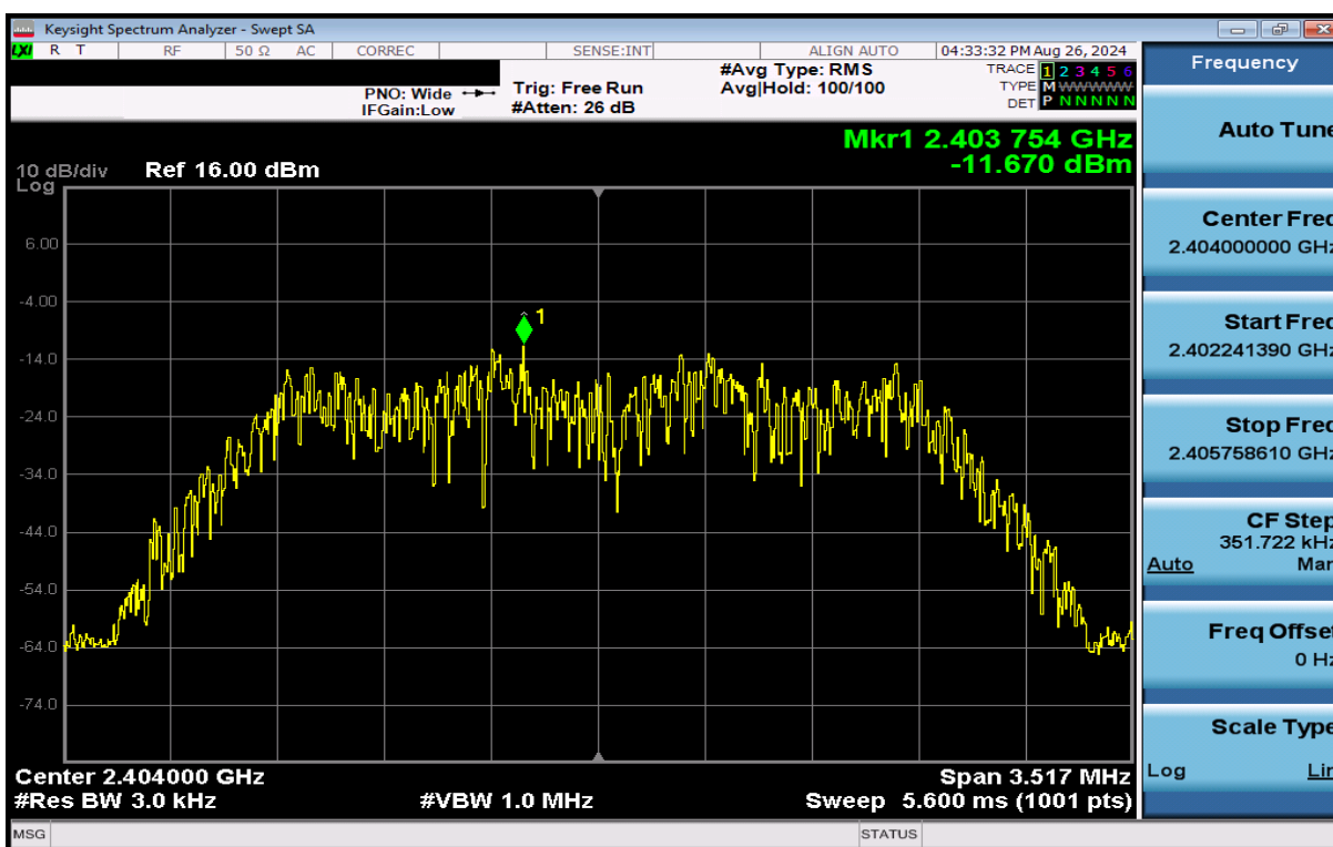
Plot 7-34. Power Spectral Density Plot Antenna 1a (Bluetooth (HDR4), 4Mbps, iPA – Ch. 1)
