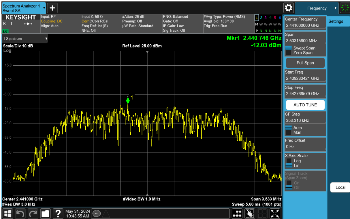
Plot 7-57. Power Spectral Density Plot TxBF Antenna 3a (Bluetooth (HDR4), 4Mbps, iPA – Ch. 38)
