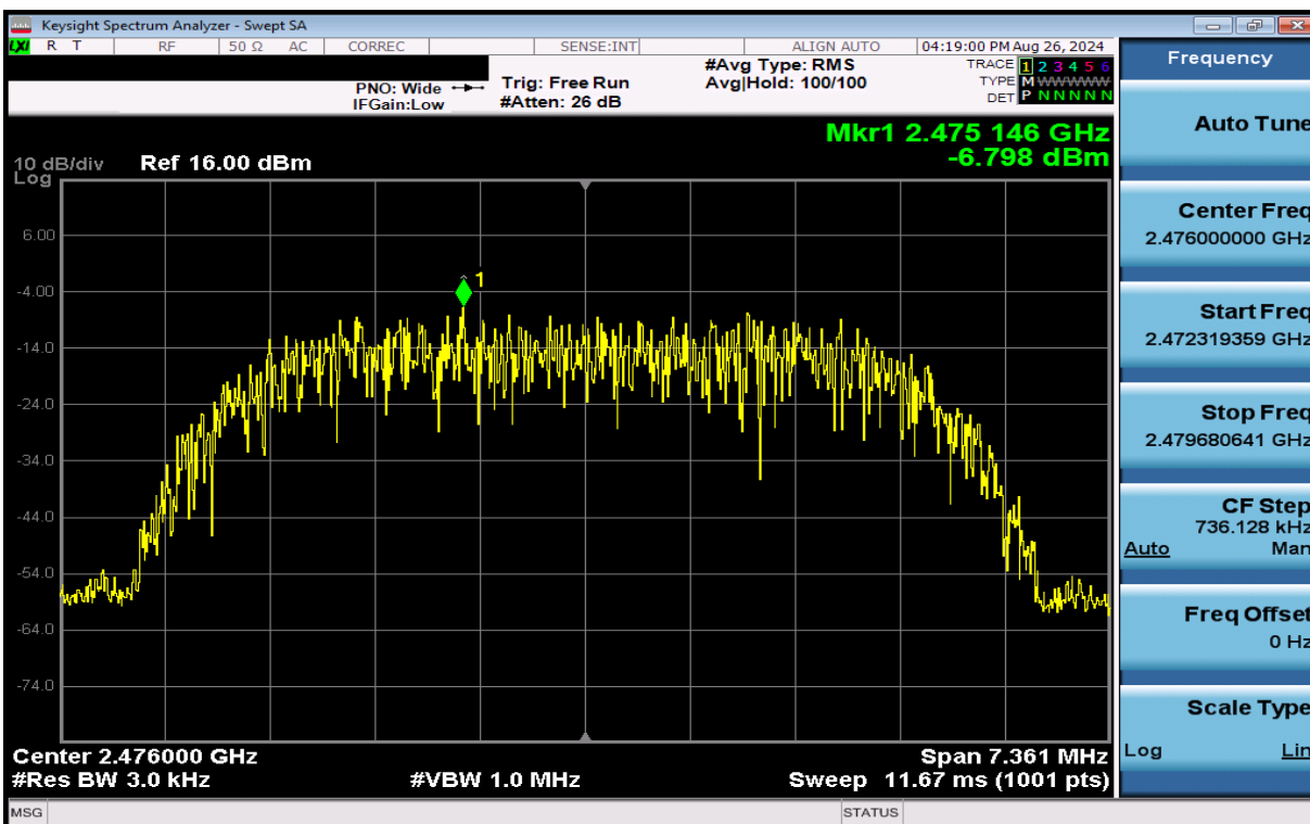
Plot 7-27. Power Spectral Density Plot Antenna 3a (Bluetooth (HDR8), 8Mbps, ePA – Ch. 73)
