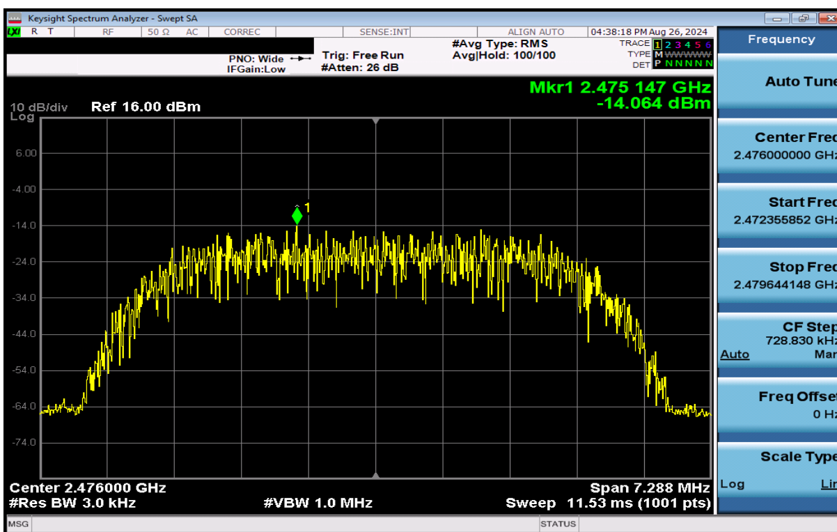
Plot 7-42. Power Spectral Density Plot Antenna 1a (Bluetooth (HDR8), 8Mbps, iPA – Ch. 73)
