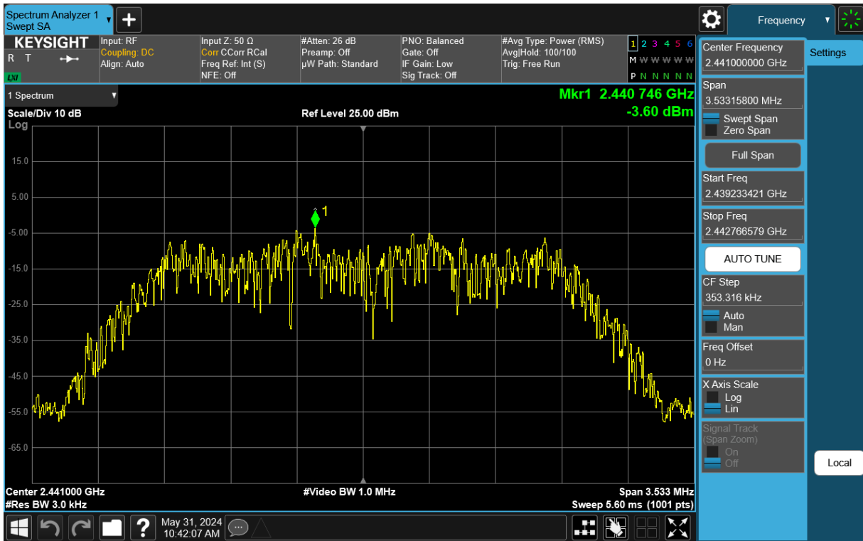
Plot 7-51. Power Spectral Density Plot TxBF Antenna 3a (Bluetooth (HDR4), 4Mbps, ePA – Ch. 38)
