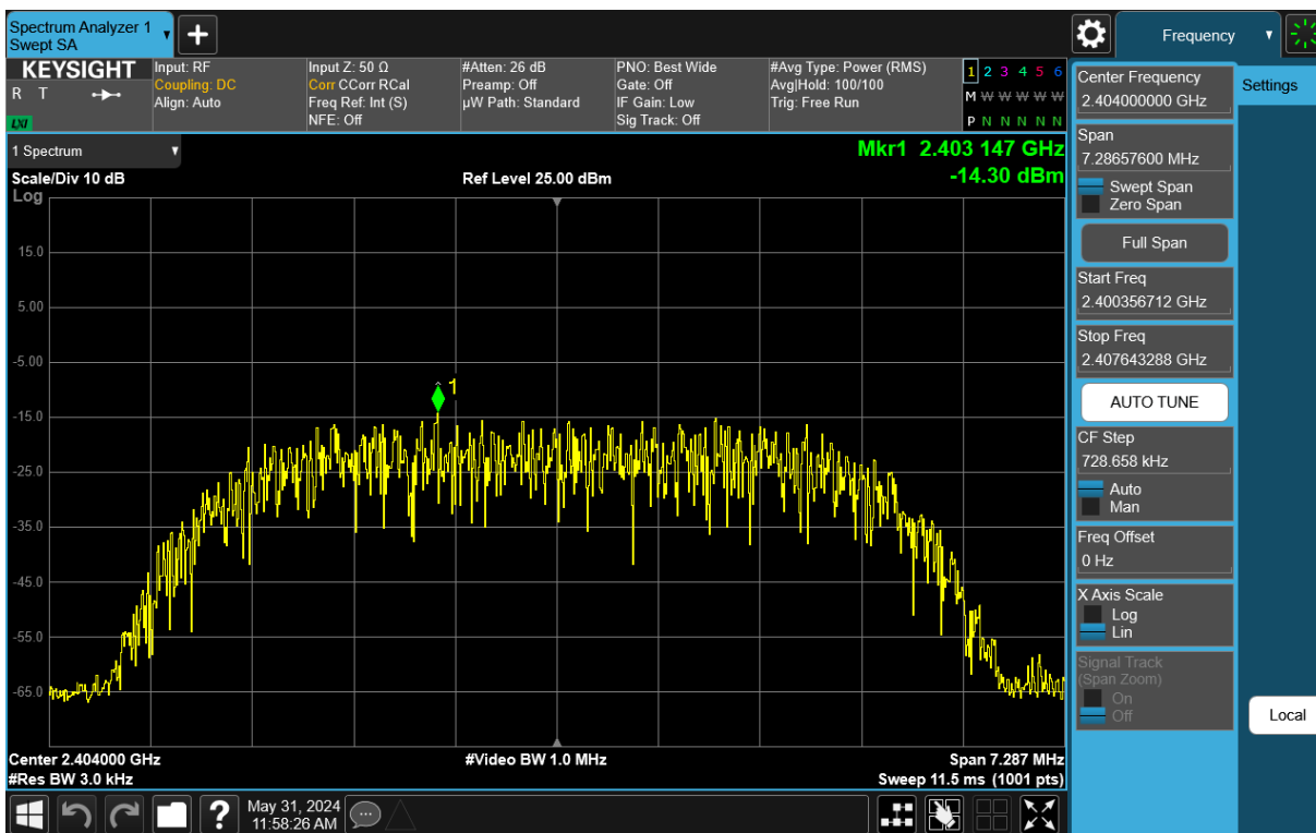
Plot 7-68. Power Spectral Density Plot Tx BF Antenna 1a (Bluetooth (HDR8), 8Mbps, iPA – Ch. 1)
