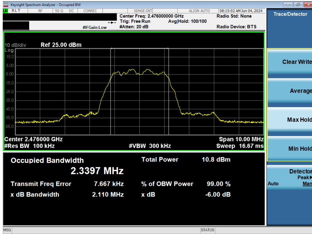
Plot 7-15. 6dB BW & 99% OBW Plot Antenna 4 (Bluetooth (HDR4), 4Mbps, iPA – Ch. 73)
