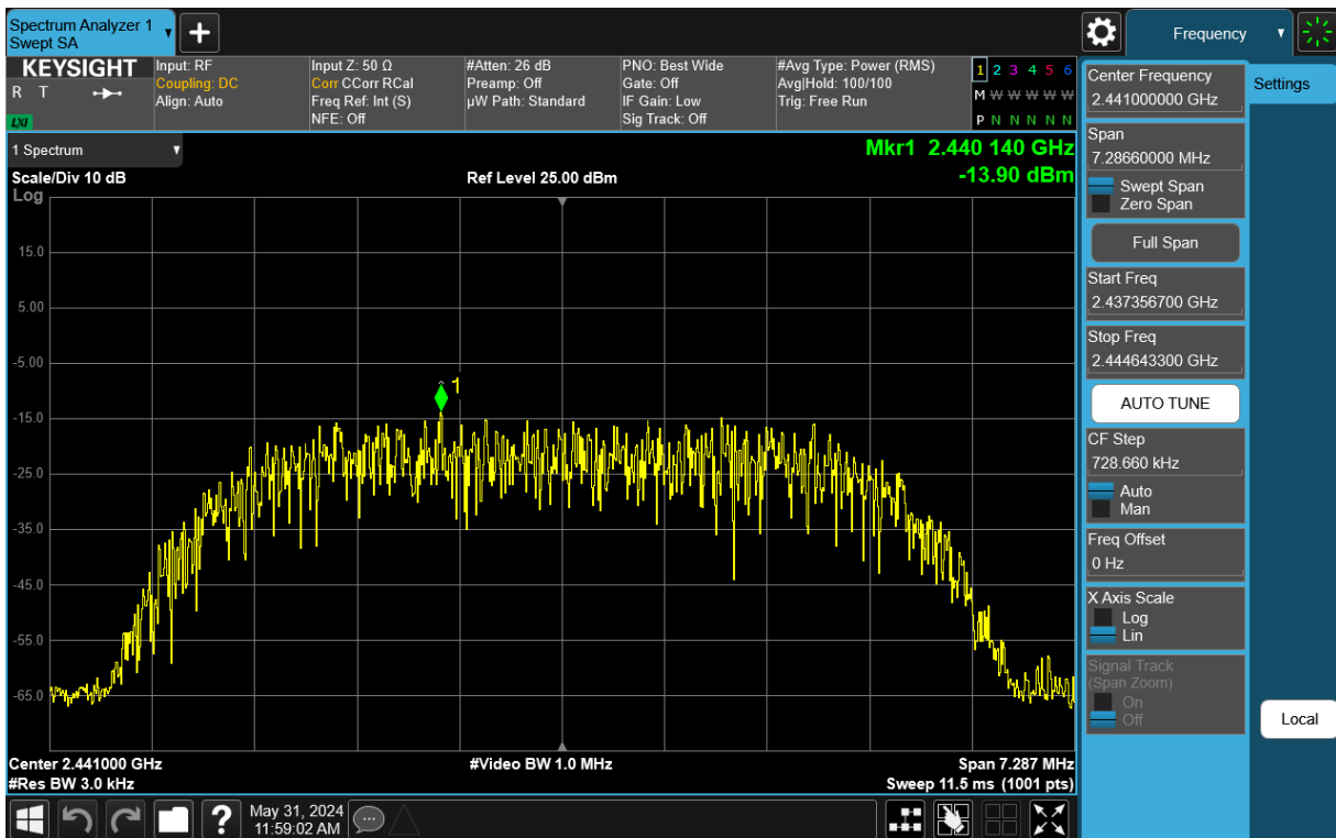
Plot 7-70. Power Spectral Density Plot TxBF Antenna 1a (Bluetooth (HDR8), 8Mbps, iPA – Ch. 38)
