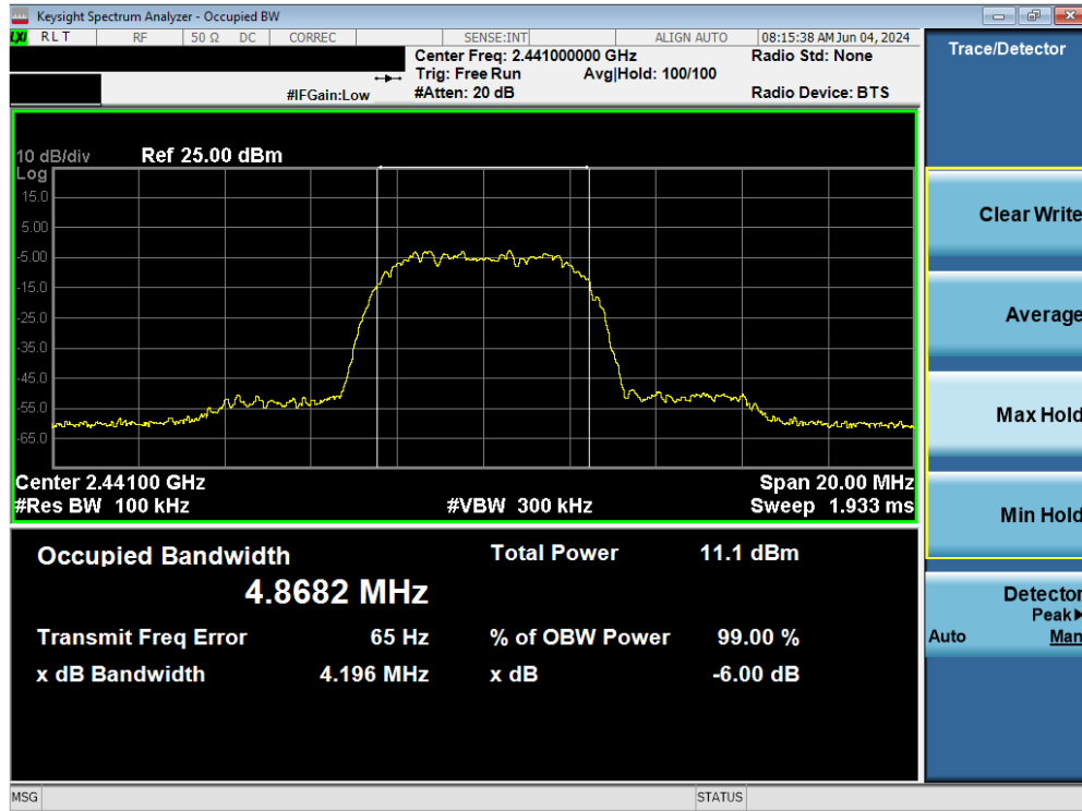
Plot 7-17. 6dB BW & 99% OBW Plot Antenna 4 (Bluetooth (HDR8), 8Mbps, iPA – Ch. 38)
