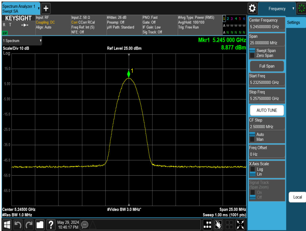
Plot 7-57. PSD Antenna 5T (NB UNII BDR, ePA– 5245MHz)
