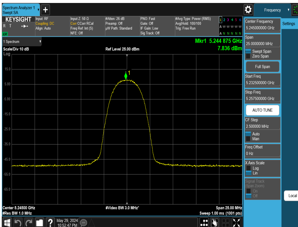
Plot 7-63. PSD Antenna 5T (NB UNII HDR4, ePA- 5245MHz)
