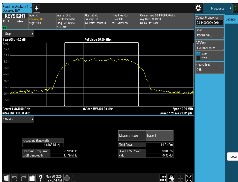
Plot 7-54. 6dB BW & 99% OBW Antenna 1b (NB UNII HDR8, ePA – 5844MHz)
