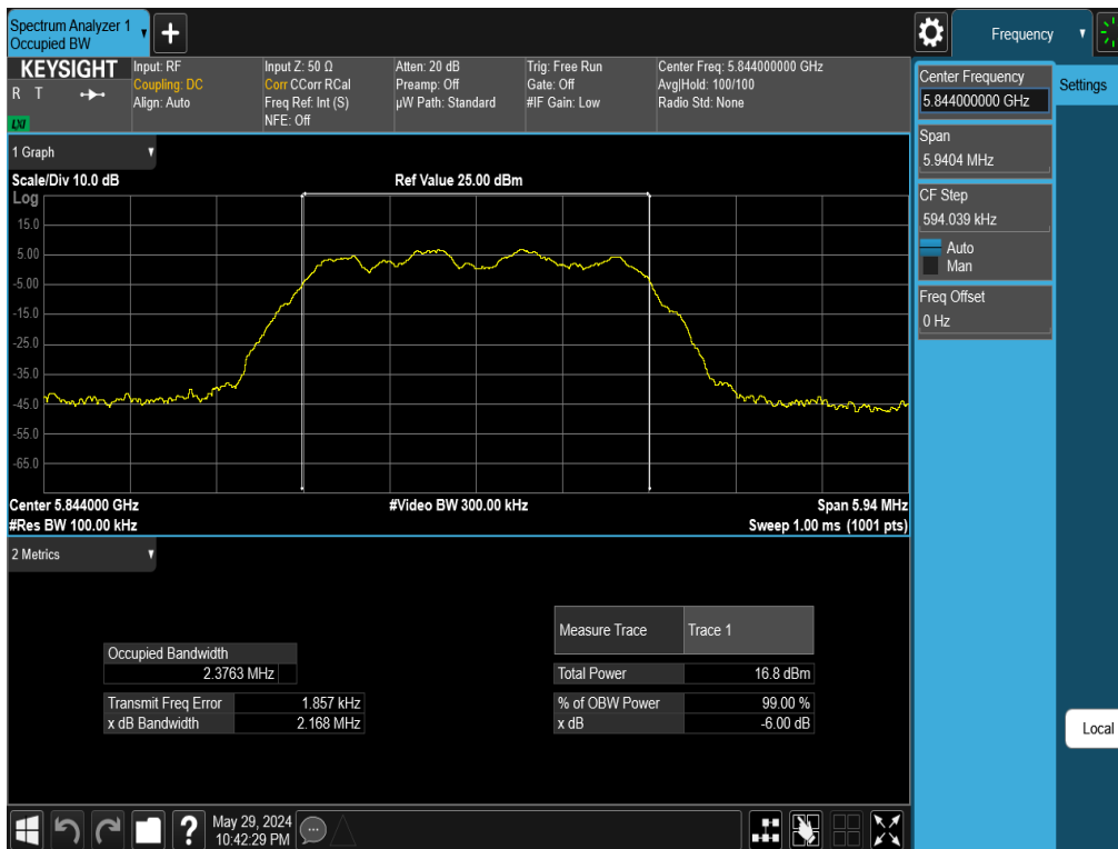
Plot 7-33. 6dB BW & 99% OBW Antenna 5T (NB UNII HDR4, ePA – 5844MHz)
