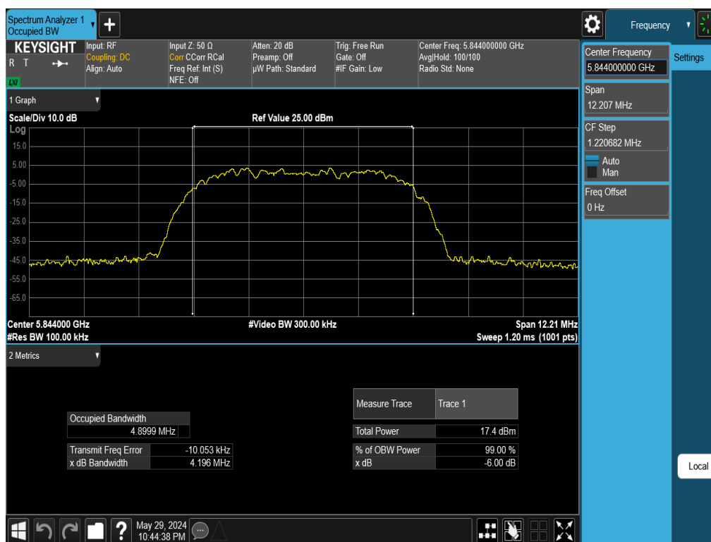
Plot 7-36. 6dB BW & 99% OBW Antenna 5T (NB UNII HDR8, ePA – 5844MHz)
