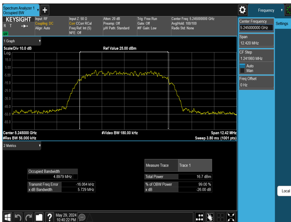
Plot 7-9. 26dB BW & 99% OBW Antenna 5T (NB UNII HDR8, ePA– 5245MHz)
