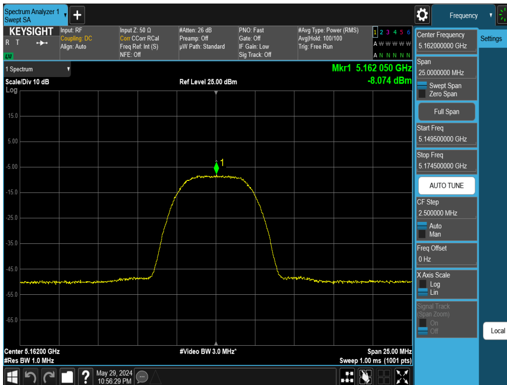
Plot 7-70. PSD Antenna 5T (NB UNII HDR8, iPA – 5162MHz)
