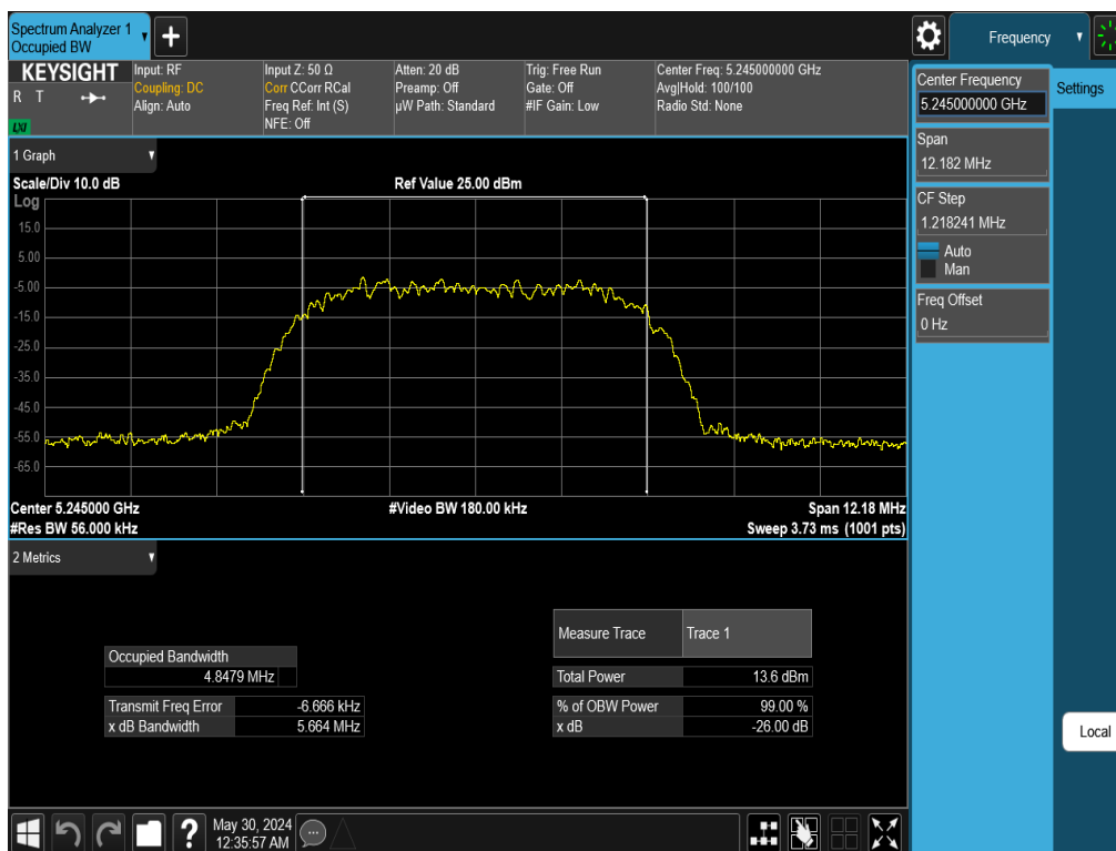
Plot 7-27. 26dB BW & 99% OBW Antenna 1b (NB UNII HDR8, ePA– 5245MHz)
