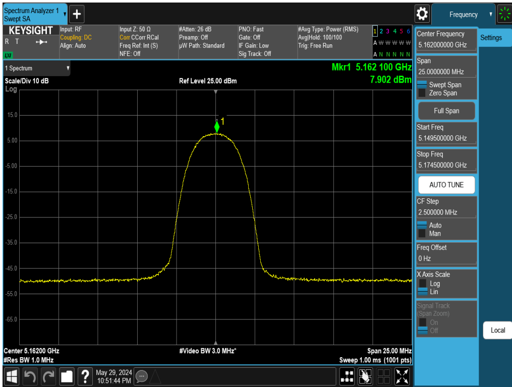
Plot 7-61. PSD Antenna 5T (NB UNII HDR4, ePA – 5162MHz)
