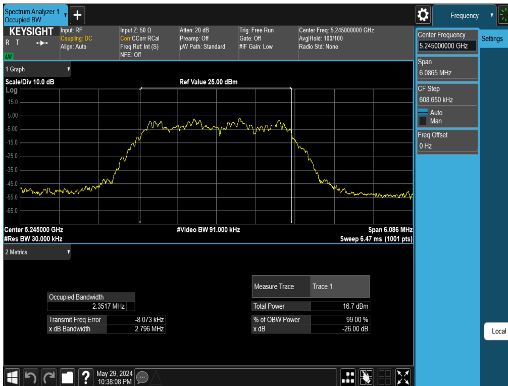
Plot 7-6. 26dB BW & 99% OBW Antenna 5T (NB UNII HDR4, ePA– 5245MHz)
