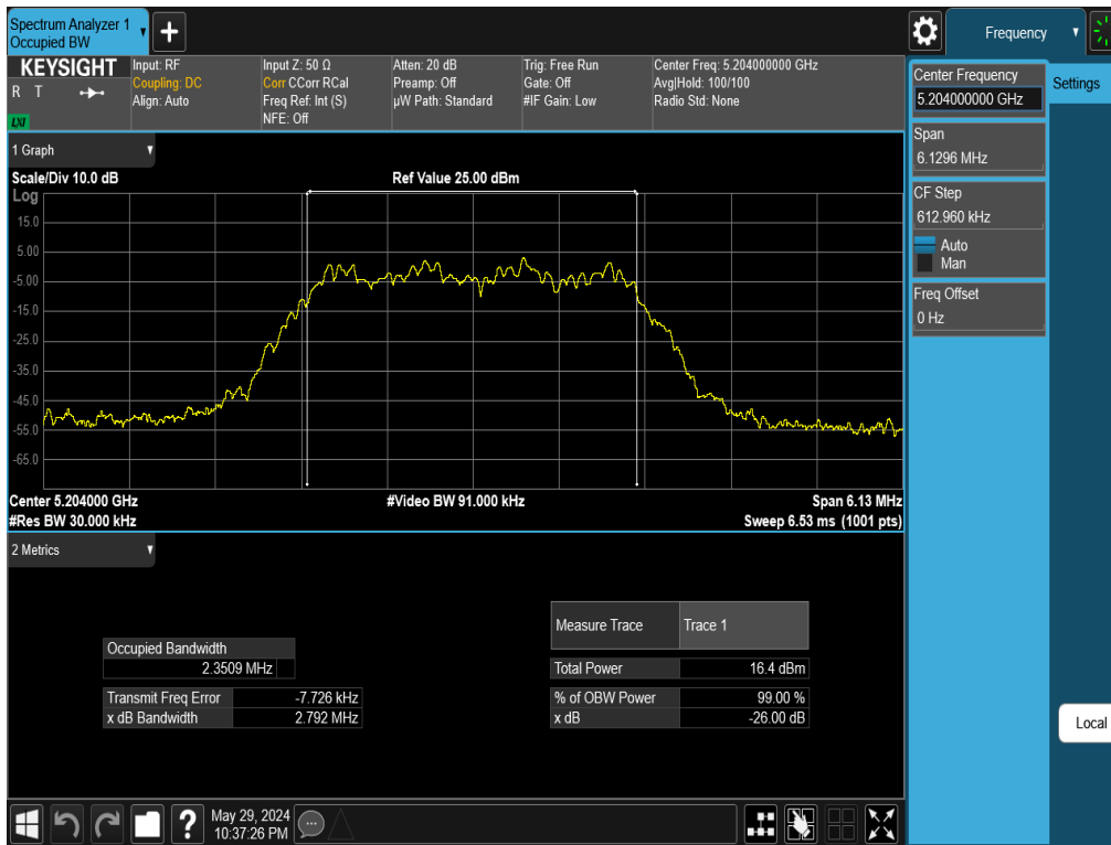
Plot 7-5. 26dB BW & 99% OBW Antenna 5T (NB UNII HDR4, ePA– 5204MHz)
