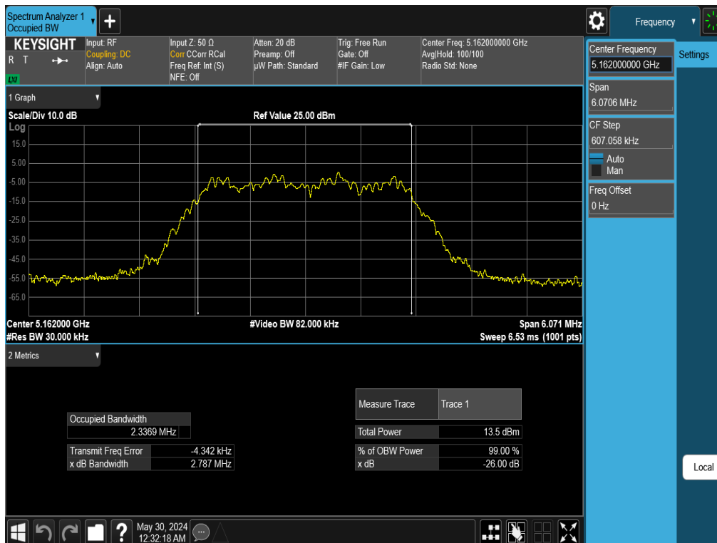
Plot 7-22. 26dB BW & 99% OBW Antenna 1b (NB UNII HDR4, ePA– 5162MHz)
