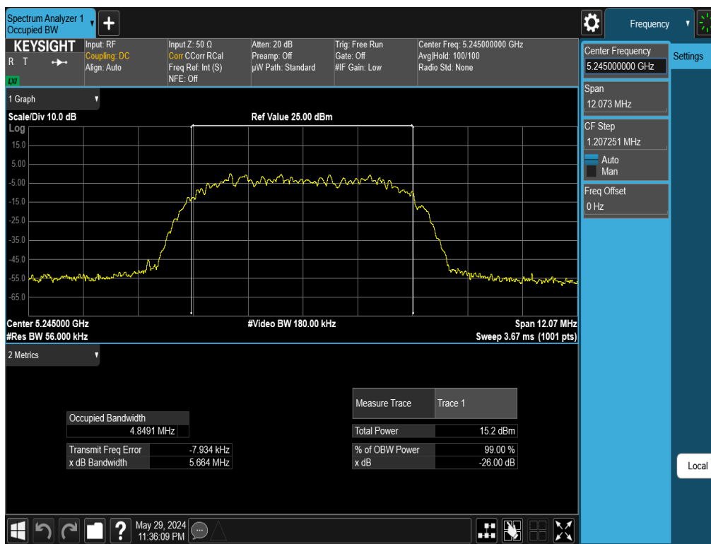
Plot 7-18. 26dB BW & 99% OBW Antenna 3b (NB UNII HDR8, ePA– 5245MHz)
