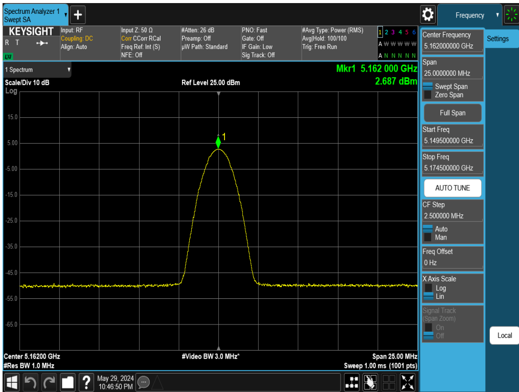
Plot 7-58. PSD Antenna 5T (NB UNII BDR, iPA – 5162MHz)
