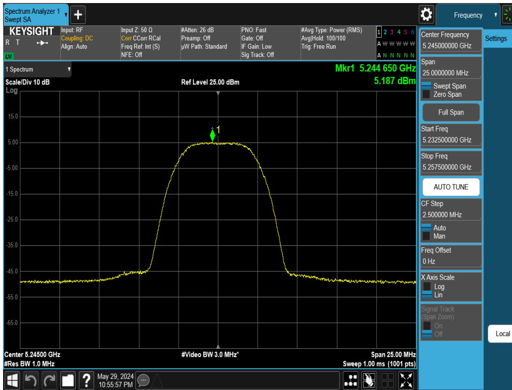
Plot 7-69. PSD Antenna 5T (NB UNII HDR8, ePA– 5245MHz)
