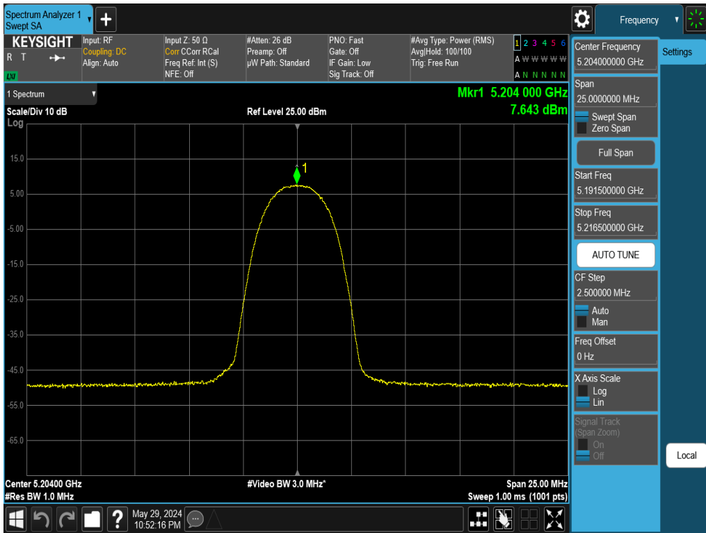
Plot 7-62. PSD Antenna 5T (NB UNII HDR4, ePA – 5204MHz)
