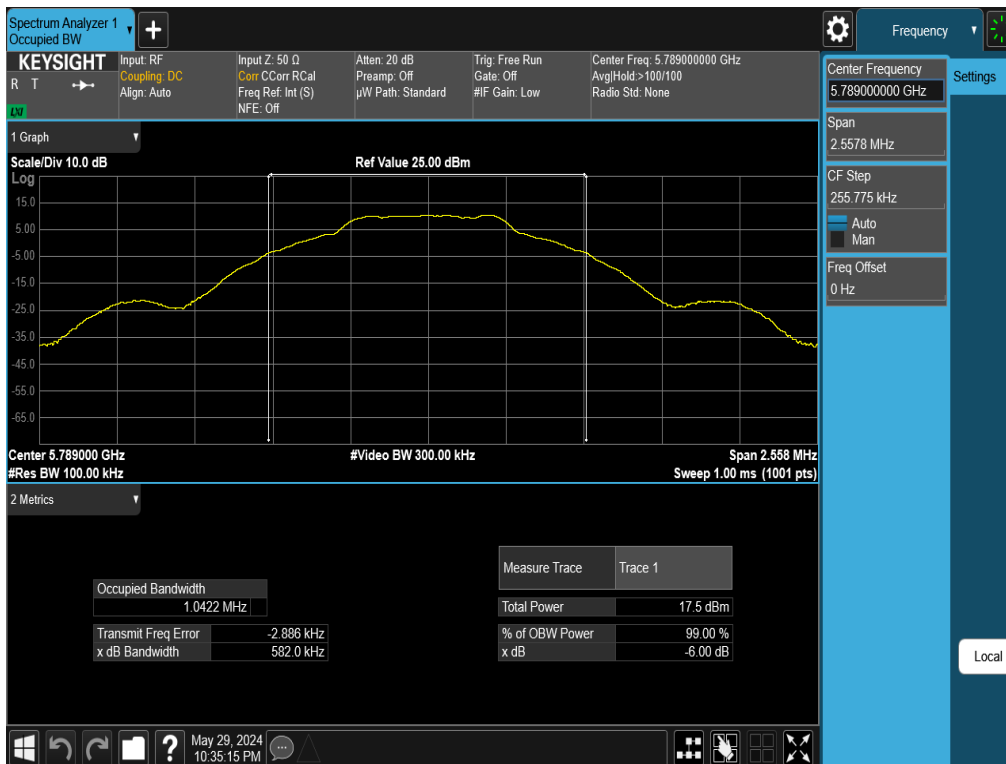
Plot 7-29. 6dB BW & 99% OBW Antenna 5T (NB UNII BDR, ePA – 5789MHz)
