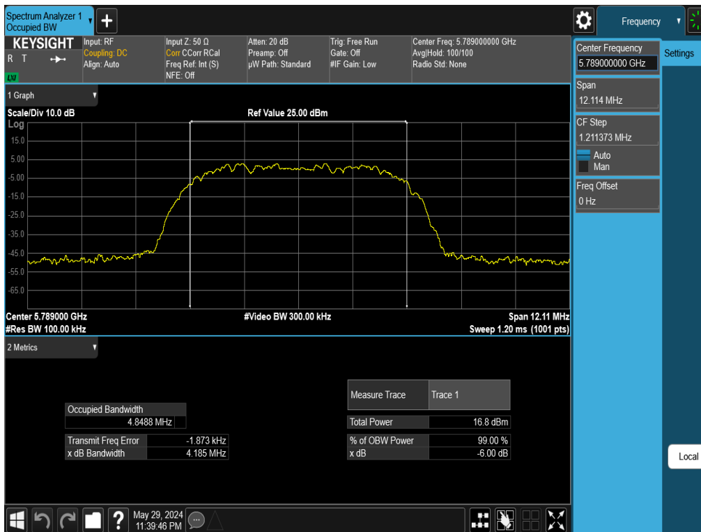
Plot 7-44. 6dB BW & 99% OBW Antenna 3b (NB UNII HDR8, ePA – 5789MHz)
