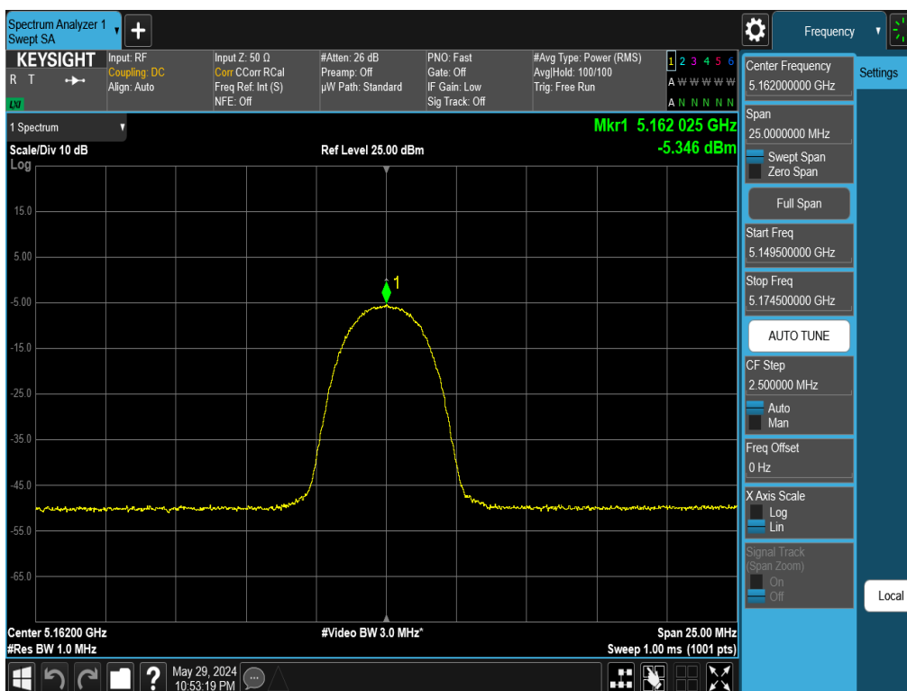
Plot 7-64. PSD Antenna 5T (NB UNII HDR4, iPA - 5162MHz)
