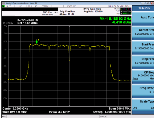
Plot 7-678. PSD CDD Primary Antenna 3b (160MHz BW 802.11ac - Ch. 50, MCS9)
