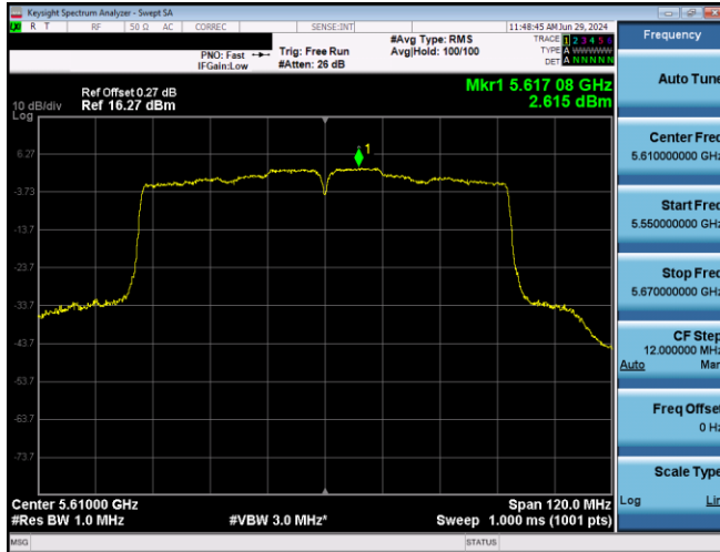
Plot 7-657. PSD CDD Primary Antenna 5T (80MHz BW 802.11ac - Ch. 122, MCS4)
