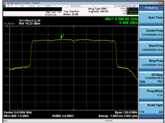
Plot 7-660. PSD CDD Primary Antenna 3b (80MHz BW 802.11ax(SU) - Ch. 122, MCS4)
