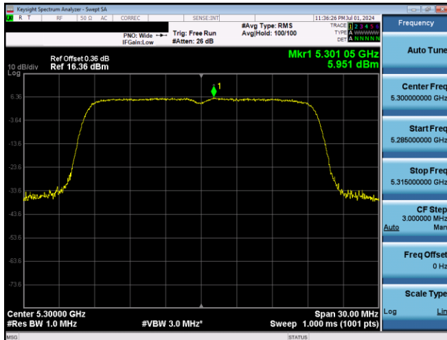
Plot 7-684. PSD SDM Primary Antenna 3b (20MHz BW 802.11ax(SU) – Ch. 60, MCS11)
