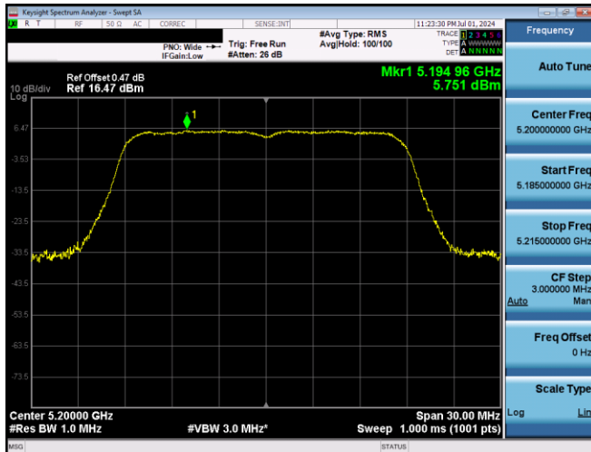
Plot 7-666. PSD SDM Primary Antenna 3b (20MHz BW 802.11n - Ch. 40, MCS15)
