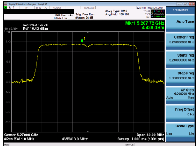
Plot 7-687. PSD CDD Primary Antenna 5T (40MHz BW 802.11ax(SU) – Ch. 54, MCS11)
