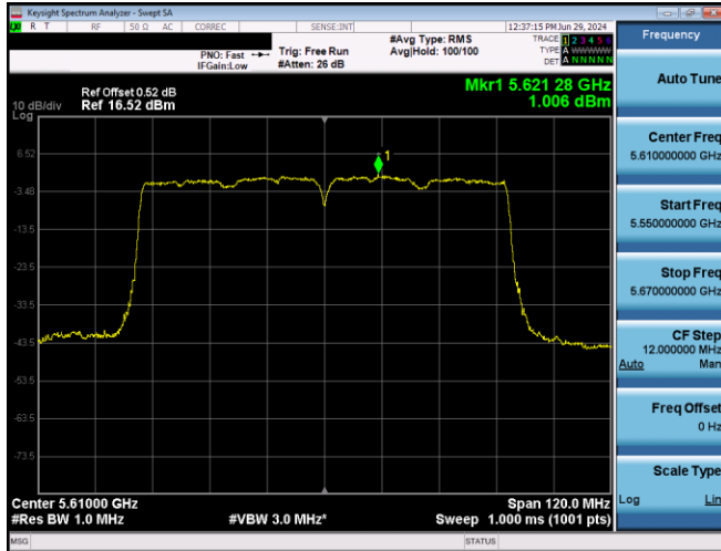
Plot 7-701. PSD CDD Primary Antenna 5T (80MHz BW 802.11ac - Ch. 122, MCS9)
