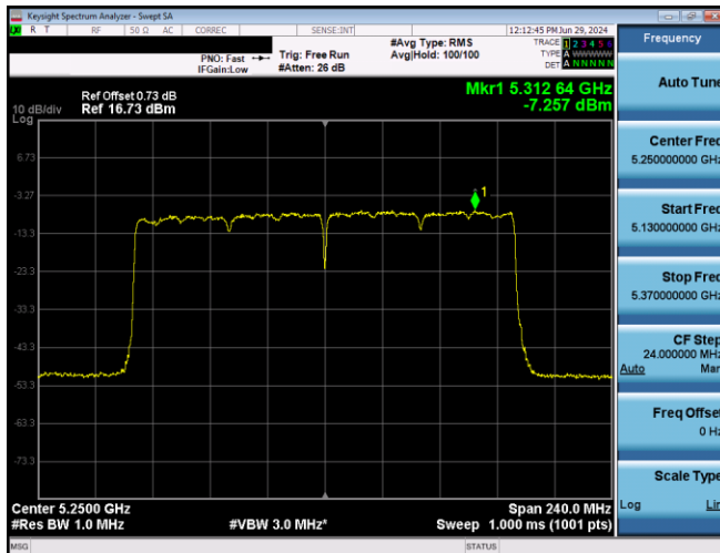
Plot 7-679. PSD CDD Primary Antenna 5T (160MHz BW 802.11ax(SU) - Ch. 50, MCS11)
