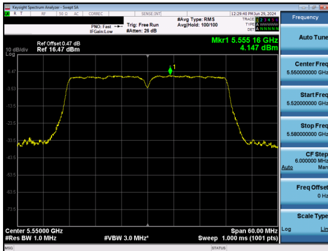
Plot 7-697. PSD CDD Primary Antenna 5T (40MHz BW 802.11n – Ch. 110, MCS15)
