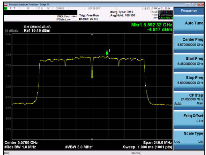
Plot 7-662. PSD CDD Primary Antenna 3b (160MHz BW 802.11ac - Ch. 114, MCS4)
