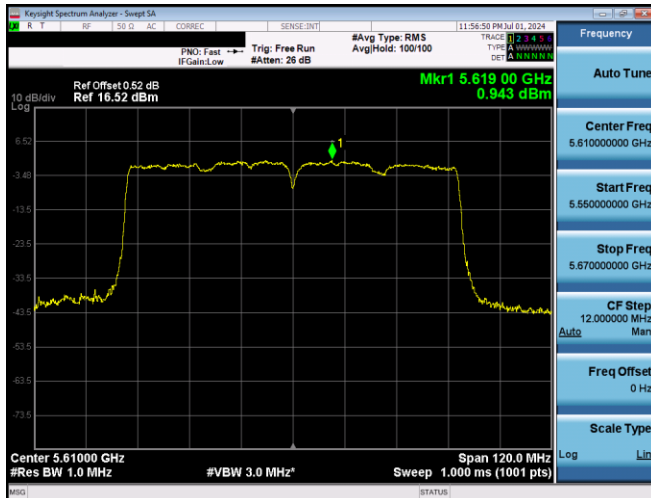
Plot 7-702. PSD CDD Primary Antenna 3b (80MHz BW 802.11ac - Ch. 122, MCS9)
