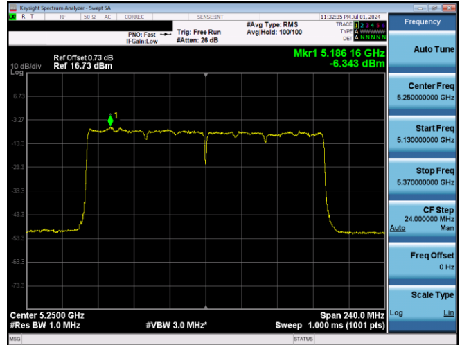
Plot 7-680. PSD CDD Primary Antenna 3b (160MHz BW 802.11ax(SU) - Ch. 50, MCS11)
