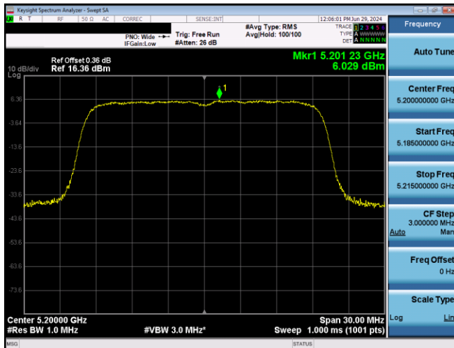
Plot 7-667. PSD SDM Primary Antenna 5T (20MHz BW 802.11ax(SU) - Ch. 40, MCS11)
