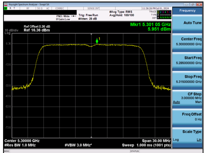
Plot 7-682. PSD SDM Primary Antenna 3b (20MHz BW 802.11n - Ch. 60, MCS15)
