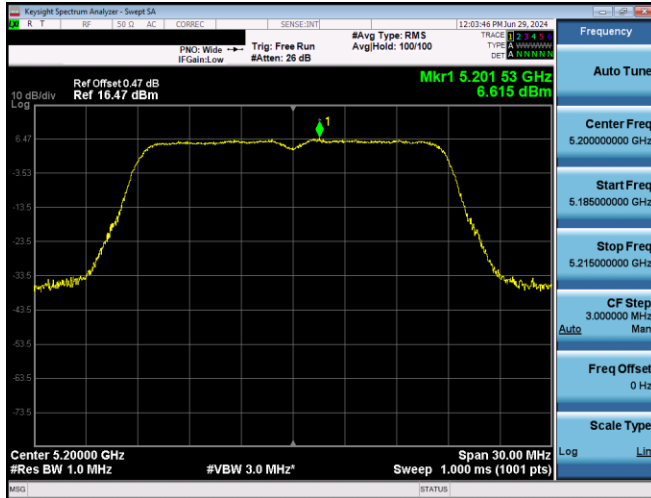
Plot 7-665. PSD SDM Primary Antenna 5T (20MHz BW 802.11n - Ch. 40, MCS15)
