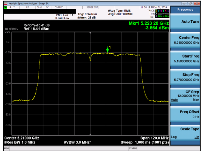
Plot 7-674. PSD CDD Primary Antenna 3b (80MHz BW 802.11ac – Ch. 42, MCS9)
