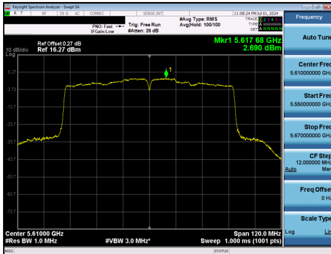
Plot 7-658. PSD CDD Primary Antenna 3b (80MHz BW 802.11ac - Ch. 122, MCS4)
