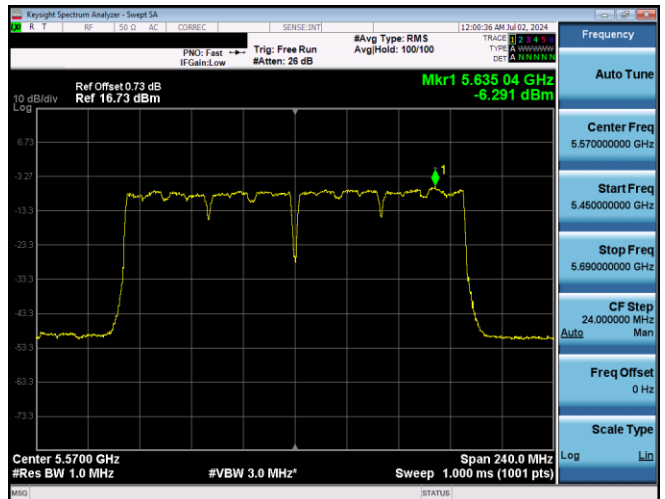
Plot 7-706. PSD CDD Primary Antenna 3b (160MHz BW 802.11ac - Ch. 114, MCS9)
