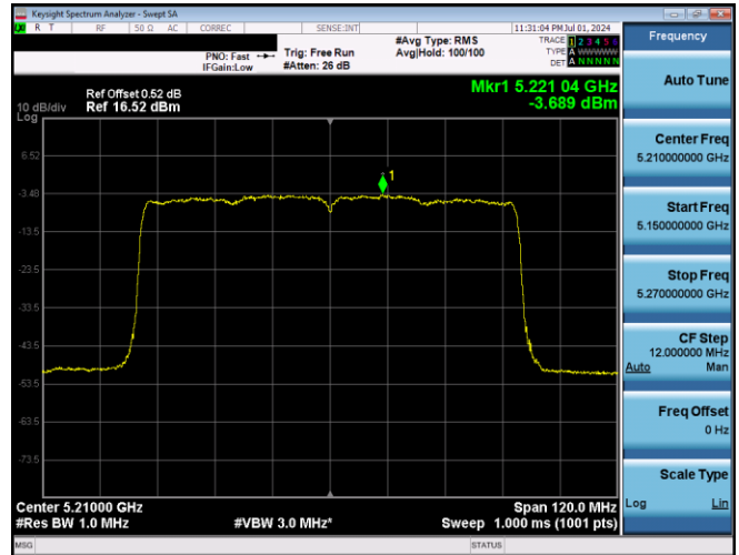
Plot 7-676. PSD CDD Primary Antenna 3b (80MHz BW 802.11ax(SU) – Ch. 42, MCS11)
