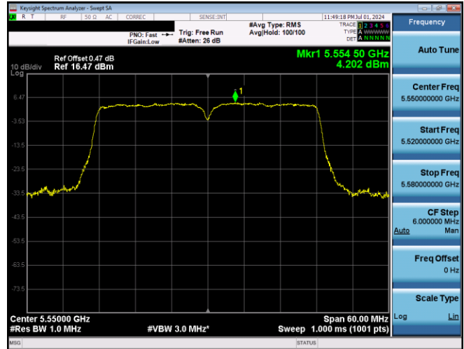
Plot 7-698. PSD CDD Primary Antenna 3b (40MHz BW 802.11n – Ch. 110, MCS15)
