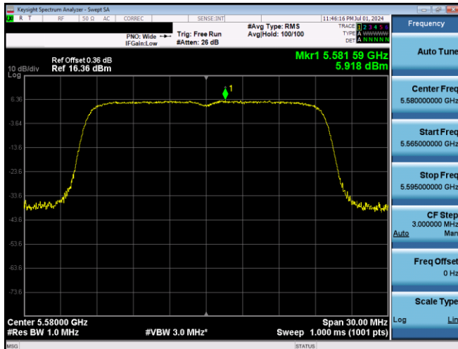
Plot 7-696. PSD SDM Primary Antenna 3b (20MHz BW 802.11ax(SU) – Ch. 116, MCS11)
