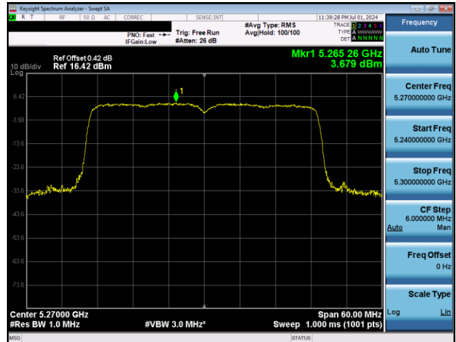
Plot 7-688. PSD CDD Primary Antenna 3b (40MHz BW 802.11ax(SU) – Ch. 54, MCS11)
