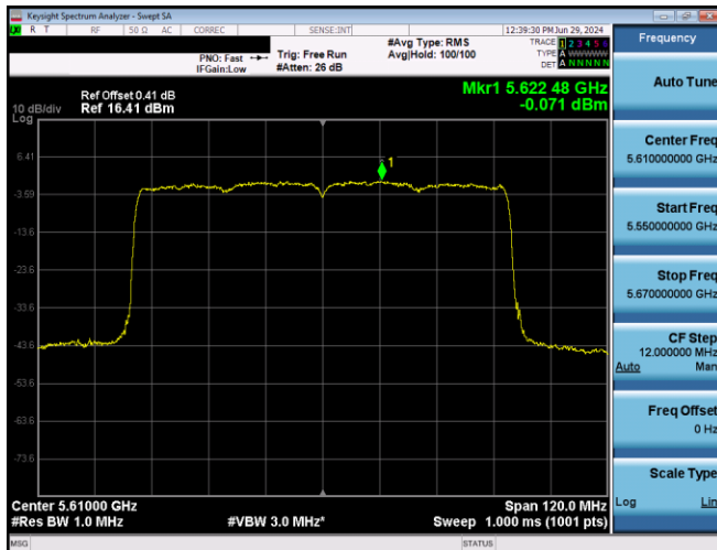
Plot 7-703. PSD CDD Primary Antenna 5T (80MHz BW 802.11ax(SU) - Ch. 122, MCS11)
