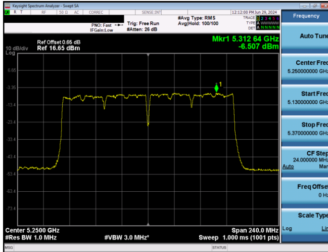
Plot 7-677. PSD CDD Primary Antenna 5T (160MHz BW 802.11ac - Ch. 50, MCS9)
