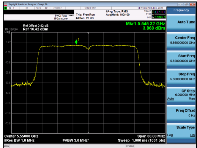
Plot 7-700. PSD CDD Primary Antenna 3b (40MHz BW 802.11ax(SU) – Ch. 110, MCS11)
