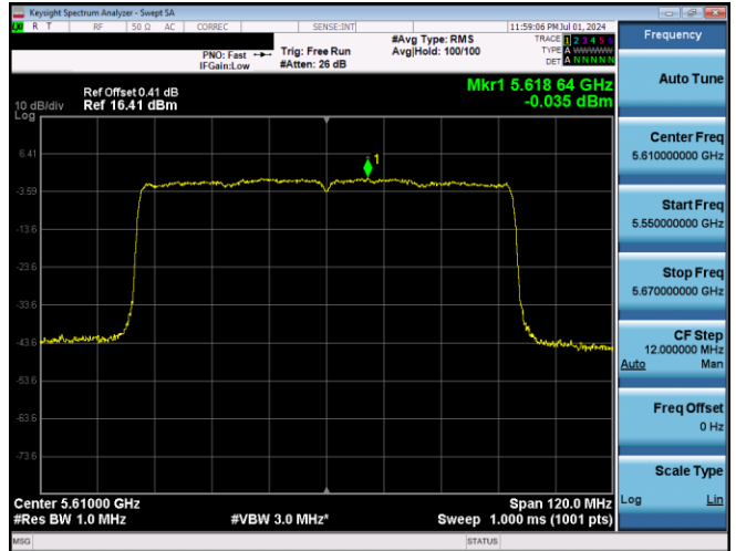
Plot 7-704. PSD CDD Primary Antenna 3b (80MHz BW 802.11ax(SU) - Ch. 122, MCS11)
