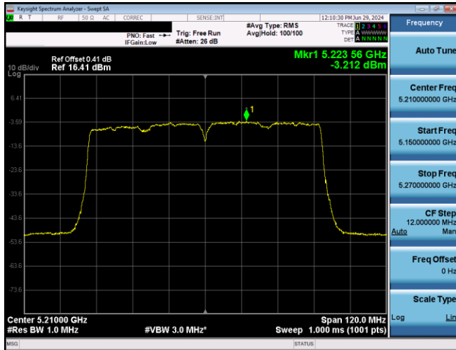
Plot 7-673. PSD CDD Primary Antenna 5T (80MHz BW 802.11ac – Ch. 42, MCS9)
