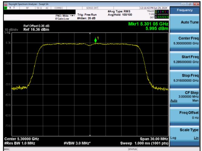
Plot 7-681. PSD SDM Primary Antenna 5T (20MHz BW 802.11n - Ch. 60, MCS15)
