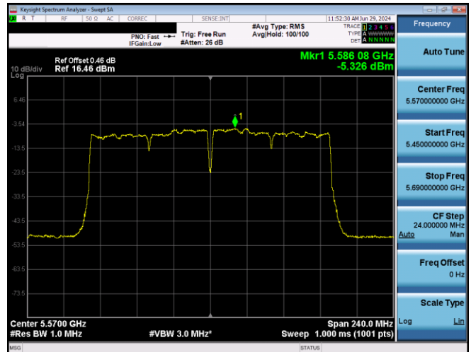
Plot 7-661. PSD CDD Primary Antenna 5T (160MHz BW 802.11ac - Ch. 114, MCS4)
