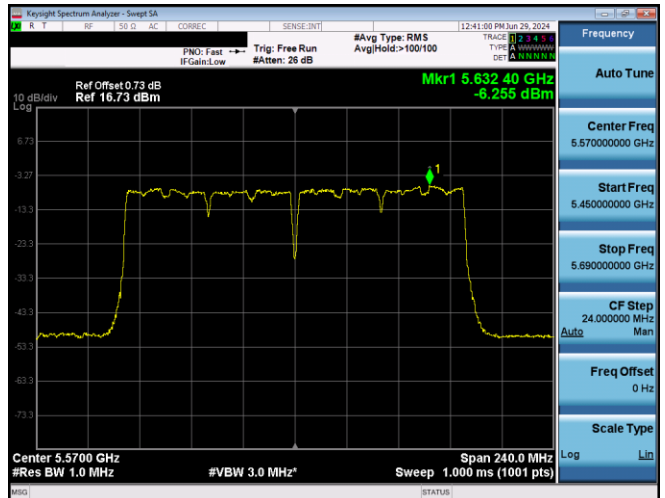
Plot 7-705. PSD CDD Primary Antenna 5T (160MHz BW 802.11ac - Ch. 114, MCS9)
