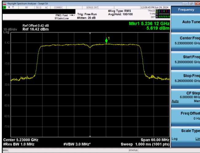
Plot 7-671. PSD SDM Primary Antenna 5T (40MHz BW 802.11ax(SU) – Ch. 46, MCS11)
