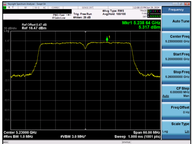
Plot 7-669. PSD SDM Primary Antenna 5T (40MHz BW 802.11n - Ch. 46, MCS15)
