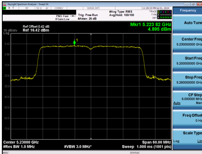
Plot 7-672. PSD SDM Primary Antenna 3b (40MHz BW 802.11ax(SU) – Ch. 46, MCS11)
