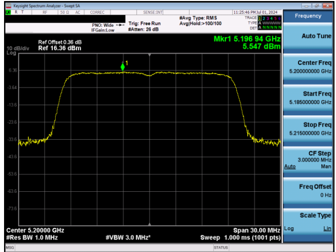
Plot 7-668. PSD SDM Primary Antenna 3b (20MHz BW 802.11ax(SU) - Ch. 40, MCS11)
