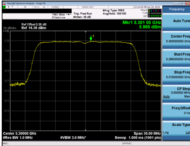
Plot 7-683. PSD SDM Primary Antenna 5T (20MHz BW 802.11ax(SU) – Ch. 60, MCS11)
