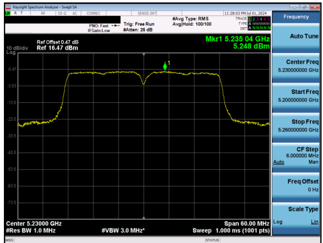
Plot 7-670. PSD SDM Primary Antenna 3b (40MHz BW 802.11n - Ch. 46, MCS15)
