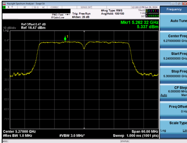
Plot 7-685. PSD CDD Primary Antenna 5T (40MHz BW 802.11n – Ch. 54, MCS15)
