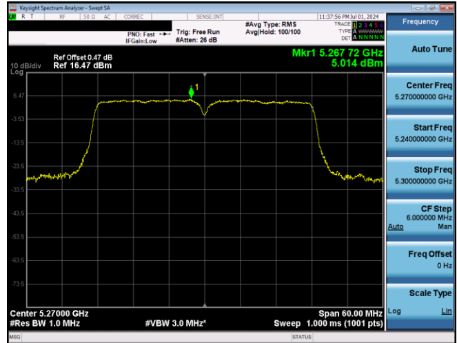
Plot 7-686. PSD CDD Primary Antenna 3b (40MHz BW 802.11n – Ch. 54, MCS15)
