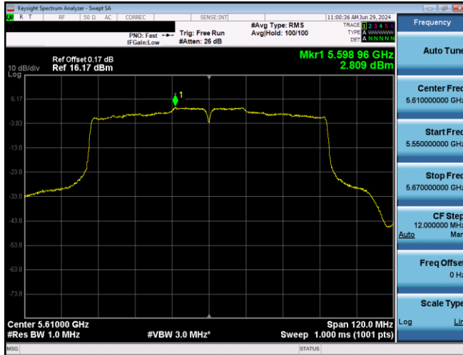
Plot 7-613. PSD CDD Primary Antenna 5T (80MHz BW 802.11ac - Ch. 122, MCS2)
