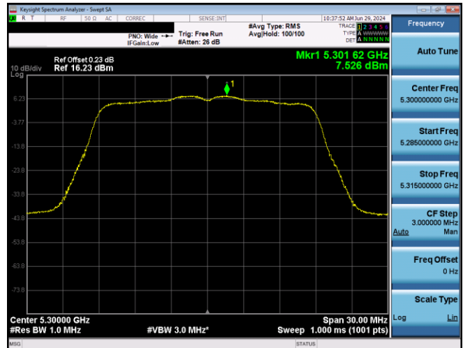
Plot 7-593. PSD SDM Primary Antenna 5T (20MHz BW 802.11n - Ch. 60, MCS10)
