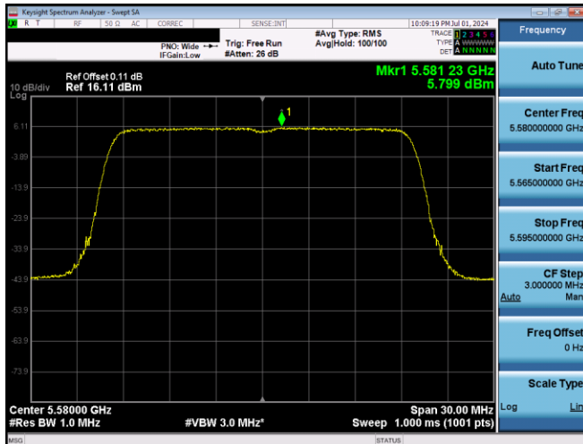
Plot 7-608. PSD SDM Primary Antenna 3b (20MHz BW 802.11ax(SU) – Ch. 116, MCS2)
