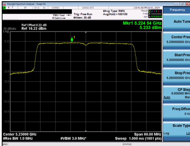
Plot 7-628. PSD SDM Primary Antenna 3b (40MHz BW 802.11ax(SU) – Ch. 46, MCS4)
