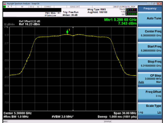
Plot 7-594. PSD SDM Primary Antenna 3b (20MHz BW 802.11n - Ch. 60, MCS10)
