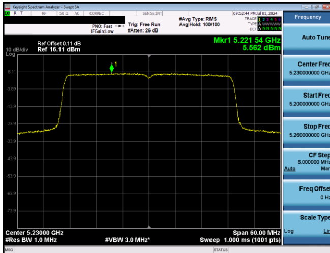
Plot 7-584. PSD SDM Primary Antenna 3b (40MHz BW 802.11ax(SU) - Ch. 46, MCS2)
