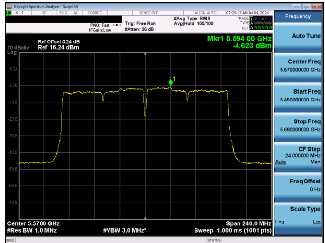
Plot 7-617. PSD CDD Primary Antenna 5T (160MHz BW 802.11ac - Ch. 114, MCS2)
