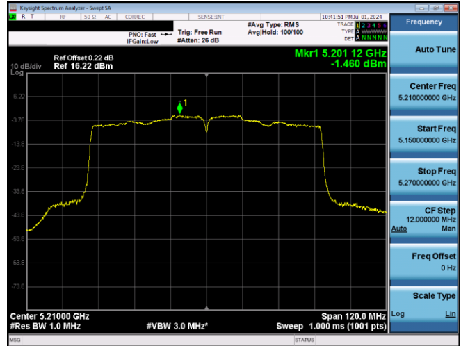
Plot 7-630. PSD CDD Primary Antenna 3b (80MHz BW 802.11ac – Ch. 42, MCS4)
