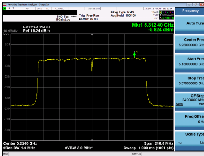
Plot 7-591. PSD CDD Primary Antenna 5T (160MHz BW 802.11ax(SU) - Ch. 50, MCS2)
