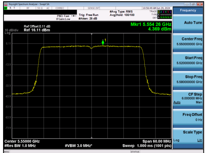
Plot 7-611. PSD CDD Primary Antenna 5T (40MHz BW 802.11ax(SU) – Ch. 110, MCS2)
