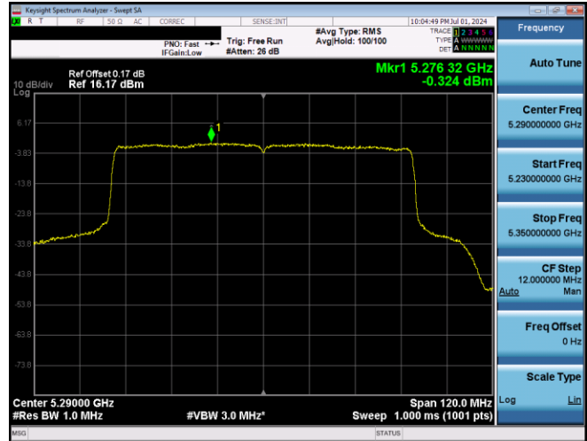
Plot 7-604. PSD CDD Primary Antenna 3b (80MHz BW 802.11ax(SU) – Ch. 58, MCS2)
