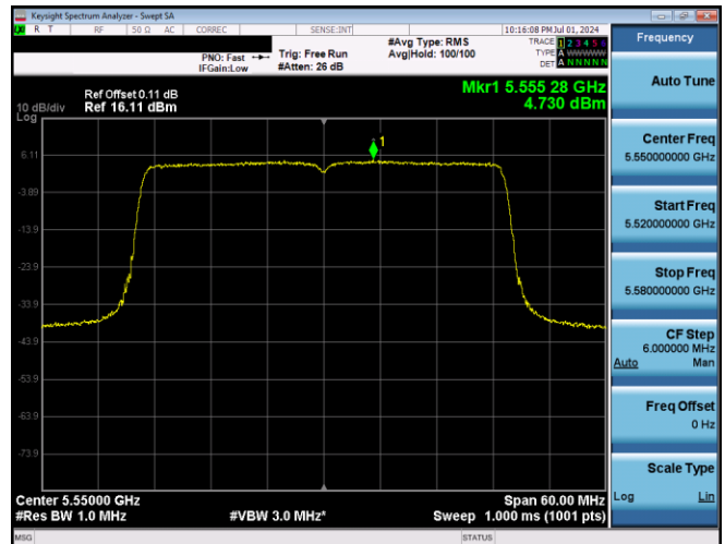
Plot 7-612. PSD CDD Primary Antenna 3b (40MHz BW 802.11ax(SU) – Ch. 110, MCS2)
