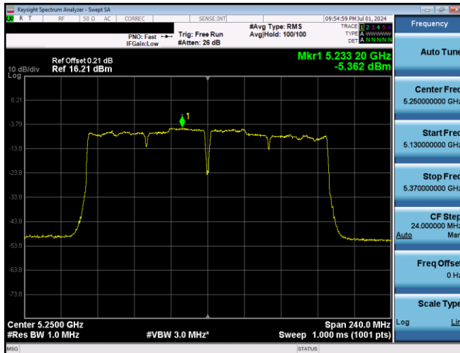
Plot 7-590. PSD CDD Primary Antenna 3b (160MHz BW 802.11ac - Ch. 50, MCS2)
