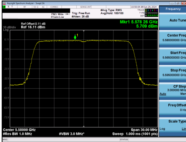
Plot 7-607. PSD SDM Primary Antenna 5T (20MHz BW 802.11ax(SU) – Ch. 116, MCS2)
