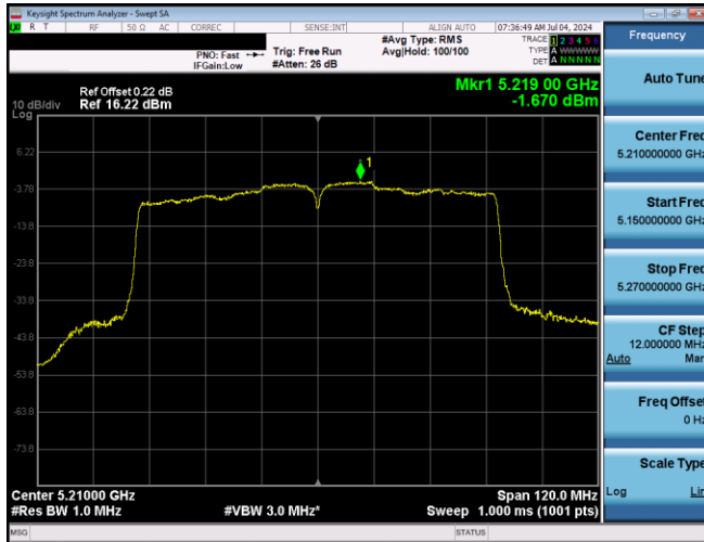
Plot 7-629. PSD CDD Primary Antenna 5T (80MHz BW 802.11ac – Ch. 42, MCS4)
