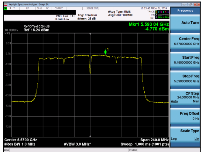
Plot 7-618. PSD CDD Primary Antenna 3b (160MHz BW 802.11ac - Ch. 114, MCS2)
