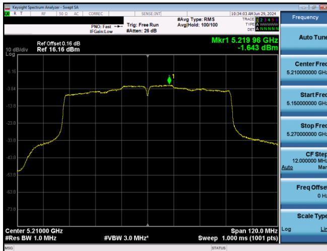
Plot 7-585. PSD CDD Primary Antenna 5T (80MHz BW 802.11ac - Ch. 42, MCS2)
