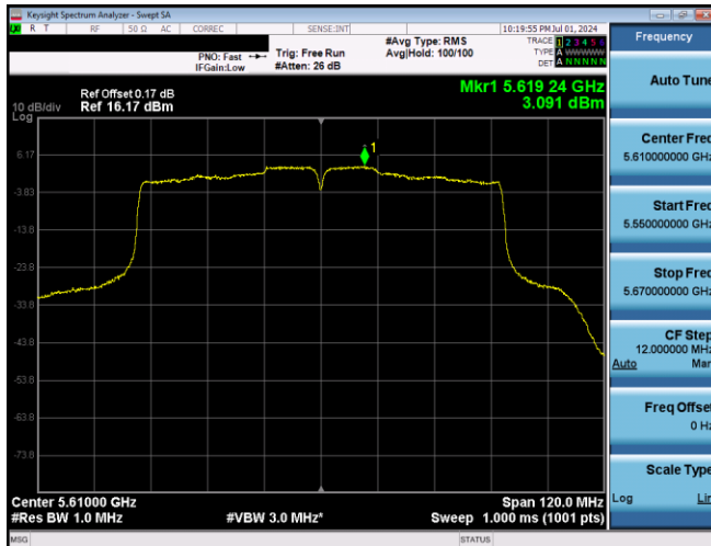
Plot 7-614. PSD CDD Primary Antenna 3b (80MHz BW 802.11ac - Ch. 122, MCS2)
