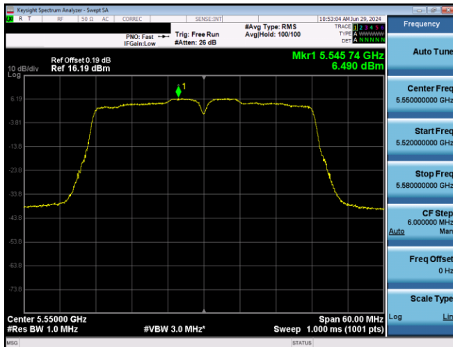
Plot 7-609. PSD SDM Primary Antenna 5T (40MHz BW 802.11n – Ch. 110, MCS10)
