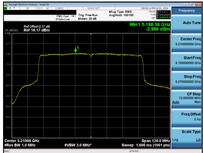
Plot 7-588. PSD CDD Primary Antenna 3b (80MHz BW 802.11ax(SU) - Ch. 42, MCS2)
