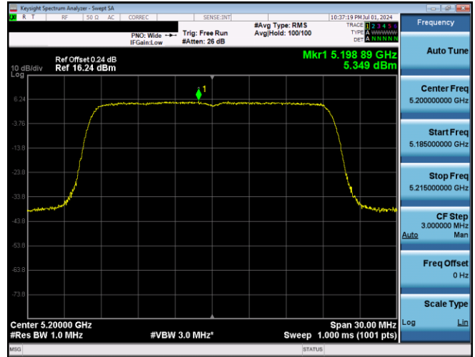
Plot 7-624. PSD SDM Primary Antenna 3b (20MHz BW 802.11ax(SU) - Ch. 40, MCS4)
