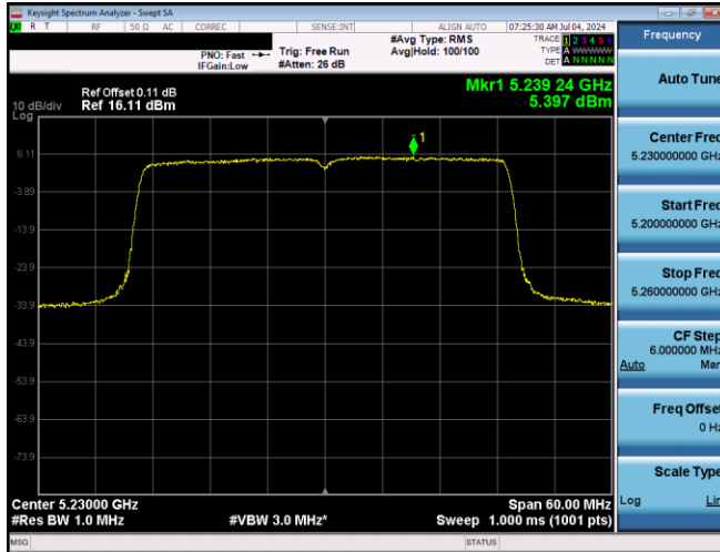
Plot 7-583. PSD SDM Primary Antenna 5T (40MHz BW 802.11ax(SU) - Ch. 46, MCS2)
