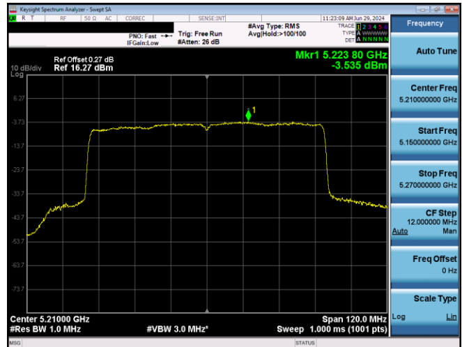
Plot 7-631. PSD CDD Primary Antenna 5T (80MHz BW 802.11ax(SU) – Ch. 42, MCS4)
