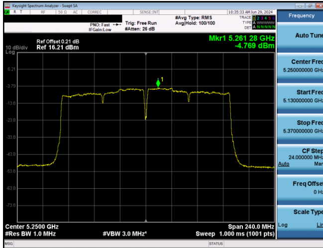
Plot 7-589. PSD CDD Primary Antenna 5T (160MHz BW 802.11ac - Ch. 50, MCS2)
