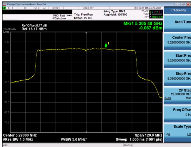
Plot 7-603. PSD CDD Primary Antenna 5T (80MHz BW 802.11ax(SU) – Ch. 58, MCS2)
