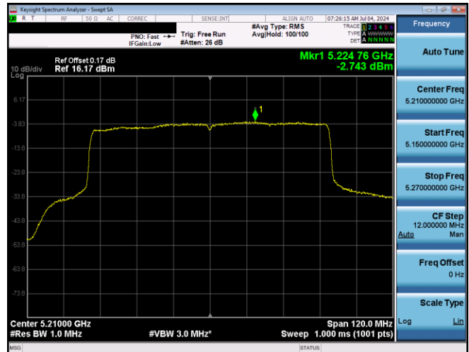
Plot 7-587. PSD CDD Primary Antenna 5T (80MHz BW 802.11ax(SU) - Ch. 42, MCS2)
