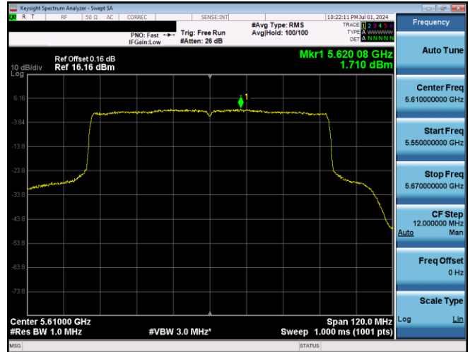
Plot 7-616. PSD CDD Primary Antenna 3b (80MHz BW 802.11ax(SU) - Ch. 122, MCS2)
