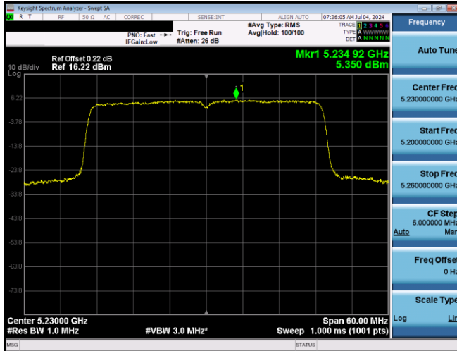
Plot 7-627. PSD SDM Primary Antenna 5T (40MHz BW 802.11ax(SU) – Ch. 46, MCS4)
