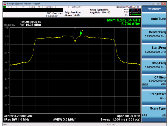
Plot 7-626. PSD SDM Primary Antenna 3b (40MHz BW 802.11n - Ch. 46, MCS12)
