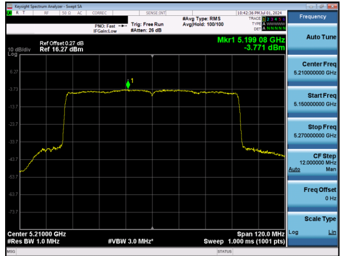
Plot 7-632. PSD CDD Primary Antenna 3b (80MHz BW 802.11ax(SU) – Ch. 42, MCS4)
