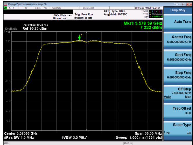
Plot 7-606. PSD SDM Primary Antenna 3b (20MHz BW 802.11n – Ch. 116, MCS10)
