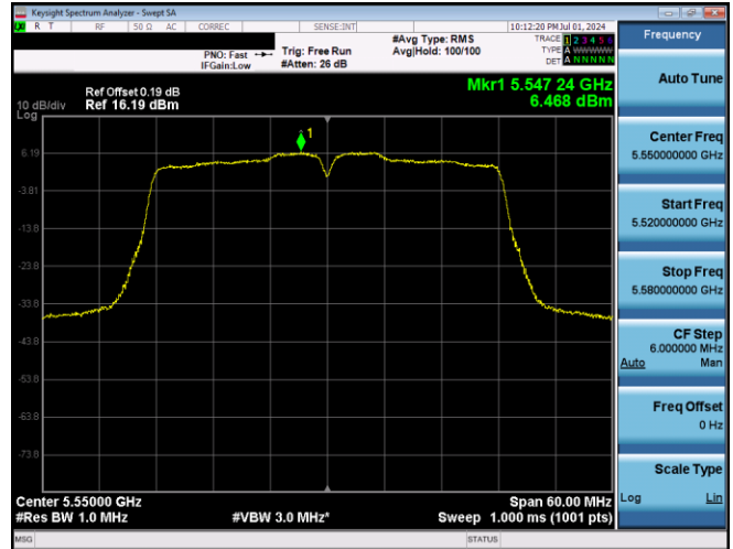
Plot 7-610. PSD SDM Primary Antenna 3b (40MHz BW 802.11n – Ch. 110, MCS10)
