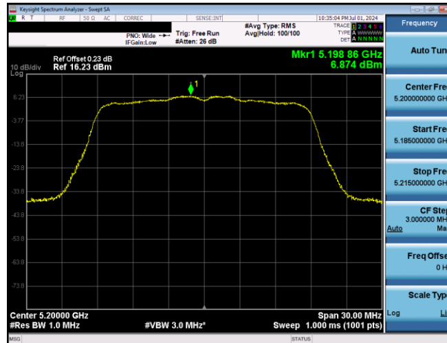
Plot 7-622. PSD SDM Primary Antenna 3b (20MHz BW 802.11n - Ch. 40, MCS12)
