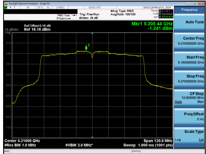
Plot 7-586. PSD CDD Primary Antenna 3b (80MHz BW 802.11ac - Ch. 42, MCS2)
