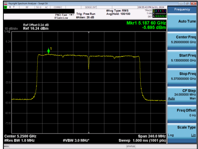
Plot 7-592. PSD CDD Primary Antenna 3b (160MHz BW 802.11ax(SU) - Ch. 50, MCS2)
