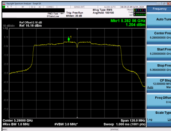
Plot 7-602. PSD CDD Primary Antenna 3b (80MHz BW 802.11ac – Ch. 58, MCS2)
