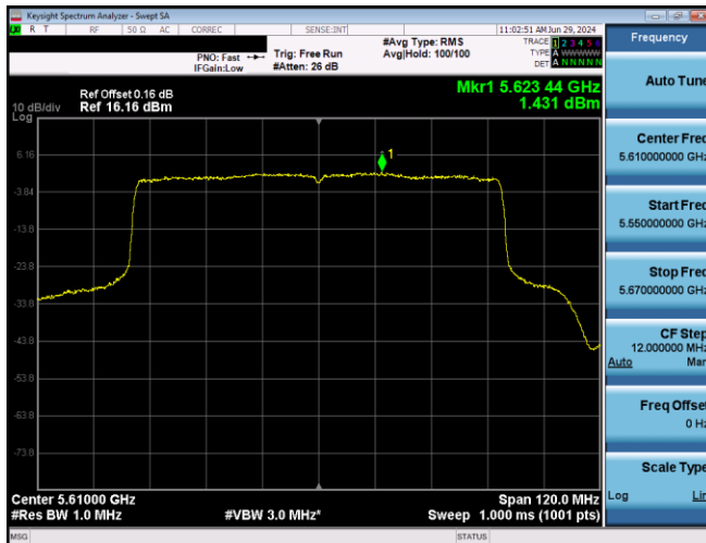
Plot 7-615. PSD CDD Primary Antenna 5T (80MHz BW 802.11ax(SU) - Ch. 122, MCS2)
