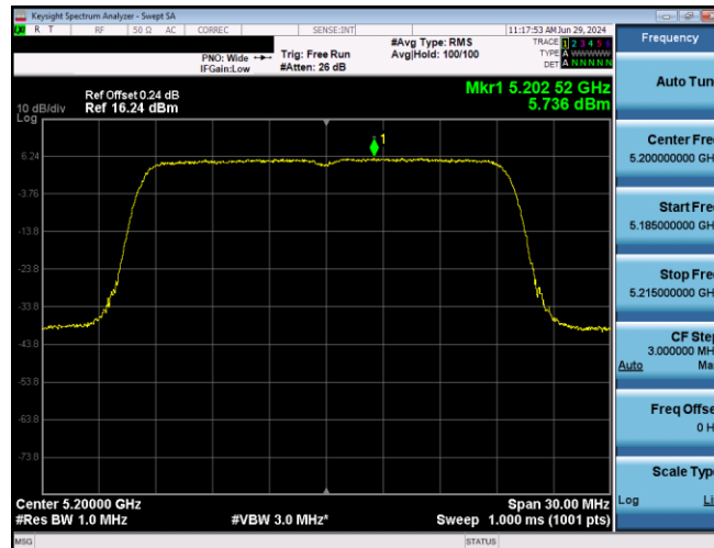
Plot 7-623. PSD SDM Primary Antenna 5T (20MHz BW 802.11ax(SU) - Ch. 40, MCS4)
