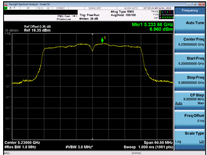
Plot 7-625. PSD SDM Primary Antenna 5T (40MHz BW 802.11n - Ch. 46, MCS12)
