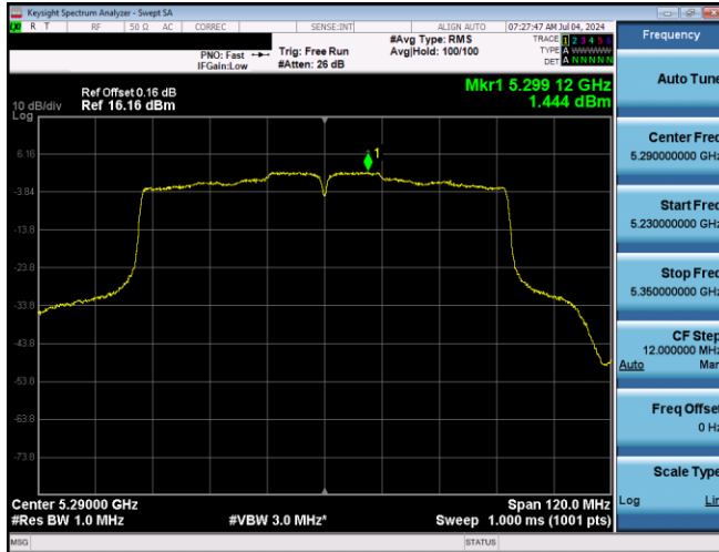
Plot 7-601. PSD CDD Primary Antenna 5T (80MHz BW 802.11ac – Ch. 58, MCS2)
