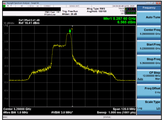
Plot 7-575. PSD SDM Diversity Antenna 1b (80MHz BW 11ax Index 44 - RU52 - Ch.58)
