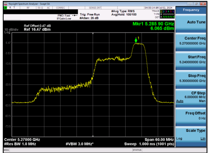
Plot 7-569. PSD SDM Diversity Antenna 1b (40MHz BW 11ax Index 44 - RU52 - Ch.54)
