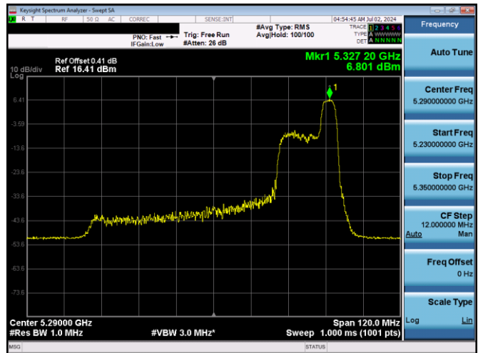
Plot 7-577. PSD SDM Diversity Antenna 1b (80MHz BW 11ax Index 52 - RU52 - Ch.58)
