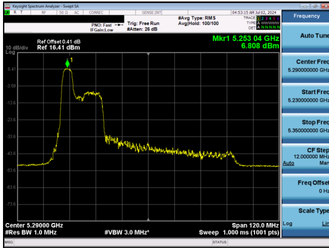
Plot 7-573. PSD SDM Diversity Antenna 1b (80MHz BW 11ax Index 37 - RU52 - Ch.58)
