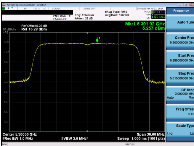
Plot 7-563. PSD SDM Diversity Antenna 1b (20MHz BW 11ax- RU242 - Ch.60)
