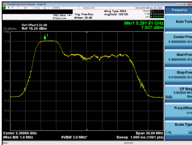
Plot 7-556. PSD SDM Diversity Antenna 5T (20MHz BW 11ax Index 37 - RU52 - Ch.60)
