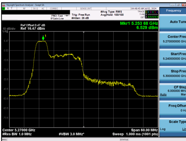
Plot 7-565. PSD SDM Diversity Antenna 1b (40MHz BW 11ax Index 37 - RU52 - Ch.54)
