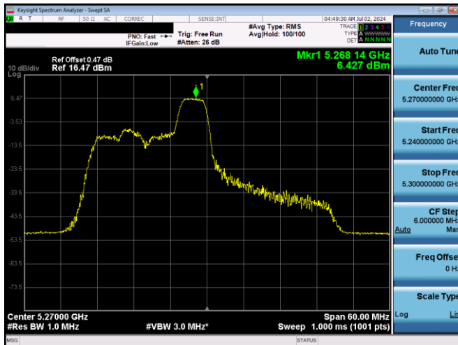
Plot 7-567. PSD SDM Diversity Antenna 1b (40MHz BW 11ax Index 40 - RU52 - Ch.54)
