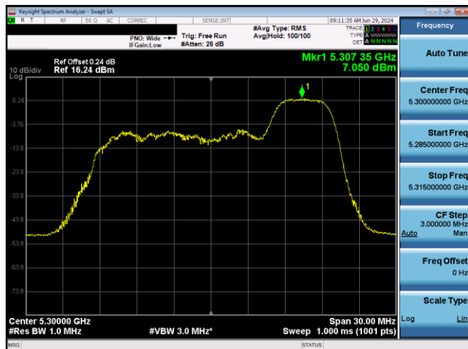
Plot 7-560. PSD SDM Diversity Antenna 5T (20MHz BW 11ax Index 40 - RU52 - Ch.60)
