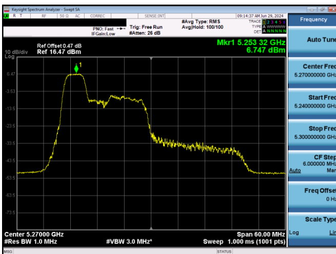
Plot 7-564. PSD SDM Diversity Antenna 5T (40MHz BW 11ax Index 37 - RU52 - Ch.54)
