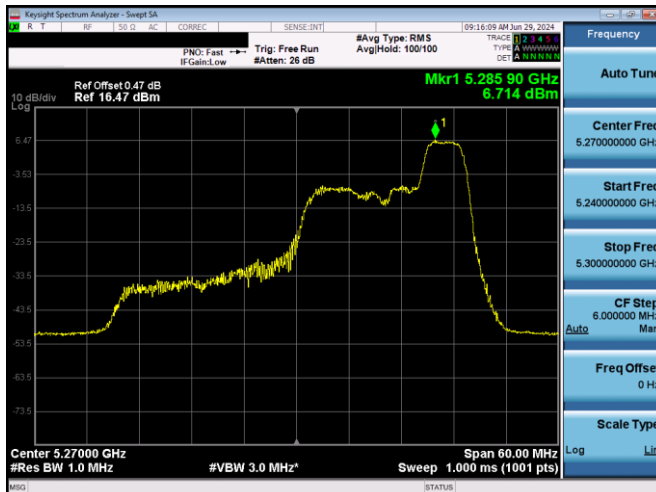
Plot 7-568. PSD SDM Diversity Antenna 5T (40MHz BW 11ax Index 44 - RU52 - Ch.54)
