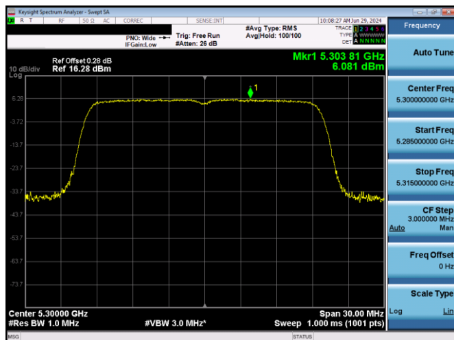
Plot 7-562. PSD SDM Diversity Antenna 5T (20MHz BW 11ax- RU242 - Ch.60)
