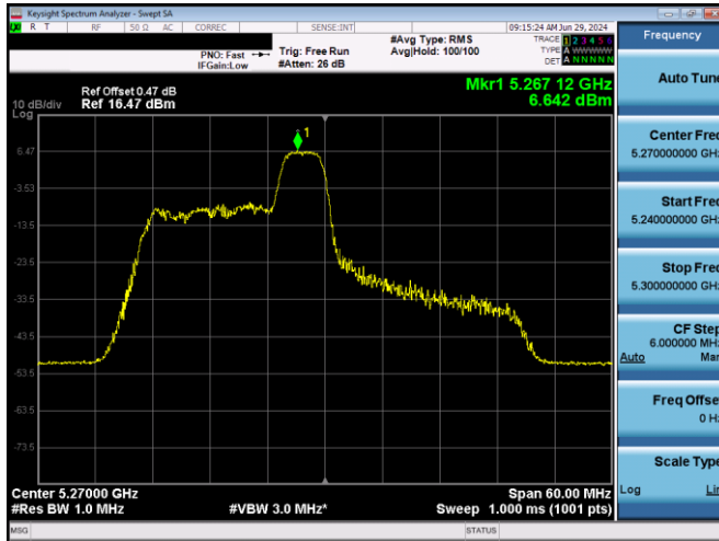
Plot 7-566. PSD SDM Diversity Antenna 5T (40MHz BW 11ax Index 40 - RU52 - Ch.54)
