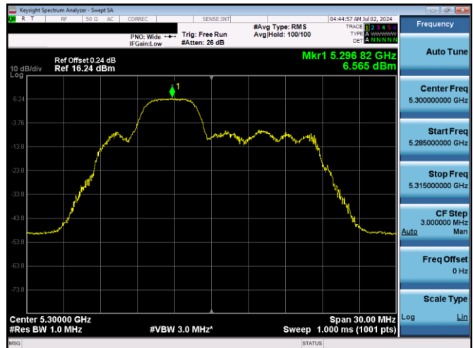
Plot 7-559. PSD SDM Diversity Antenna 1b (20MHz BW 11ax Index 38 - RU52 - Ch.60)
