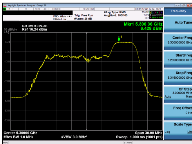
Plot 7-561. PSD SDM Diversity Antenna 1b (20MHz BW 11ax Index 40 - RU52 - Ch.60)
