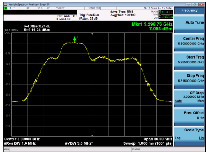
Plot 7-558. PSD SDM Diversity Antenna 5T (20MHz BW 11ax Index 38 - RU52 - Ch.60)
