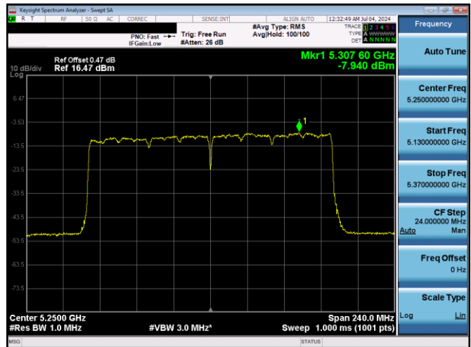
Plot 7-184. PSD Antenna 5T (160MHz BW 11ax - RU96x2 - Ch.50)
