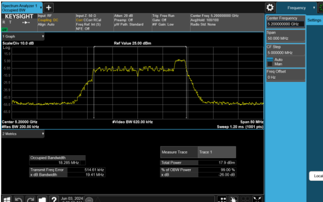
Plot 7-47. 26dB BW & 99% OBW Antenna 3b (20MHz BW 11ax Index 8 – RU26 – Ch.40)
