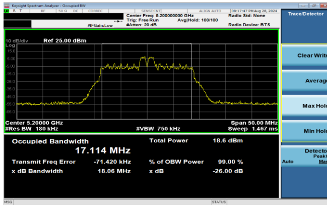
Plot 7-46. 26dB BW & 99% OBW Antenna 3b (20MHz BW 11ax Index 4 – RU26 – Ch.40)
