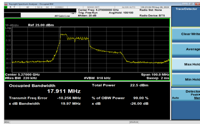
Plot 7-65. 26dB BW & 99% OBW Antenna 3b (40MHz BW 11ax Index 37 – RU52 – Ch.54)
