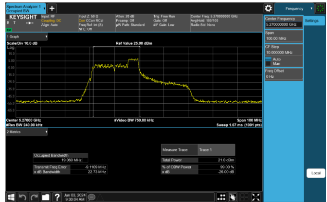
Plot 7-66. 26dB BW & 99% OBW Antenna 3b (40MHz BW 11ax Index 40 – RU52 – Ch.54)
