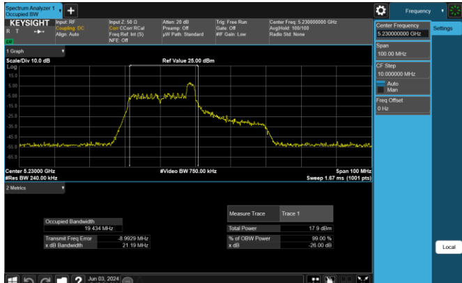
Plot 7-50. 26dB BW & 99% OBW Antenna 3b (40MHz BW 11ax Index 8 – RU26 – Ch.46)
