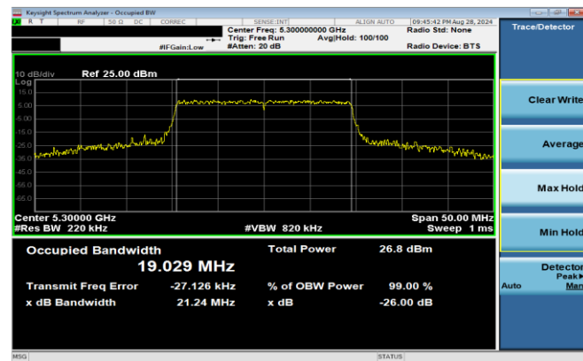
Plot 7-64. 26dB BW & 99% OBW Antenna 3b (20MHz BW 11ax – RU242 – Ch.60)
