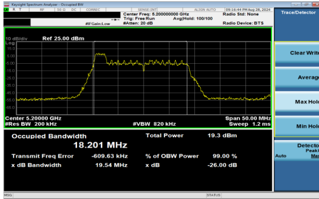
Plot 7-45. 26dB BW & 99% OBW Antenna 3b (20MHz BW 11ax Index 0 – RU26 – Ch.40)
