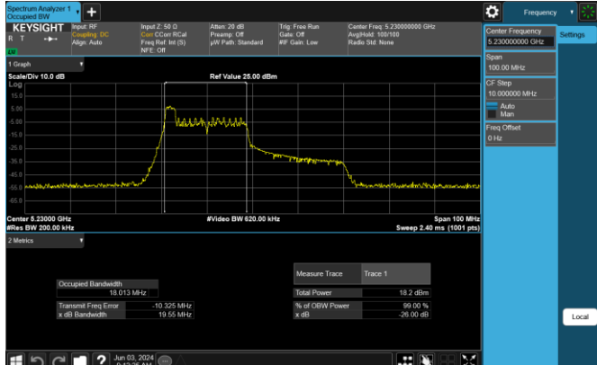
Plot 7-49. 26dB BW & 99% OBW Antenna 3b (40MHz BW 11ax Index 0 – RU26 – Ch.46)
