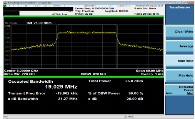
Plot 7-48. 26dB BW & 99% OBW Antenna 3b (20MHz BW 11ax – RU242 – Ch.40)
