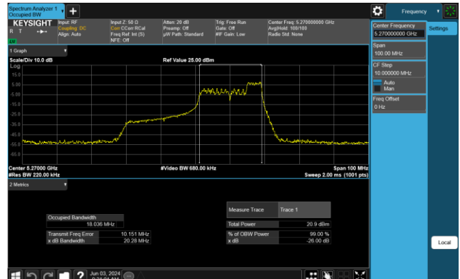
Plot 7-67. 26dB BW & 99% OBW Antenna 3b (40MHz BW 11ax Index 44 – RU52 – Ch.54)
