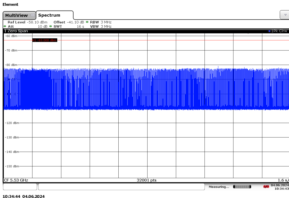
Figure 9-1. 5530MHz - Channel Loading - Mode 1 (80MHz)
