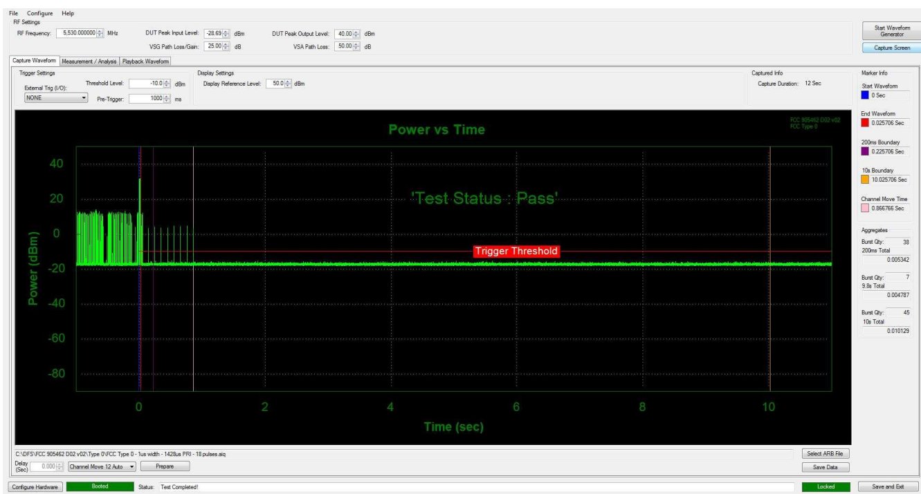
Figure 9-13. 5530MHz - Channel Move/ Closing Transmission Time - Mode 2 (80 MHz)
