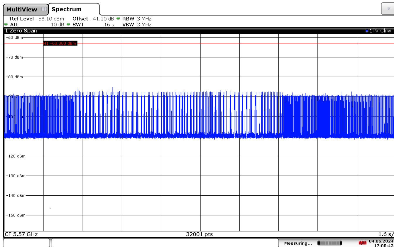
Figure 9-3. 5570MHz - Channel Loading - Mode 1 (160MHz)
