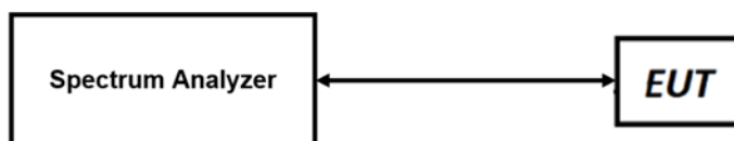
Figure 7-2. FR1 Test Instrument & Measurement Setup
