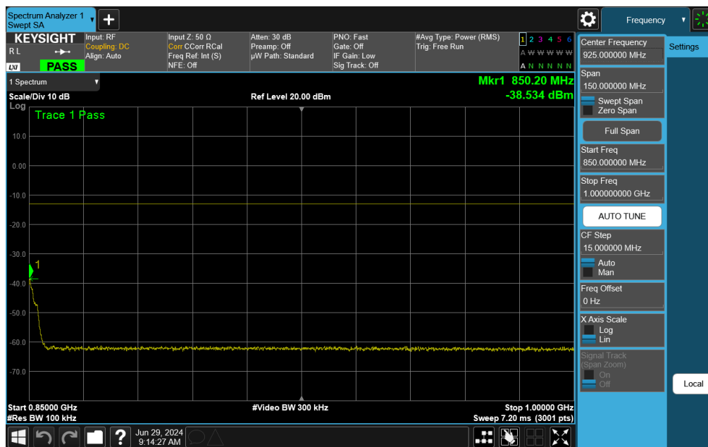
Plot 7-76. Conducted Spurious Plot (WCDMA Ch. 4233)
