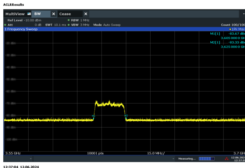
Plot 7-168. Run#1 End User Device Frequency of Operations
