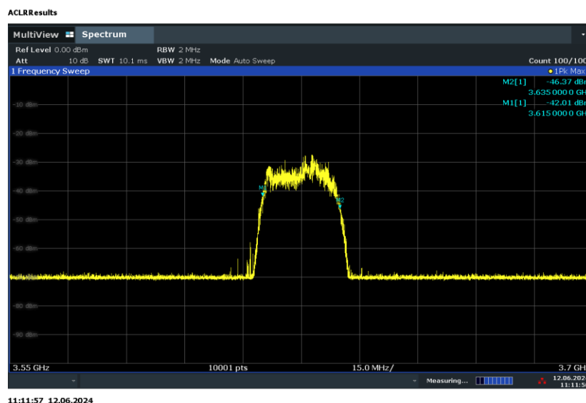
Plot 7-170. Run#2 End User Device Frequency of Operations
