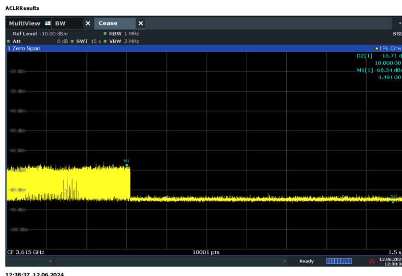
Plot 7-169. Run#1 End User Device Discontinues Operations within 10s
