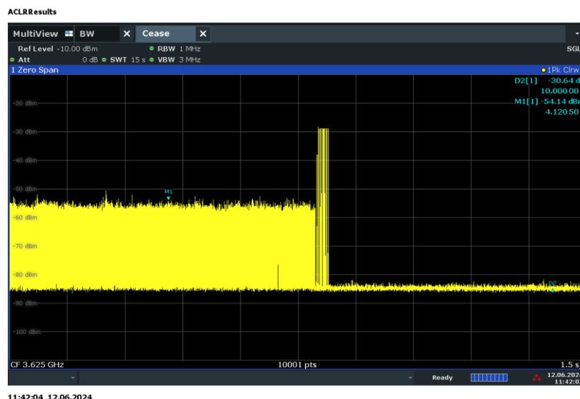
Plot 7-171. Run#2 End User Device Discontinues Operations within 10s
