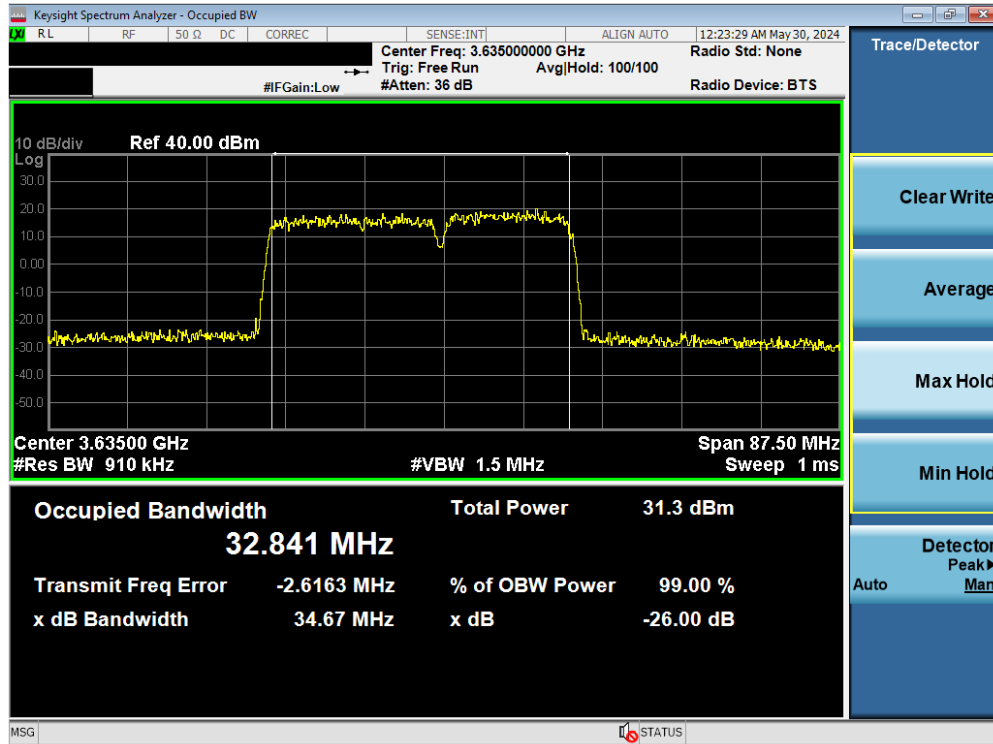
Plot 7-27. Occupied Bandwidth Plot (ULCA LTE Band 48 - 20+15MHz 64-QAM - Full RB Configuration)
