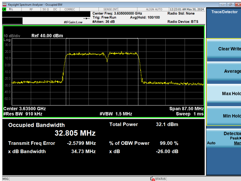
Plot 7-26. Occupied Bandwidth Plot (ULCA LTE Band 48 - 20+15MHz 16-QAM - Full RB Configuration)
