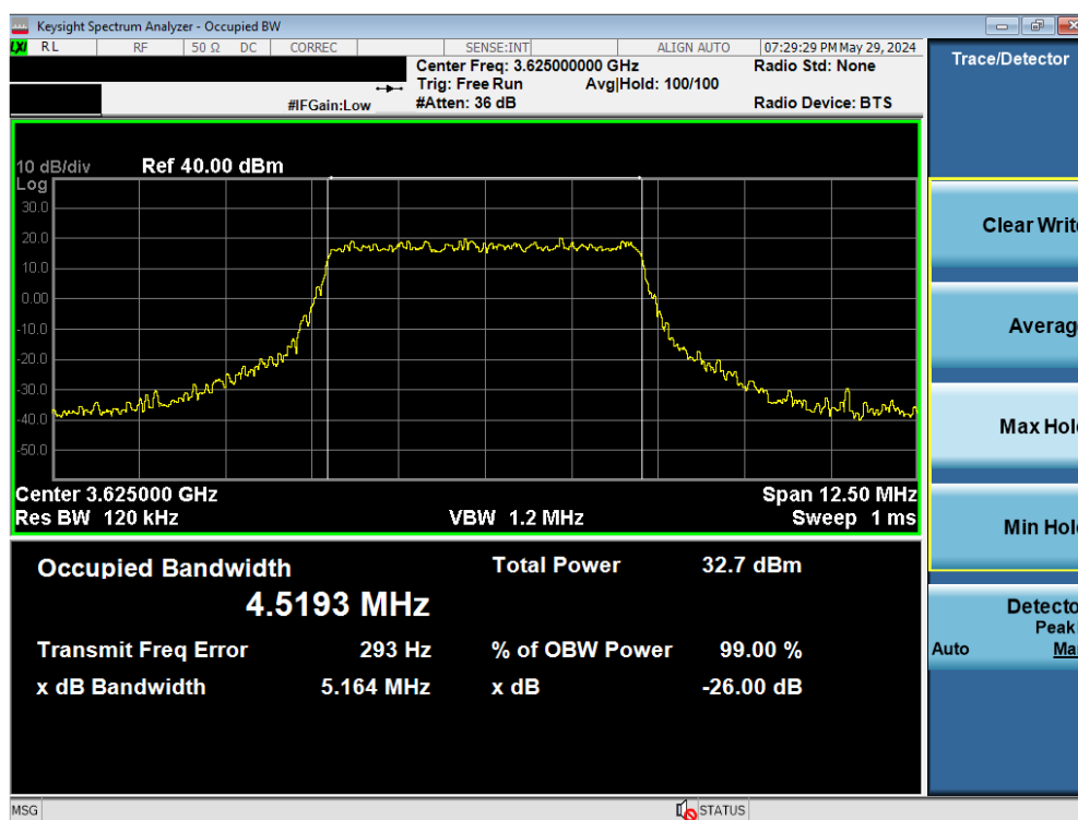
Plot 7-1. Occupied Bandwidth Plot (LTE Band 48 - 5MHz QPSK - Full RB Configuration)
