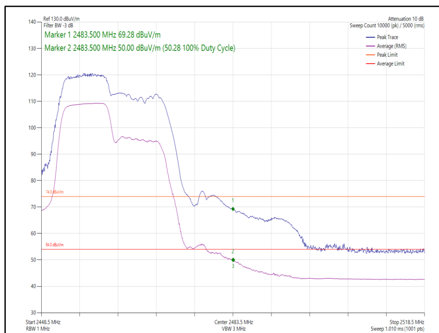
Figure 16 - 802.11ax, HE20, RU 106-53, SISO, Core 0 - 2462 MHz, Band Edge Frequency 2483.5 MHz
