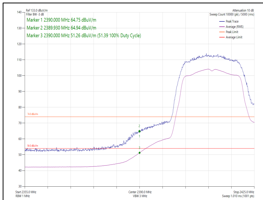
Figure 3 - 802.11n, HT20, SISO, Core 0 - 2412 MHz, Band Edge Frequency 2390 MHz
