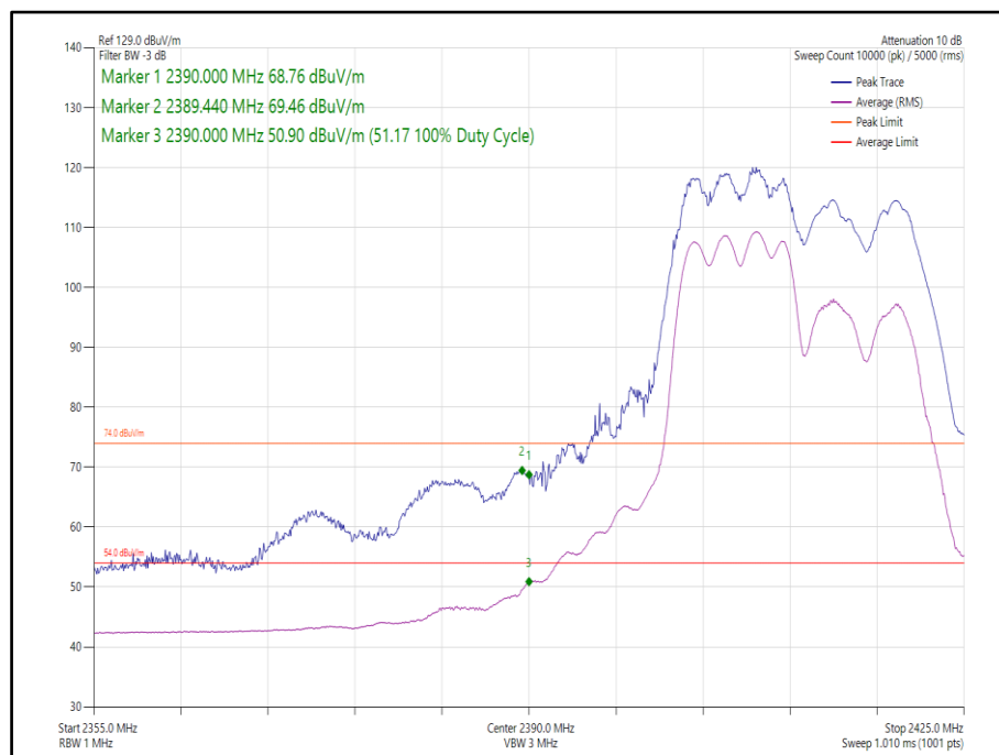
Figure 43 - 802.11ax, HE20, RU 106-53, CDD, Core 0-1 - 2412 MHz, Band Edge Frequency 2390 MHz
