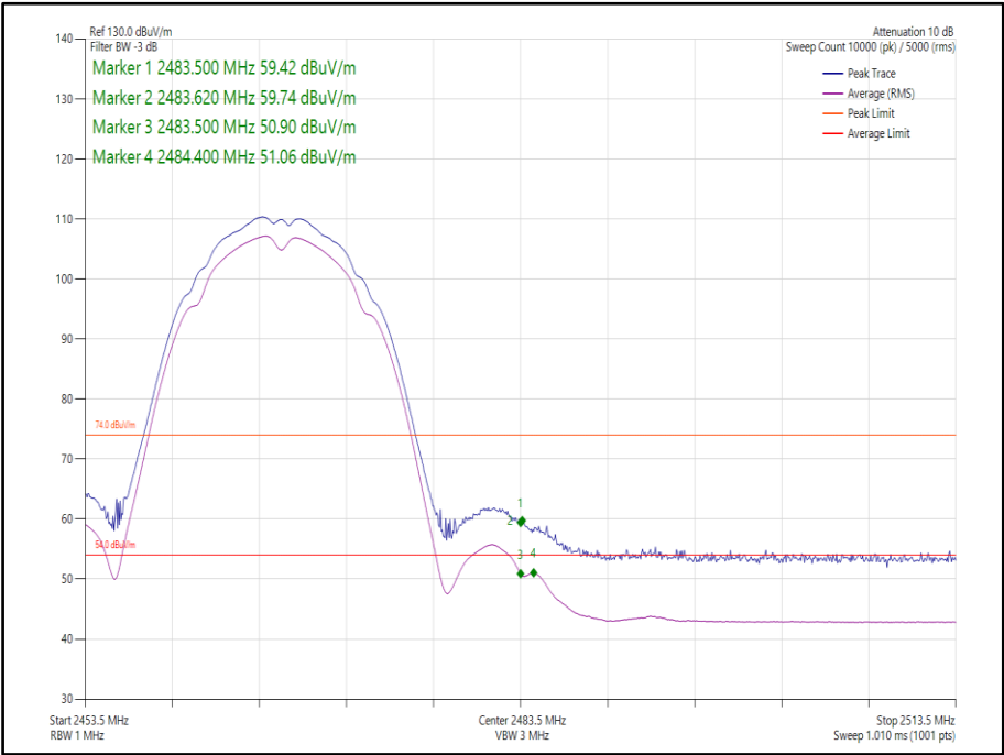
Figure 27 - 802.11b, SISO, Core 1 - 2467 MHz, Band Edge Frequency 2483.5 MHz
