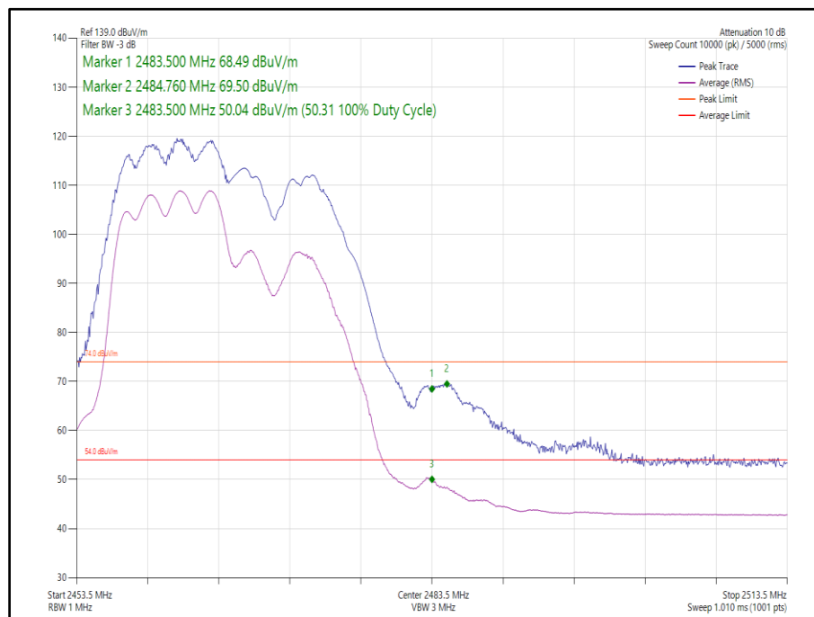
Figure 50 - 802.11ax, HE20, RU 106-53, CDD, Core 0-1 - 2467 MHz, Band Edge Frequency 2483.5 MHz
