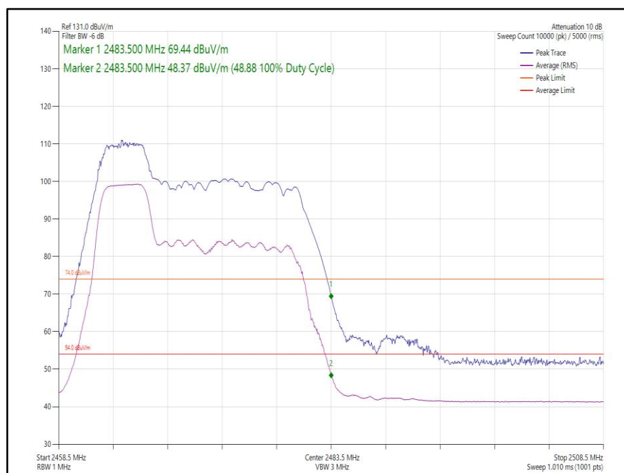
Figure 20 - 802.11ax, HE20, RU 52-37, SISO, Core 0 - 2472 MHz, Band Edge Frequency 2483.5 MHz
