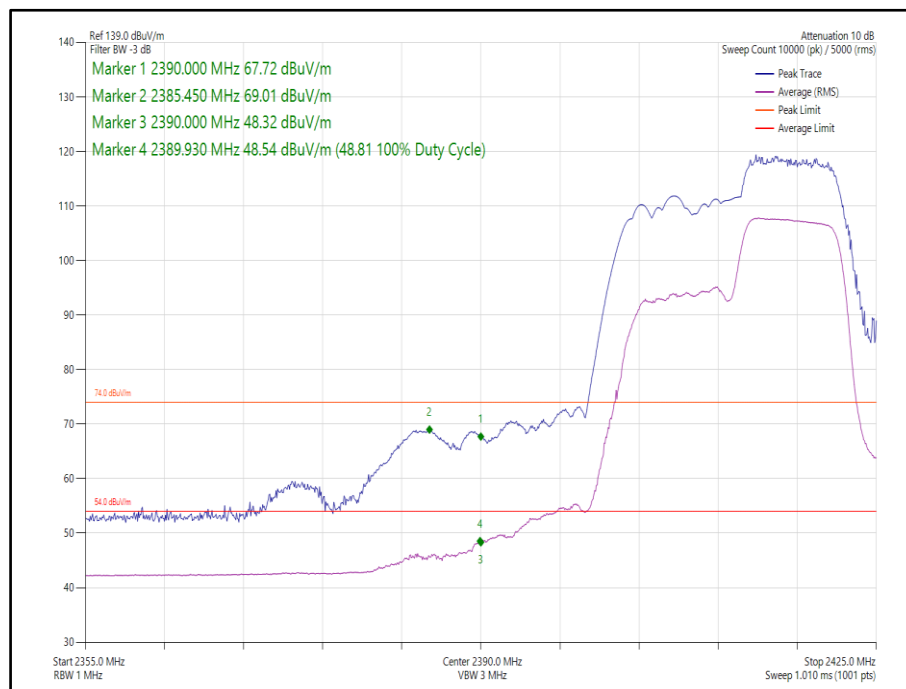
Figure 25 - 802.11ax, HE20, RU 106-54, SISO, Core 1 - 2412 MHz, Band Edge Frequency 2390 MHz
