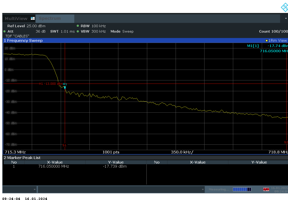
Plot 7-293. Upper Band Edge Plot (LTE Band 12 – 1.4MHz QPSK – Full RB)
