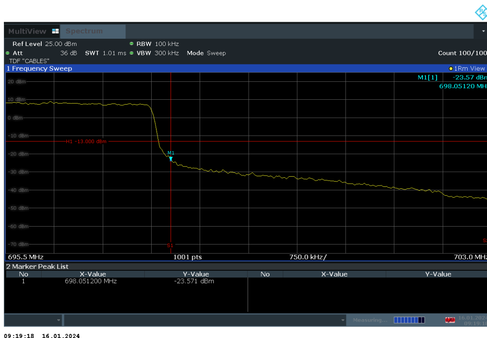
Plot 7-285. Upper Band Edge Plot (LTE Band 71 - 5MHz QPSK – Full RB)
