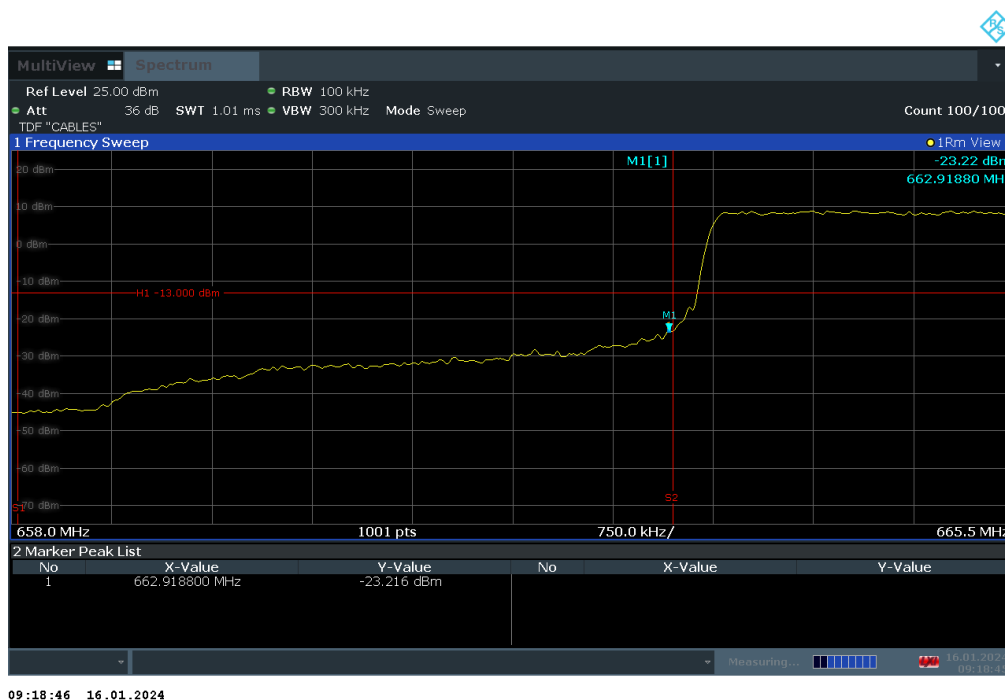
Plot 7-284. Lower Band Edge Plot (LTE Band 71 - 5MHz QPSK – Full RB)
