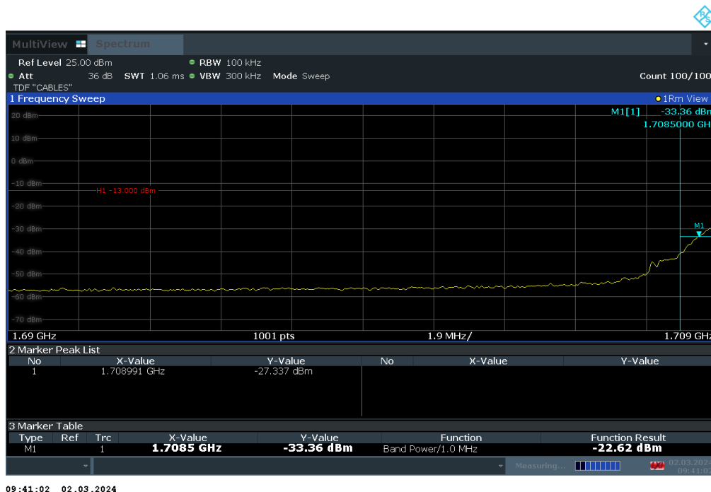
Plot 7-261. Lower Extended Band Edge Plot (LTE Band 4 – 1.4MHz QPSK – Full RB)
