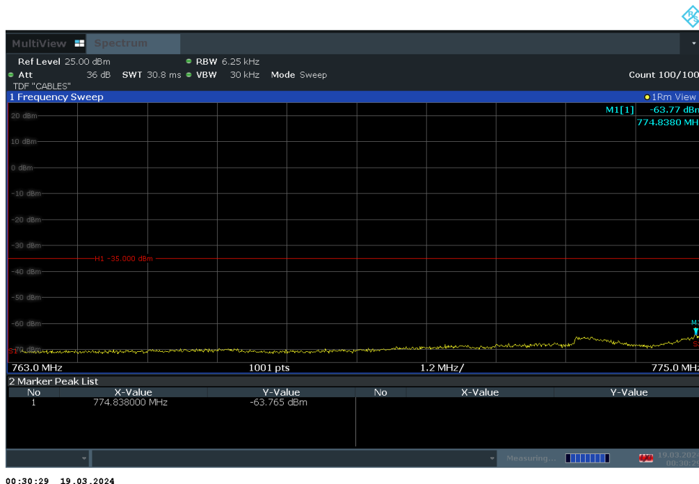
Plot 7-305. Lower Emission Mask Plot (LTE Band 13 - 5MHz QPSK – Full RB)
