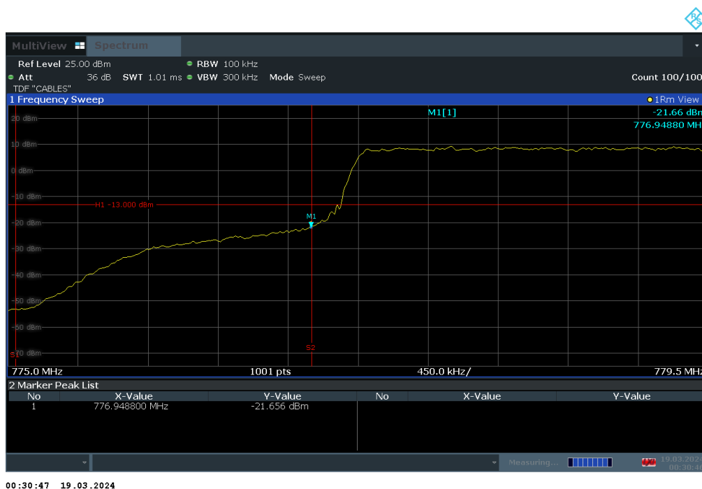
Plot 7-304. Lower Band Edge Plot (LTE Band 13 - 5MHz QPSK – Full RB)
