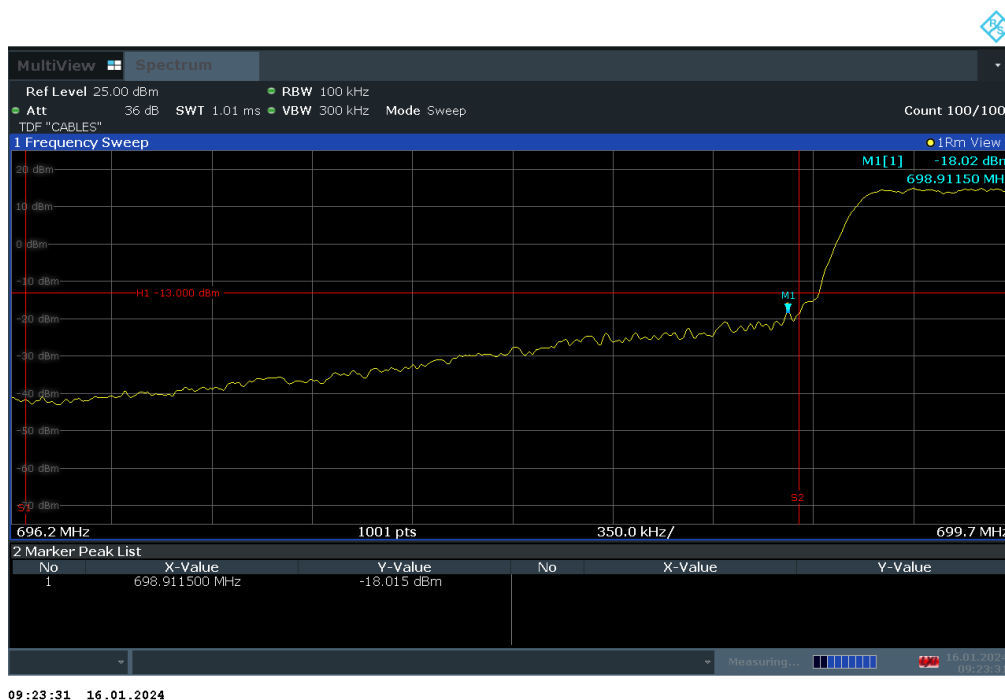
Plot 7-292. Lower Band Edge Plot (LTE Band 12 – 1.4MHz QPSK – Full RB)
