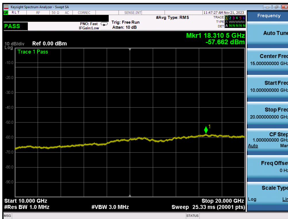
Plot 7-235. Conducted Spurious Plot (WCDMA Ch. 1513- High Channel)
