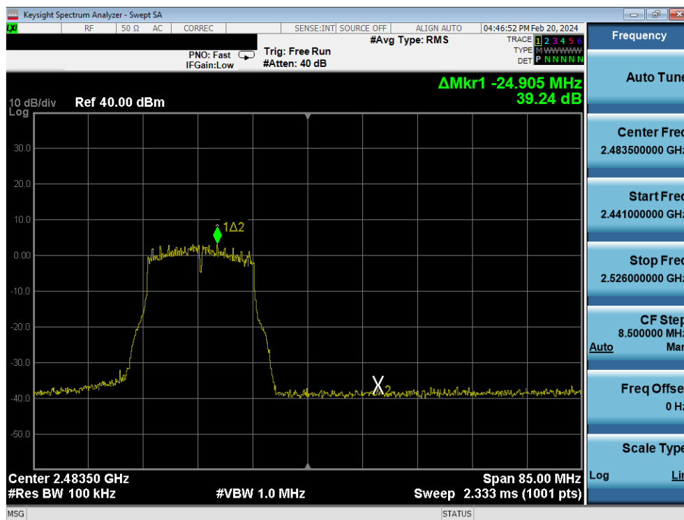
Plot 7-309. Band Edge Plot Antenna 2a (802.11g – Ch. 12) – 24Mbps
