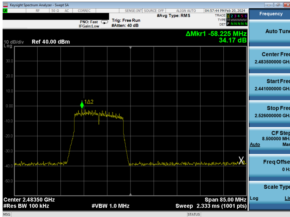
Plot 7-320. Band Edge Plot Antenna 2a (802.11n (2.4GHz) - Ch. 13) - MCS4
