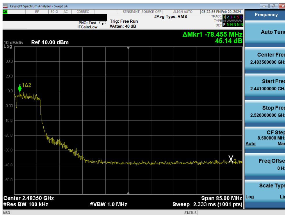
Plot 7-353. Band Edge Plot Antenna 2a (802.11n (2.4GHz) - Ch. 7) - MCS7
