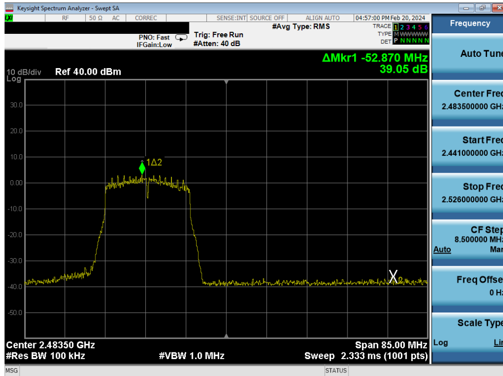
Plot 7-319. Band Edge Plot Antenna 2a (802.11n (2.4GHz) - Ch. 12) - MCS4
