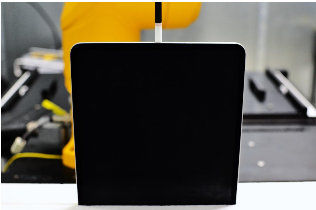
Near Field Power Density Test Setup 10: Top Edge at 2mm – Antenna 2a/4a/WF5B
