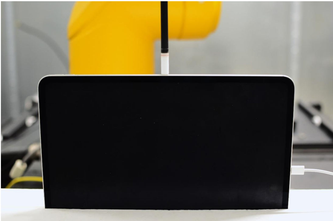
Near Field Power Density Test Setup 12: Right Edge at 2mm – Antenna 2a/4a/WF5B
