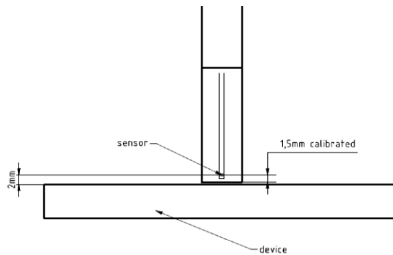
Figure I-2 EUMmWVx Probe
