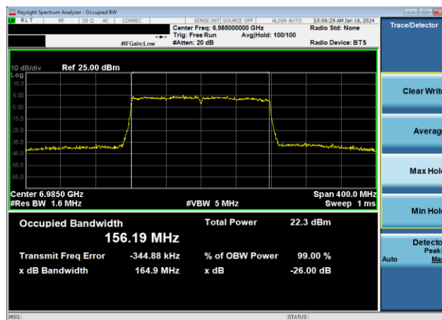
Plot 7-20. 26dB & 99% Bandwidth Plot Antenna WF5B (160MHz 802.11ax (UNII Band 8) – Ch. 207, MCS2)
