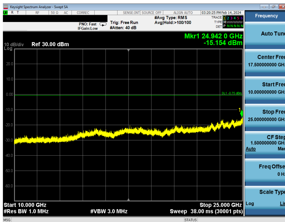
Plot 7-39. Conducted Spurious Antenna WF8 (802.15.4, ePA – Ch. 25)
