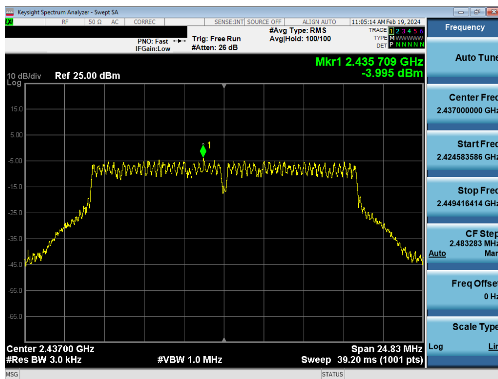
Plot 7-113. Power Spectral Density Plot Antenna WF8 (802.11g – Ch. 6) – 54Mbps
