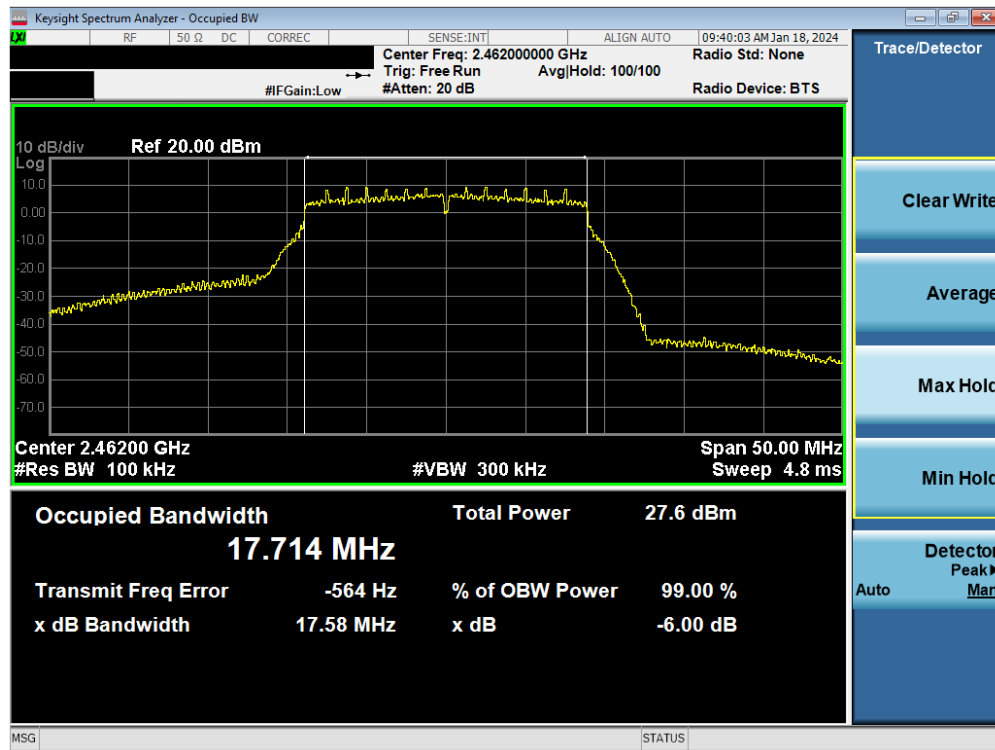
Plot 7-66. 6 dB BW and 99% OBW Plot Antenna WF9 (802.11n (2.4GHz) – Ch. 11) – MCS2
