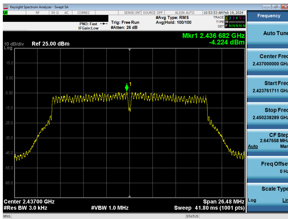
Plot 7-95. Power Spectral Density Plot Antenna WF8 (802.11n (2.4GHz) – Ch. 6) – MCS2
