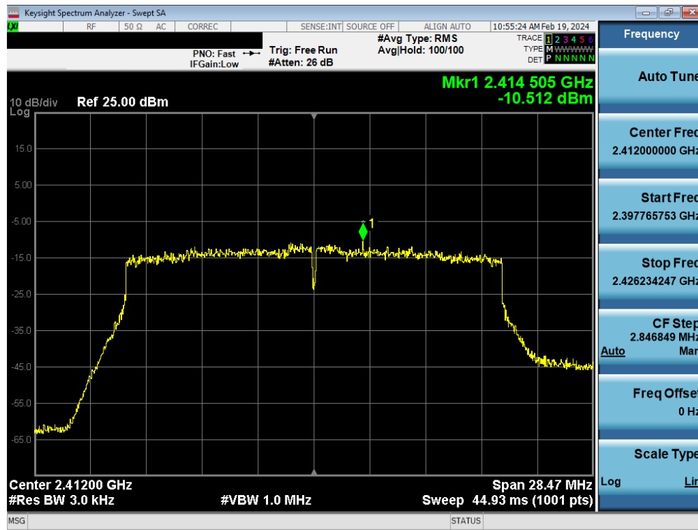
Plot 7-97. Power Spectral Density Plot Antenna WF8 (802.11ax (SU - 2.4GHz) - Ch. 1) - MCS2
