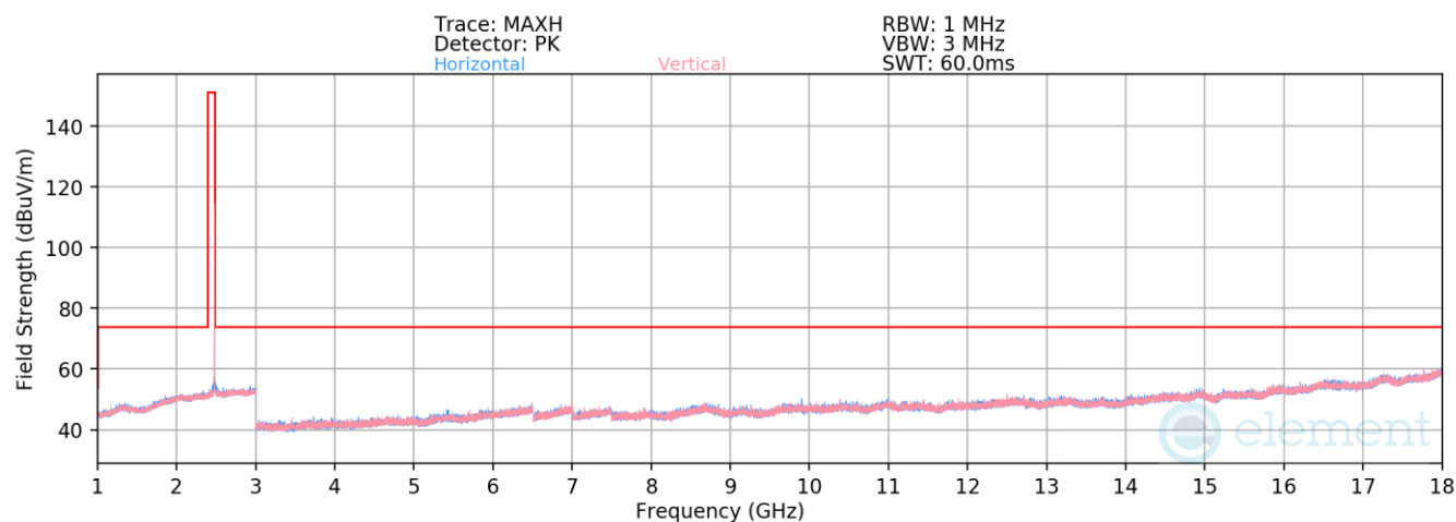
Plot 7-114. Radiated Spurious Emissions 1-18GHz Antenna WF7 (1Mbps ePA – Ch. 39)
