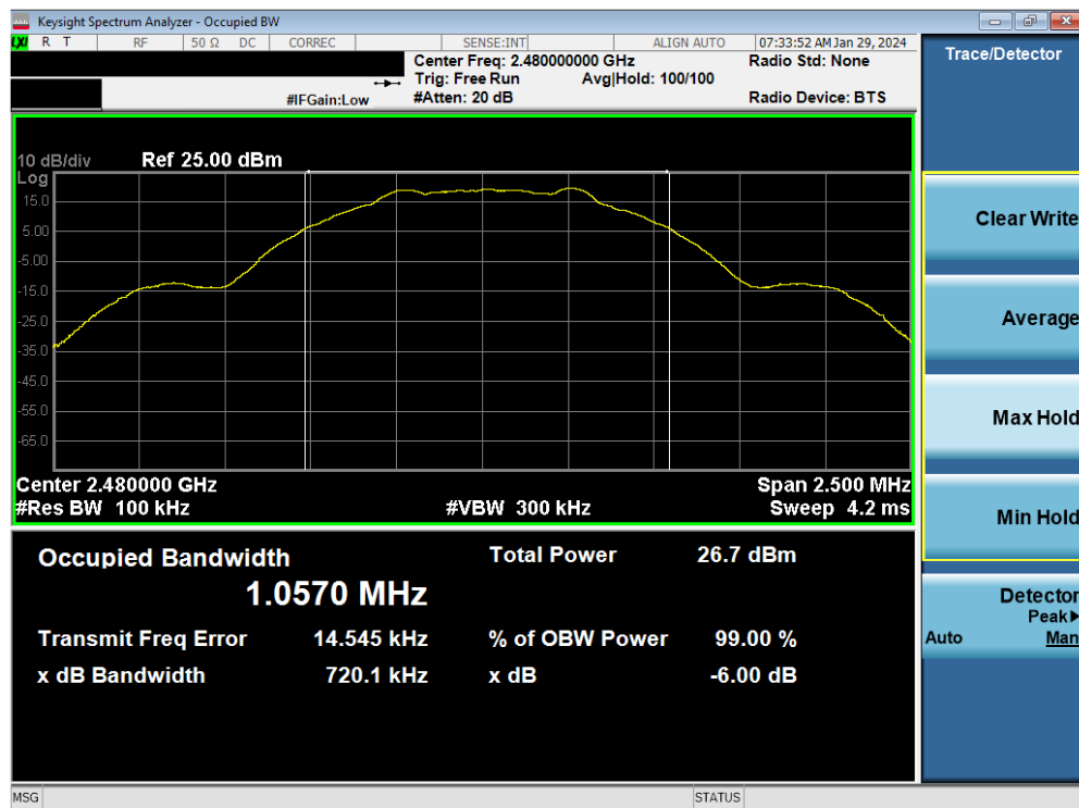
Plot 7-9. 6dB BW & 99% OBW Plot Antenna WF7 (Bluetooth (LE), 1Mbps, ePA – Ch. 39)
