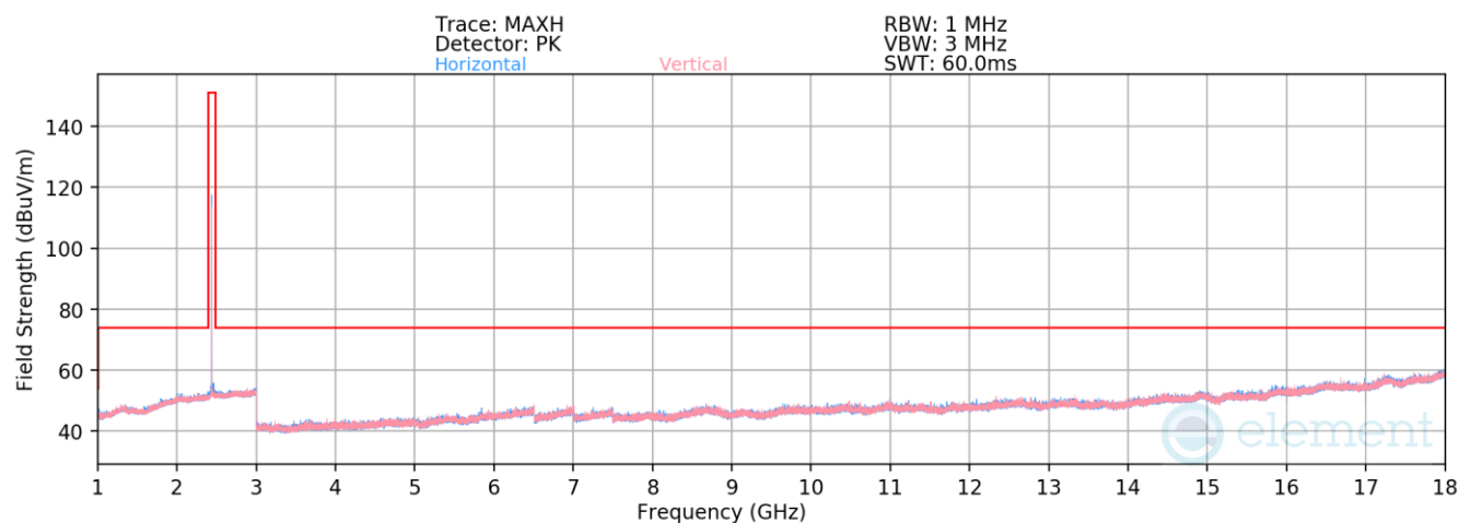
Plot 7-113. Radiated Spurious Emissions 1-18GHz Antenna WF7 (1Mbps, ePA – Ch. 19)
