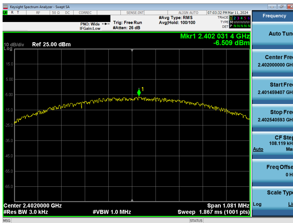
Plot 7-22. Power Spectral Density Plot Antenna WF8 (Bluetooth (LE), 1Mbps, iPA – Ch. 0)
