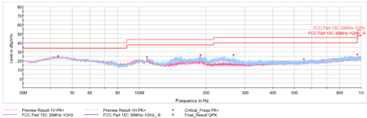
Plot 6-12. Radiated Spurious Emissions 30MHz – 1GHz (Mode 1, with Laptop)
