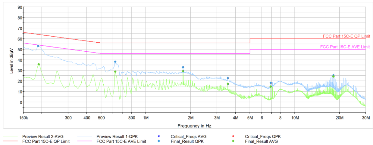
Plot 6-13. AC Line Conducted Plot (L1 - Mode 1, with Laptop)
