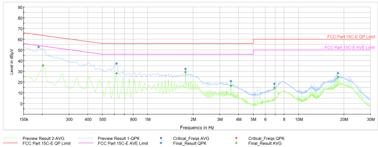
Plot 6-14. AC Line Conducted Plot (N - Mode 1, with Laptop)
