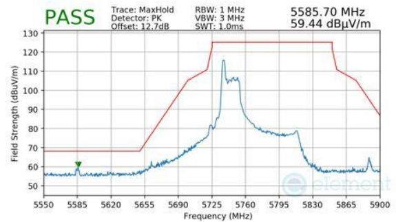
Plot 7-901. ANTENNA 3A (PK, RU26, INDEX 0, CH.155, MCS11)
