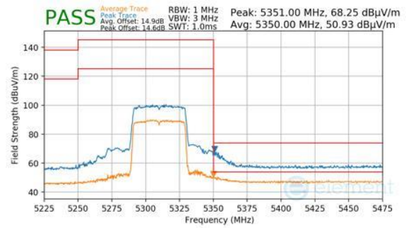
Plot 7-888. ANTENNA 3A (PK & AVG, RU484, INDEX 65, CH.62, MCS11)
