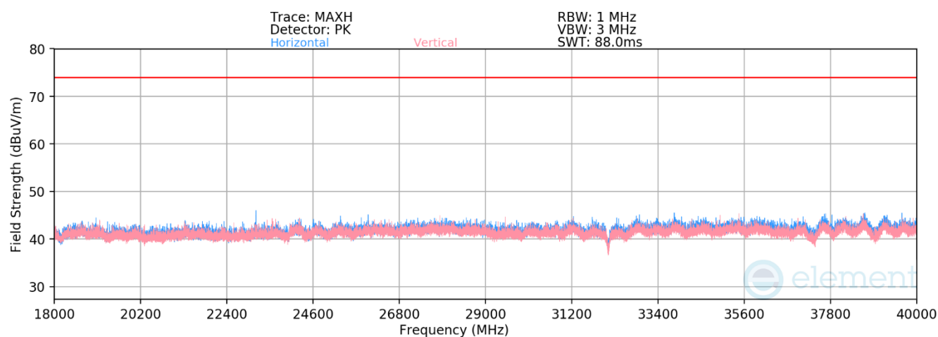
Plot 7-800. RSE 18GHz – 40 GHz CDD Diversity (11ax Ch.157 — RU242)
