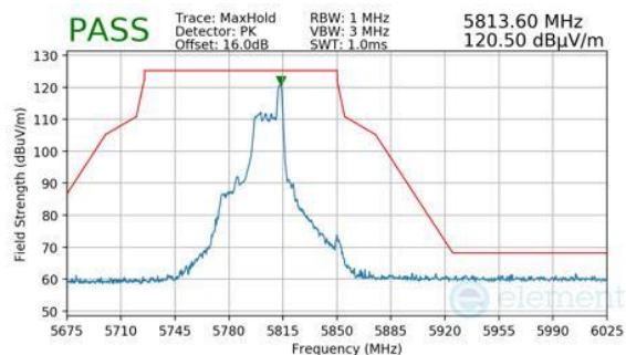
Plot 7-884. ANTENNA 3A (PK, RU26, INDEX 17, CH.159, MCS11)
