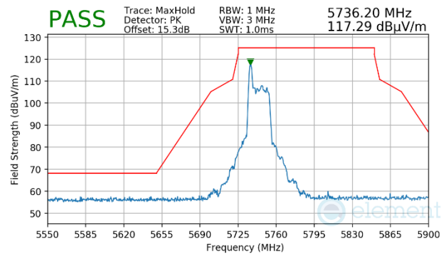
Plot 7-925. ANTENNA 1B (PK, RU26, INDEX 0, CH.149, MCS11)
