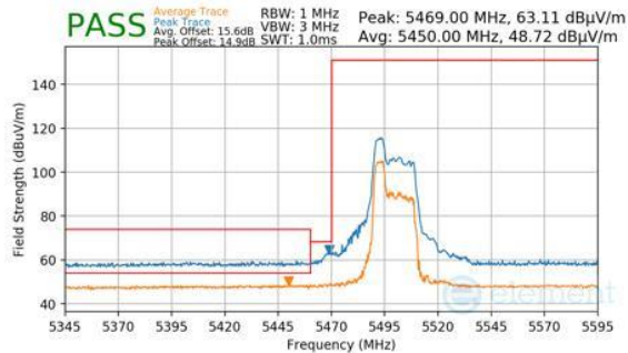
Plot 7-923. ANTENNA 1B (PK & AVG, RU52, INDEX 37, CH.100, MCS11)
