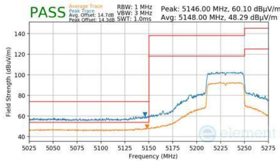
Plot 7-886. ANTENNA 3A (PK & AVG, RU484, INDEX 65, CH.46, MCS11)
