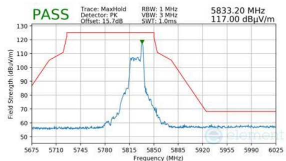
Plot 7-926. ANTENNA 1B (PK, RU26, INDEX 8, CH.165, MCS11)
