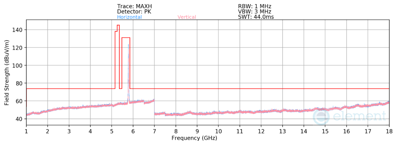
Plot 7-783. RSE above 1GHz CDD Diversity (11ax – Ch.157 – RU26)
