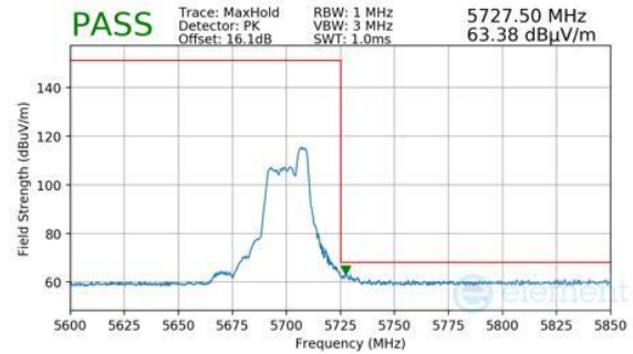
Plot 7-924. ANTENNA 1B (PK, RU52, INDEX 40, CH.140, MCS11)
