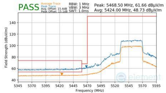
Plot 7-890. ANTENNA 3A (PK & AVG, RU484, INDEX 65, CH.110, MCS11)
