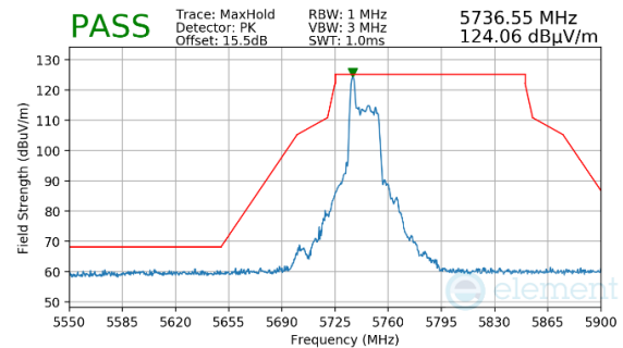
Plot 7-806. ANTENNA 3C (PK, RU26, INDEX 0, CH.149, MCS11)
