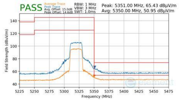
Plot 7-930. ANTENNA 1B (PK & AVG, RU242, INDEX 61, CH.64, MCS11)
