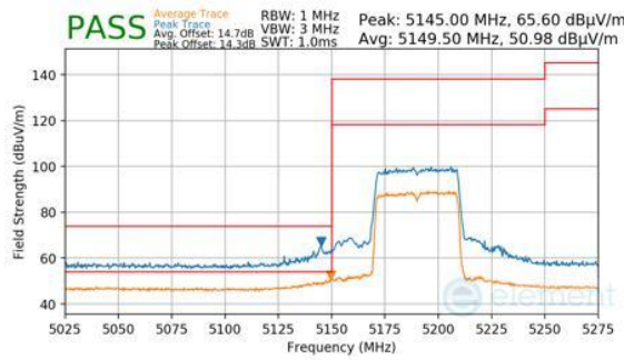
Plot 7-885. ANTENNA 3A (PK & AVG, RU484, INDEX 65, CH.38, MCS11)
