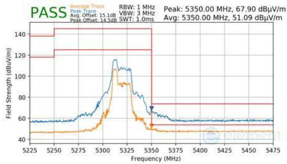
Plot 7-922. ANTENNA 1B (PK & AVG, RU52, INDEX 37, CH.64, MCS11)
