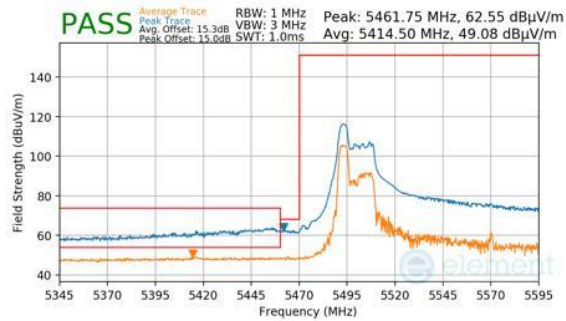
Plot 7-913. ANTENNA 3A (PK & AVG, RU52, INDEX 37, CH.114, MCS11)
