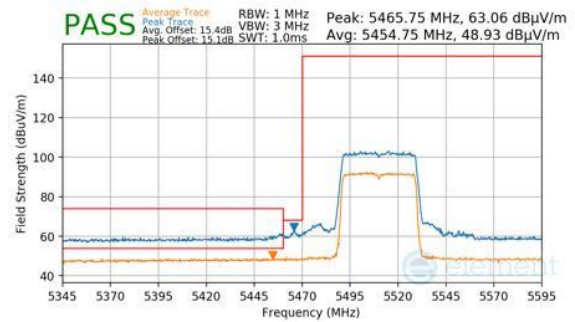
Plot 7-889. ANTENNA 3A (PK & AVG, RU484, INDEX 65, CH.102, MCS11)
