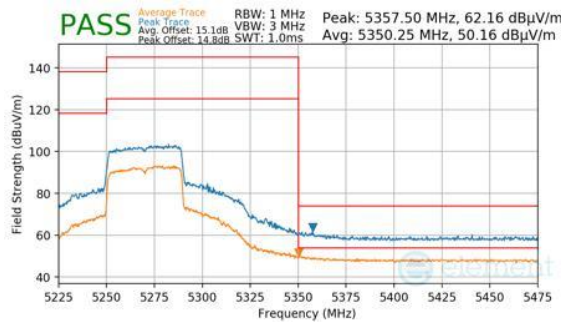
Plot 7-887. ANTENNA 3A (PK & AVG, RU484, INDEX 65, CH.54, MCS11)
