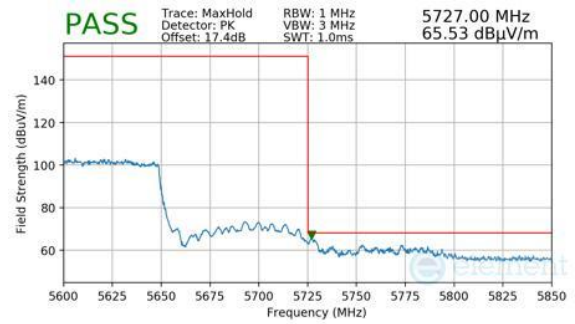
Plot 7-859. ANTENNA 3C (PK, RU996X2, INDEX 68, CH.114, MCS11)
