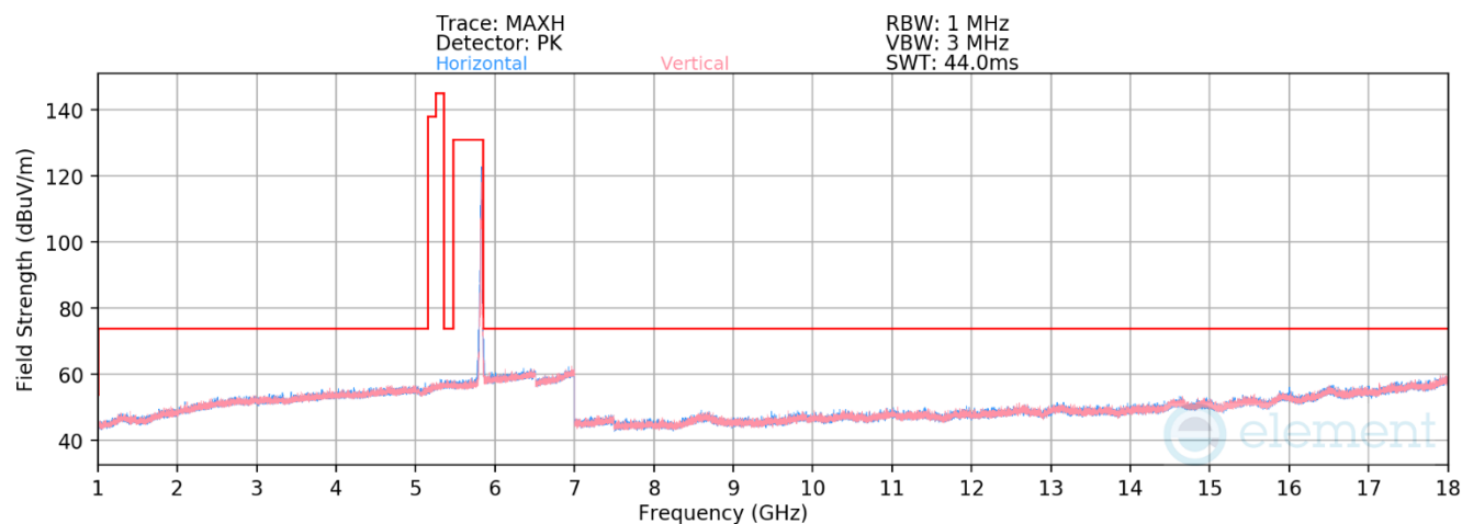
Plot 7-785. RSE above 1GHz CDD Diversity (11ax – Ch.165 – RU26)
