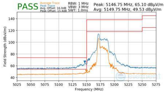
Plot 7-921. ANTENNA 1B (PK & AVG, RU26, INDEX 0, CH.36, MCS11)
