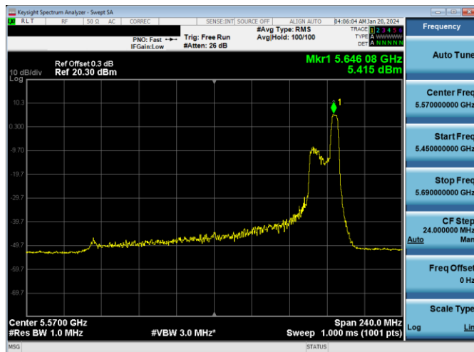
Plot 7-609. PSD CDD Antenna 1b (160MHz BW 11ax Index 52 - RU52 - Ch.114 (U))
