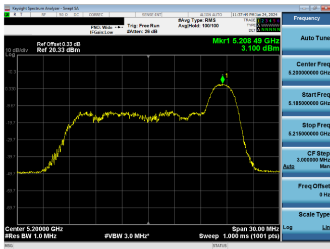
Plot 7-640. ISED PSD SDM Antenna 3c (20MHz BW 11ax Index 8– RU26 – Ch.40)
