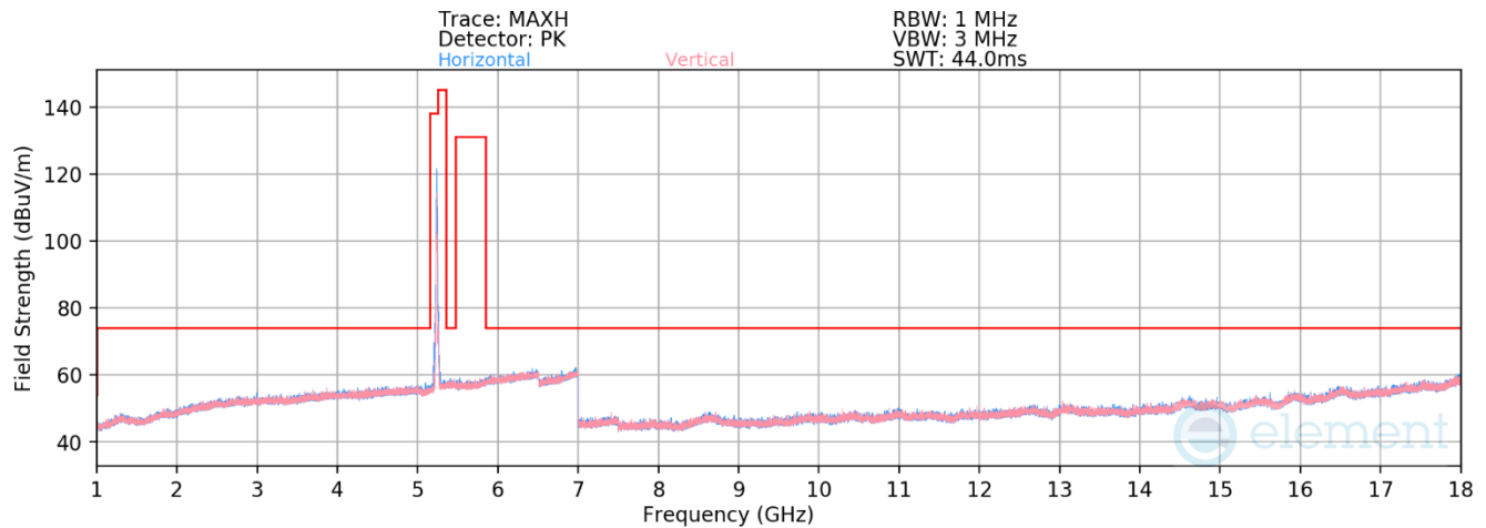
Plot 7-668. RSE above 1GHz Antenna 3c (11ax – Ch.48 – RU26)
