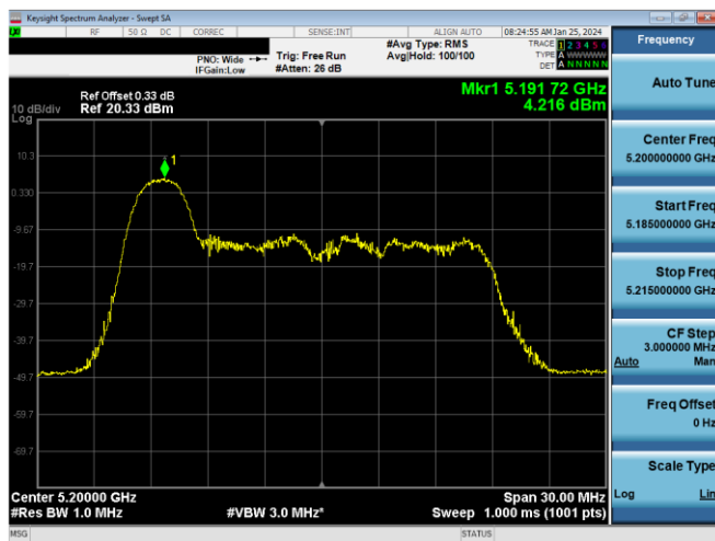
Plot 7-637. ISED PSD SDM Antenna 1b (20MHz BW 11ax Index 0 – RU26 – Ch.40)
