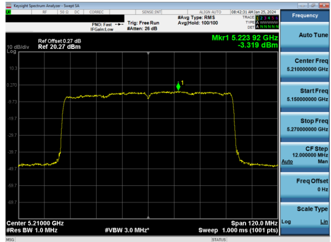
Plot 7-659. ISED PSD CDD Antenna 1b (80MHz BW 11ax – RU996 – Ch.42)
