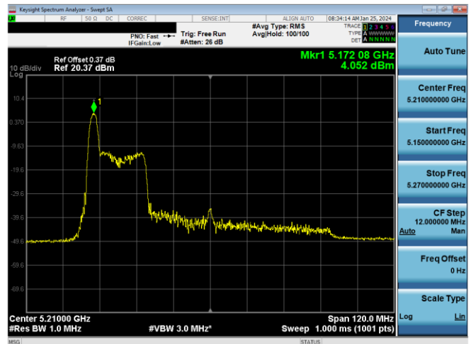
Plot 7-653. ISPD PSD SDM Antenna 1b (80MHz BW 11ax Index 0 - RU26 - Ch.42)
