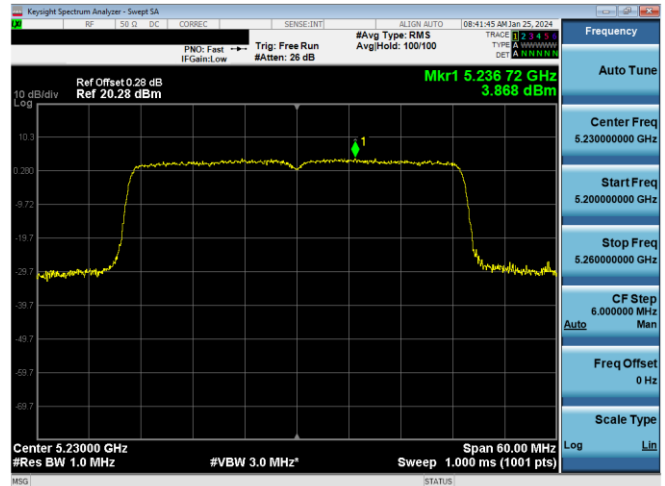
Plot 7-651. ISPD PSD SDM Antenna 1b (40MHz BW 11ax - RU484 - Ch.46)
