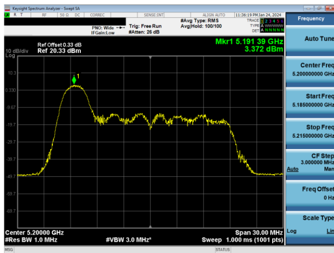
Plot 7-636. ISED PSD SDM Antenna 3c (20MHz BW 11ax Index 0 – RU26 – Ch.40)
