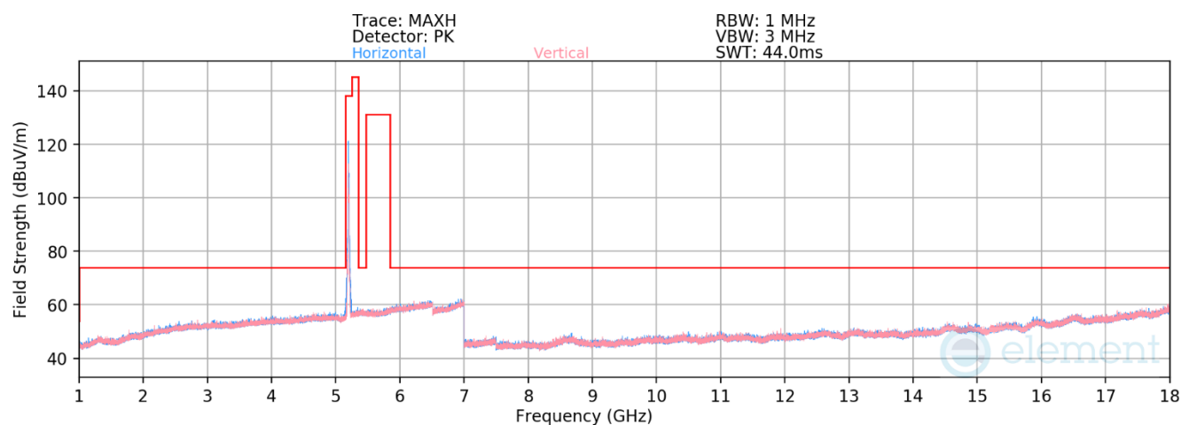
Plot 7-667. RSE above 1GHz Antenna 3c (11ax – Ch.40 – RU26)
