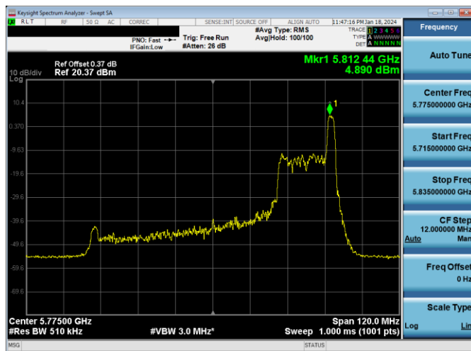
Plot 7-632. PSD CDD Antenna 3c (80MHz BW 11ax Index 36 - RU26 - Ch.155)
