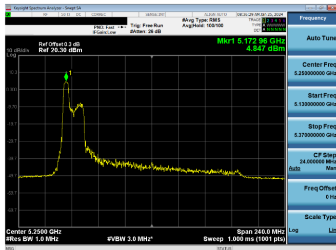
Plot 7-661. ISD PSD SDM Antenna 1b (160MHz BW 11ax Index 37 - RU52 - Ch.50 (L))
