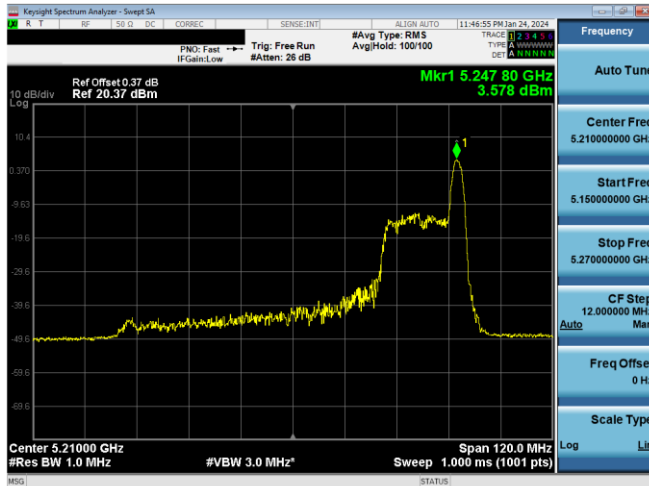
Plot 7-656. ISED PSD SDM Antenna 3c (80MHz BW 11ax Index 36 – RU26 – Ch.42)
