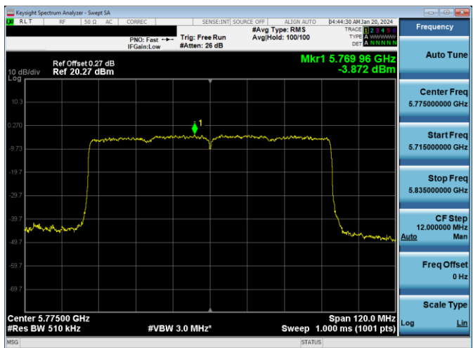
Plot 7-635. PSD CDD Antenna 1b (80MHz BW 11ax - RU996 - Ch.155)
