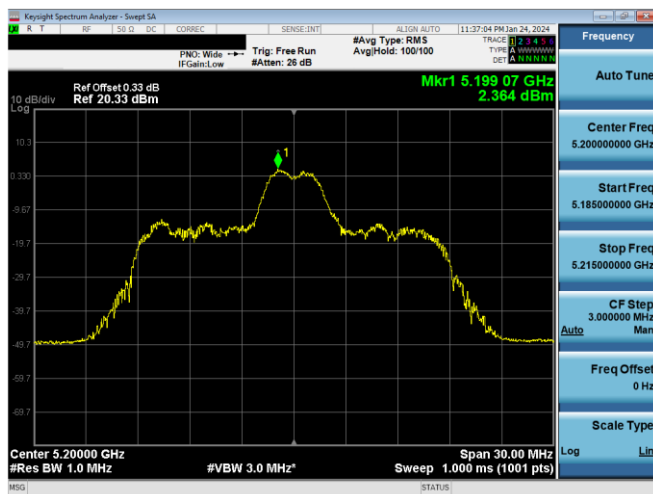
Plot 7-638. ISED PSD SDM Antenna 3c (20MHz BW 11ax Index 4 – RU26 – Ch.40)
