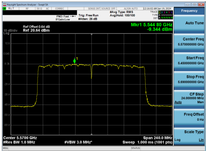
Plot 7-610. PSD CDD Antenna 3c (160MHz BW 11ax - RU996x2 - Ch.114)
