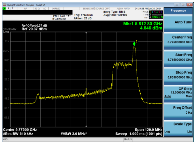
Plot 7-633. PSD CDD Antenna 1b (80MHz BW 11ax Index 36 - RU26 - Ch.155)
