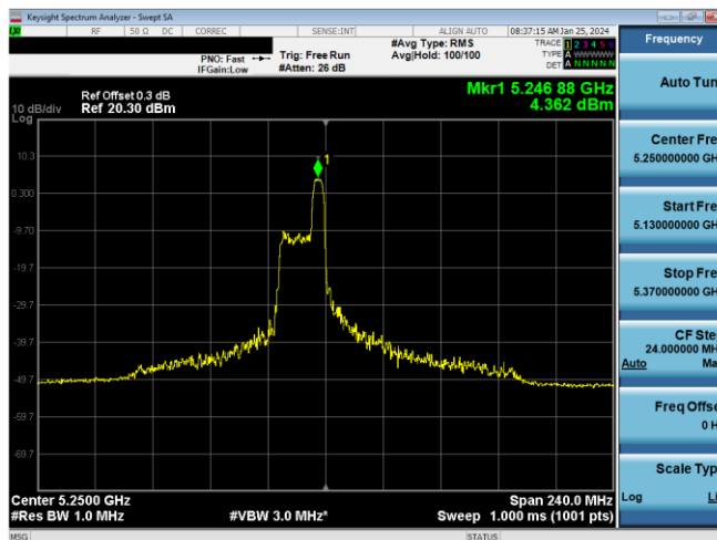
Plot 7-663. ISD PSD SDM Antenna 1b (160MHz BW 11ax Index 44 - RU52 - Ch.50 (L))
