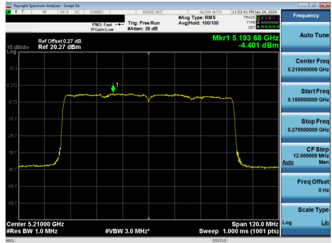
Plot 7-658. ISED PSD CDD Antenna 3c (80MHz BW 11ax – RU996 – Ch.42)
