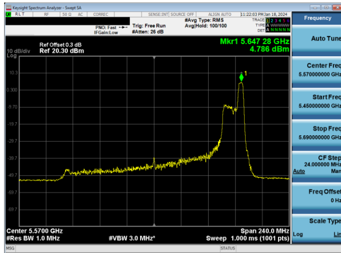
Plot 7-608. PSD CDD Antenna 3c (160MHz BW 11ax Index 52 - RU52 - Ch.114 (U))
