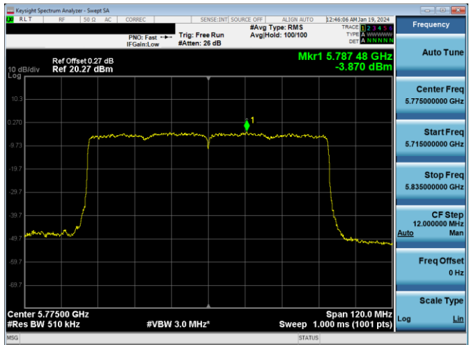
Plot 7-634. PSD CDD Antenna 3c (80MHz BW 11ax - RU996 - Ch.155)
