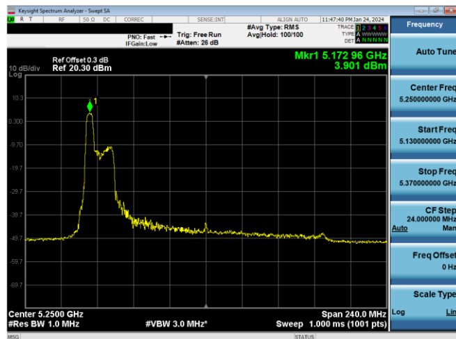
Plot 7-660. ISD PSD SDM Antenna 3c (160MHz BW 11ax Index 37 - RU52 - Ch.50 (L))
