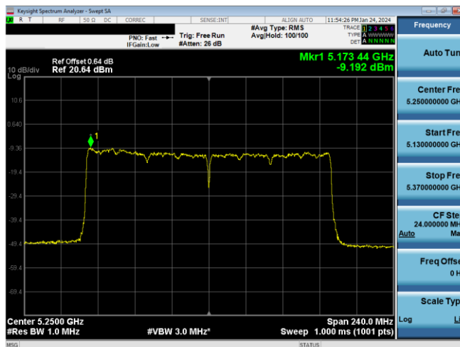
Plot 7-664. ISD PSD CDD Antenna 3c (160MHz BW 11ax - RU996x2 - Ch.50)
