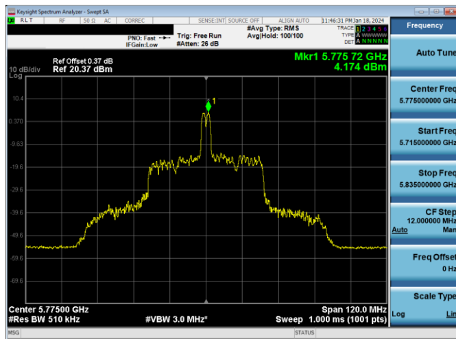
Plot 7-630. PSD CDD Antenna 3c (80MHz BW 11ax Index 18 - RU26 - Ch.155)
