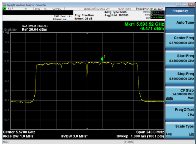
Plot 7-611. PSD CDD Antenna 1b (160MHz BW 11ax - RU996x2 - Ch.114)
