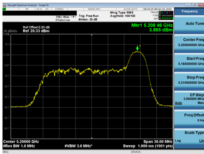
Plot 7-641. ISED PSD SDM Antenna 1b (20MHz BW 11ax Index 8– RU26 – Ch.40)
