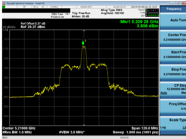
Plot 7-655. ISED PSD SDM Antenna 1b (80MHz BW 11ax Index 18 – RU26 – Ch.42)
