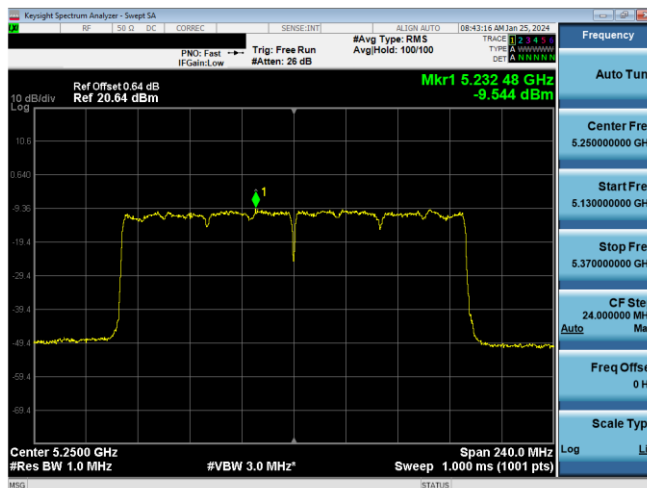
Plot 7-665. ISD PSD CDD Antenna 1b (160MHz BW 11ax - RU996x2 - Ch.50)
