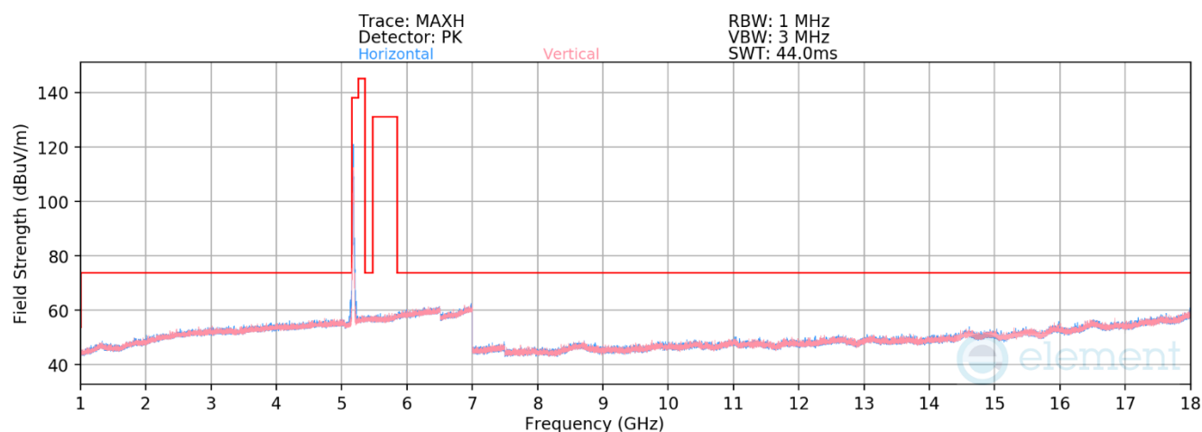
Plot 7-666. RSE above 1GHz Antenna 3c (11ax – Ch.36 – RU26)
