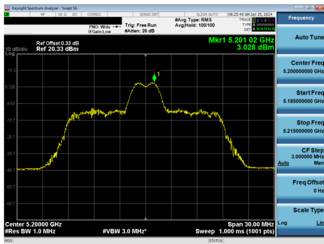
Plot 7-639. ISED PSD SDM Antenna 1b (20MHz BW 11ax Index 4 – RU26 – Ch.40)
