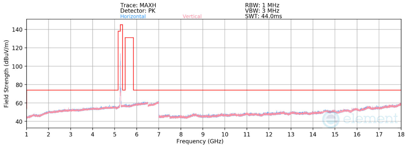
Plot 7-669. RSE above 1GHz Antenna 3c (11ax – Ch.52 – RU52)
