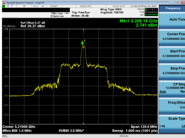
Plot 7-654. ISED PSD SDM Antenna 3c (80MHz BW 11ax Index 18 – RU26 – Ch.42)
