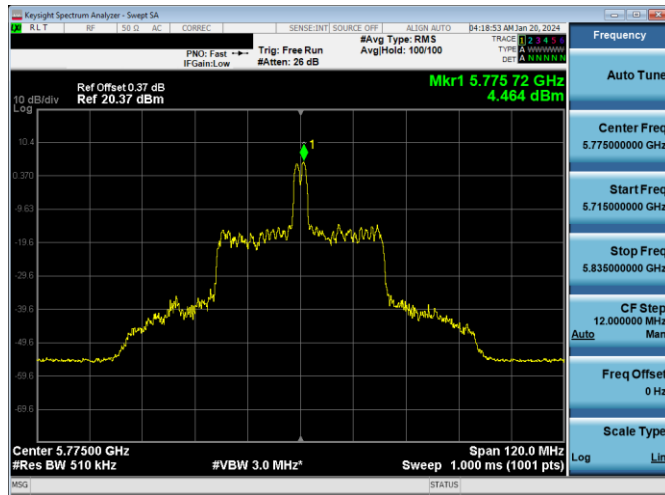
Plot 7-631. PSD CDD Antenna 1b (80MHz BW 11ax Index 18 - RU26 - Ch.155)
