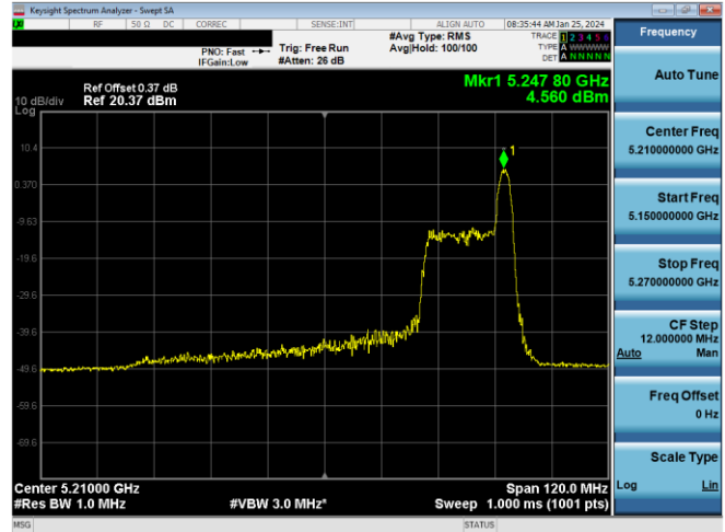
Plot 7-657. ISED PSD SDM Antenna 1b (80MHz BW 11ax Index 36 – RU26 – Ch.42)
