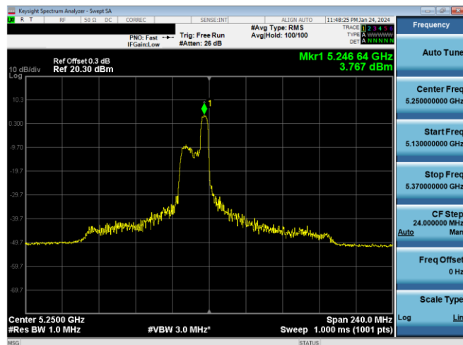
Plot 7-662. ISD PSD SDM Antenna 3c (160MHz BW 11ax Index 44 - RU52 - Ch.50 (L))
