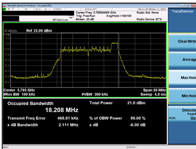
Plot 7-159. 6dB BW & 99% OBW Antenna 1b (20MHz BW 11ax Index 8 – RU26 – Ch.157)
