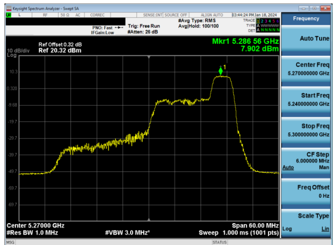
Plot 7-191. PSD Antenna 3c (40MHz BW 11ax Index 44 - RU52 - Ch.54)
