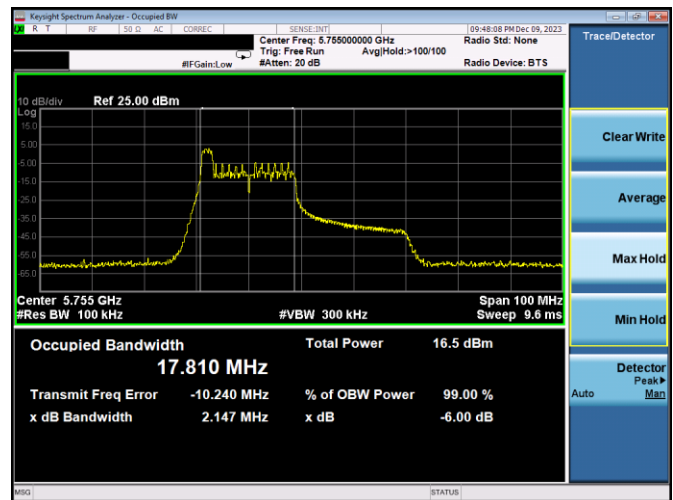
Plot 7-149. 6dB BW & 99% OBW Antenna 3a (40MHz BW 11ax Index 0 – RU26 – Ch.151)
