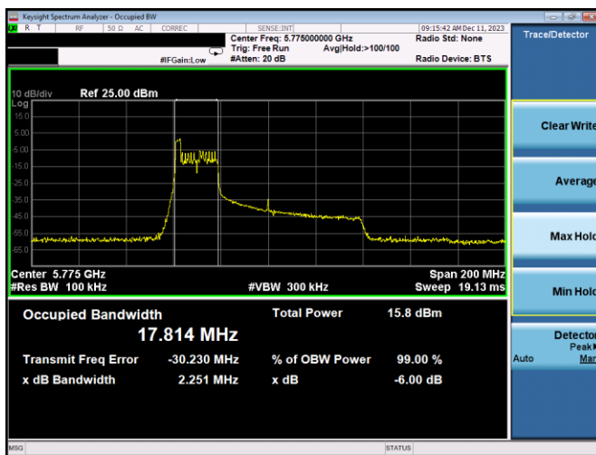
Plot 7-165. 6dB BW & 99% OBW Antenna 1b (80MHz BW 11ax Index 0 – RU26 – Ch.155)
