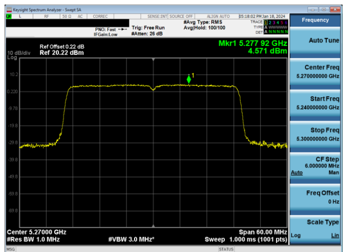
Plot 7-192. PSD Antenna 3c (40MHz BW 11ax - RU484 - Ch.54)
