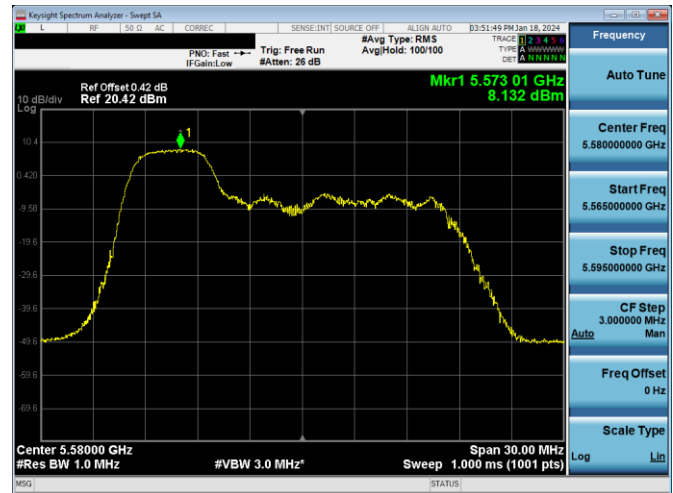
Plot 7-197. PSD Antenna 3c (20MHz BW 11ax Index 37 – RU52 – Ch.116)
