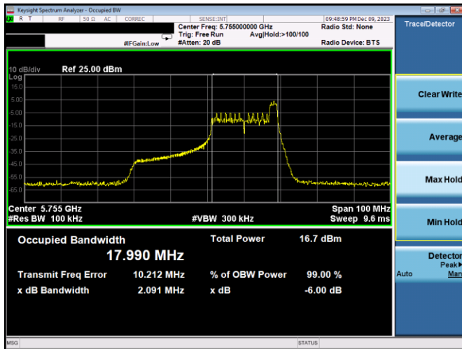
Plot 7-151. 6dB BW & 99% OBW Antenna 3a (40MHz BW 11ax Index 17 – RU26 – Ch.151)
