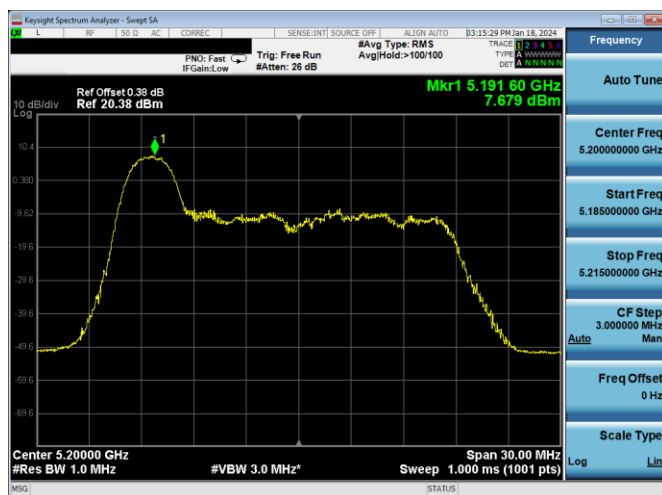
Plot 7-169. PSD Antenna 3c (20MHz BW 11ax Index 0 - RU26 - Ch.40)
