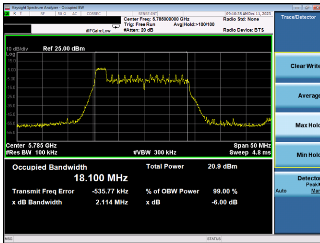
Plot 7-157. 6dB BW & 99% OBW Antenna 1b (20MHz BW 11ax Index 0 – RU26 – Ch.157)
