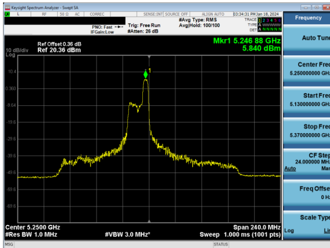
Plot 7-182. PSD Antenna 3c (160MHz BW 11ax Index 52 - RU52 - Ch.50 (L))
