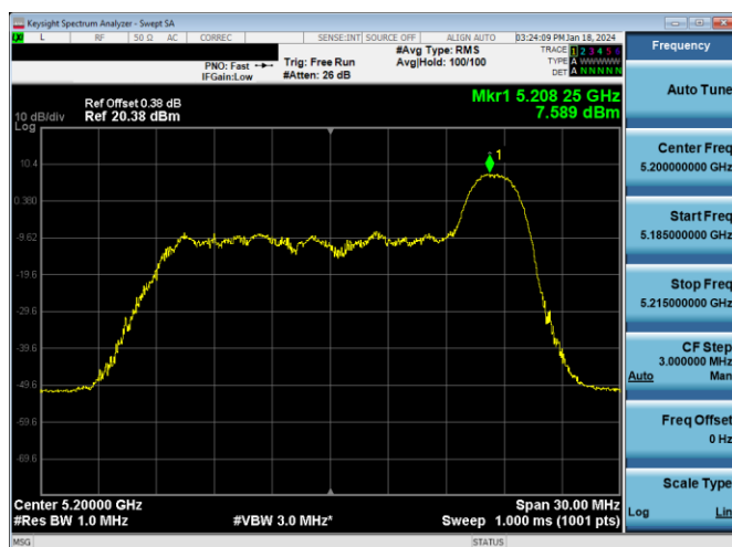
Plot 7-171. PSD Antenna 3c (20MHz BW 11ax Index 8- RU26 - Ch.40)
