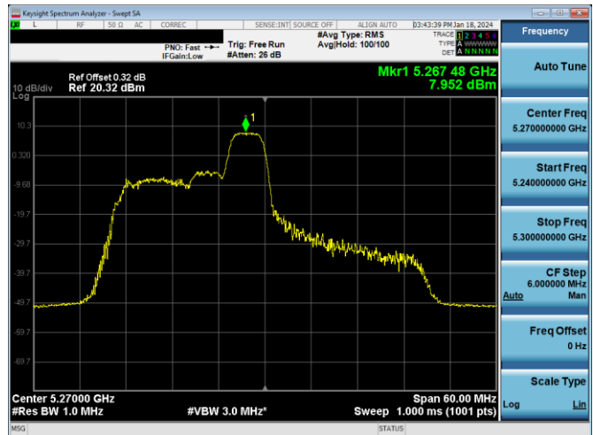
Plot 7-190. PSD Antenna 3c (40MHz BW 11ax Index 40 - RU52 - Ch.54)
