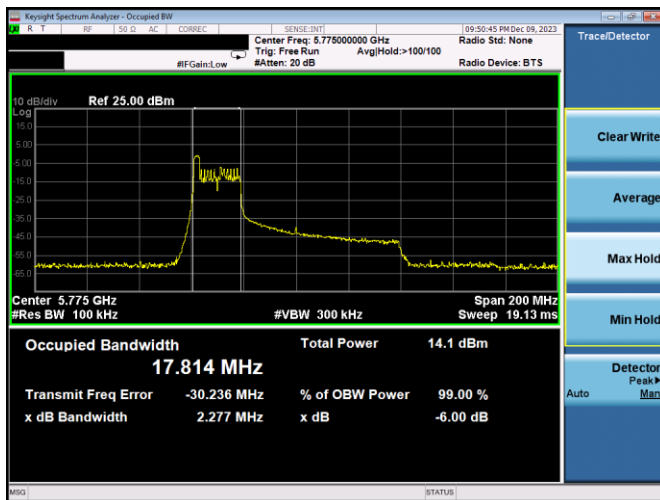
Plot 7-153. 6dB BW & 99% OBW Antenna 3a (80MHz BW 11ax Index 0 – RU26 – Ch.155)
