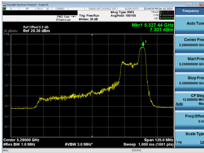
Plot 7-195. PSD Antenna 3c (80MHz BW 11ax Index 52 – RU52 – Ch.58)
