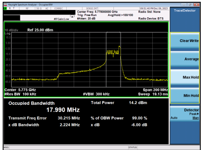
Plot 7-155. 6dB BW & 99% OBW Antenna 3a (80MHz BW 11ax Index 36 – RU26 – Ch.155)
