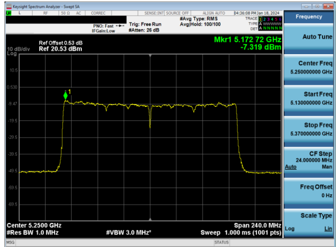
Plot 7-184. PSD Antenna 3c (160MHz BW 11ax - RU96x2 - Ch.50)
