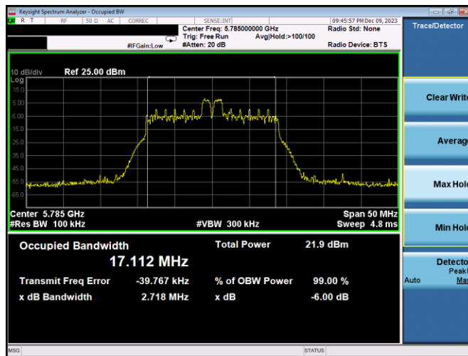
Plot 7-146. 6dB BW & 99% OBW Antenna 3a (20MHz BW 11ax Index 4 – RU26 – Ch.157)
