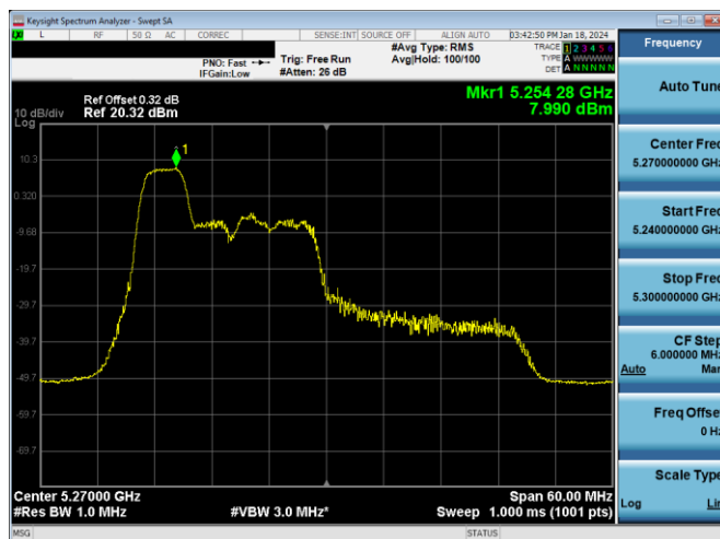
Plot 7-189. PSD Antenna 3c (40MHz BW 11ax Index 37 - RU52 - Ch.54)
