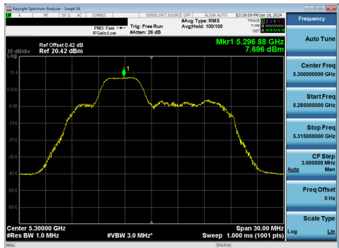
Plot 7-186. PSD Antenna 3c (20MHz BW 11ax Index 38 - RU52 - Ch.60)
