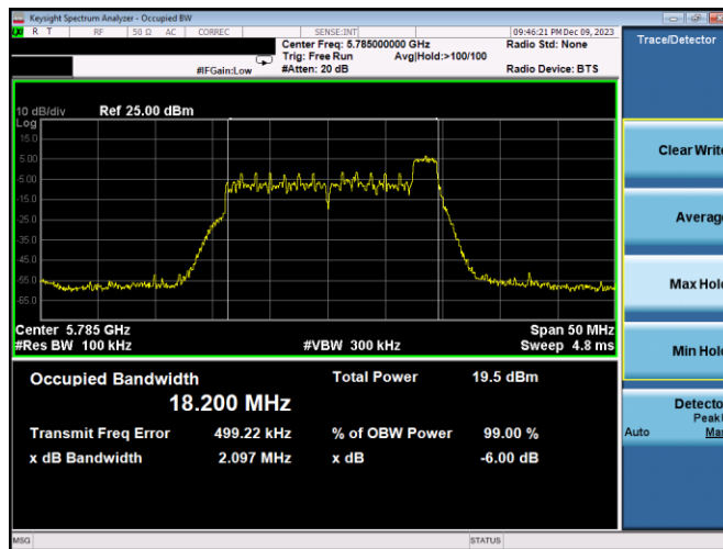
Plot 7-147. 6dB BW & 99% OBW Antenna 3a (20MHz BW 11ax Index 8 – RU26 – Ch.157)
