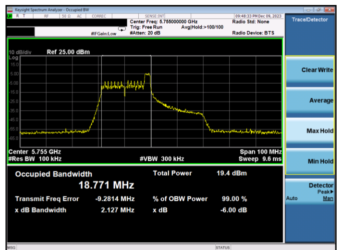
Plot 7-150. 6dB BW & 99% OBW Antenna 3a (40MHz BW 11ax Index 8 – RU26 – Ch.151)
