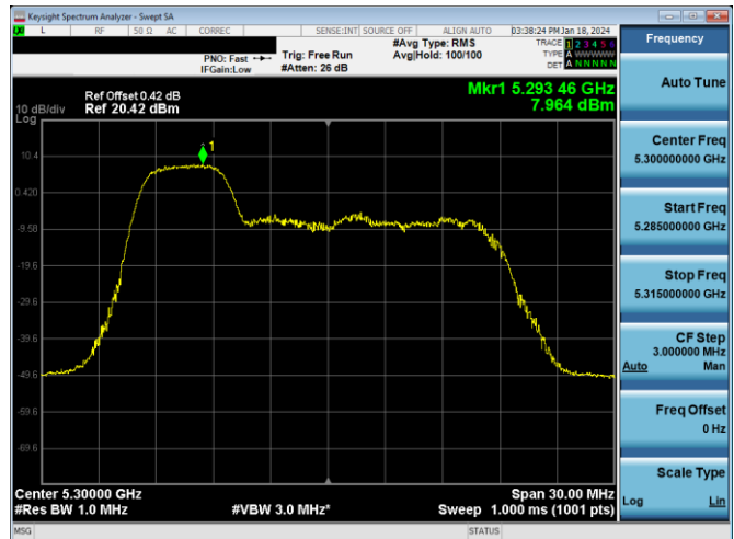
Plot 7-185. PSD Antenna 3c (20MHz BW 11ax Index 37 - RU52 - Ch.60)
