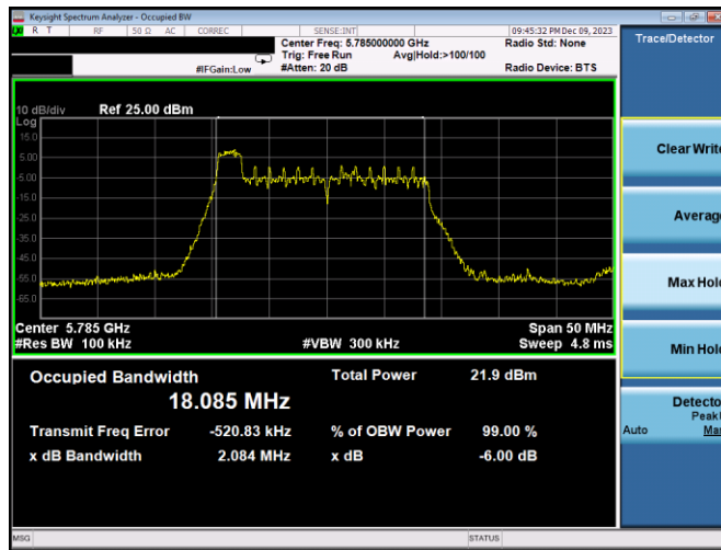
Plot 7-145. 6dB BW & 99% OBW Antenna 3a (20MHz BW 11ax Index 0 – RU26 – Ch.157)
