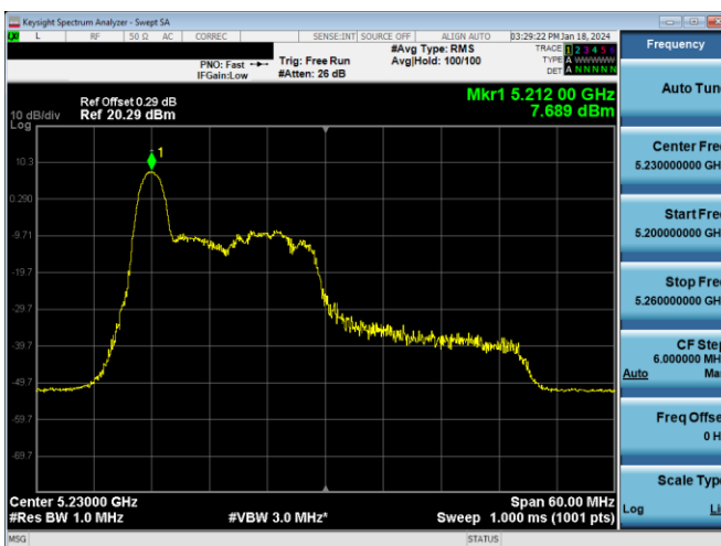
Plot 7-173. PSD Antenna 3c (40MHz BW 11ax Index 0 - RU26 - Ch.46)
