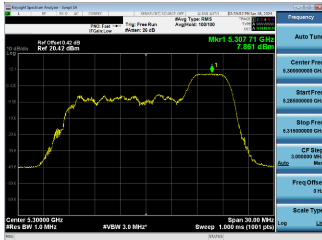
Plot 7-187. PSD Antenna 3c (20MHz BW 11ax Index 40 - RU52 - Ch.60)
