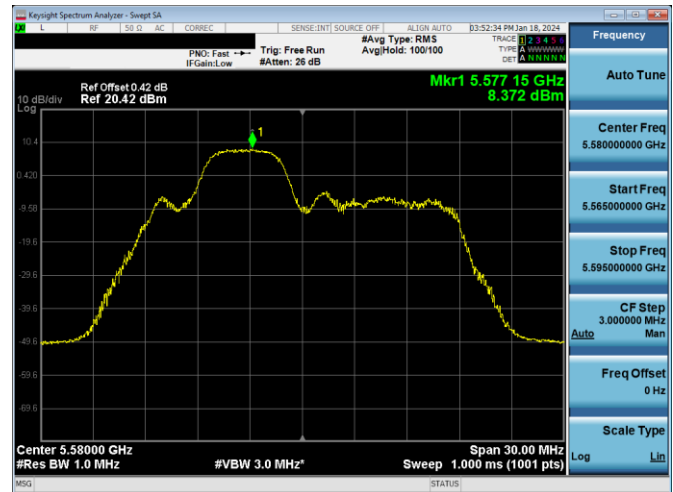
Plot 7-198. PSD Antenna 3c (20MHz BW 11ax Index 38 – RU52 – Ch.116)
