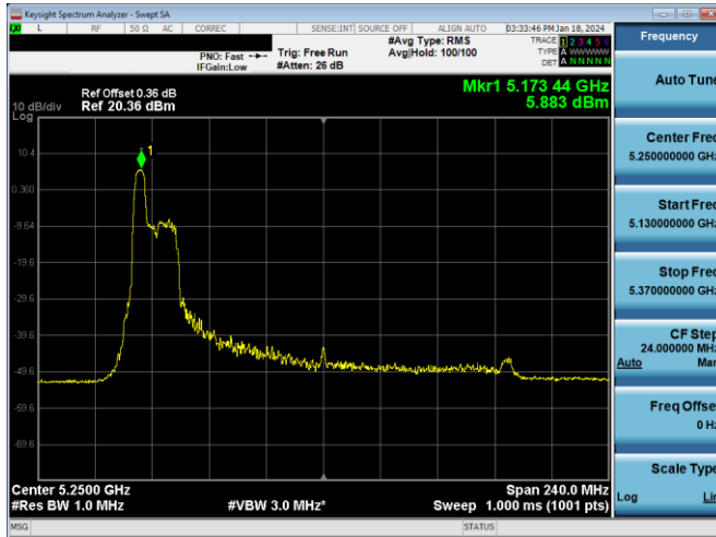
Plot 7-181. PSD Antenna 3c (160MHz BW 11ax Index 37 - RU52 - Ch.50 (L))
