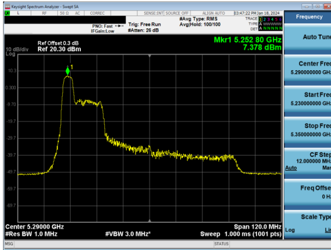
Plot 7-193. PSD Antenna 3c (80MHz BW 11ax Index 37 – RU52 – Ch.58)
