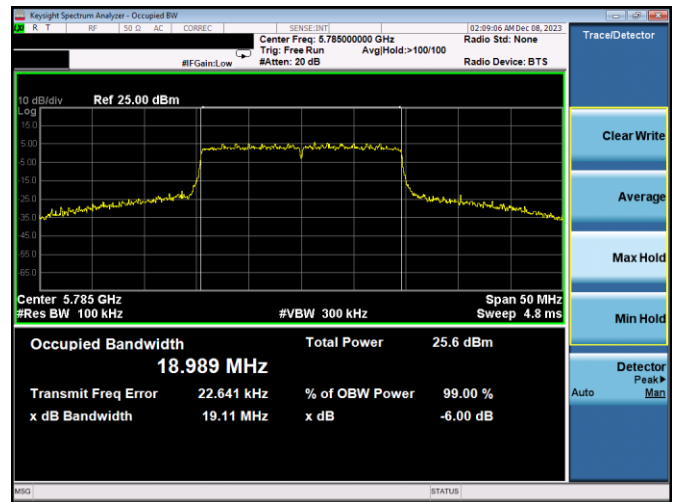
Plot 7-148. 6dB BW & 99% OBW Antenna 3a (20MHz BW 11ax – RU242 – Ch.157)
