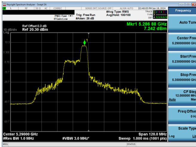
Plot 7-194. PSD Antenna 3c (80MHz BW 11ax Index 44 – RU52 – Ch.58)
