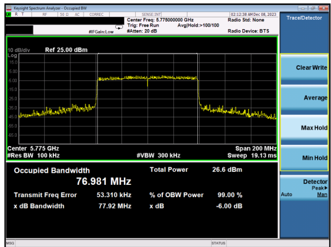
Plot 7-156. 6dB BW & 99% OBW Antenna 1b (80MHz BW 11ax – RU996 – Ch.155)
