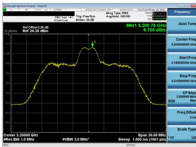
Plot 7-170. PSD Antenna 3c (20MHz BW 11ax Index 4 - RU26 - Ch.40)
