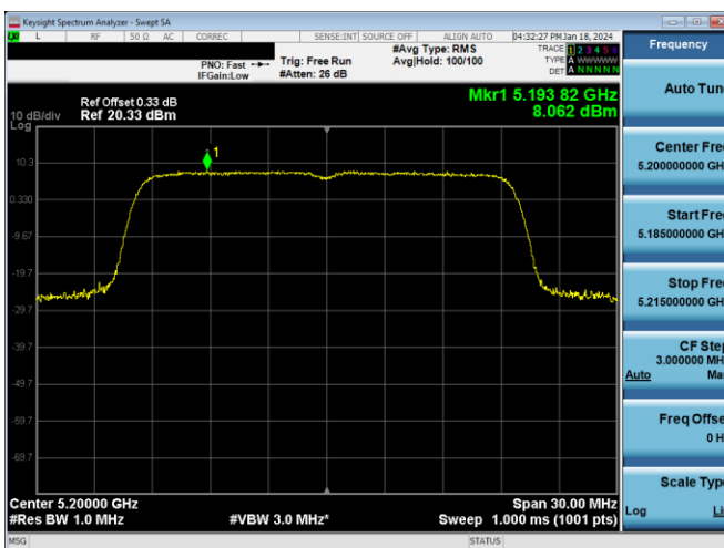
Plot 7-172. PSD Antenna 3c (20MHz BW 11ax- RU242 - Ch.40)
