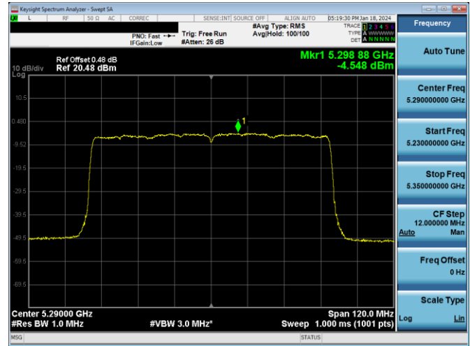
Plot 7-196. PSD Antenna 3c (80MHz BW 11ax – RU96 – Ch.58)
