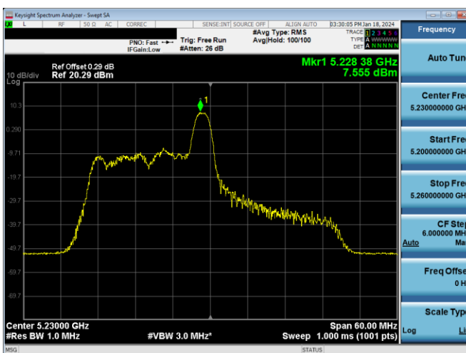
Plot 7-174. PSD Antenna 3c (40MHz BW 11ax Index 8 - RU26 - Ch.46)
