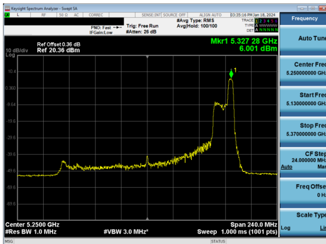
Plot 7-183. PSD Antenna 3c (160MHz BW 11ax Index 52 - RU52 - Ch.50 (U))
