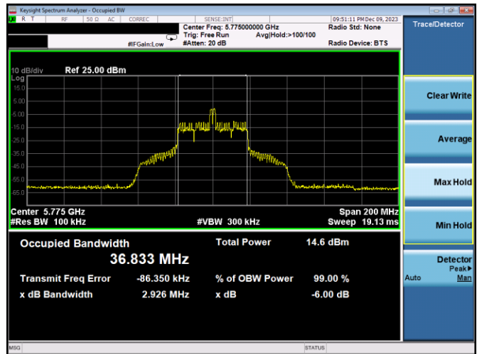
Plot 7-154. 6dB BW & 99% OBW Antenna 3a (80MHz BW 11ax Index 18 – RU26 – Ch.155)
