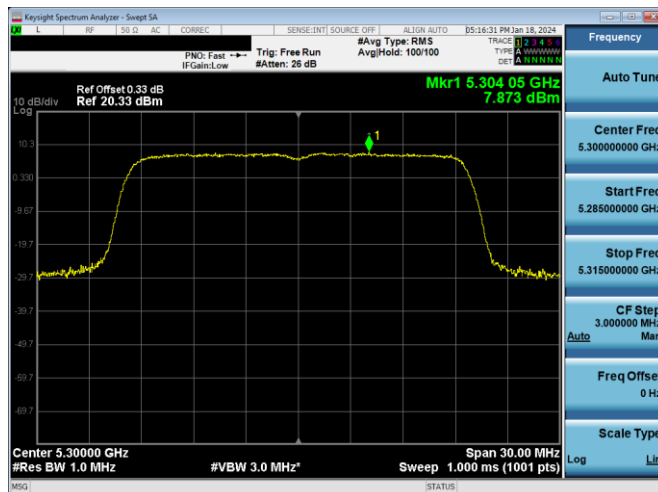
Plot 7-188. PSD Antenna 3c (20MHz BW 11ax- RU242 - Ch.60)
