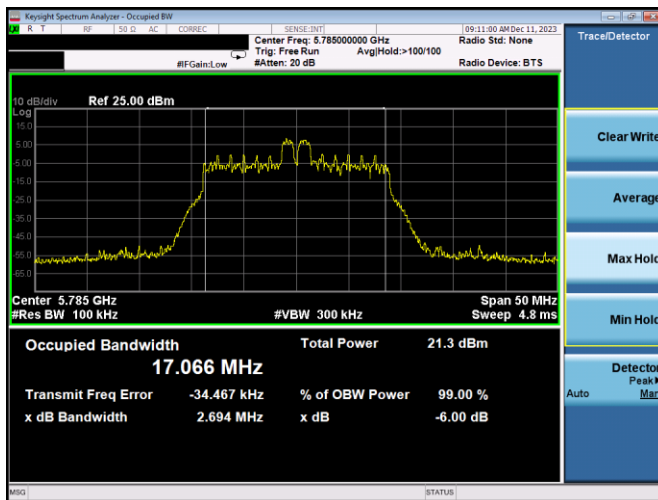
Plot 7-158. 6dB BW & 99% OBW Antenna 1b (20MHz BW 11ax Index 4 – RU26 – Ch.157)
