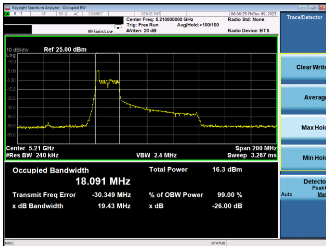
Plot 7-9. 26dB BW & 99% OBW Antenna 3c (80MHz BW 11ax Index 0 – RU26 – Ch.42)
