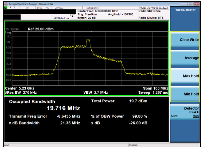
Plot 7-50. 26dB BW & 99% OBW Antenna 3a (40MHz BW 11ax Index 8 - RU26 - Ch.46)
