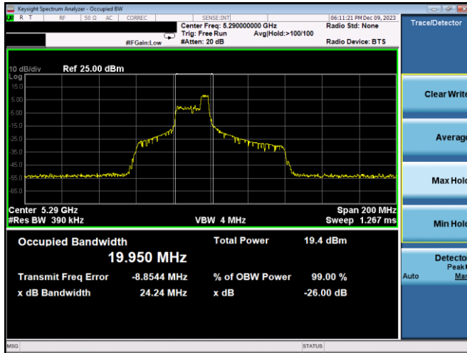
Plot 7-26. 26dB BW & 99% OBW Antenna 3c (80MHz BW 11ax Index 44 - RU52 - Ch.58)
