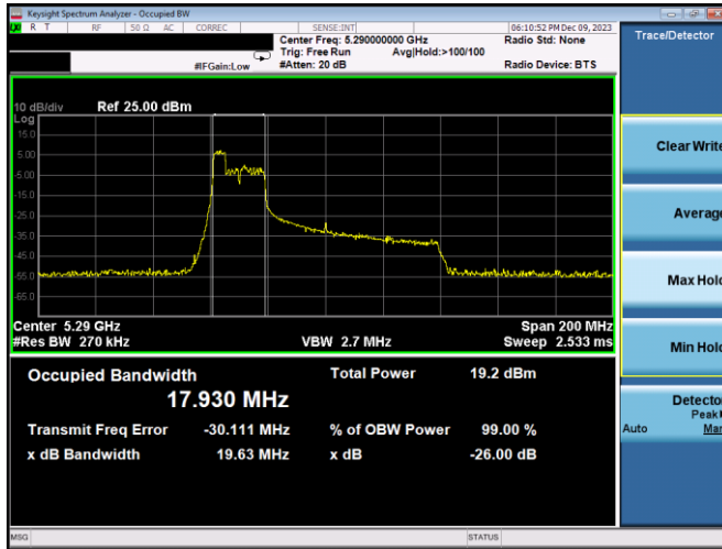
Plot 7-25. 26dB BW & 99% OBW Antenna 3c (80MHz BW 11ax Index 37 - RU52 - Ch.58)
