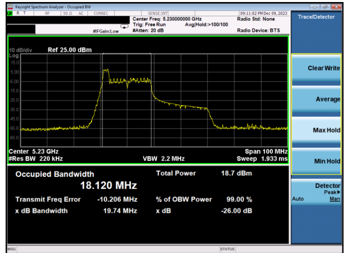
Plot 7-49. 26dB BW & 99% OBW Antenna 3a (40MHz BW 11ax Index 0 - RU26 - Ch.46)
