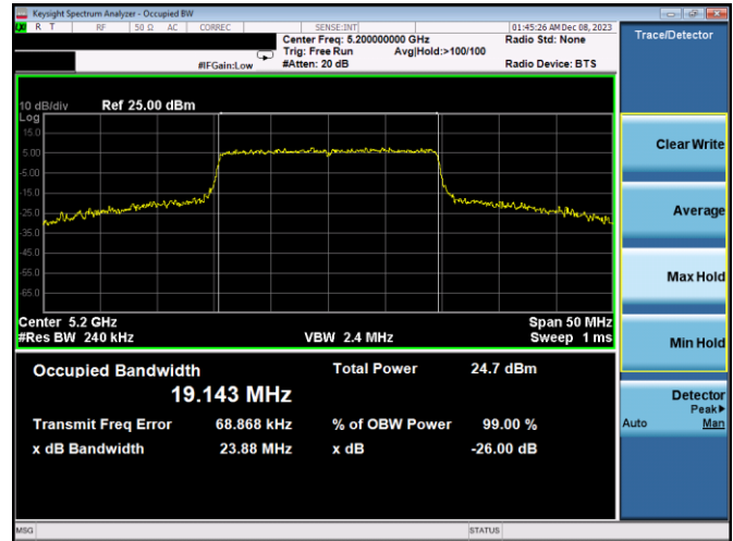
Plot 7-48. 26dB BW & 99% OBW Antenna 3a (20MHz BW 11ax - RU242 - Ch.40)
