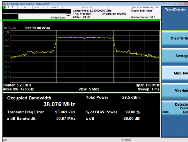
Plot 7-8. 26dB BW & 99% OBW Antenna 3c (40MHz BW 11ax – RU484 – Ch.46)
