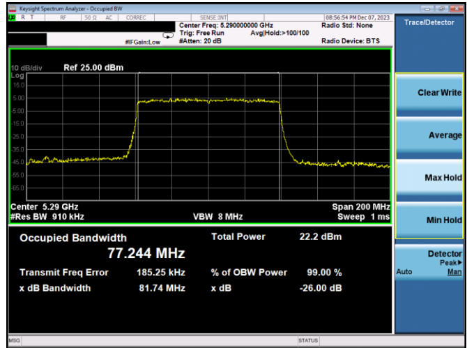
Plot 7-28. 26dB BW & 99% OBW Antenna 3c (80MHz BW 11ax - RU96 - Ch.58)
