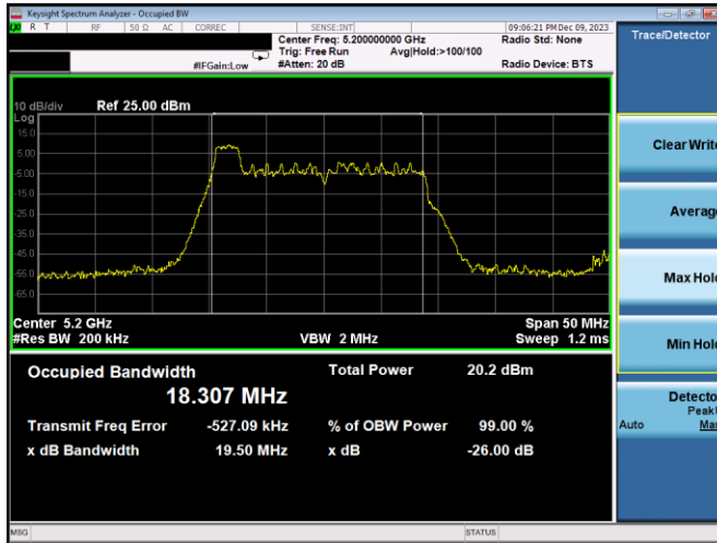
Plot 7-45. 26dB BW & 99% OBW Antenna 3a (20MHz BW 11ax Index 0 - RU26 - Ch.40)
