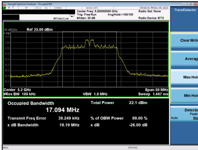
Plot 7-46. 26dB BW & 99% OBW Antenna 3a (20MHz BW 11ax Index 4 - RU26 - Ch.40)
