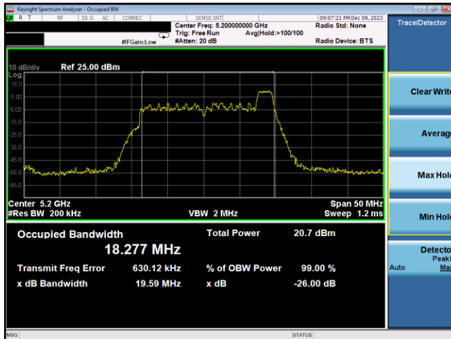
Plot 7-47. 26dB BW & 99% OBW Antenna 3a (20MHz BW 11ax Index 8 - RU26 - Ch.40)
