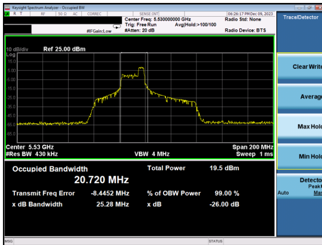
Plot 7-38. 26dB BW & 99% OBW Antenna 3c (80MHz BW 11ax Index 44 – RU52 – Ch.106)
