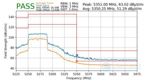
Plot 7-1569. Antenna 1b (Pk & Avg, Ch.54, 802.11ax(SU), MCS11)
