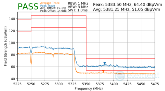
Plot 7-1436. Antenna 3a (Pk & Avg, Ch.50, 802.11ac, MCS4)
