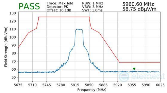
Plot 7-1489. Antenna 1b (Pk, Ch.165, 802.11n, MCS7)
