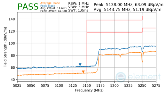
Plot 7-1432. Antenna 3a (Pk & Avg, Ch.50, 802.11ac, MCS2)
