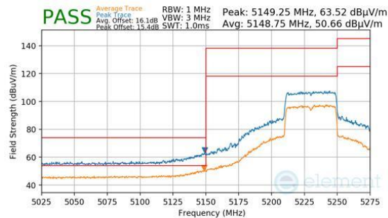
Plot 7-1566. Antenna 1b (Pk & Avg, Ch.46, 802.11ax(SU), MCS11)
