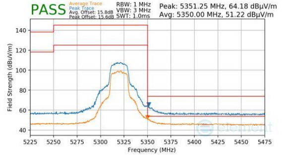
Plot 7-1465. Antenna 1b (Pk & Avg, Ch.64, 802.11n, MCS2)
