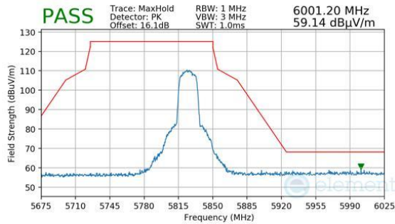
Plot 7-1487. Antenna 1b (Pk, Ch.165, 802.11n, MCS2)
