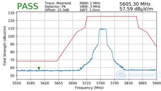
Plot 7-1486. Antenna 1b (Pk, Ch.153, 802.11n, MCS7)
