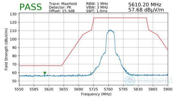
Plot 7-1484. Antenna 1b (Pk, Ch.153, 802.11n, MCS2)
