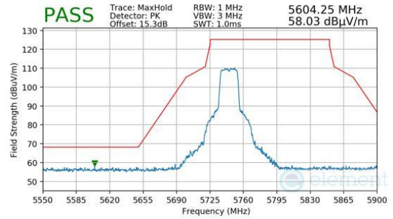
Plot 7-1483. Antenna 1b (Pk, Ch.149, 802.11n, MCS7)
