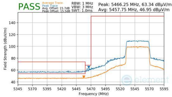
Plot 7-1576. Antenna 1b (Pk & Avg, Ch.110, 802.11ax(SU), MCS2)
