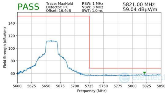
Plot 7-1512. Antenna 1b (Pk, Ch.132, 802.11ax(SU), MCS11)
