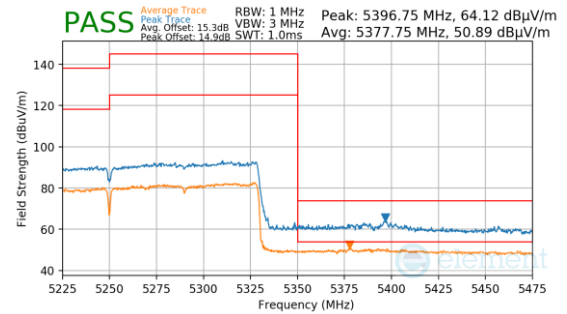
Plot 7-1448. Antenna 3a (Pk & Avg, Ch.50, 802.11ax(SU), MCS4)
