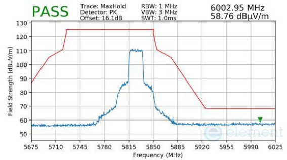
Plot 7-1526. Antenna 1b (Pk, Ch.165, 802.11ax(SU), MCS4)
