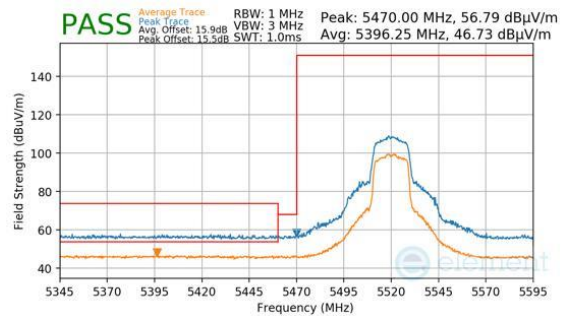
Plot 7-1472. Antenna 1b (Pk & Avg, Ch.104, 802.11n, MCS4)
