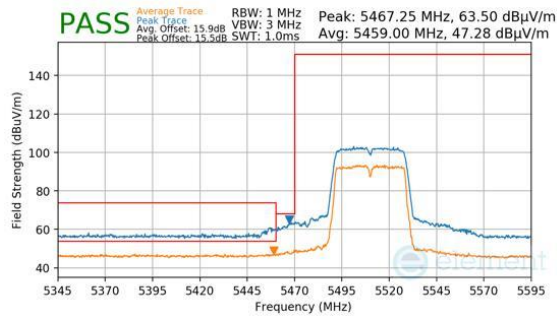
Plot 7-1542. Antenna 1b (Pk & Avg, Ch.102, 802.11n, MCS7)
