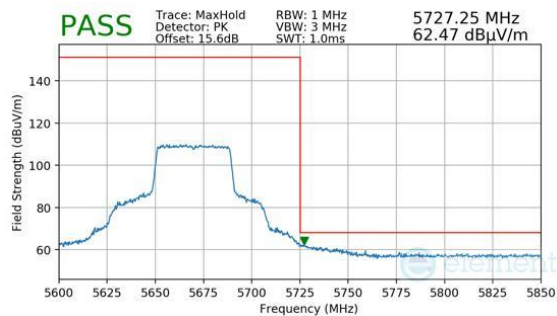
Plot 7-1584. Antenna 1b (Pk, Ch.134, 802.11ax(SU), MCS2)
