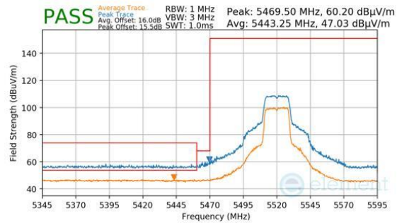
Plot 7-1473. Antenna 1b (Pk & Avg, Ch.104, 802.11n, MCS7)
