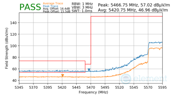
Plot 7-1581. Antenna 1b (Pk & Avg, Ch.118, 802.11ax(SU), MCS11)
