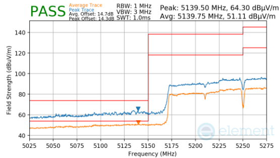
Plot 7-1433. Antenna 3a (Pk & Avg, Ch.50, 802.11ac, MCS4)
