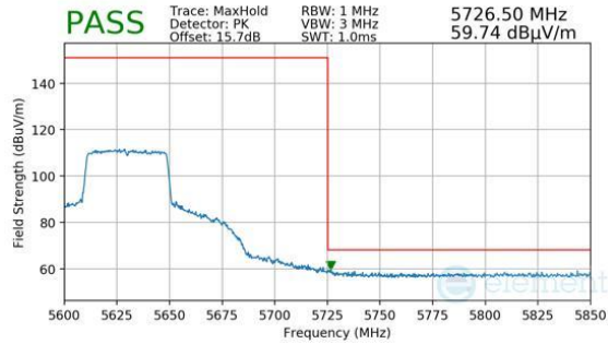
Plot 7-1582. Antenna 1b (Pk, Ch.126, 802.11ax(SU), MCS4)
