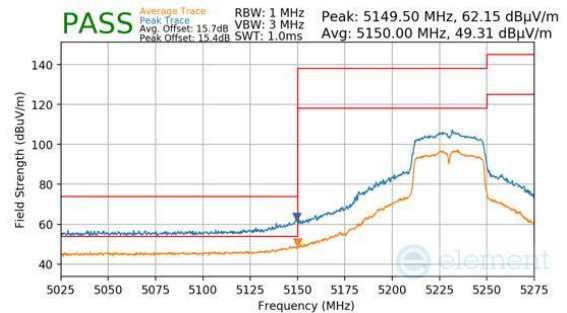
Plot 7-1532. Antenna 1b (Pk & Avg, Ch.46, 802.11n, MCS4)
