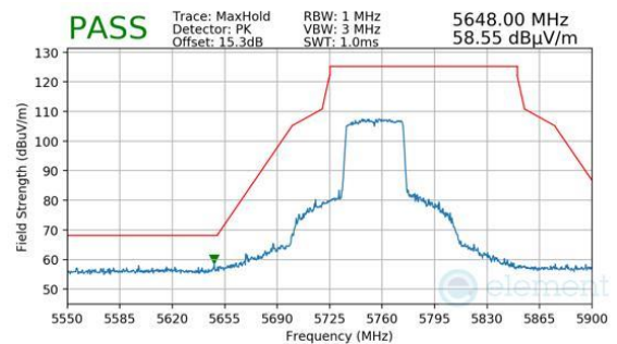
Plot 7-1587. Antenna 1b (Pk, Ch.151, 802.11ax(SU), MCS2)
