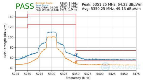
Plot 7-1497. Antenna 1b (Pk & Avg, Ch.60, 802.11ax(SU), MCS4)
