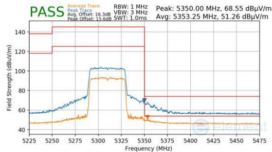
Plot 7-1572. Antenna 1b (Pk & Avg, Ch.62, 802.11ax(SU), MCS11)
