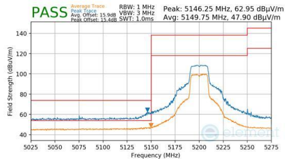
Plot 7-1461. Antenna 1b (Pk & Avg, Ch.40, 802.11n, MCS7)
