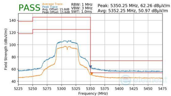
Plot 7-1537. Antenna 1b (Pk & Avg, Ch.62, 802.11n, MCS2)
