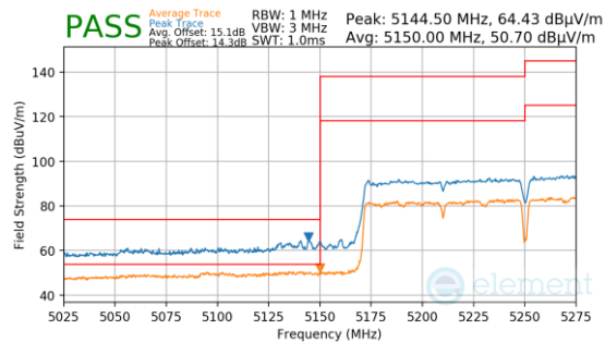
Plot 7-1434. Antenna 3a (Pk & Avg, Ch.50, 802.11ac, MCS9)
