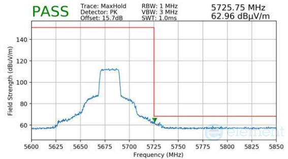
Plot 7-1514. Antenna 1b (Pk, Ch.136, 802.11ax(SU), MCS4)
