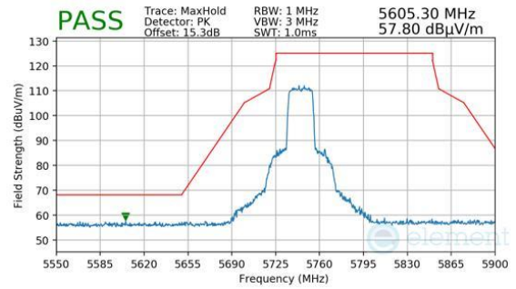
Plot 7-1520. Antenna 1b (Pk, Ch.149, 802.11ax(SU), MCS4)
