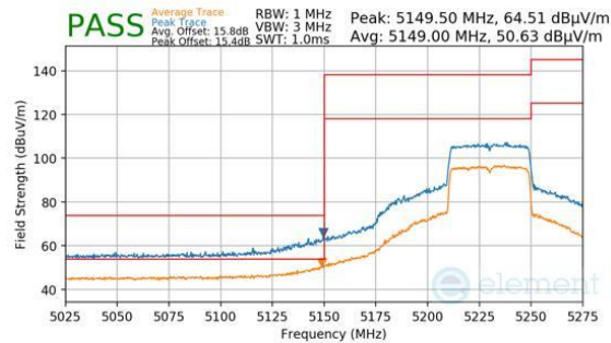
Plot 7-1565. Antenna 1b (Pk & Avg, Ch.46, 802.11ax(SU), MCS4)
