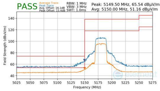
Plot 7-1492. Antenna 1b (Pk & Avg, Ch.36, 802.11ax(SU), MCS11)
