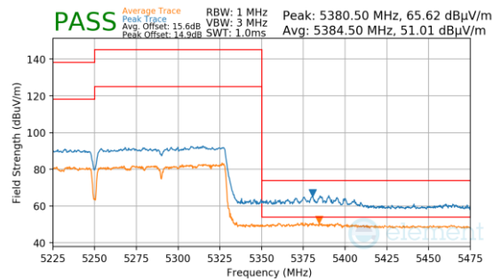
Plot 7-1437. Antenna 3a (Pk & Avg, Ch.50, 802.11ac, MCS9)
