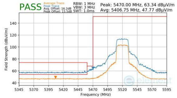
Plot 7-1507. Antenna 1b (Pk & Avg, Ch.104, 802.11ax(SU), MCS11)
