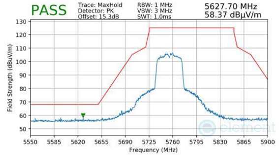
Plot 7-1555. Antenna 1b (Pk, Ch.151, 802.11n, MCS2)
