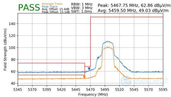
Plot 7-1469. Antenna 1b (Pk & Avg, Ch.100, 802.11n, MCS4)
