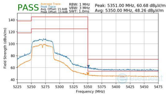
Plot 7-1534. Antenna 1b (Pk & Avg, Ch.54, 802.11n, MCS2)
