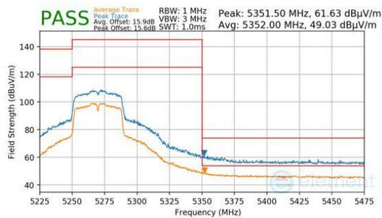
Plot 7-1535. Antenna 1b (Pk & Avg, Ch.54, 802.11n, MCS4)
