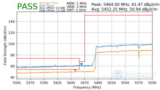
Plot 7-1451. Antenna 3a (Pk & Avg, Ch.114, 802.11ax(SU), MCS4)
