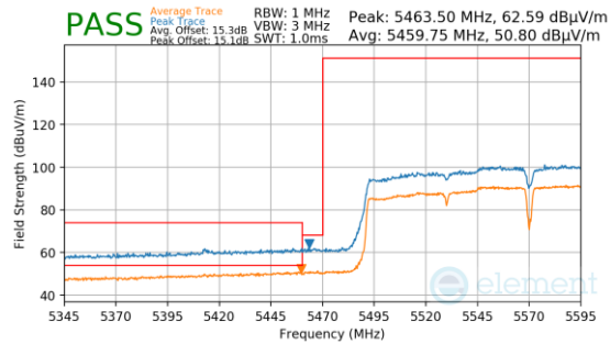
Plot 7-1438. Antenna 3a (Pk & Avg, Ch.114, 802.11ac, MCS2)
