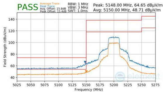
Plot 7-1494. Antenna 1b (Pk & Avg, Ch.40, 802.11ax(SU), MCS4)
