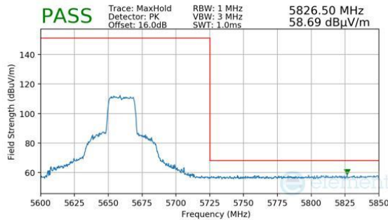
Plot 7-1511. Antenna 1b (Pk, Ch.132, 802.11ax(SU), MCS4)
