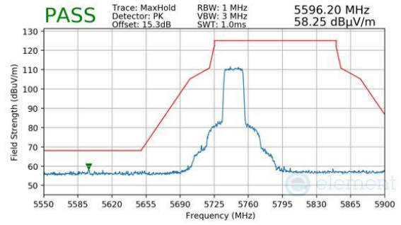
Plot 7-1519. Antenna 1b (Pk, Ch.149, 802.11ax(SU), MCS2)
