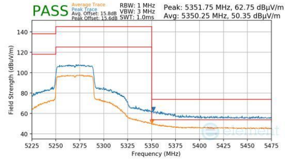
Plot 7-1567. Antenna 1b (Pk & Avg, Ch.54, 802.11ax(SU), MCS2)
