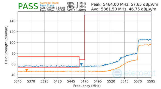
Plot 7-1579. Antenna 1b (Pk & Avg, Ch.118, 802.11ax(SU), MCS2)
