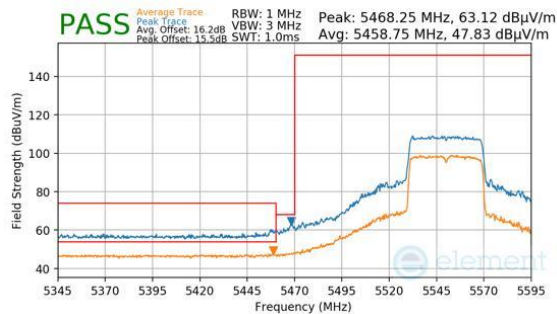
Plot 7-1578. Antenna 1b (Pk & Avg, Ch.110, 802.11ax(SU), MCS11)
