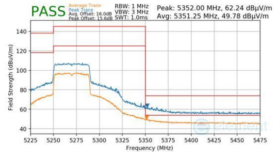
Plot 7-1568. Antenna 1b (Pk & Avg, Ch.54, 802.11ax(SU), MCS4)
