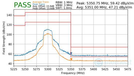
Plot 7-1463. Antenna 1b (Pk & Avg, Ch.60, 802.11n, MCS4)
