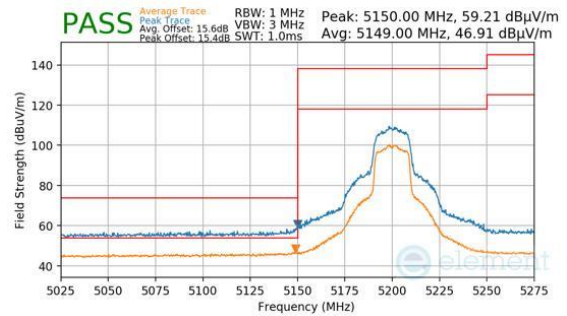
Plot 7-1459. Antenna 1b (Pk & Avg, Ch.40, 802.11n, MCS2)
