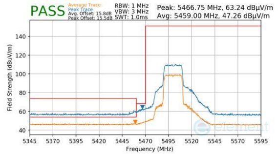
Plot 7-1503. Antenna 1b (Pk & Avg, Ch.100, 802.11ax(SU), MCS4)
