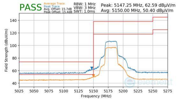
Plot 7-1490. Antenna 1b (Pk & Avg, Ch.36, 802.11ax(SU), MCS2)
