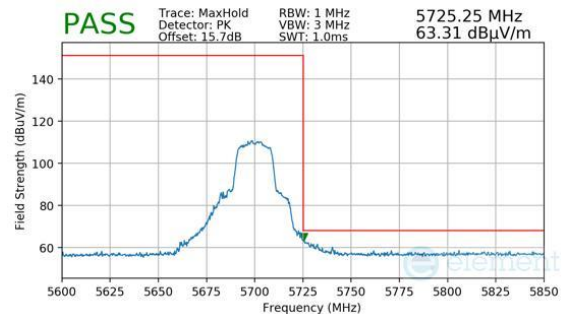
Plot 7-1479. Antenna 1b (Pk, Ch.140, 802.11n, MCS4)
