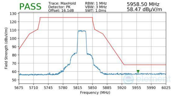
Plot 7-1525. Antenna 1b (Pk, Ch.165, 802.11ax(SU), MCS2)
