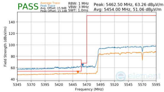
Plot 7-1452. Antenna 3a (Pk & Avg, Ch.114, 802.11ax(SU), MCS11)
