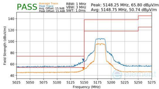
Plot 7-1458. Antenna 1b (Pk & Avg, Ch.36, 802.11n, MCS7)
