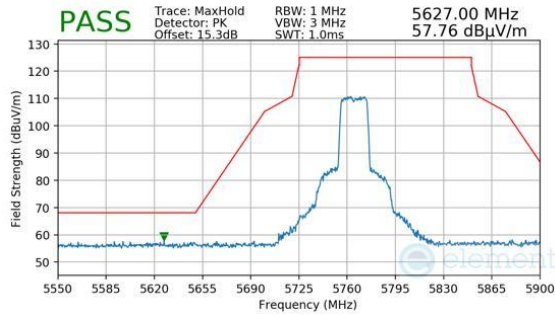
Plot 7-1522. Antenna 1b (Pk, Ch.153, 802.11ax(SU), MCS2)
