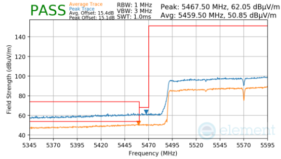
Plot 7-1450. Antenna 3a (Pk & Avg, Ch.114, 802.11ax(SU), MCS2)
