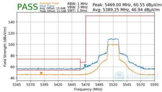
Plot 7-1505. Antenna 1b (Pk & Avg, Ch.104, 802.11ax(SU), MCS2)
