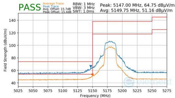
Plot 7-1457. Antenna 1b (Pk & Avg, Ch.36, 802.11n, MCS4)
