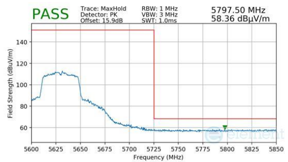
Plot 7-1550. Antenna 1b (Pk, Ch.126, 802.11n, MCS4)
