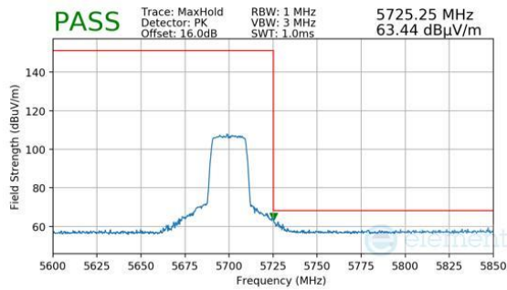
Plot 7-1518. Antenna 1b (Pk, Ch.140, 802.11ax(SU), MCS11)
