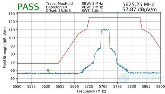
Plot 7-1523. Antenna 1b (Pk, Ch.153, 802.11ax(SU), MCS4)
