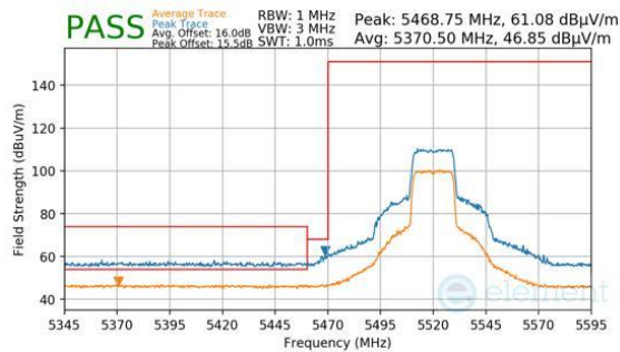
Plot 7-1506. Antenna 1b (Pk & Avg, Ch.104, 802.11ax(SU), MCS4)
