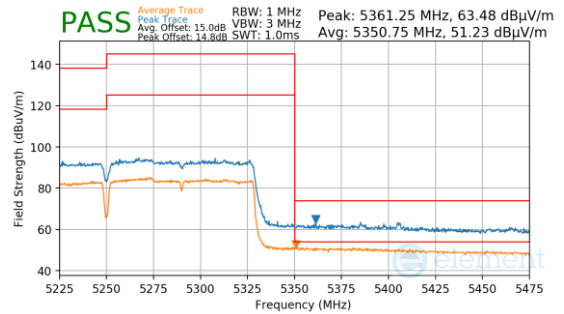
Plot 7-1435. Antenna 3a (Pk & Avg, Ch.50, 802.11ac, MCS2)
