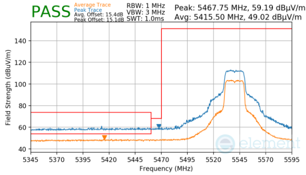
Plot 7-1474. Antenna 1b (Pk & Avg, Ch.108, 802.11n, MCS7)
