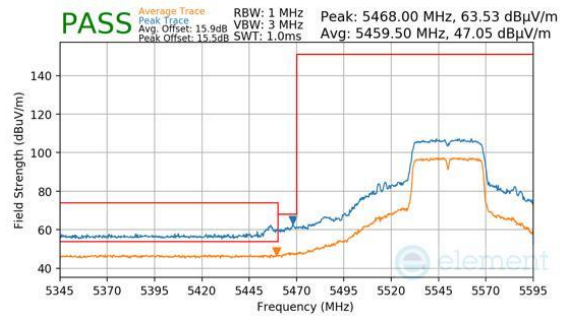
Plot 7-1545. Antenna 1b (Pk & Avg, Ch.110, 802.11n, MCS7)
