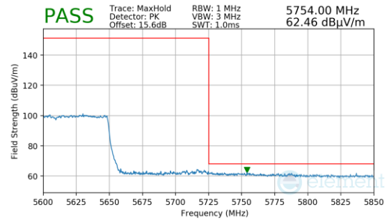
Plot 7-1454. Antenna 3a (Pk, Ch.114, 802.11ax(SU), MCS4)
