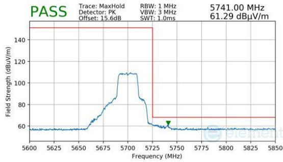
Plot 7-1517. Antenna 1b (Pk, Ch.140, 802.11ax(SU), MCS4)
