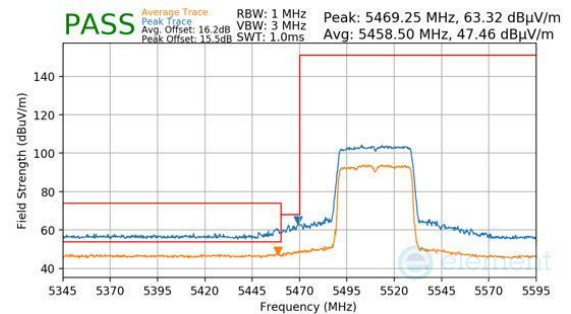
Plot 7-1575. Antenna 1b (Pk & Avg, Ch.102, 802.11ax(SU), MCS11)
