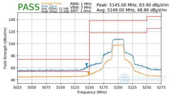
Plot 7-1493. Antenna 1b (Pk & Avg, Ch.40, 802.11ax(SU), MCS2)
