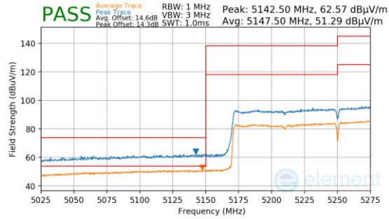
Plot 7-1444. Antenna 3a (Pk & Avg, Ch.50, 802.11ax(SU), MCS2)
