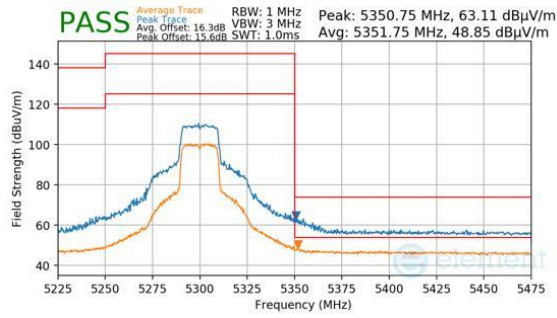
Plot 7-1498. Antenna 1b (Pk & Avg, Ch.60, 802.11ax(SU), MCS11)
