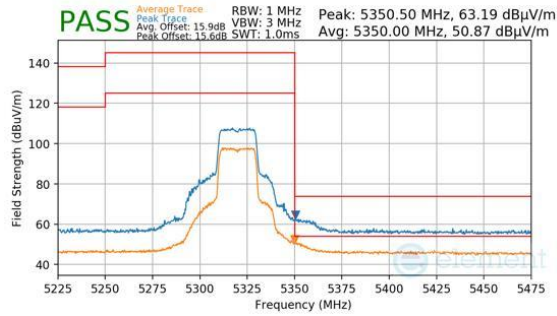
Plot 7-1499. Antenna 1b (Pk & Avg, Ch.64, 802.11ax(SU), MCS2)
