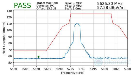
Plot 7-1481. Antenna 1b (Pk, Ch.149, 802.11n, MCS2)
