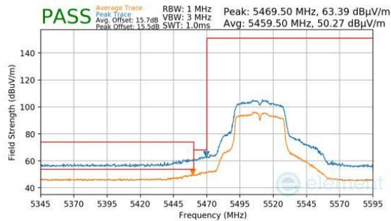
Plot 7-1540. Antenna 1b (Pk & Avg, Ch.102, 802.11n, MCS2)
