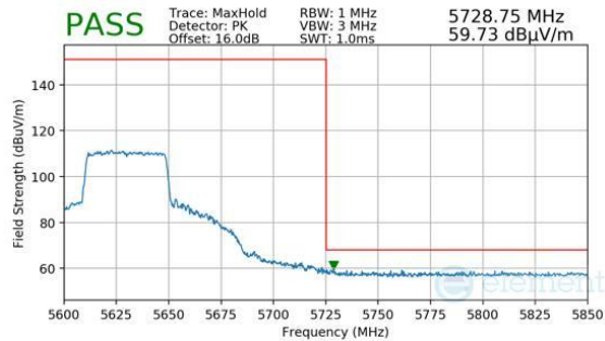
Plot 7-1583. Antenna 1b (Pk, Ch.126, 802.11ax(SU), MCS11)
