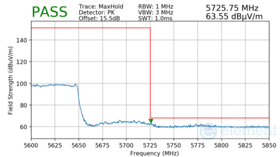
Plot 7-1455. Antenna 3a (Pk, Ch.114, 802.11ax(SU), MCS11)
