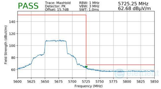
Plot 7-1585. Antenna 1b (Pk, Ch.134, 802.11ax(SU), MCS4)
