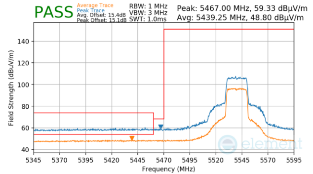
Plot 7-1509. Antenna 1b (Pk & Avg, Ch.108, 802.11ax(SU), MCS4)
