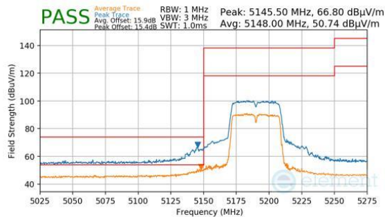
Plot 7-1530. Antenna 1b (Pk & Avg, Ch.38, 802.11n, MCS7)
