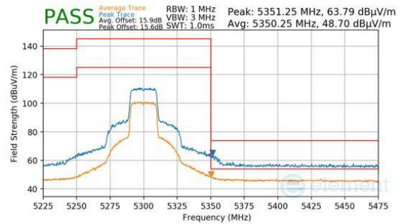
Plot 7-1496. Antenna 1b (Pk & Avg, Ch.60, 802.11ax(SU), MCS2)
