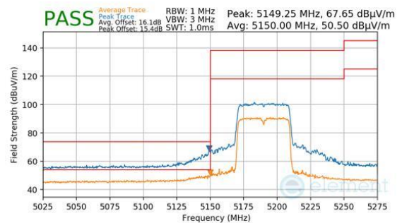
Plot 7-1563. Antenna 1b (Pk & Avg, Ch.38, 802.11ax(SU), MCS11)
