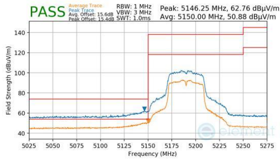
Plot 7-1528. Antenna 1b (Pk & Avg, Ch.38, 802.11n, MCS2)
