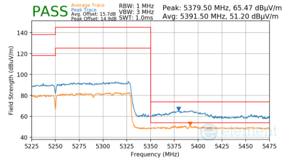
Plot 7-1449. Antenna 3a (Pk & Avg, Ch.50, 802.11ax(SU), MCS11)
