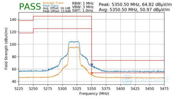
Plot 7-1467. Antenna 1b (Pk & Avg, Ch.64, 802.11n, MCS7)
