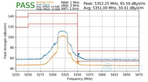
Plot 7-1466. Antenna 1b (Pk & Avg, Ch.64, 802.11n, MCS4)
