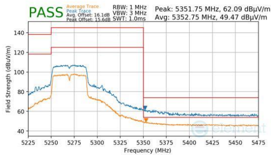
Plot 7-1536. Antenna 1b (Pk & Avg, Ch.54, 802.11n, MCS7)
