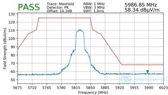
Plot 7-1488. Antenna 1b (Pk, Ch.165, 802.11n, MCS4)
