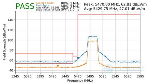
Plot 7-1470. Antenna 1b (Pk & Avg, Ch.100, 802.11n, MCS7)
