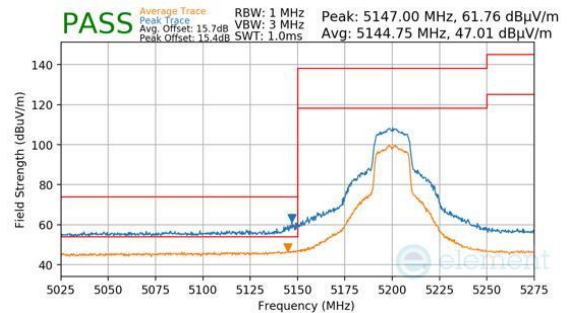
Plot 7-1460. Antenna 1b (Pk & Avg, Ch.40, 802.11n, MCS4)
