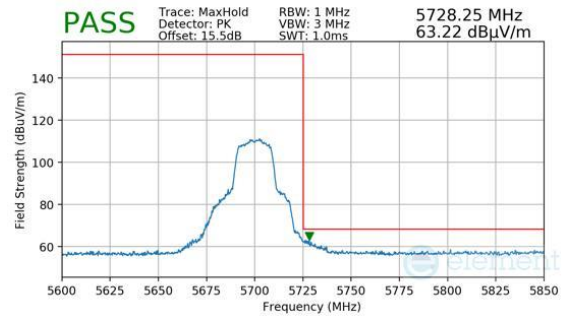
Plot 7-1478. Antenna 1b (Pk, Ch.140, 802.11n, MCS2)
