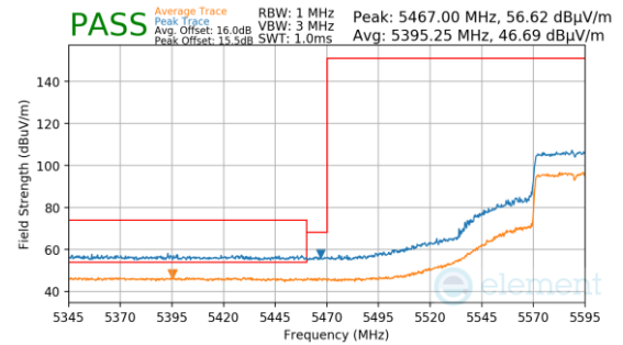
Plot 7-1580. Antenna 1b (Pk & Avg, Ch.118, 802.11ax(SU), MCS4)
