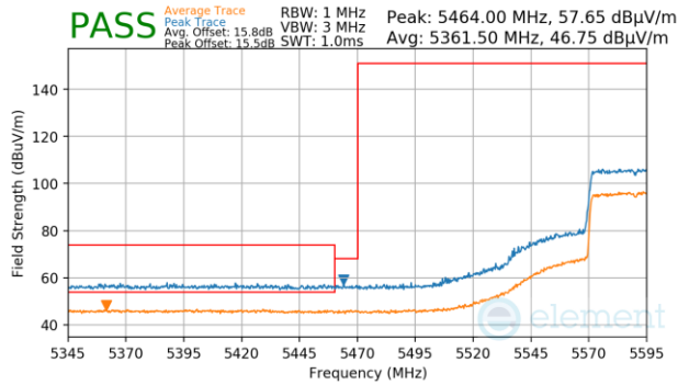
Plot 7-1546. Antenna 1b (Pk & Avg, Ch.118, 802.11n, MCS2)
