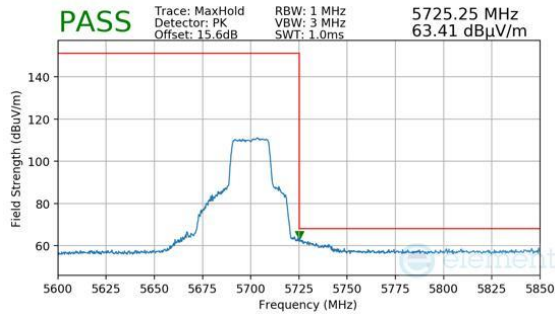
Plot 7-1516. Antenna 1b (Pk, Ch.140, 802.11ax(SU), MCS2)
