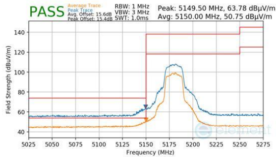
Plot 7-1456. Antenna 1b (Pk & Avg, Ch.36, 802.11n, MCS2)
