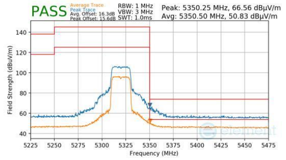
Plot 7-1501. Antenna 1b (Pk & Avg, Ch.64, 802.11ax(SU), MCS11)
