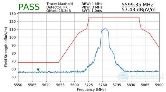
Plot 7-1485. Antenna 1b (Pk, Ch.153, 802.11n, MCS4)
