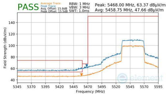
Plot 7-1577. Antenna 1b (Pk & Avg, Ch.110, 802.11ax(SU), MCS4)
