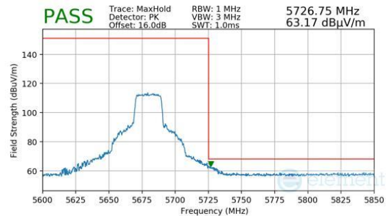
Plot 7-1515. Antenna 1b (Pk, Ch.136, 802.11ax(SU), MCS11)
