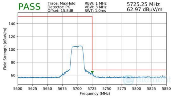
Plot 7-1480. Antenna 1b (Pk, Ch.140, 802.11n, MCS7)
