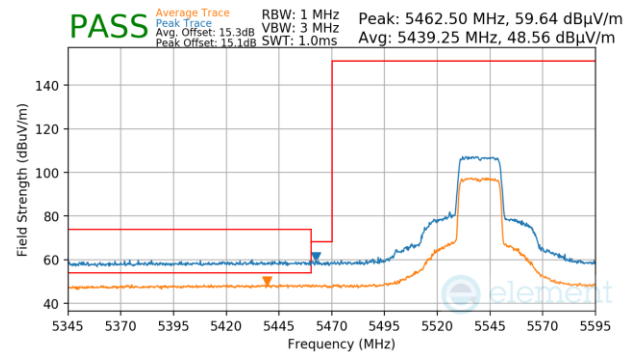
Plot 7-1508. Antenna 1b (Pk & Avg, Ch.108, 802.11ax(SU), MCS2)
