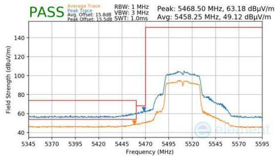
Plot 7-1541. Antenna 1b (Pk & Avg, Ch.102, 802.11n, MCS4)
