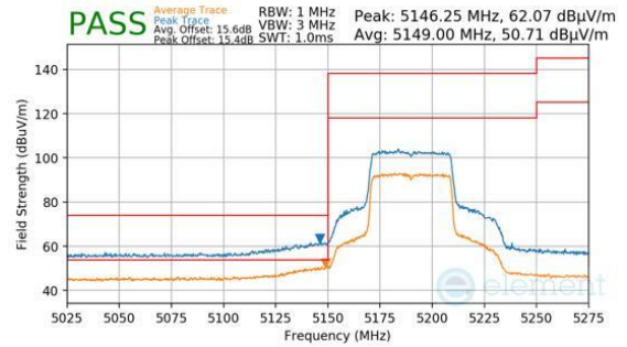
Plot 7-1561. Antenna 1b (Pk & Avg, Ch.38, 802.11ax(SU), MCS2)
