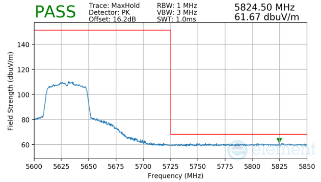
Plot 7-1549. Antenna 1b (Pk, Ch.126, 802.11n, MCS2)
