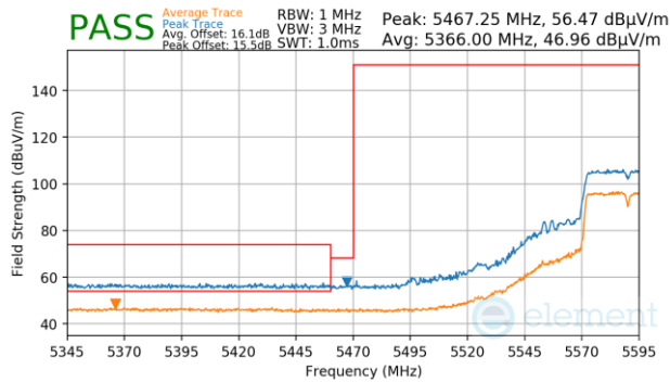
Plot 7-1548. Antenna 1b (Pk & Avg, Ch.118, 802.11n, MCS7)
