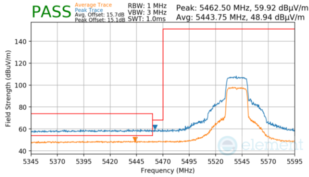
Plot 7-1510. Antenna 1b (Pk & Avg, Ch.108, 802.11ax(SU), MCS11)
