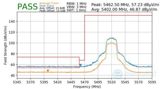
Plot 7-1471. Antenna 1b (Pk & Avg, Ch.104, 802.11n, MCS2)
