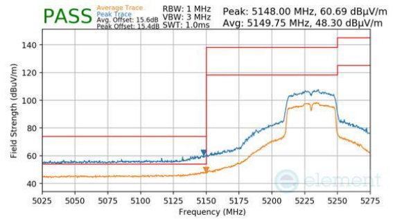
Plot 7-1531. Antenna 1b (Pk & Avg, Ch.46, 802.11n, MCS2)
