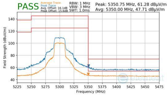
Plot 7-1464. Antenna 1b (Pk & Avg, Ch.60, 802.11n, MCS7)
