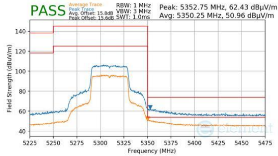
Plot 7-1570. Antenna 1b (Pk & Avg, Ch.62, 802.11ax(SU), MCS2)
