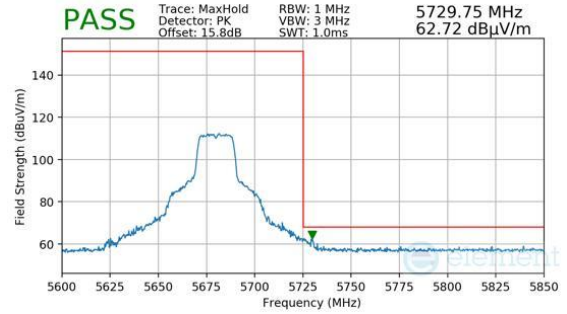
Plot 7-1477. Antenna 1b (Pk, Ch.136, 802.11n, MCS7)
