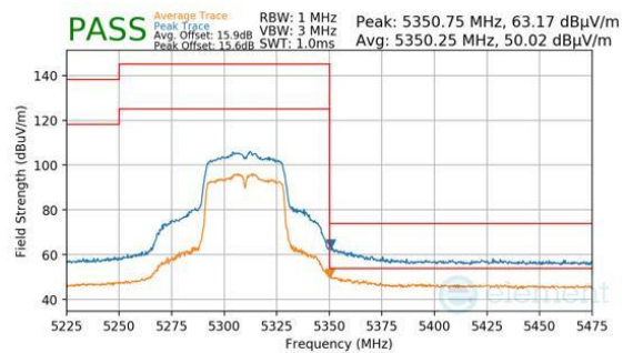
Plot 7-1538. Antenna 1b (Pk & Avg, Ch.62, 802.11n, MCS4)
