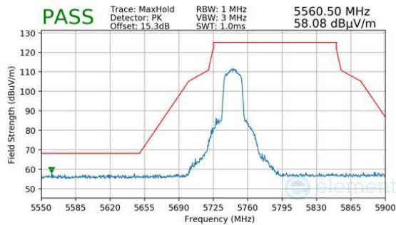
Plot 7-1482. Antenna 1b (Pk, Ch.149, 802.11n, MCS4)
