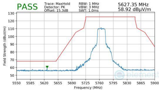
Plot 7-1524. Antenna 1b (Pk, Ch.153, 802.11ax(SU), MCS11)
