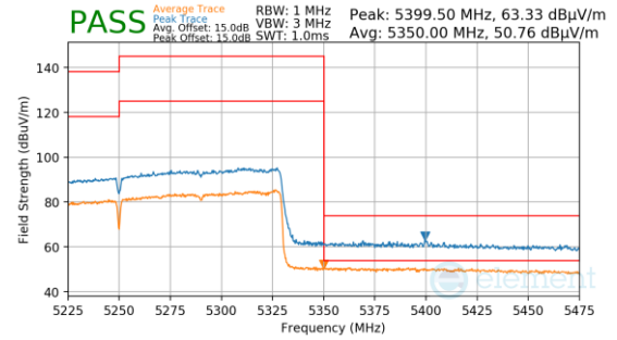
Plot 7-1447. Antenna 3a (Pk & Avg, Ch.50, 802.11ax(SU), MCS2)
