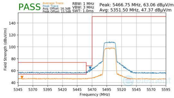
Plot 7-1504. Antenna 1b (Pk & Avg, Ch.100, 802.11ax(SU), MCS11)
