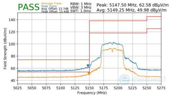
Plot 7-1529. Antenna 1b (Pk & Avg, Ch.38, 802.11n, MCS4)
