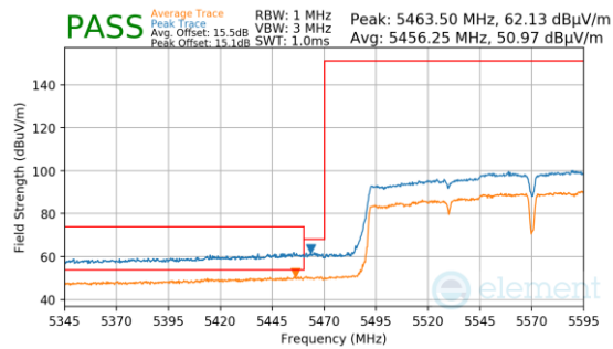
Plot 7-1439. Antenna 3a (Pk & Avg, Ch.114, 802.11ac, MCS4)
