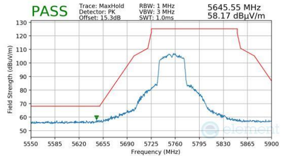
Plot 7-1556. Antenna 1b (Pk, Ch.151, 802.11n, MCS4)
