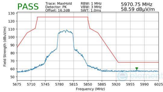
Plot 7-1559. Antenna 1b (Pk, Ch.159, 802.11n, MCS4)
