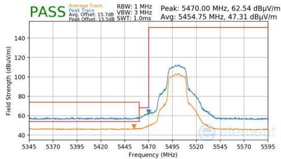
Plot 7-1468. Antenna 1b (Pk & Avg, Ch.100, 802.11n, MCS2)
