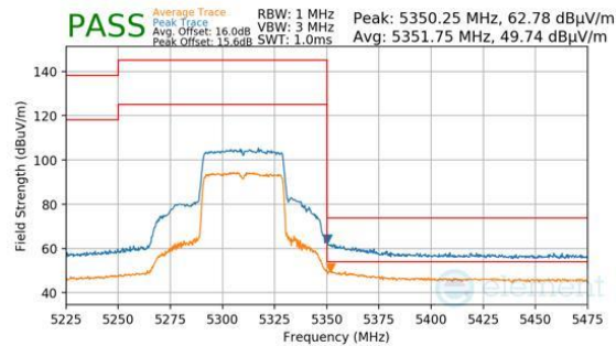
Plot 7-1571. Antenna 1b (Pk & Avg, Ch.62, 802.11ax(SU), MCS4)
