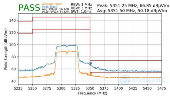
Plot 7-1539. Antenna 1b (Pk & Avg, Ch.62, 802.11n, MCS7)
