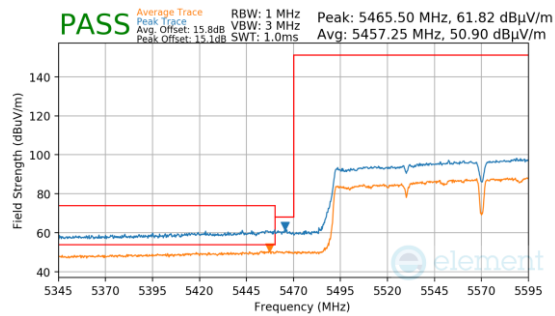
Plot 7-1440. Antenna 3a (Pk & Avg, Ch.114, 802.11ac, MCS9)
