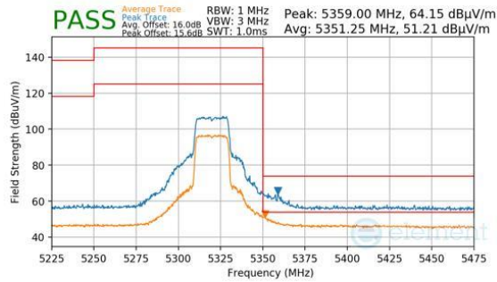
Plot 7-1500. Antenna 1b (Pk & Avg, Ch.64, 802.11ax(SU), MCS4)
