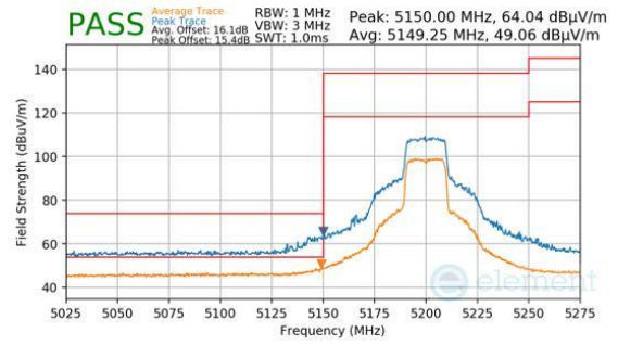
Plot 7-1495. Antenna 1b (Pk & Avg, Ch.40, 802.11ax(SU), MCS11)
