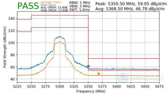
Plot 7-1462. Antenna 1b (Pk & Avg, Ch.60, 802.11n, MCS2)
