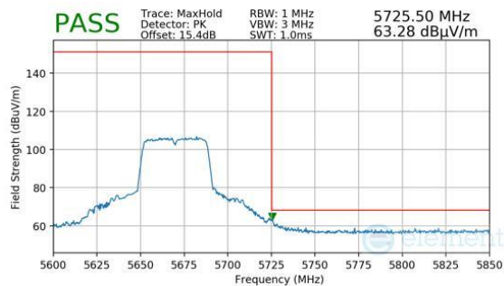
Plot 7-1554. Antenna 1b (Pk, Ch.134, 802.11n, MCS7)
