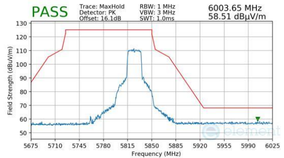
Plot 7-1527. Antenna 1b (Pk, Ch.165, 802.11ax(SU), MCS11)
