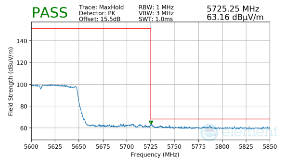
Plot 7-1442. Antenna 3a (Pk, Ch.114, 802.11ac, MCS4)
