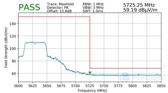
Plot 7-1551. Antenna 1b (Pk, Ch.126, 802.11n, MCS7)
