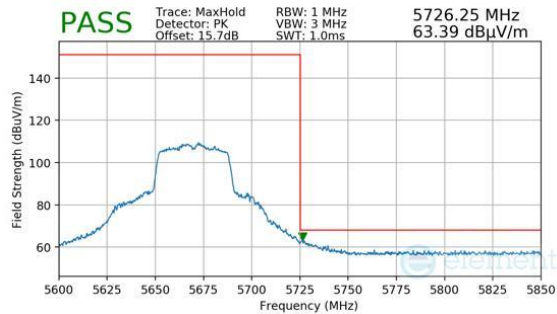
Plot 7-1553. Antenna 1b (Pk, Ch.134, 802.11n, MCS4)
