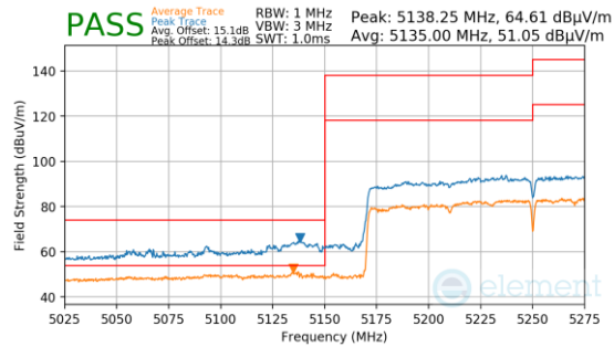
Plot 7-1446. Antenna 3a (Pk & Avg, Ch.50, 802.11ax(SU), MCS11)
