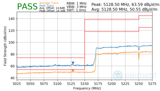
Plot 7-1445. Antenna 3a (Pk & Avg, Ch.50, 802.11ax(SU), MCS4)
