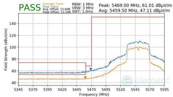
Plot 7-1544. Antenna 1b (Pk & Avg, Ch.110, 802.11n, MCS4)
