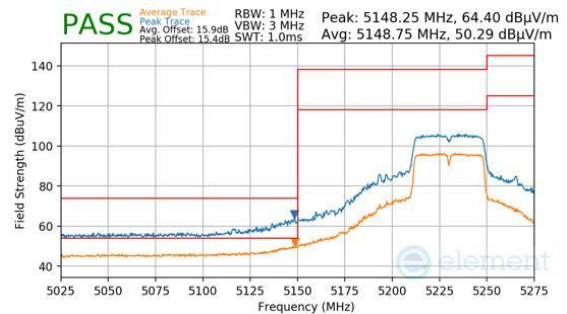
Plot 7-1533. Antenna 1b (Pk & Avg, Ch.46, 802.11n, MCS7)
