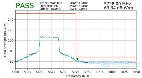
Plot 7-1586. Antenna 1b (Pk, Ch.134, 802.11ax(SU), MCS11)
