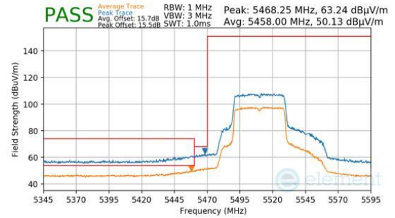
Plot 7-1573. Antenna 1b (Pk & Avg, Ch.102, 802.11ax(SU), MCS2)
