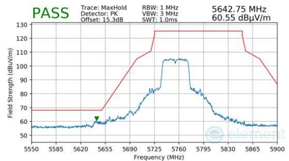
Plot 7-1557. Antenna 1b (Pk, Ch.151, 802.11n, MCS7)
