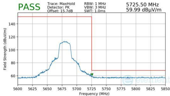
Plot 7-1476. Antenna 1b (Pk, Ch.136, 802.11n, MCS4)
