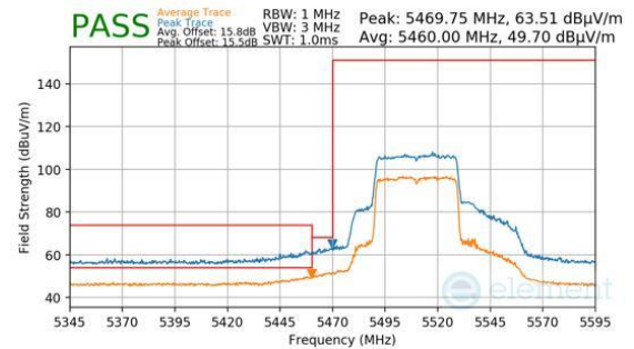
Plot 7-1574. Antenna 1b (Pk & Avg, Ch.102, 802.11ax(SU), MCS4)
