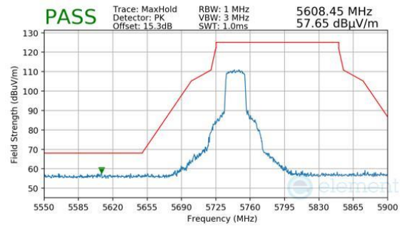
Plot 7-1521. Antenna 1b (Pk, Ch.149, 802.11ax(SU), MCS11)
