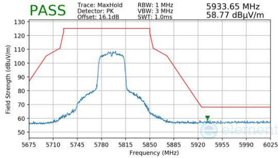
Plot 7-1558. Antenna 1b (Pk, Ch.159, 802.11n, MCS2)
