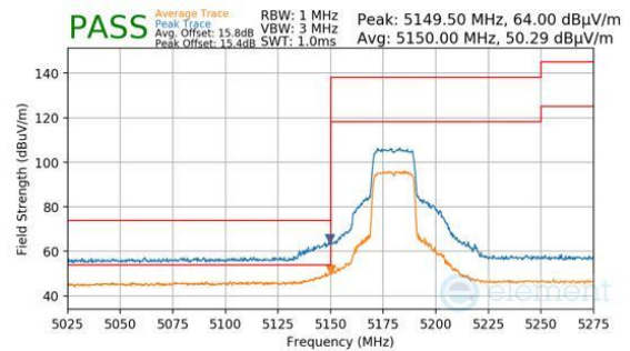
Plot 7-1491. Antenna 1b (Pk & Avg, Ch.36, 802.11ax(SU), MCS4)
