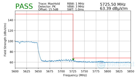
Plot 7-1443. Antenna 3a (Pk, Ch.114, 802.11ac, MCS9)
