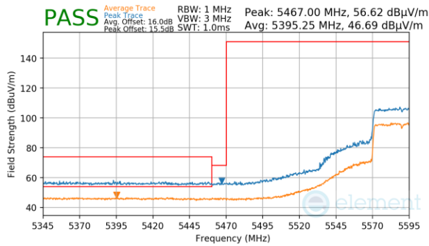
Plot 7-1547. Antenna 1b (Pk & Avg, Ch.118, 802.11n, MCS4)
