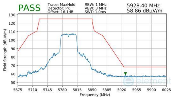
Plot 7-1560. Antenna 1b (Pk, Ch.159, 802.11n, MCS7)
