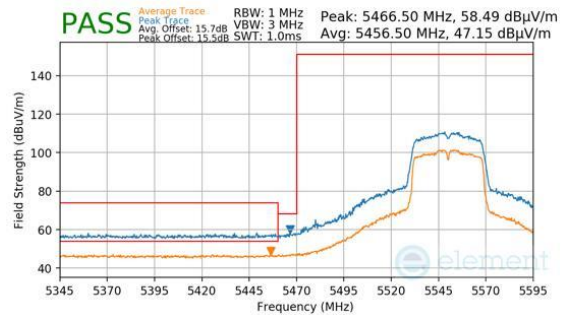
Plot 7-1543. Antenna 1b (Pk & Avg, Ch.110, 802.11n, MCS2)
