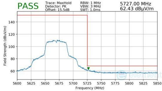
Plot 7-1552. Antenna 1b (Pk, Ch.134, 802.11n, MCS2)
