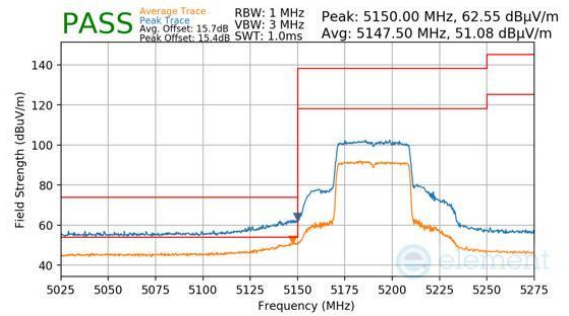
Plot 7-1562. Antenna 1b (Pk & Avg, Ch.38, 802.11ax(SU), MCS4)
