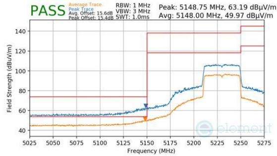
Plot 7-1564. Antenna 1b (Pk & Avg, Ch.46, 802.11ax(SU), MCS2)
