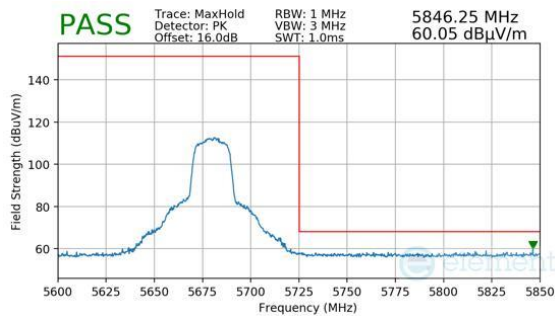
Plot 7-1475. Antenna 1b (Pk, Ch.136, 802.11n, MCS2)
