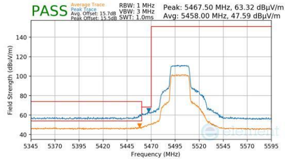
Plot 7-1502. Antenna 1b (Pk & Avg, Ch.100, 802.11ax(SU), MCS2)
