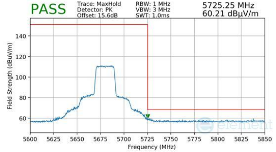
Plot 7-1513. Antenna 1b (Pk, Ch.136, 802.11ax(SU), MCS2)
