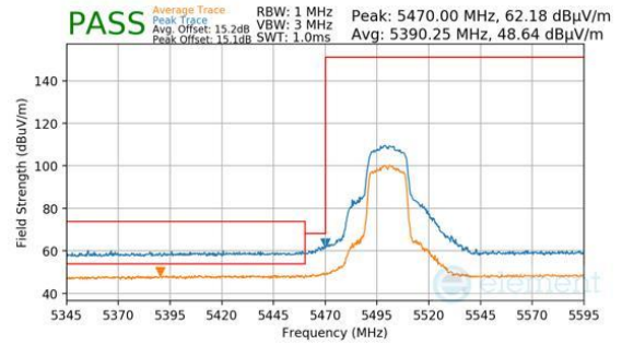
Plot 7-1271. Antenna 3a (Pk & Avg, Ch.100, 802.11n, MCS4)
