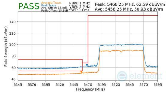
Plot 7-1419. Antenna 3a (pk & avg, ch.106, 802.11ax(su), mcs11)
