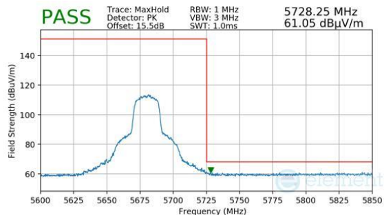
Plot 7-1277. Antenna 3a (Pk, Ch.136, 802.11n, MCS2)
