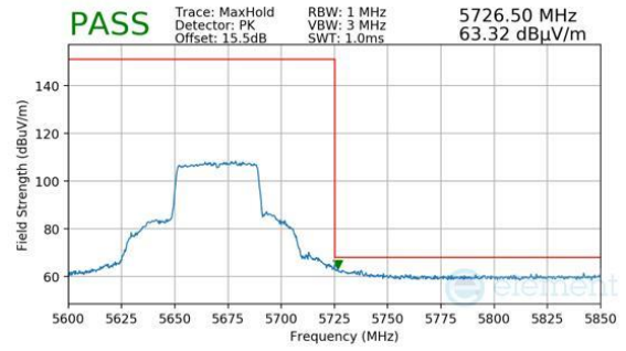
Plot 7-1382. Antenna 3a (Pk, Ch.134, 802.11ax(SU), MCS4)
