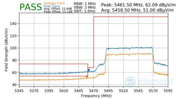
Plot 7-1418. Antenna 3a (pk & avg, ch.106, 802.11ax(su), mcs4)
