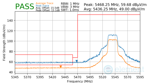
Plot 7-1275. Antenna 3a (Pk & Avg, Ch.108, 802.11n, MCS7)
