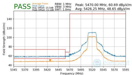
Plot 7-1276. Antenna 3a (Pk & Avg, Ch.104, 802.11n, MCS7)
