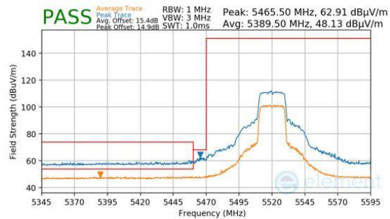
Plot 7-1306. Antenna 3a (Pk & Avg, Ch.104, 802.11ax(SU), MCS11)
