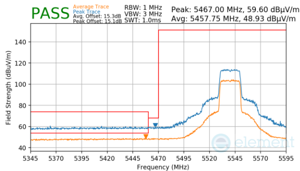
Plot 7-1307. Antenna 3a (Pk & Avg, Ch.108, 802.11ax(SU), MCS2)
