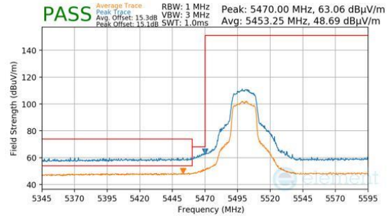
Plot 7-1270. Antenna 3a (Pk & Avg, Ch.100, 802.11n, MCS2)
