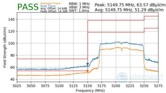
Plot 7-1195. Antenna 3c (Pk & Avg, Ch.42, 802.11ac, MCS4)
