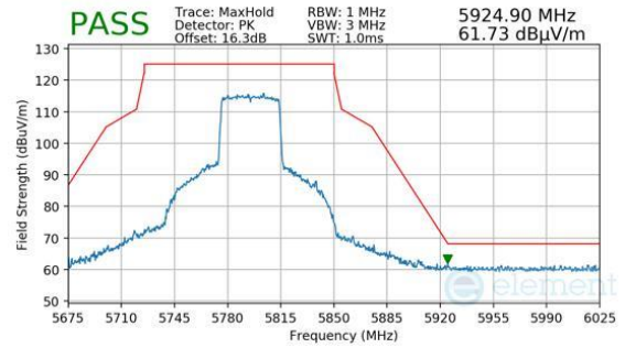
Plot 7-1192. Antenna 3c (Pk, Ch.159, 802.11ax(SU), MCS4)
