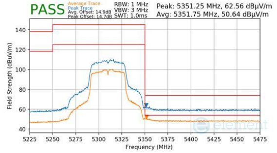
Plot 7-1138. Antenna 3c (Pk & Avg, Ch.62, 802.11n, MCS2)
