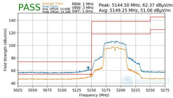
Plot 7-1130. Antenna 3c (Pk & Avg, Ch.38, 802.11n, MCS4)
