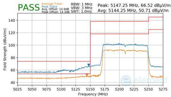
Plot 7-1196. Antenna 3c (Pk & Avg, Ch.42, 802.11ac, MCS9)
