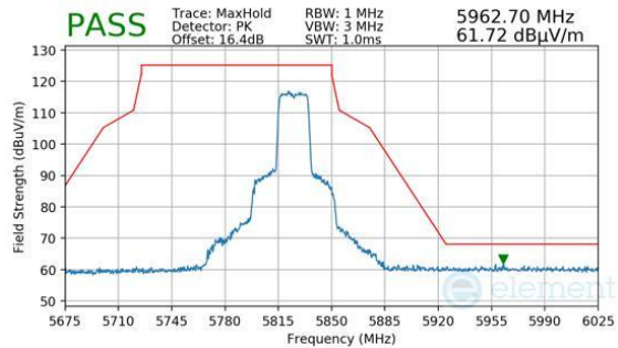
Plot 7-1126. Antenna 3c (Pk, Ch.165, 802.11ax(SU), MCS2)
