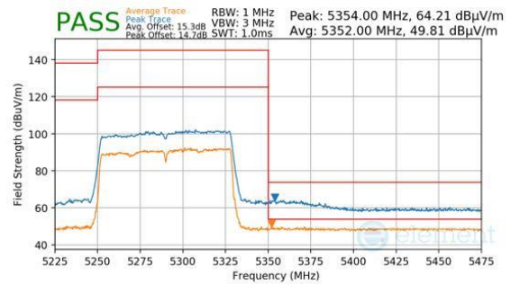
Plot 7-1199. Antenna 3c (Pk & Avg, Ch.58, 802.11ac, MCS9)
