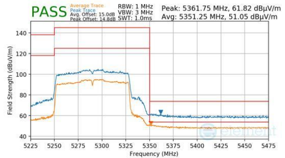
Plot 7-1198. Antenna 3c (Pk & Avg, Ch.58, 802.11ac, MCS4)
