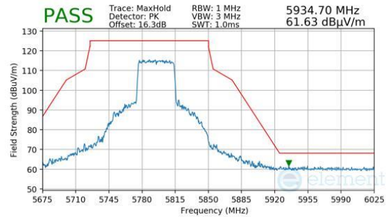
Plot 7-1193. Antenna 3c (Pk, Ch.159, 802.11ax(SU), MCS11)
