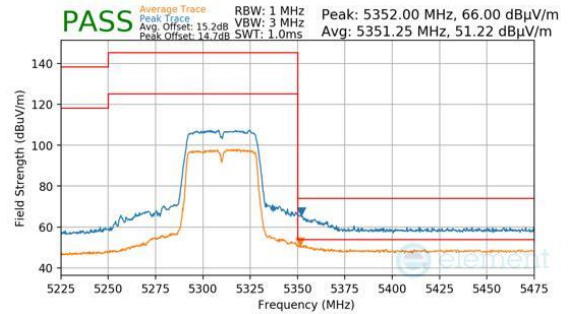
Plot 7-1140. Antenna 3c (Pk & Avg, Ch.62, 802.11n, MCS7)
