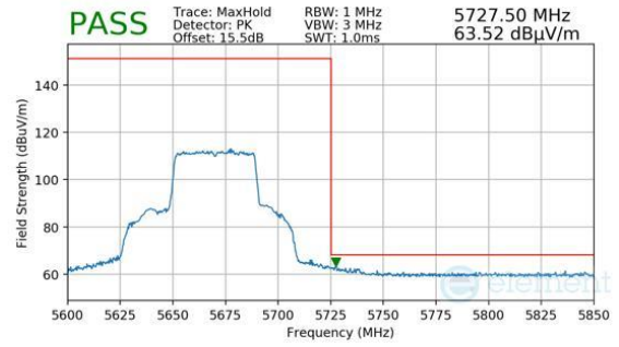
Plot 7-1186. Antenna 3c (Pk, Ch.134, 802.11ax(SU), MCS4)
