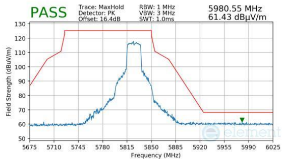
Plot 7-1128. Antenna 3c (Pk, Ch.165, 802.11ax(SU), MCS11)
