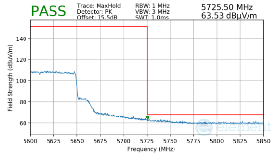
Plot 7-1228. Antenna 3c (Pk & Avg, Ch.122, 802.11ax(SU), MCS4)
