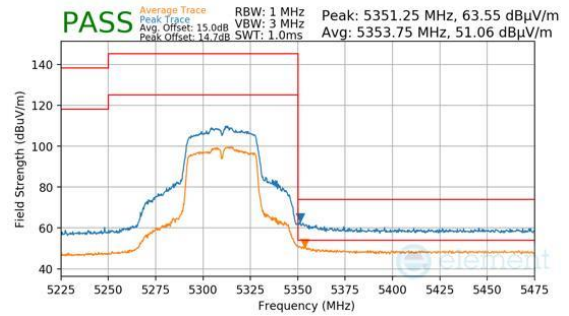
Plot 7-1139. Antenna 3c (Pk & Avg, Ch.62, 802.11n, MCS4)
