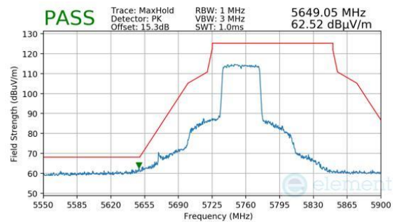
Plot 7-1188. Antenna 3c (Pk, Ch.151, 802.11ax(SU), MCS2)
