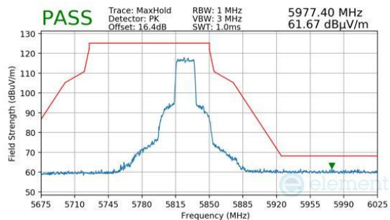
Plot 7-1127. Antenna 3c (Pk, Ch.165, 802.11ax(SU), MCS4)
