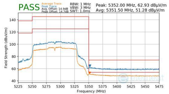
Plot 7-1197. Antenna 3c (Pk & Avg, Ch.58, 802.11ac, MCS2)
