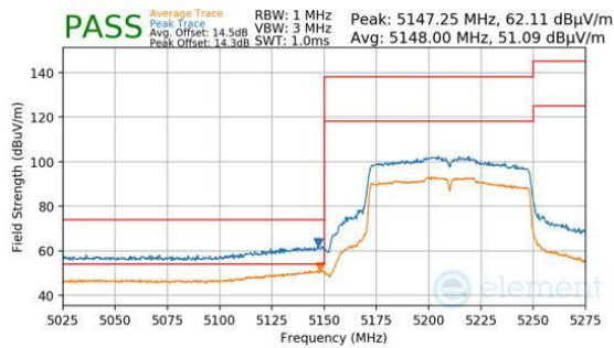
Plot 7-1194. Antenna 3c (Pk & Avg, Ch.42, 802.11ac, MCS2)
