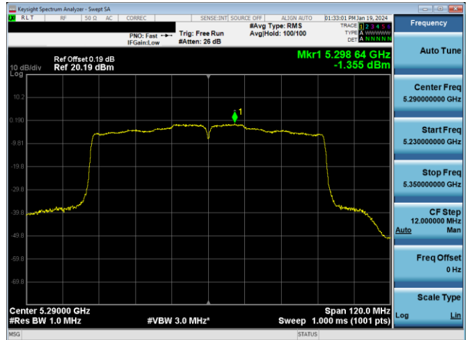
Plot 7-395. PSD Antenna 3a (80MHz BW 802.11ac – Ch. 58, MCS4)
