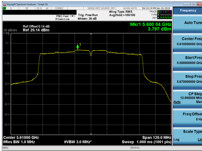
Plot 7-271. PSD Antenna 3c (80MHz BW 802.11ac – Ch. 122, MCS2)
