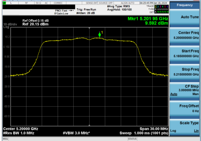
Plot 7-275. PSD Antenna 3c (20MHz BW 802.11n – Ch. 40, MCS4)
