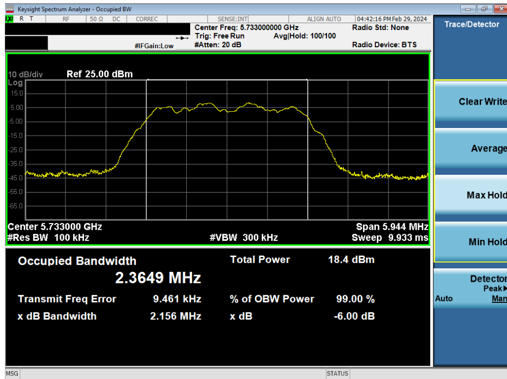
Plot 7-19. 6dB BW & 99% OBW Antenna 3c (HDR4, ePA, 5733MHz)
