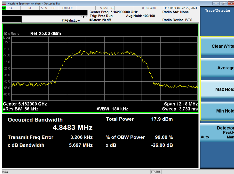
Plot 7-4. 26dB BW & 99% OBW Antenna 3c (HDR8, ePA- 5162MHz)
