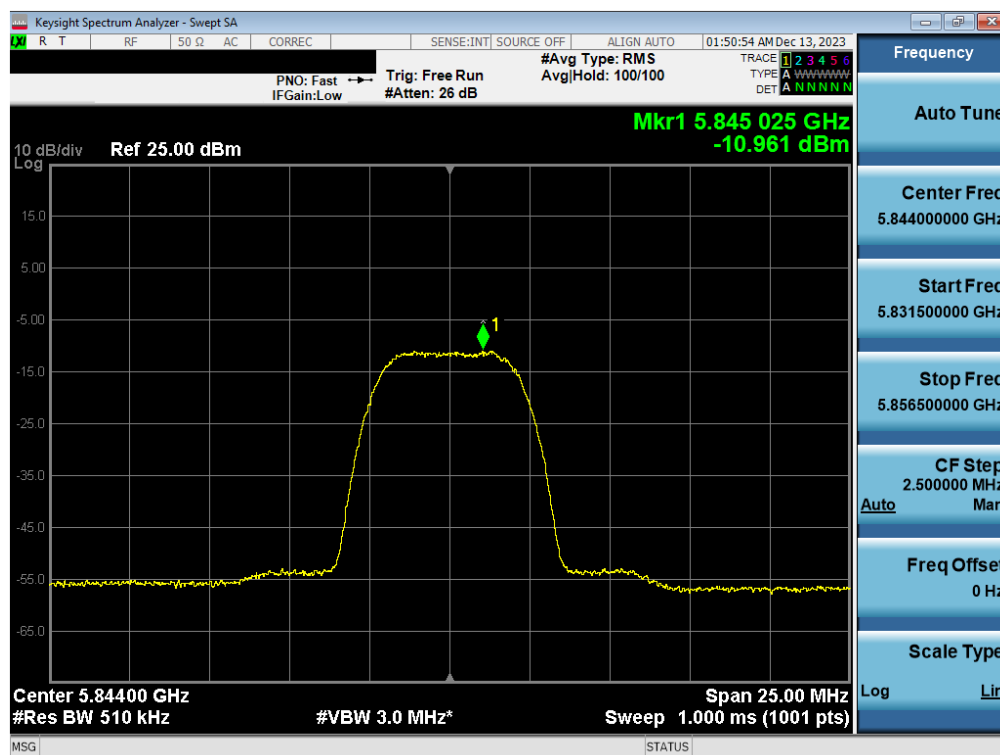
Plot 7-114. PSD Antenna 1b (HDR8, iPA 5844MHz)
