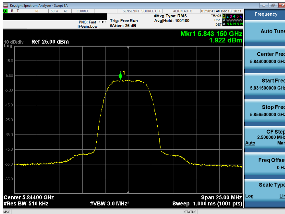
Plot 7-111. PSD Antenna 1b (HDR8, ePA 5844MHz)
