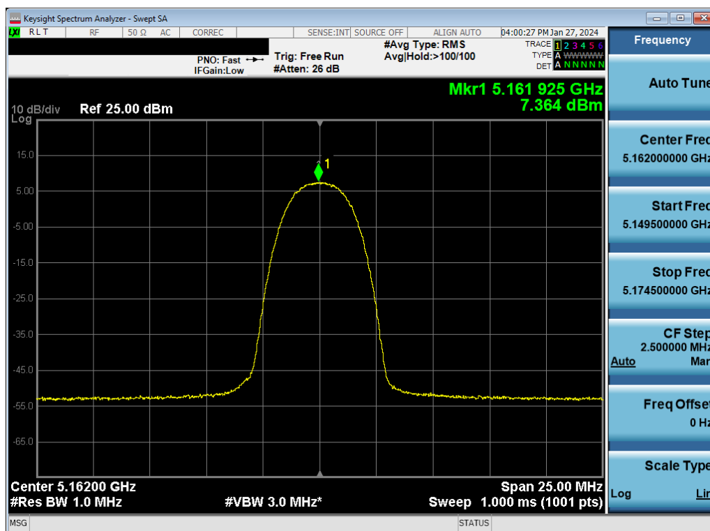
Plot 7-49. ISED PSD Antenna 3c (HDR4, ePA – 5162MHz)
