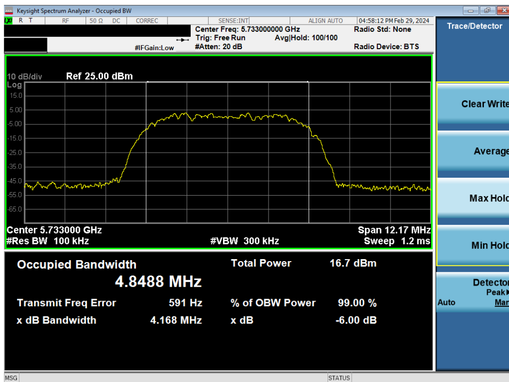
Plot 7-34. 6dB BW & 99% OBW Antenna 1b (HDR8, ePA, 5733MHz)
