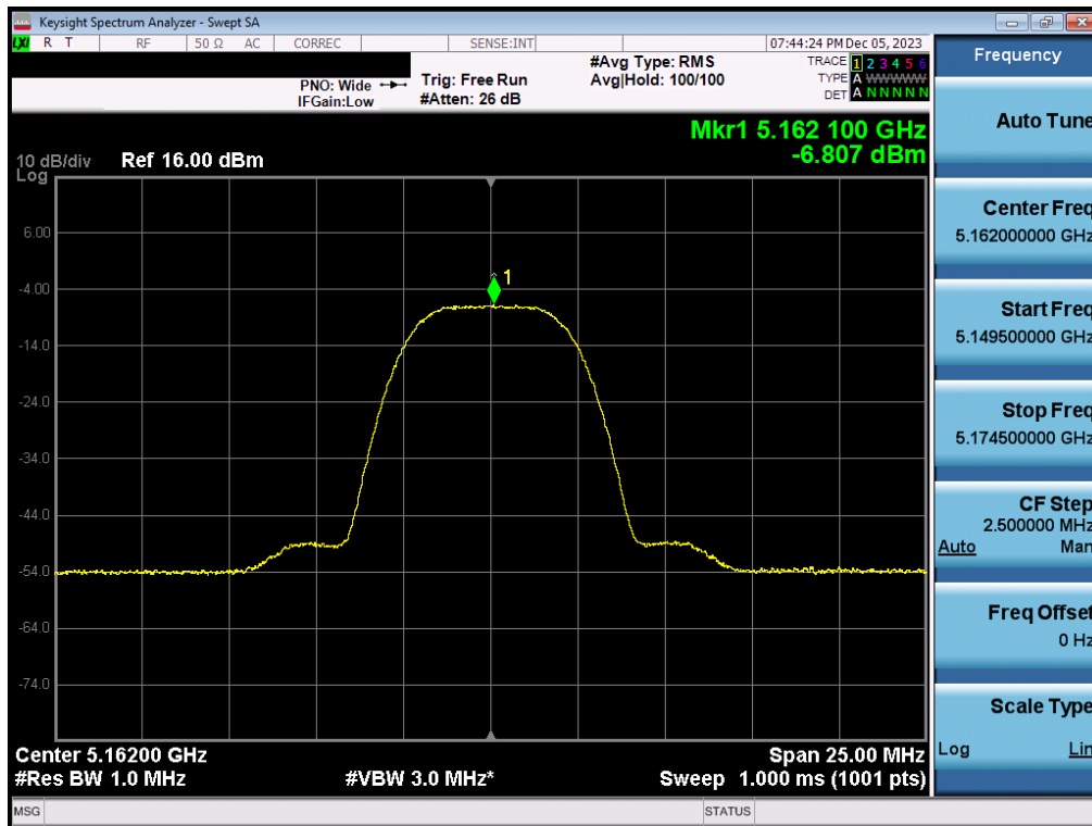
Plot 7-100. PSD Antenna 1b (HDR8, iPA – 5162MHz)
