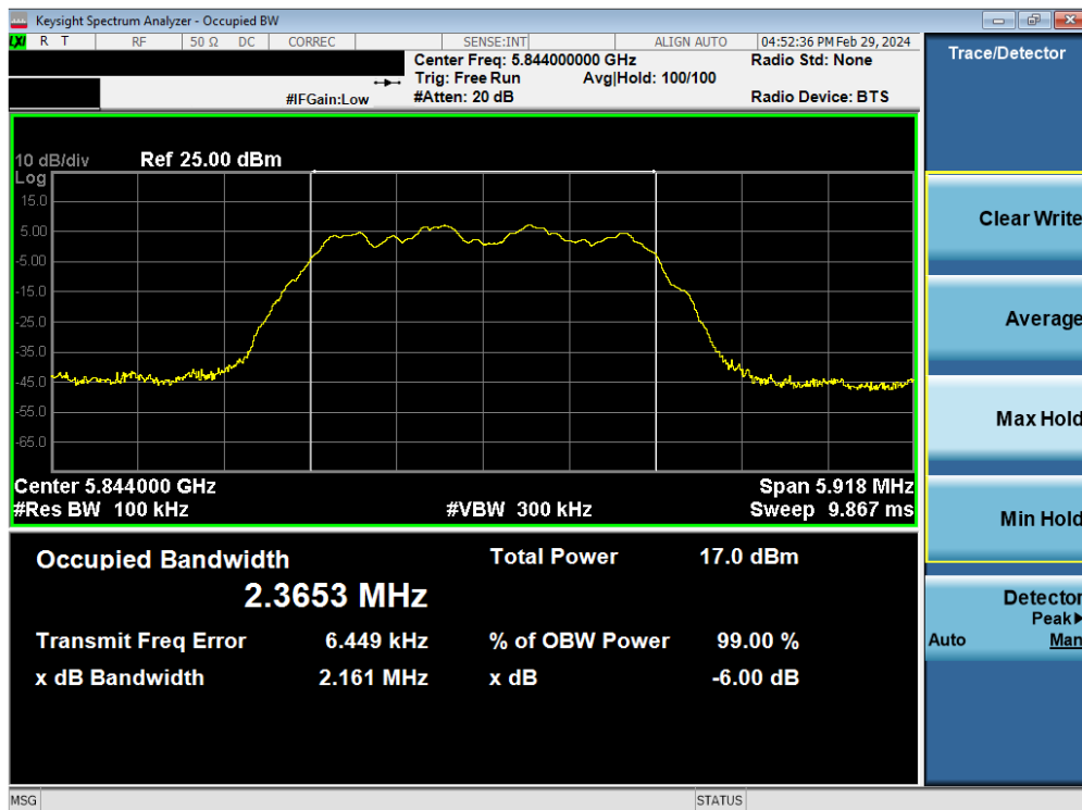
Plot 7-27. 6dB BW & 99% OBW Antenna 3a (HDR4, ePA, 5844MHz)
