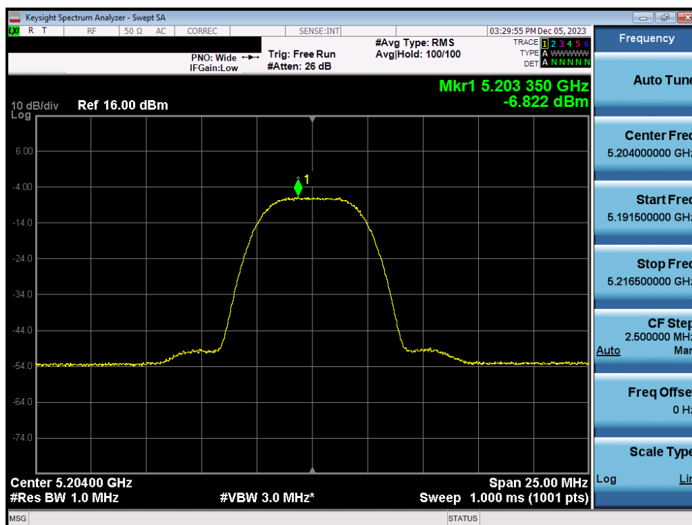
Plot 7-77. PSD Antenna 3a (HDR8, iPA – 5204MHz)
