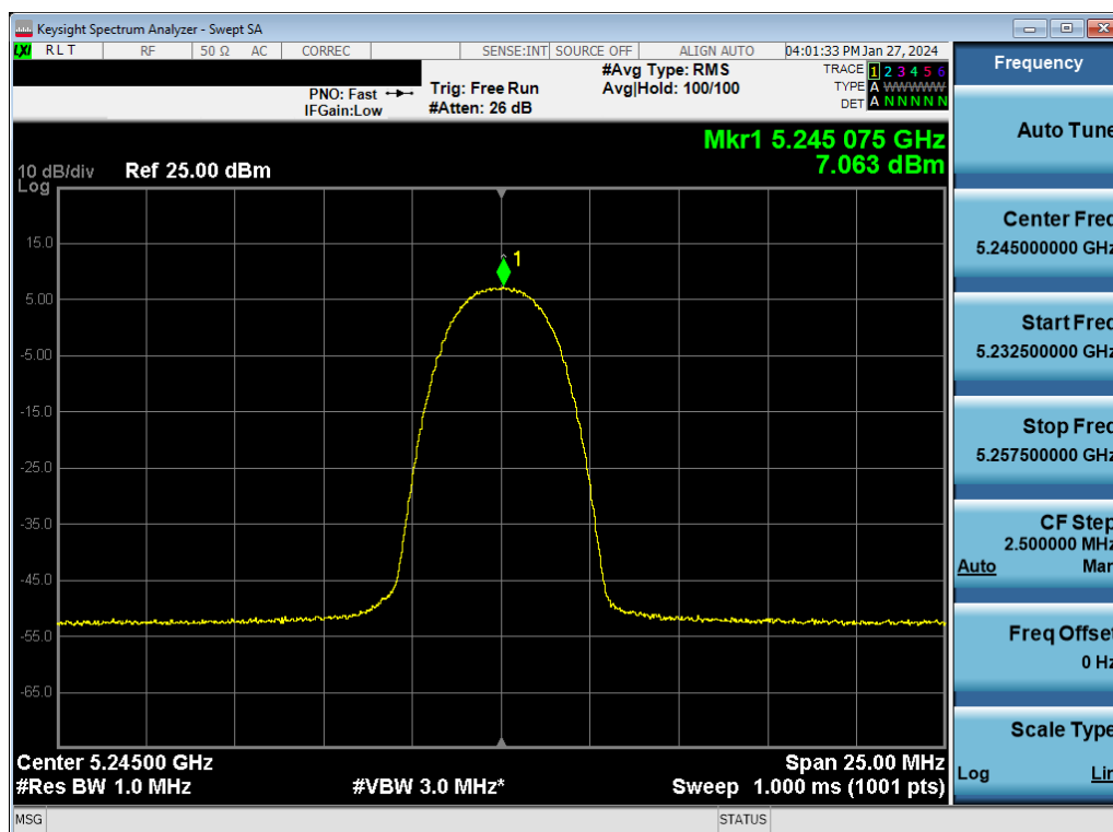
Plot 7-51. ISED PSD Antenna 3c (HDR4, ePA– 5245MHz)
