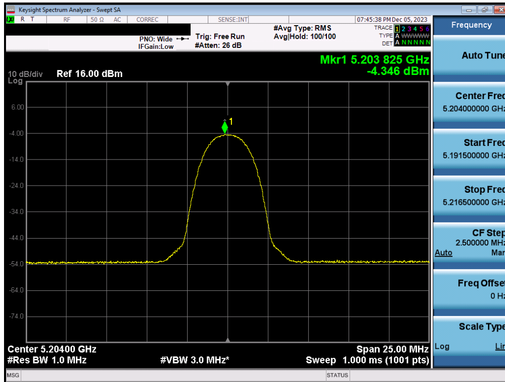
Plot 7-95. PSD Antenna 1b (HDR4, iPA - 5204MHz)
