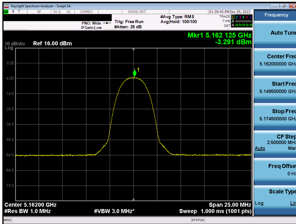
Plot 7-40. FCC/ISED PSD Antenna 3c (HDR4, iPA - 5162MHz)
