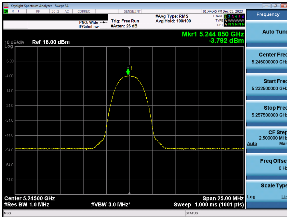
Plot 7-42. FCC/ISED PSD Antenna 3c (HDR4, iPA– 5245MHz)
