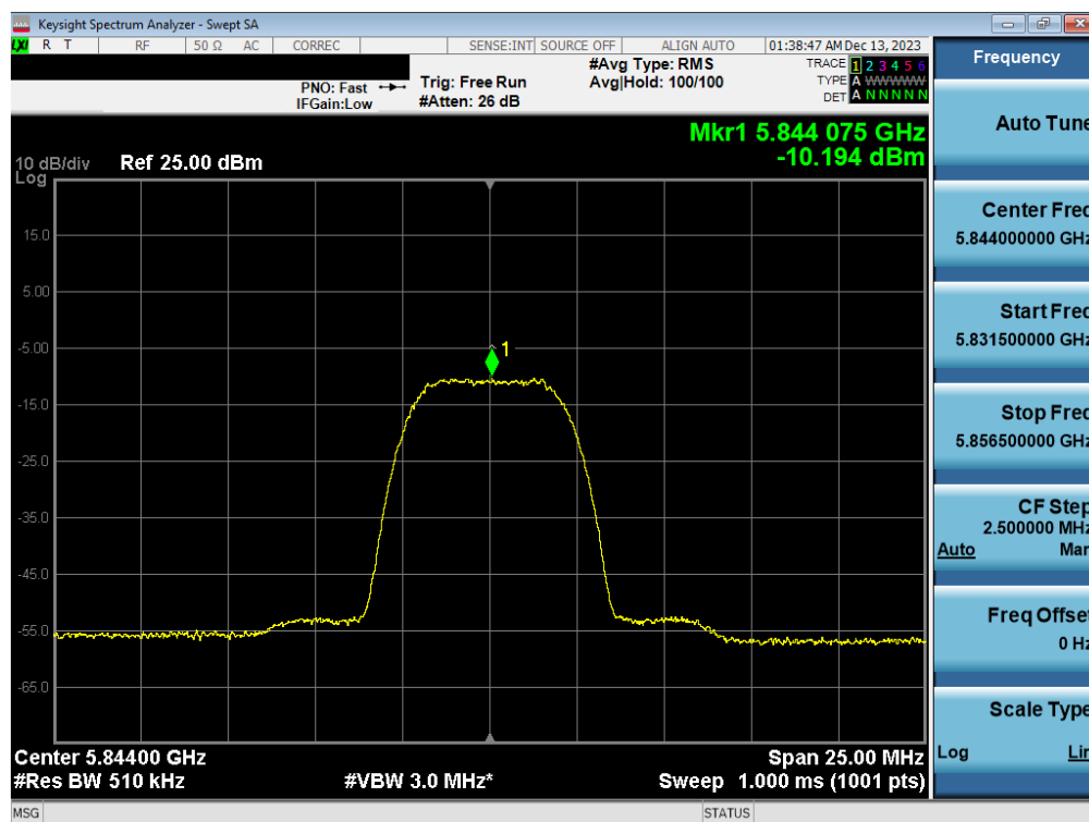
Plot 7-90. PSD Antenna 3a (HDR8, iPA 5844MHz)
