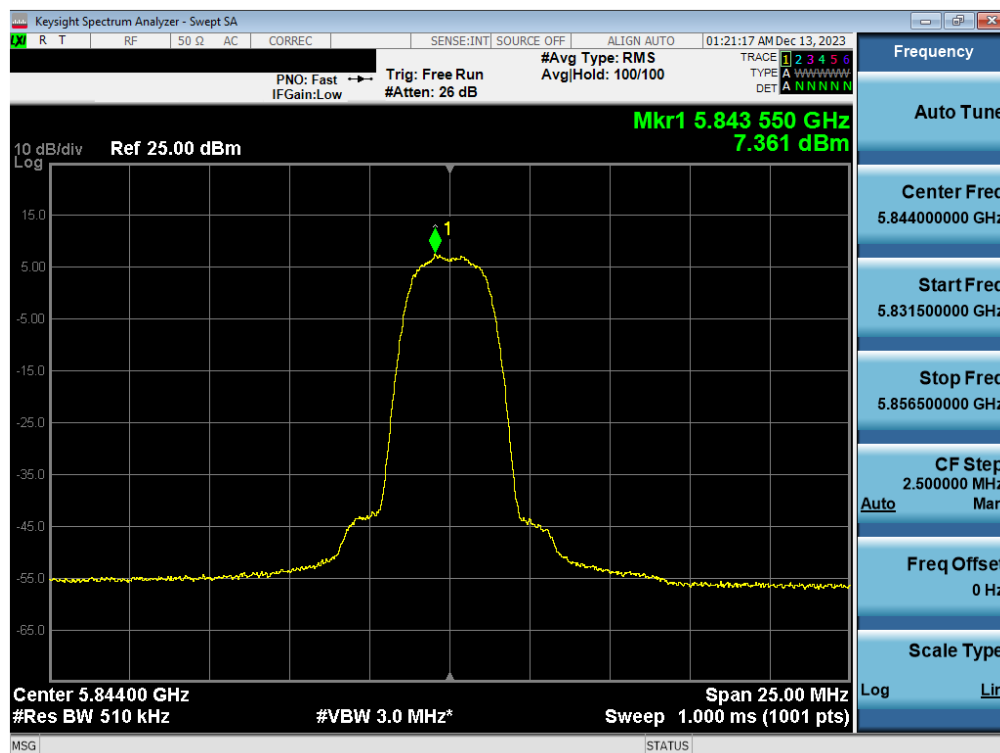
Plot 7-57. PSD Antenna 3c (HDR4, ePA 5844MHz)
