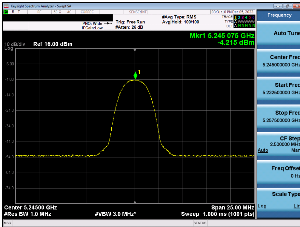
Plot 7-72. PSD Antenna 3a (HDR4, iPA- 5245MHz)
