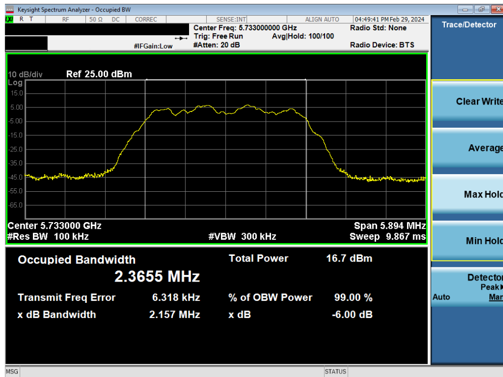
Plot 7-25. 6dB BW & 99% OBW Antenna 3a (HDR4, ePA, 5733MHz)
