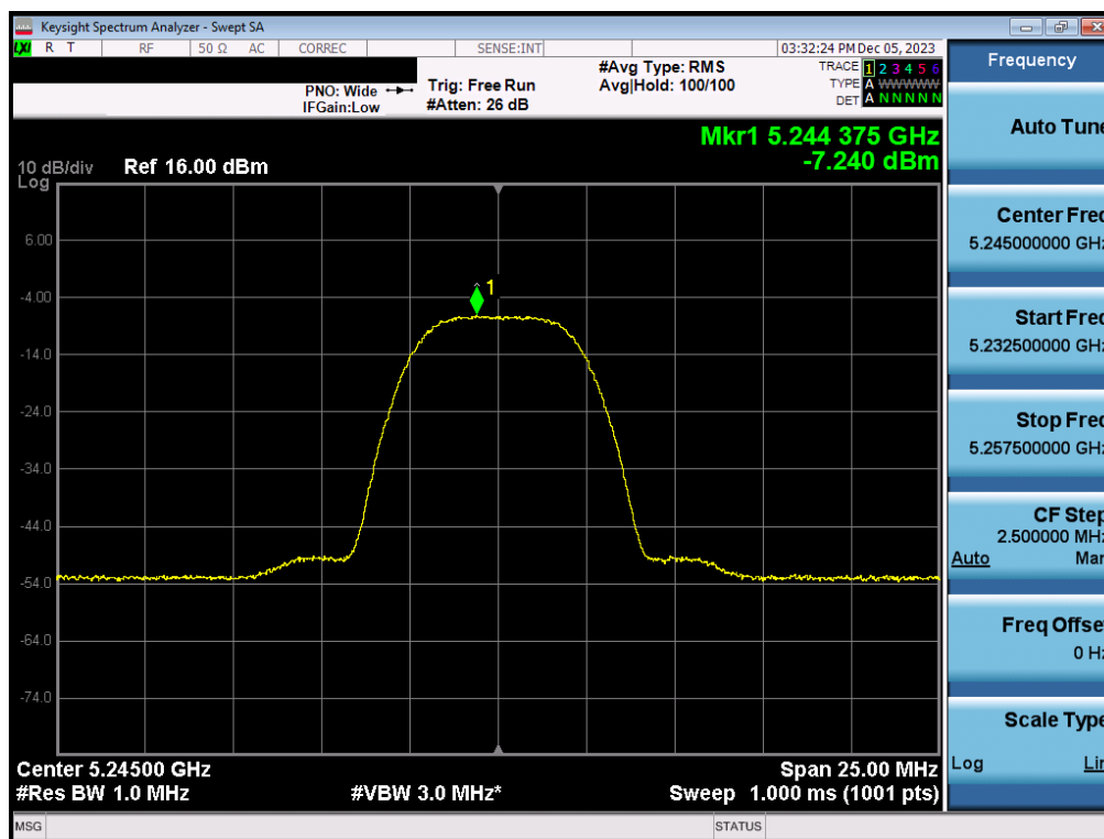
Plot 7-78. PSD Antenna 3a (HDR8, iPA– 5245MHz)
