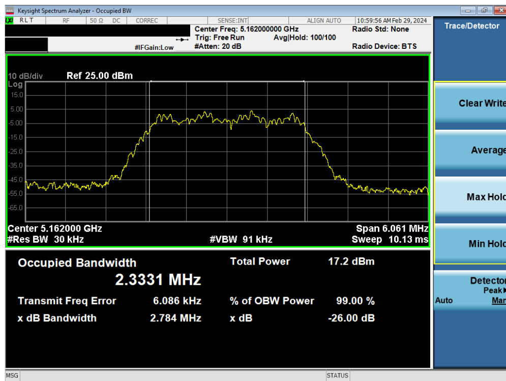
Plot 7-1. 26dB BW & 99% OBW Antenna 3c (HDR4, ePA– 5162MHz)
