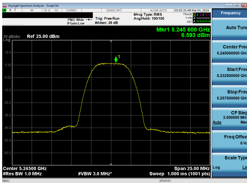
Plot 7-54. ISED PSD Antenna 3c (HDR8, ePA– 5245MHz)
