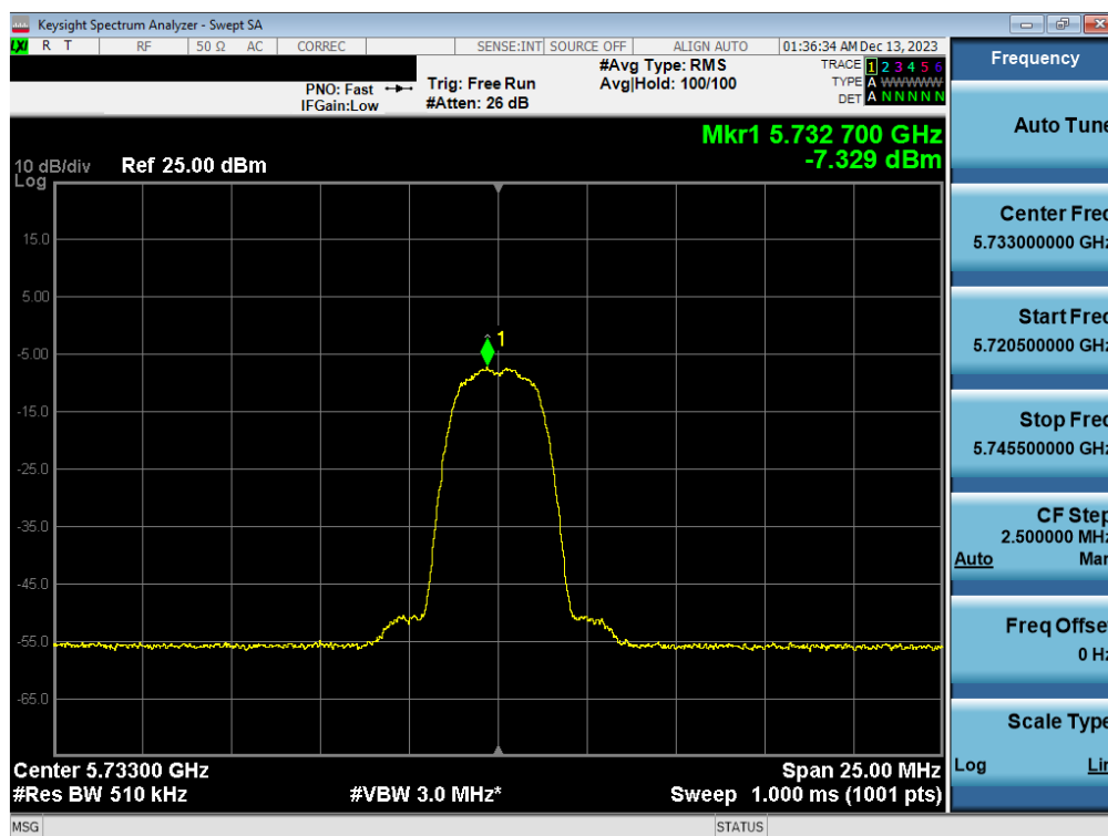
Plot 7-82. PSD Antenna 3a (HDR4, iPA 5733MHz)
