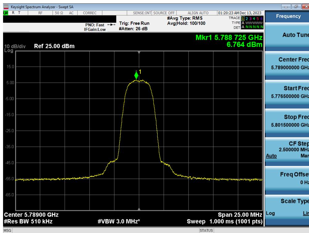
Plot 7-56. PSD Antenna 3c (HDR4, ePA 5789MHz)
