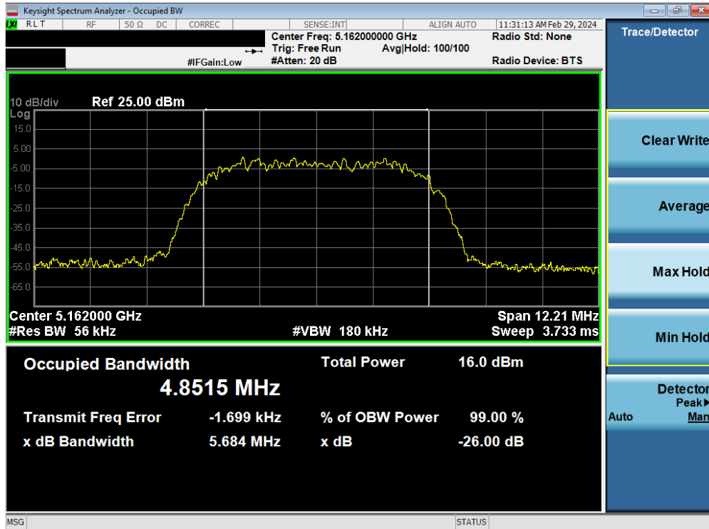
Plot 7-16. 26dB BW & 99% OBW Antenna 1b (HDR8, ePA- 5162MHz)
