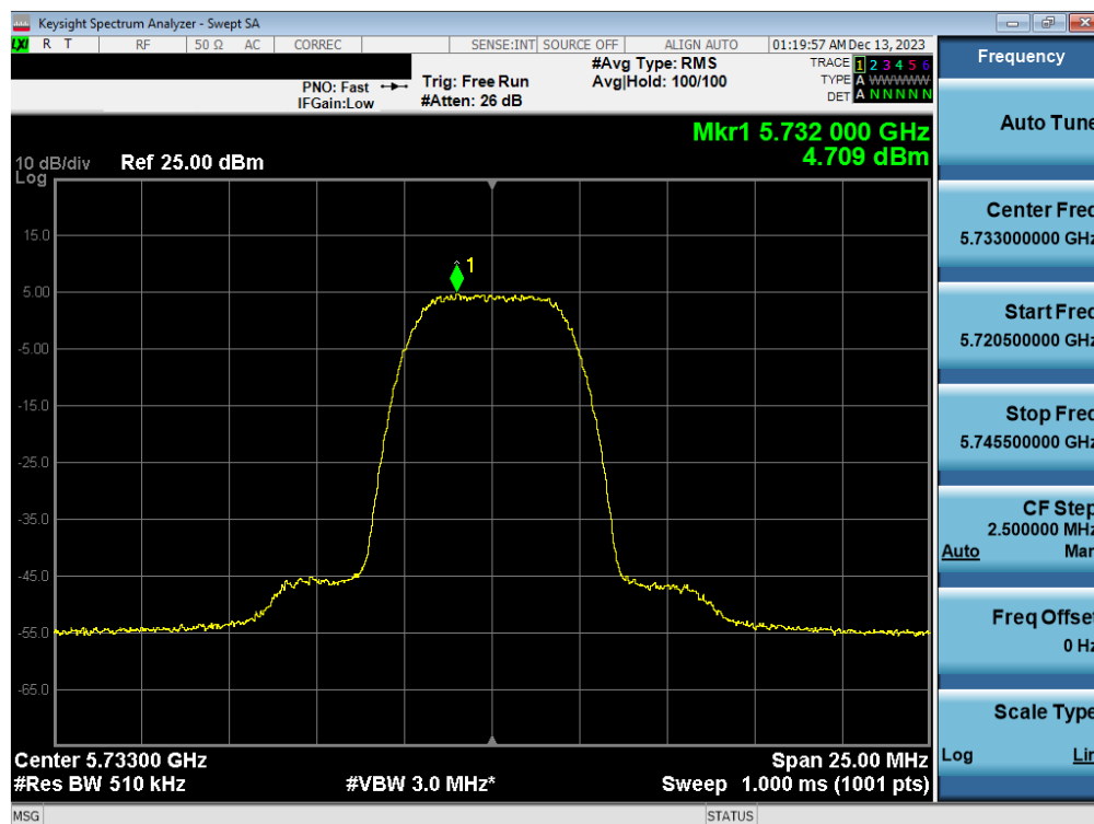
Plot 7-61. PSD Antenna 3c (HDR8, ePA 5733MHz)
