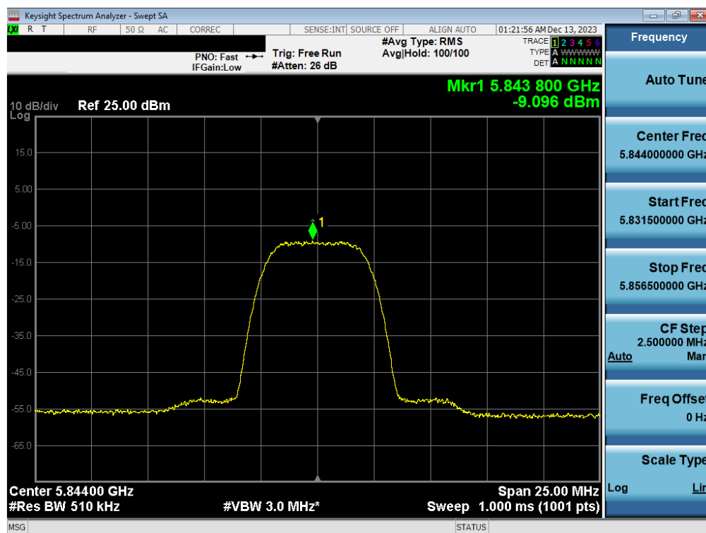
Plot 7-66. PSD Antenna 3c (HDR8, iPA 5844MHz)
