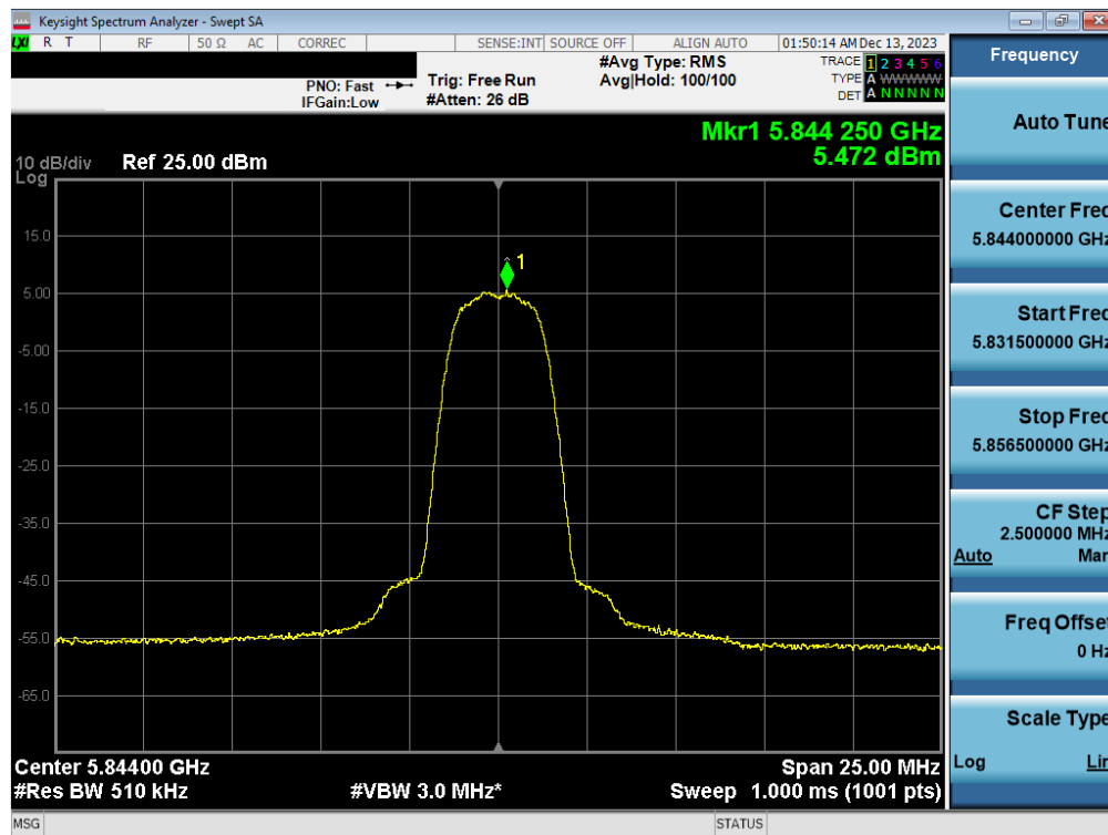
Plot 7-105. PSD Antenna 1b (HDR4, ePA 5844MHz)
