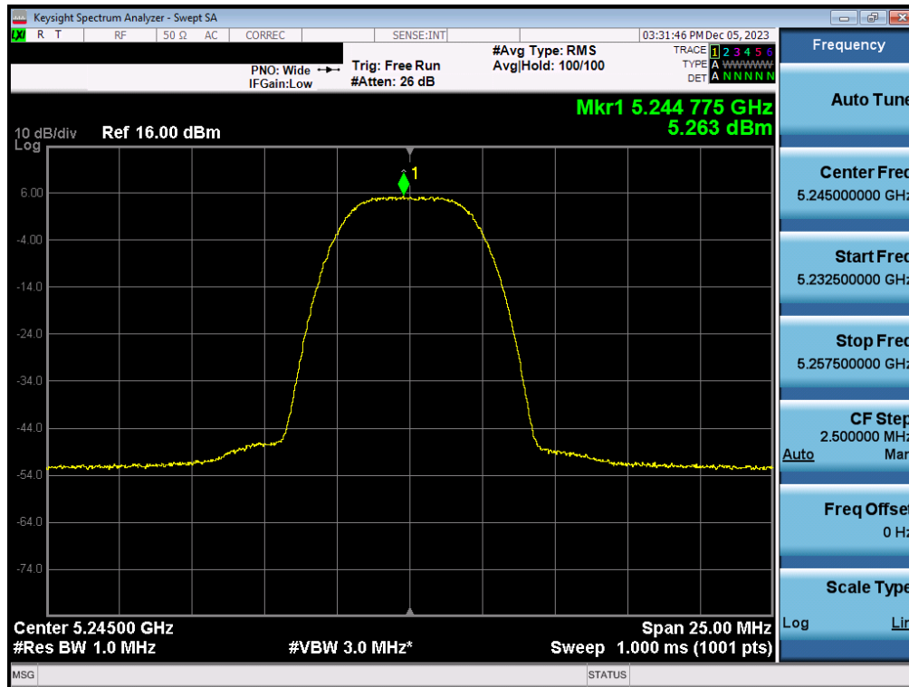
Plot 7-75. PSD Antenna 3a (HDR8, ePA– 5245MHz)
