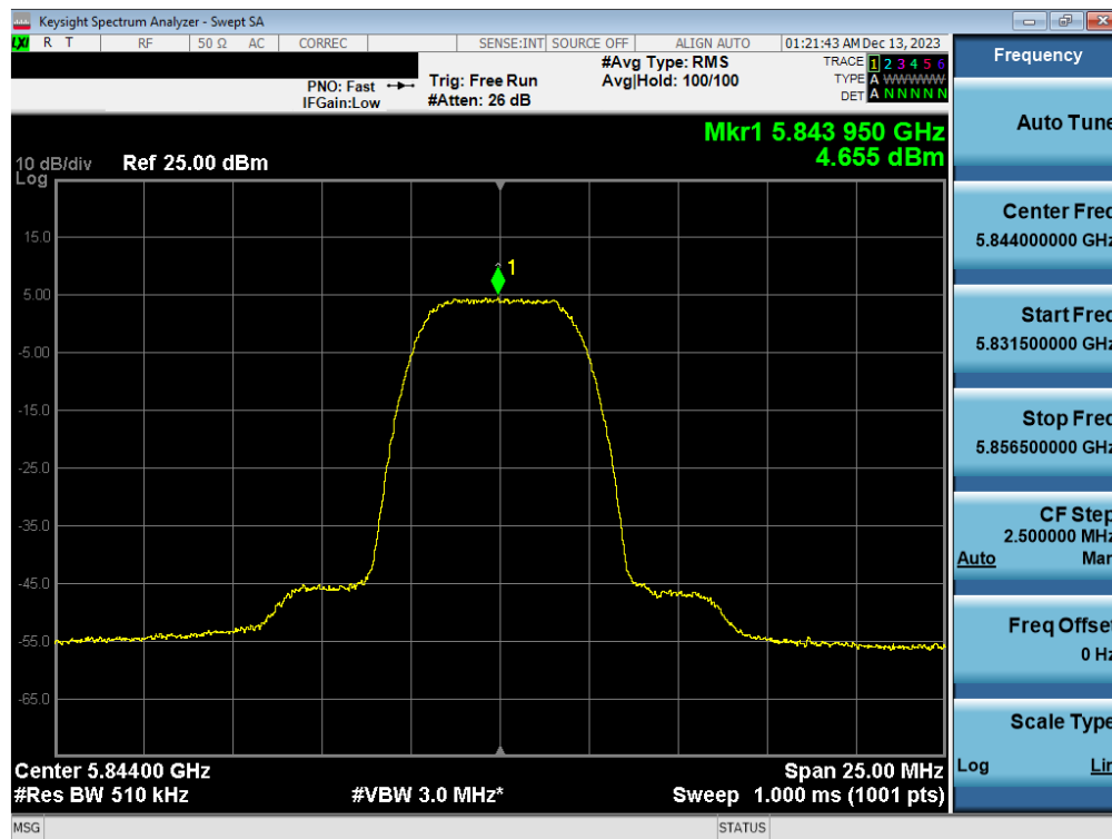
Plot 7-63. PSD Antenna 3c (HDR8, ePA 5844MHz)
