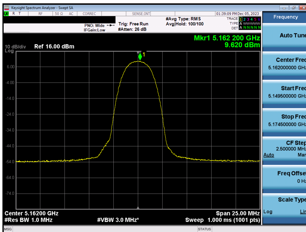
Plot 7-37. FCC PSD Antenna 3c (HDR4, ePA – 5162MHz)
