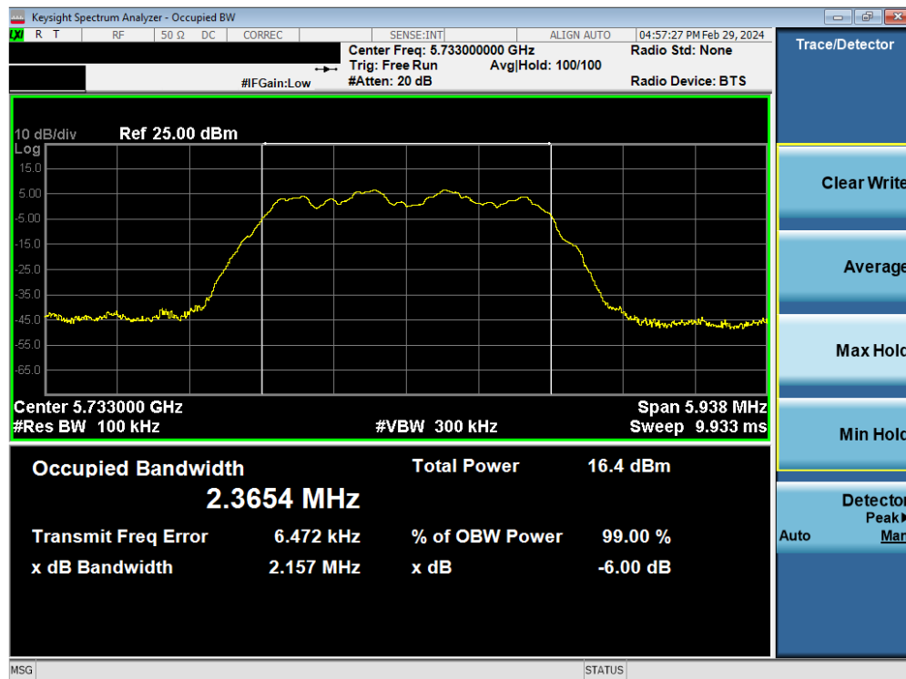
Plot 7-31. 6dB BW & 99% OBW Antenna 1b (HDR4, ePA, 5733MHz)
