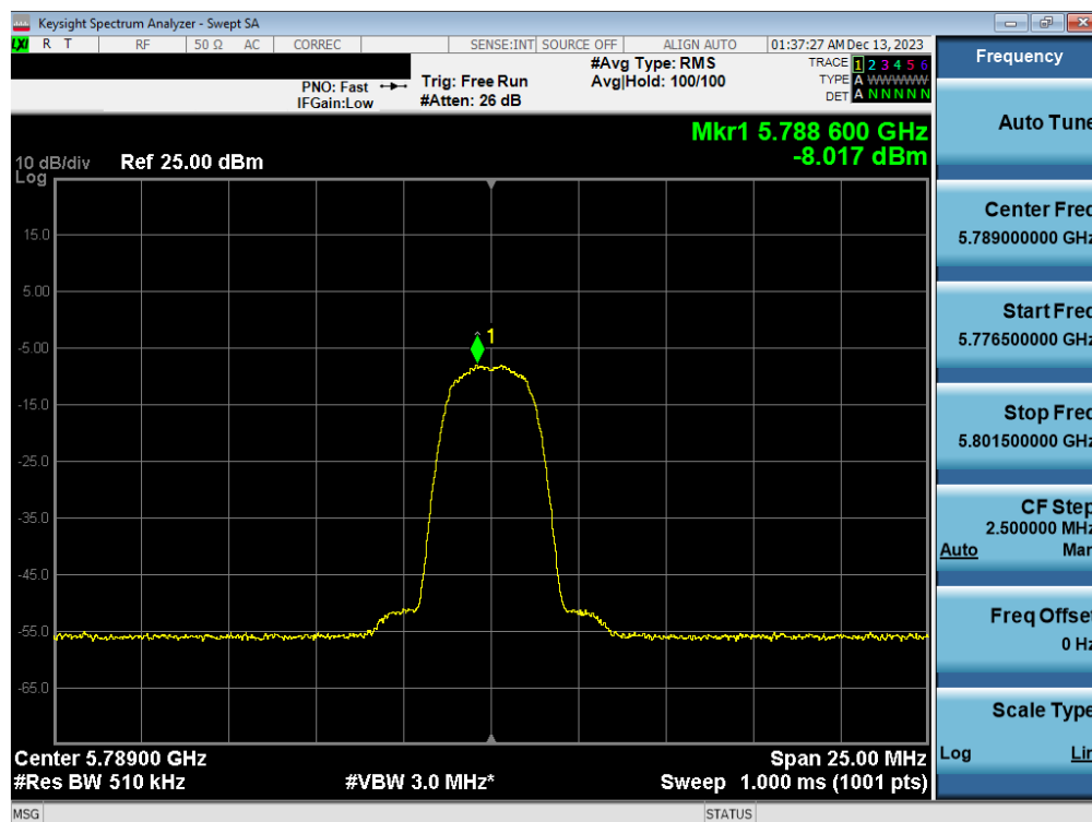
Plot 7-83. PSD Antenna 3a (HDR4, iPA 5789MHz)
