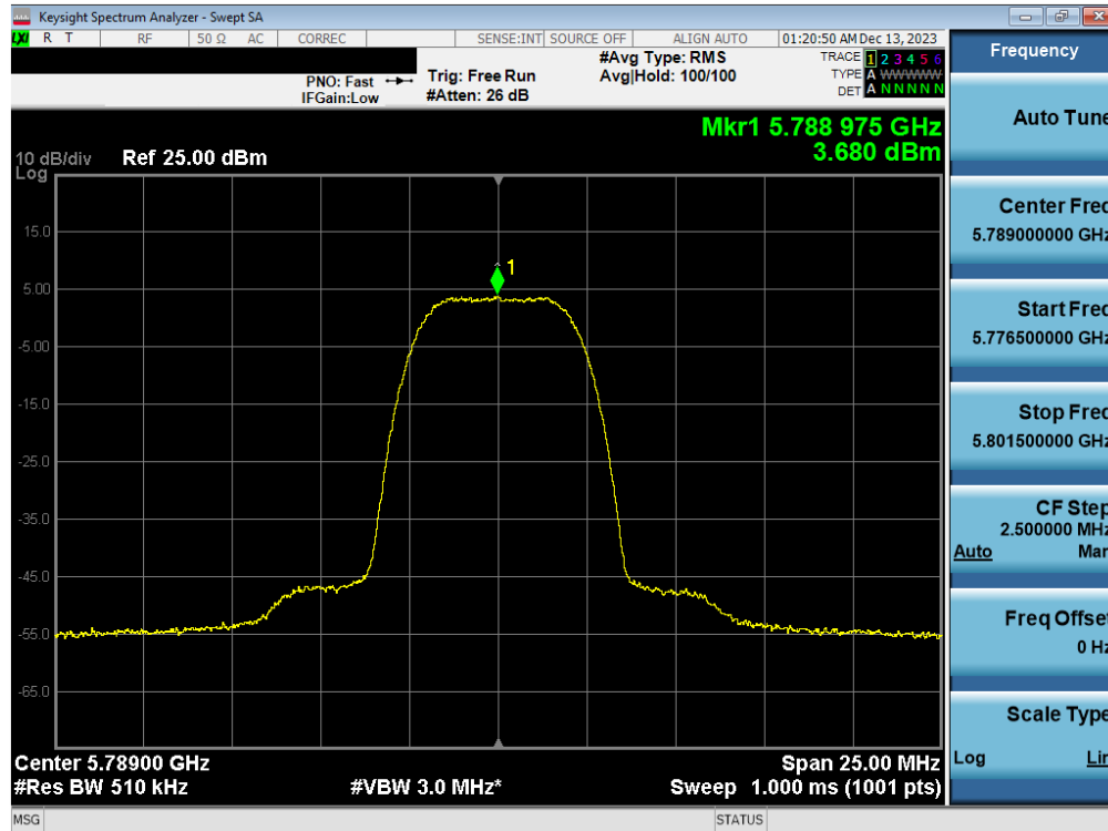
Plot 7-62. PSD Antenna 3c (HDR8, ePA 5789MHz)
