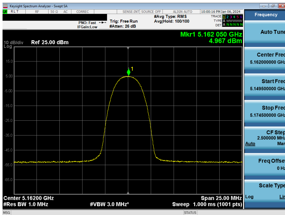
Plot 7-115. FCC PSD TxBF Antenna 3c (HDR4, ePA – 5162MHz)
