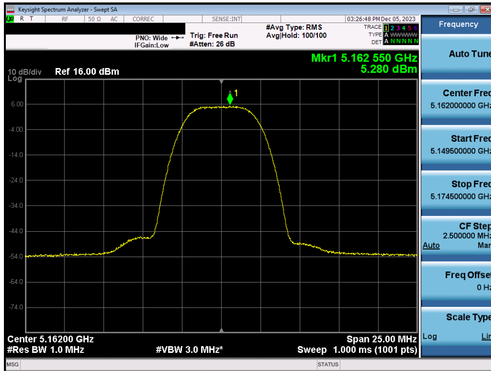
Plot 7-73. PSD Antenna 3a (HDR8, ePA – 5162MHz)
