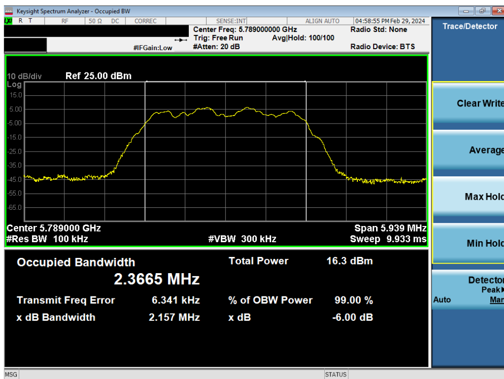
Plot 7-32. 6dB BW & 99% OBW Antenna 1b (HDR4, ePA, 5789MHz)
