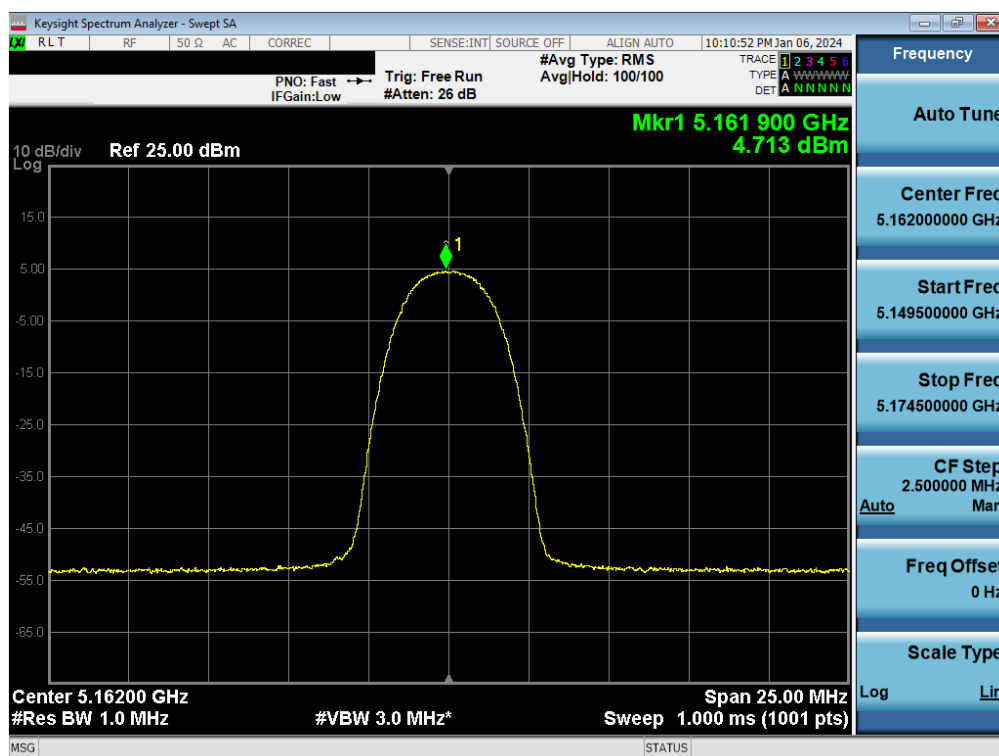
Plot 7-116. FCC PSD TxBF Antenna 3a (HDR4, ePA – 5162MHz)
