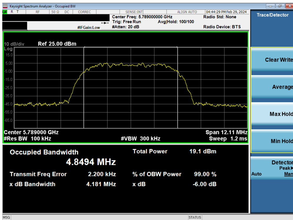
Plot 7-23. 6dB BW & 99% OBW Antenna 3c (HDR8, ePA, 5789MHz)
