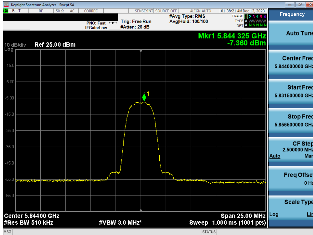
Plot 7-84. PSD Antenna 3a (HDR4, iPA 5844MHz)
