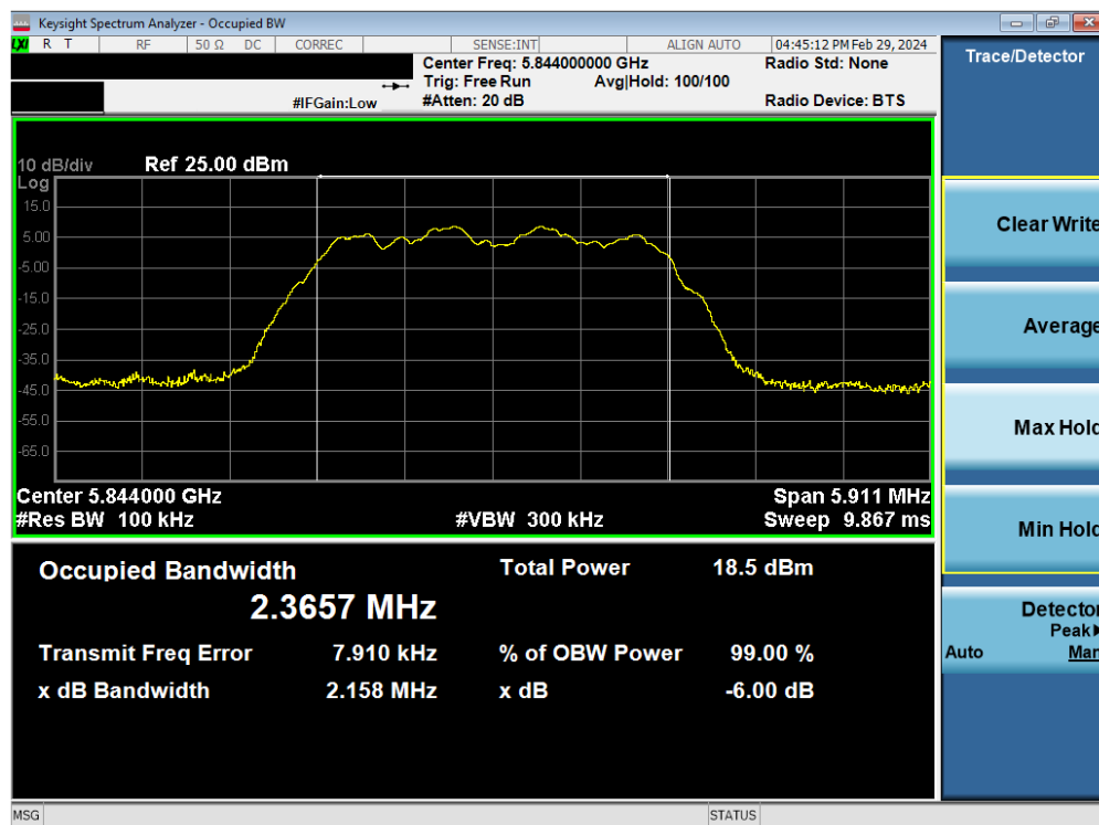
Plot 7-21. 6dB BW & 99% OBW Antenna 3c (HDR4, ePA, 5844MHz)
