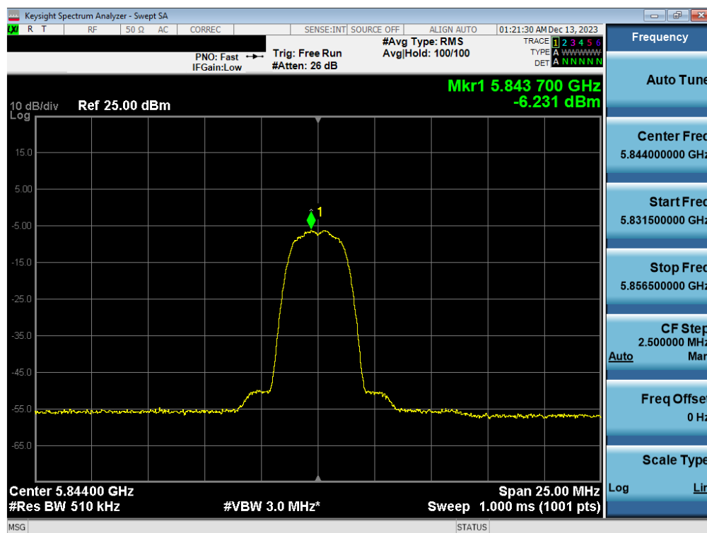
Plot 7-60. PSD Antenna 3c (HDR4, iPA 5844MHz)
