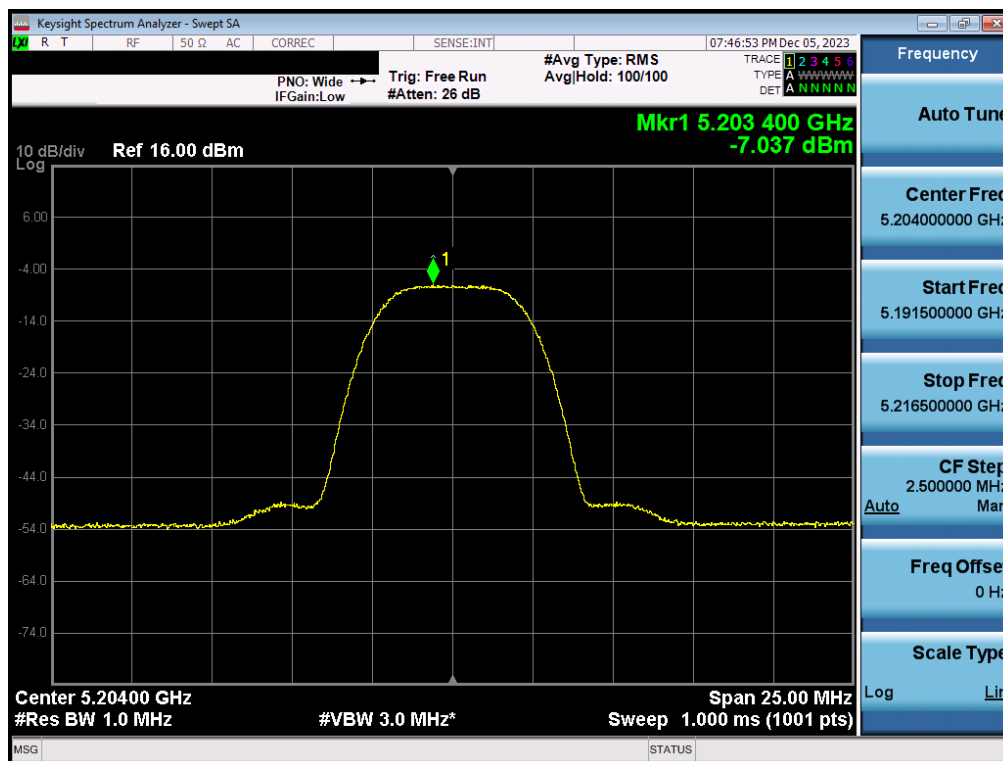
Plot 7-101. PSD Antenna 1b (HDR8, iPA – 5204MHz)
