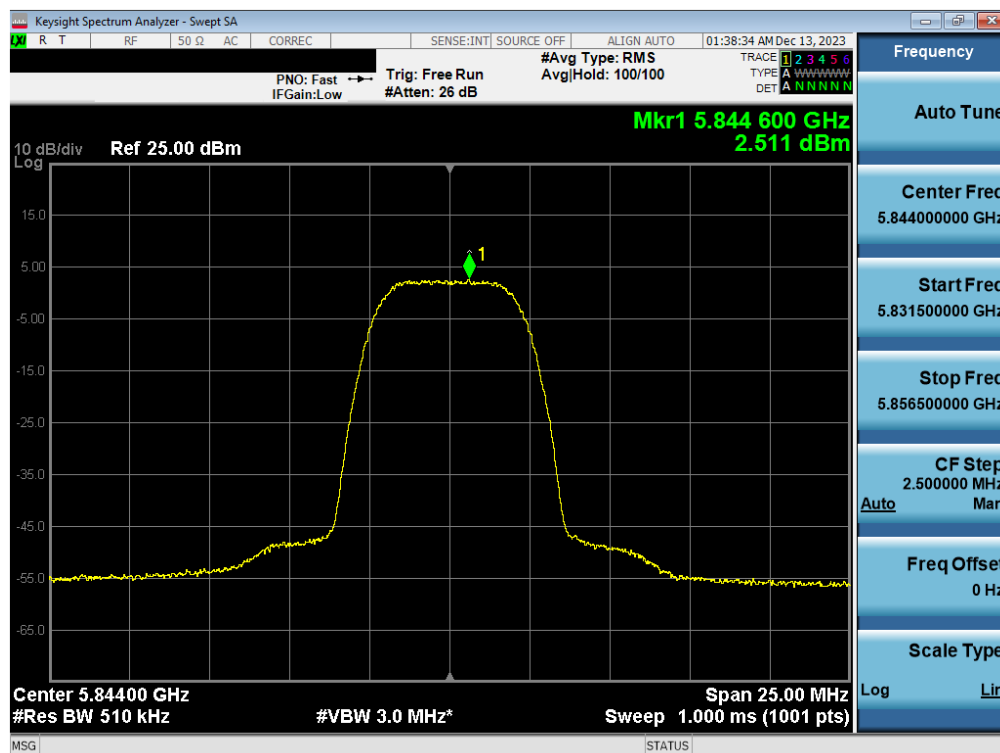
Plot 7-87. PSD Antenna 3a (HDR8, ePA 5844MHz)
