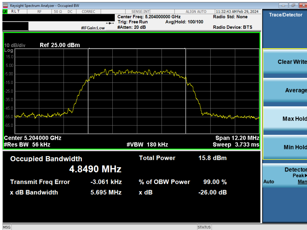
Plot 7-17. 26dB BW & 99% OBW Antenna 1b (HDR8, ePA- 5204MHz)
