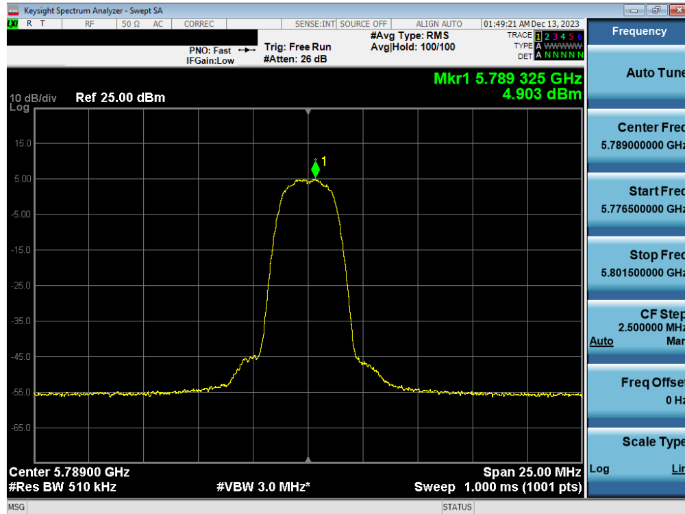
Plot 7-104. PSD Antenna 1b (HDR4, ePA 5789MHz)
