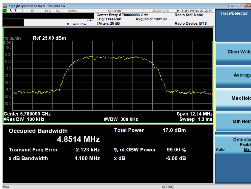
Plot 7-29. 6dB BW & 99% OBW Antenna 3a (HDR8, ePA, 5789MHz)
