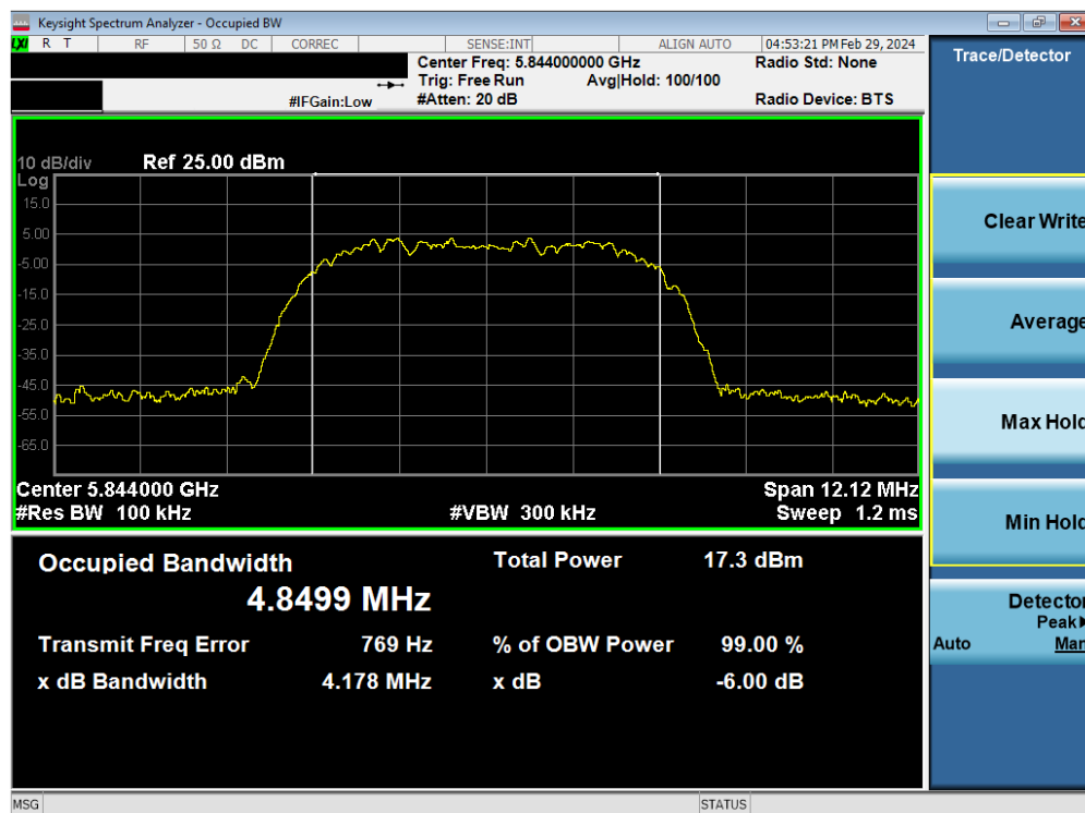
Plot 7-30. 6dB BW & 99% OBW Antenna 3a (HDR8, ePA, 5844MHz)
