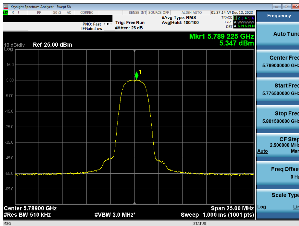
Plot 7-80. PSD Antenna 3a (HDR4, ePA 5789MHz)
