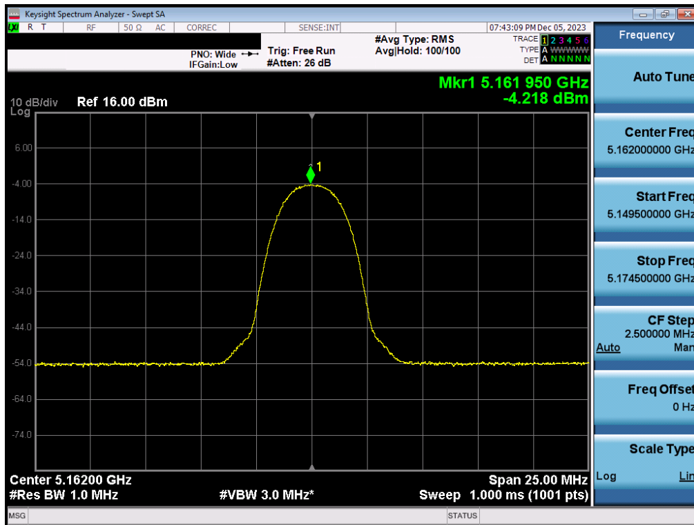
Plot 7-94. PSD Antenna 1b (HDR4, iPA – 5162MHz)
