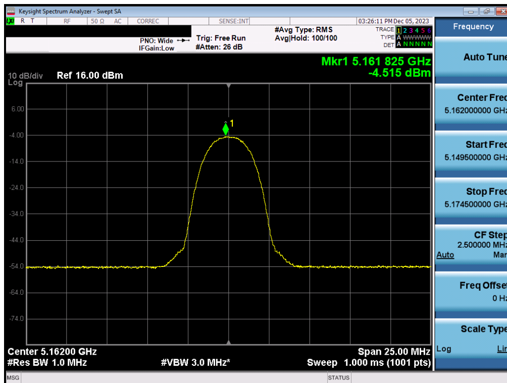
Plot 7-70. PSD Antenna 3a (HDR4, iPA – 5162MHz)
