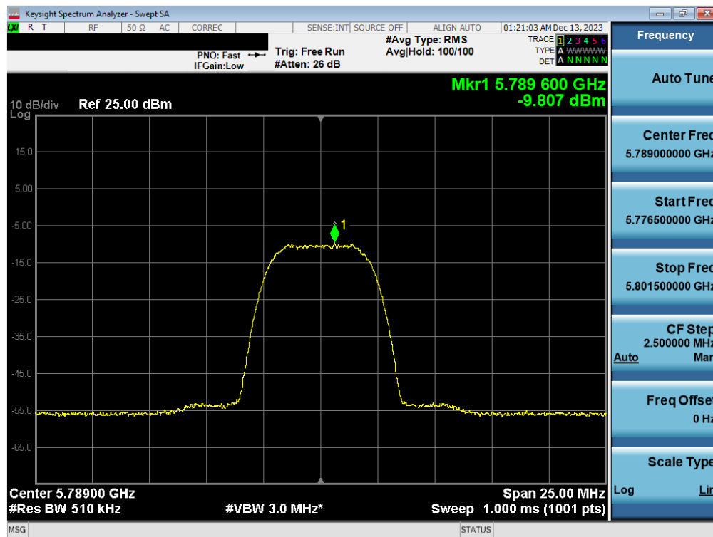
Plot 7-65. PSD Antenna 3c (HDR8, iPA 5789MHz)
