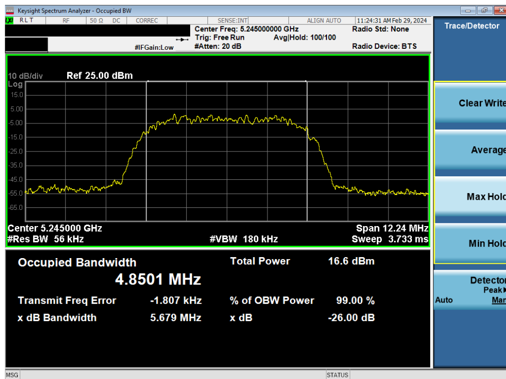
Plot 7-12. 26dB BW & 99% OBW Antenna 3a (HDR8, ePA– 5245MHz)
