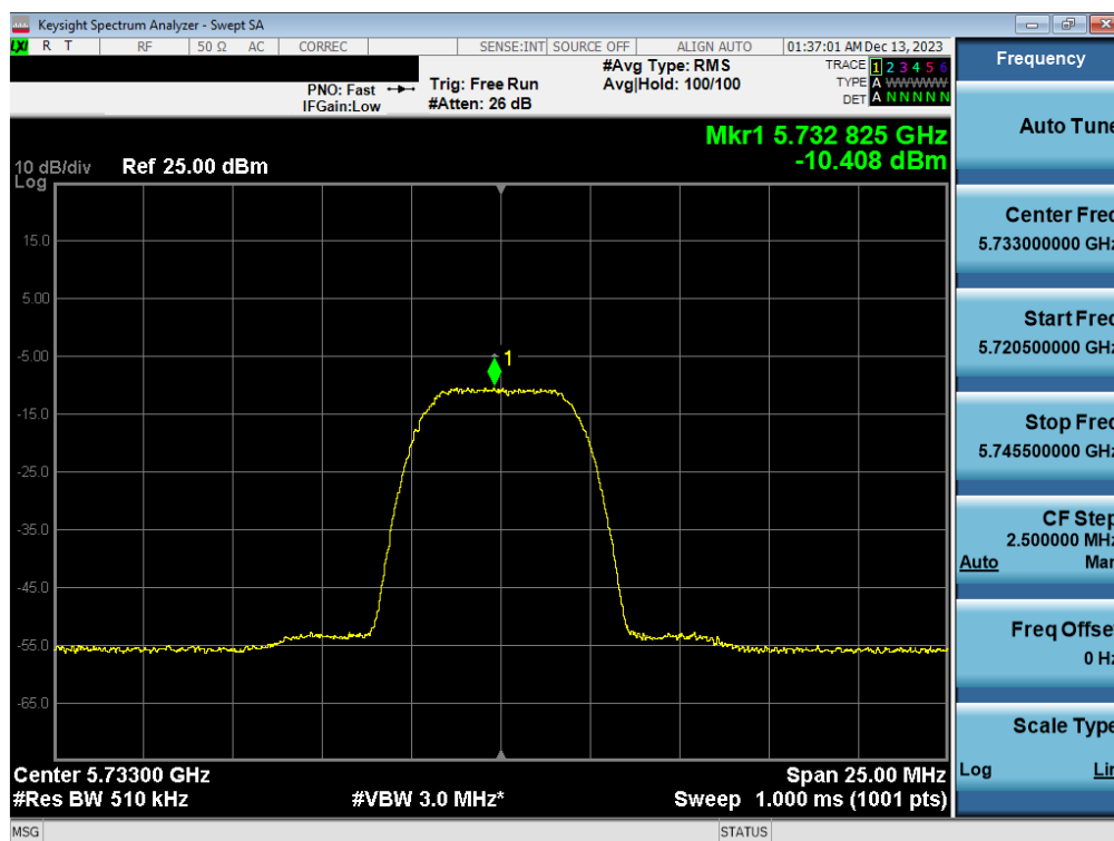
Plot 7-88. PSD Antenna 3a (HDR8, iPA 5733MHz)
