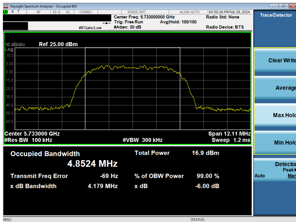
Plot 7-28. 6dB BW & 99% OBW Antenna 3a (HDR8, ePA, 5733MHz)
