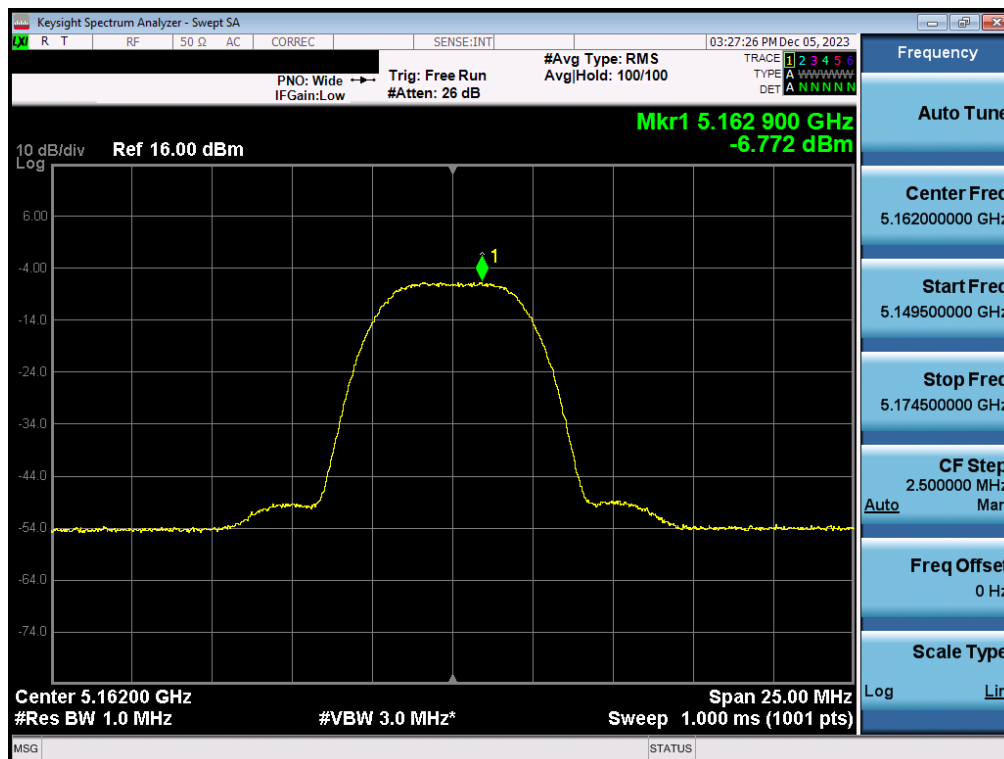
Plot 7-76. PSD Antenna 3a (HDR8, iPA – 5162MHz)
