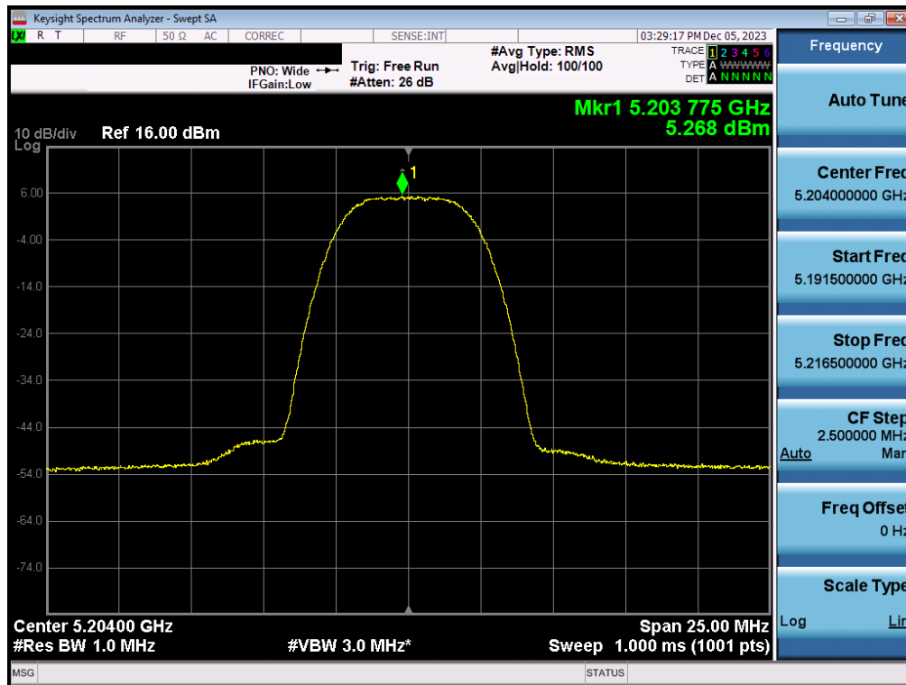
Plot 7-74. PSD Antenna 3a (HDR8, ePA – 5204MHz)
