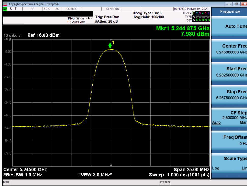
Plot 7-93. PSD Antenna 1b (HDR4, ePA– 5245MHz)
