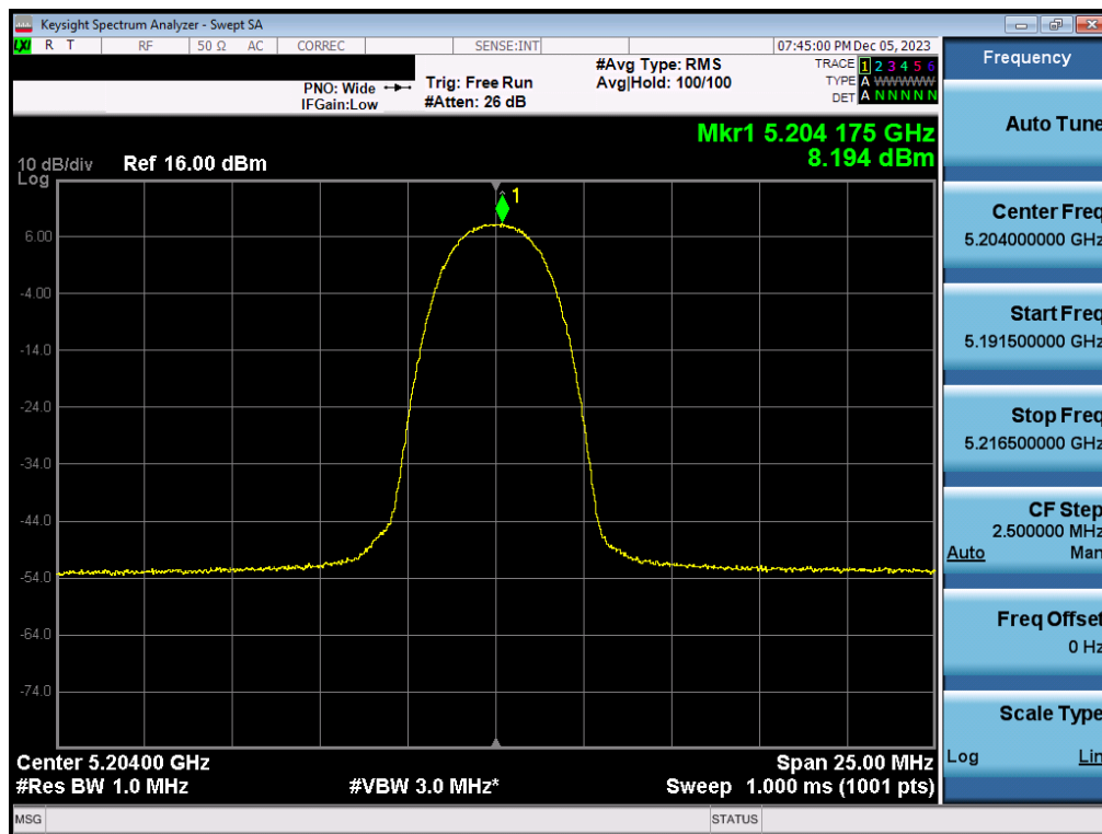
Plot 7-92. PSD Antenna 1b (HDR4, ePA – 5204MHz)
