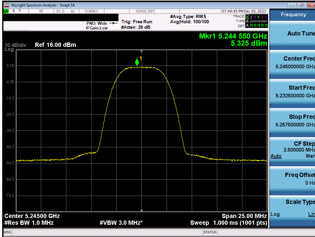
Plot 7-99. PSD Antenna 1b (HDR8, ePA– 5245MHz)
