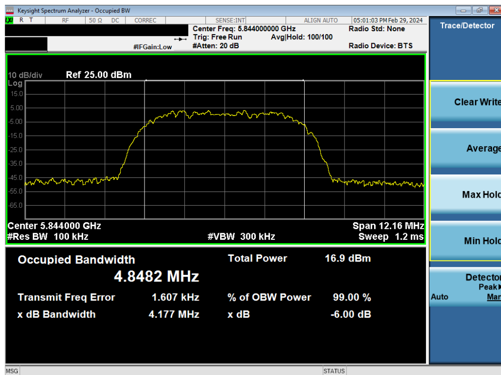
Plot 7-36. 6dB BW & 99% OBW Antenna 1b (HDR8, ePA, 5844MHz)
