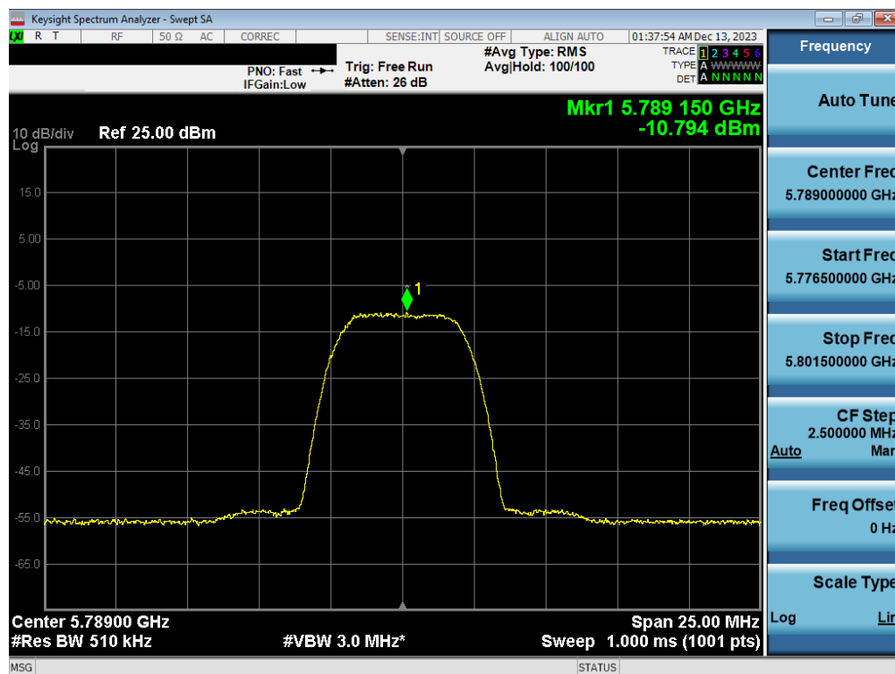
Plot 7-89. PSD Antenna 3a (HDR8, iPA 5789MHz)
