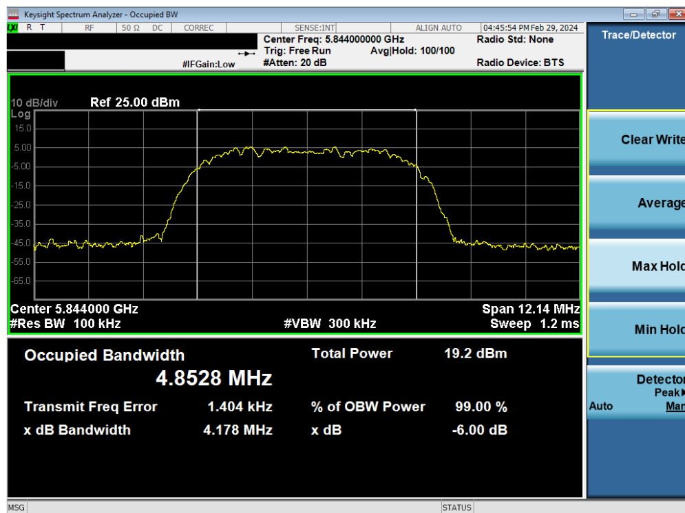
Plot 7-24. 6dB BW & 99% OBW Antenna 3c (HDR8, ePA, 5844MHz)
