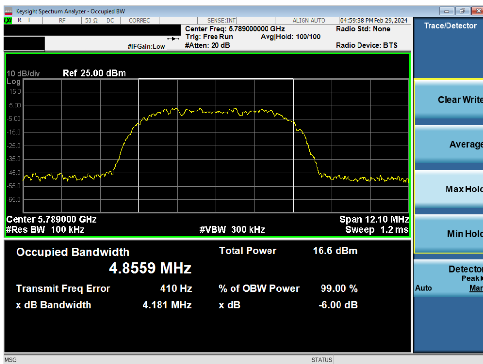
Plot 7-35. 6dB BW & 99% OBW Antenna 1b (HDR8, ePA, 5789MHz)
