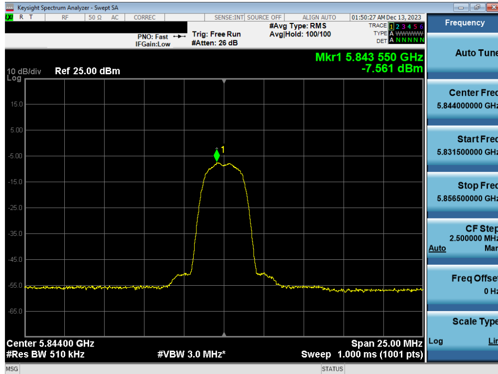
Plot 7-108. PSD Antenna 1b (HDR4, iPA 5844MHz)
