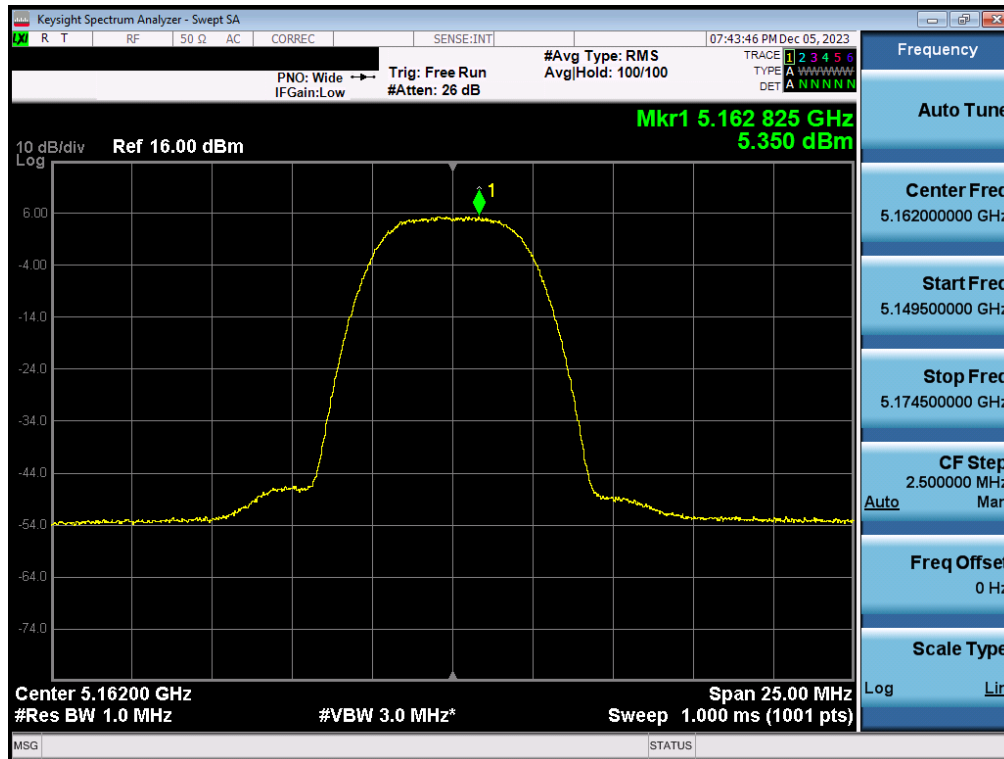
Plot 7-97. PSD Antenna 1b (HDR8, ePA – 5162MHz)
