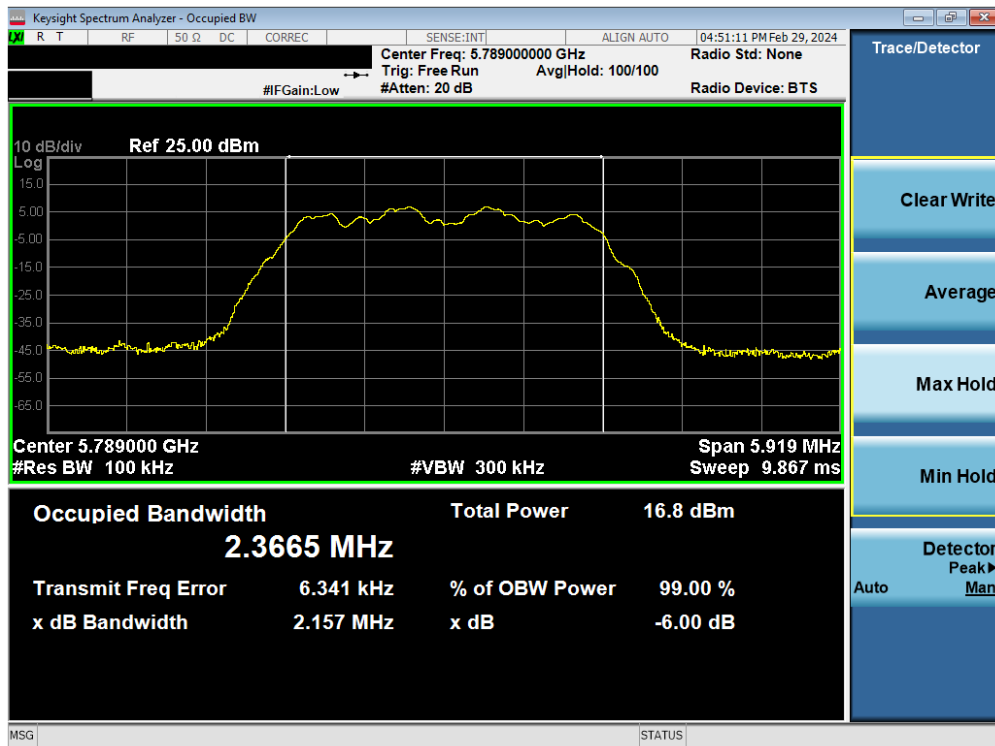
Plot 7-26. 6dB BW & 99% OBW Antenna 3a (HDR4, ePA, 5789MHz)
