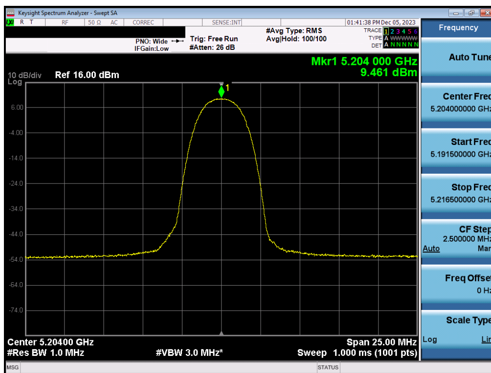
Plot 7-38. FCC PSD Antenna 3c (HDR4, ePA – 5204MHz)
