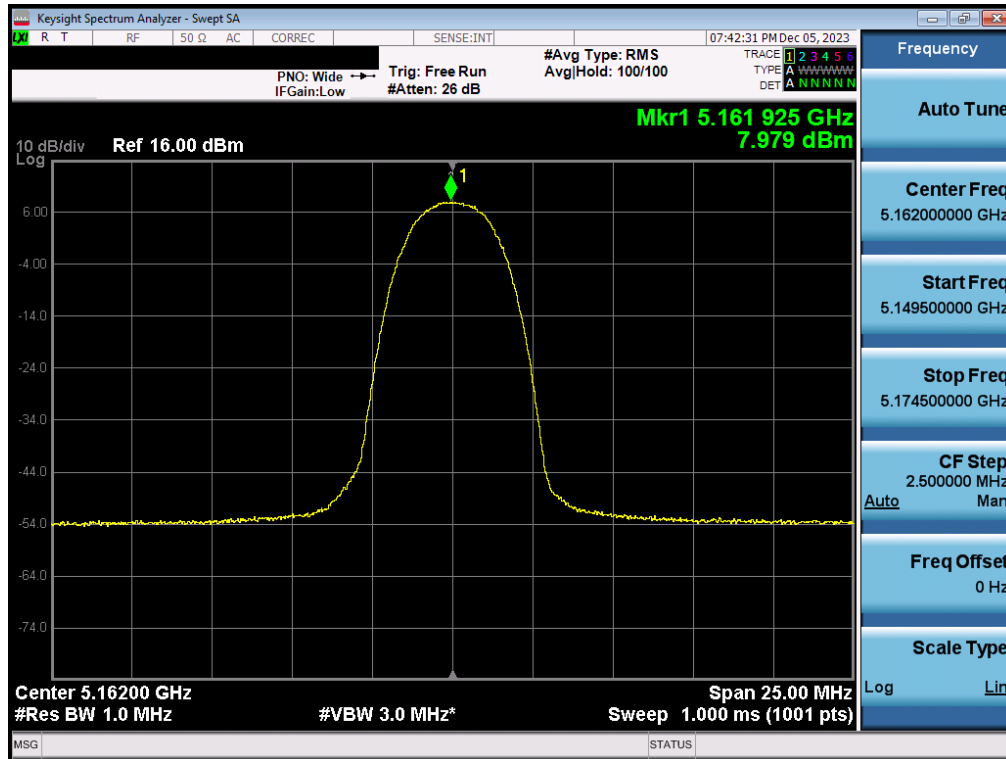
Plot 7-91. PSD Antenna 1b (HDR4, ePA – 5162MHz)
