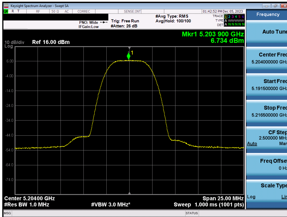
Plot 7-44. FCC PSD Antenna 3c (HDR8, ePA – 5204MHz)
