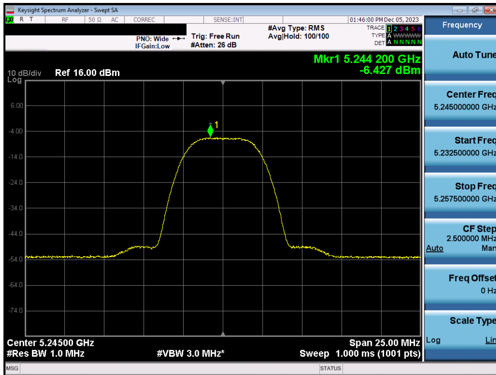
Plot 7-48. FCC/ISED PSD Antenna 3c (HDR8, iPA– 5245MHz)
