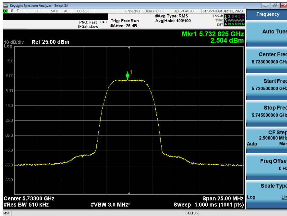
Plot 7-85. PSD Antenna 3a (HDR8, ePA 5733MHz)
