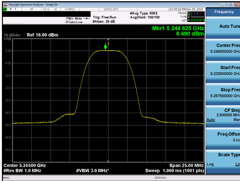
Plot 7-45. FCC PSD Antenna 3c (HDR8, ePA– 5245MHz)
