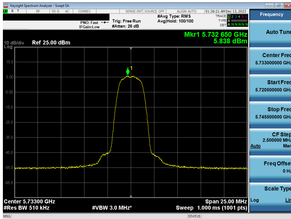
Plot 7-79. PSD Antenna 3a (HDR4, ePA 5733MHz)
