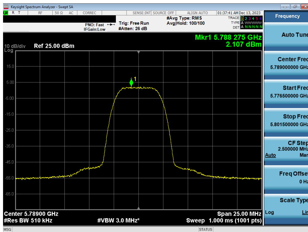
Plot 7-86. PSD Antenna 3a (HDR8, ePA 5789MHz)
