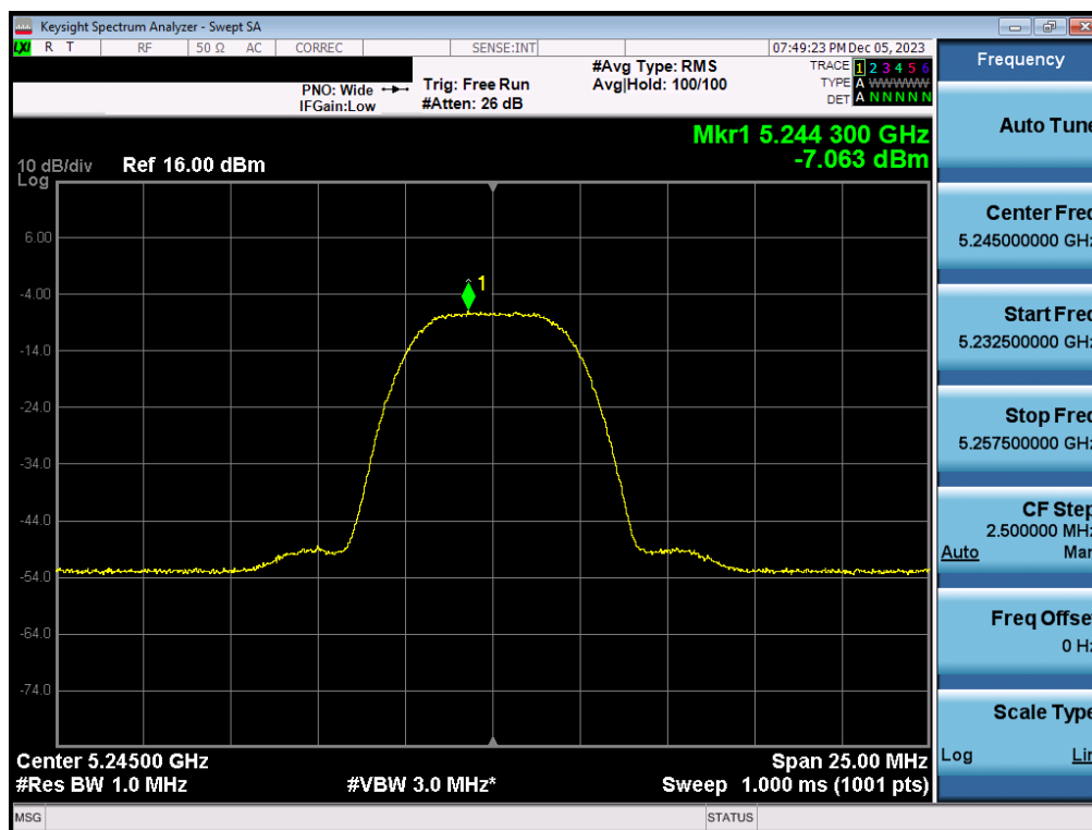
Plot 7-102. PSD Antenna 1b (HDR8, iPA – 5245MHz)
