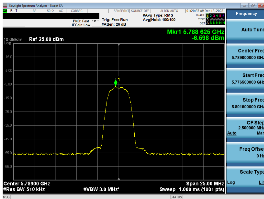
Plot 7-59. PSD Antenna 3c (HDR4, iPA 5789MHz)
