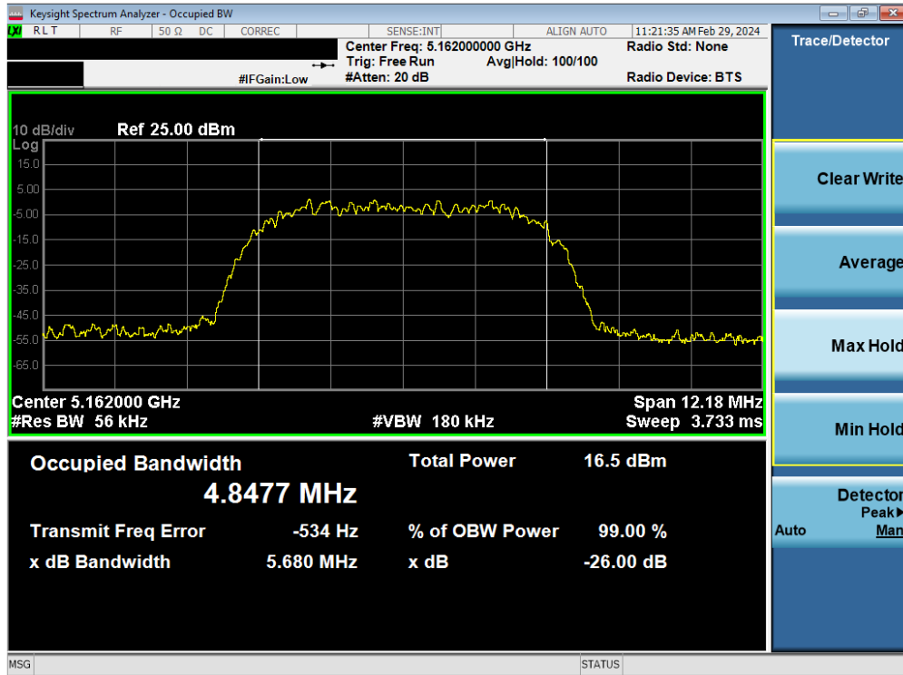
Plot 7-10. 26dB BW & 99% OBW Antenna 3a (HDR8, ePA– 5162MHz)
