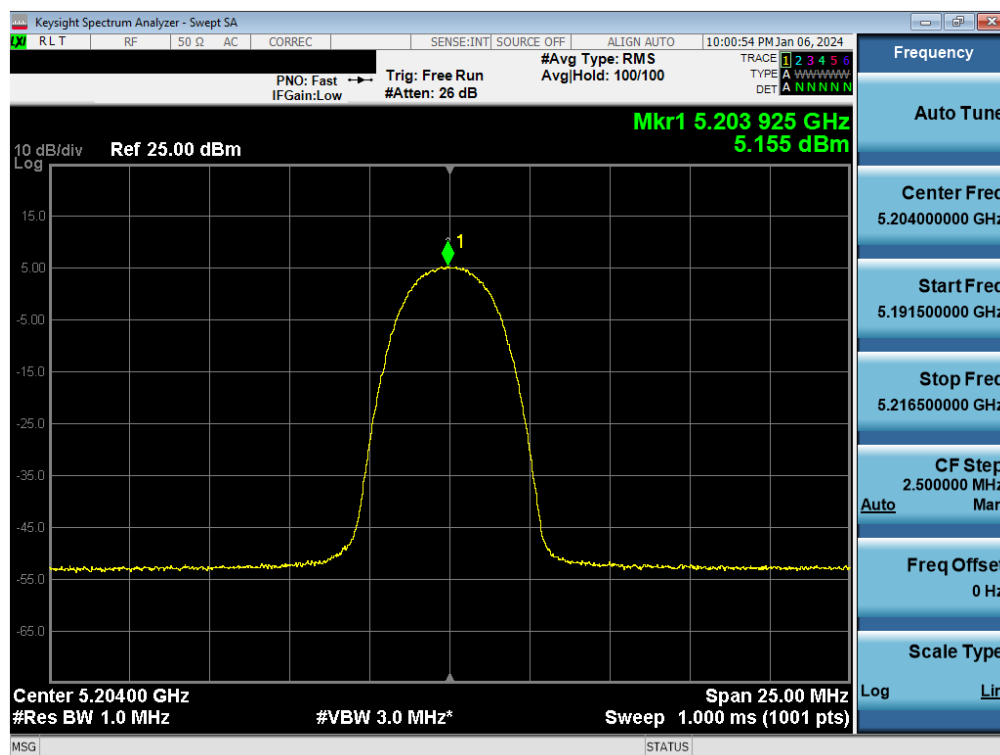
Plot 7-117. FCC PSD TxBF Antenna 3c (HDR4, ePA – 5204MHz)
