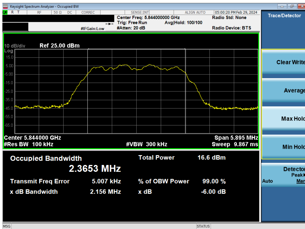
Plot 7-33. 6dB BW & 99% OBW Antenna 1b (HDR4, ePA, 5844MHz)
