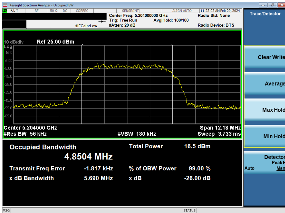
Plot 7-11. 26dB BW & 99% OBW Antenna 3a (HDR8, ePA– 5204MHz)
