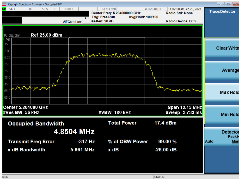
Plot 7-5. 26dB BW & 99% OBW Antenna 3c (HDR8, ePA- 5204MHz)
