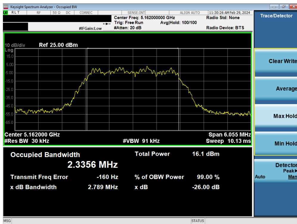
Plot 7-13. 26dB BW & 99% OBW Antenna 1b (HDR4, ePA– 5162MHz)
