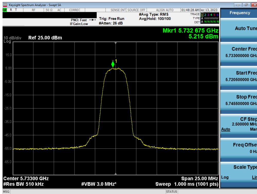
Plot 7-103. PSD Antenna 1b (HDR4, ePA 5733MHz)
