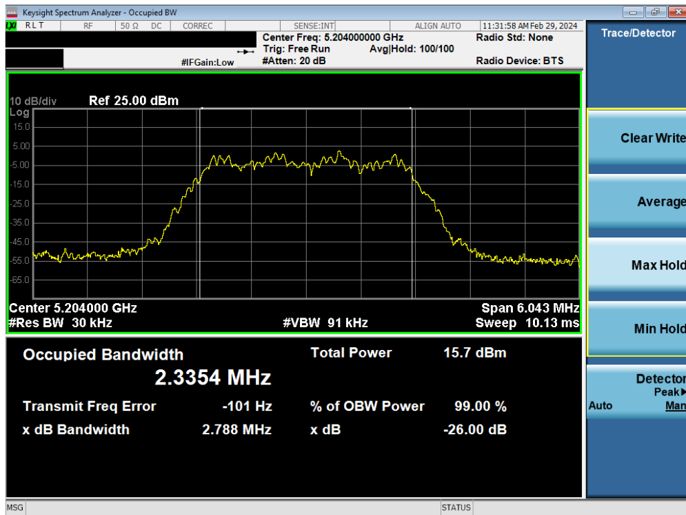
Plot 7-14. 26dB BW & 99% OBW Antenna 1b (HDR4, ePA- 5204MHz)
