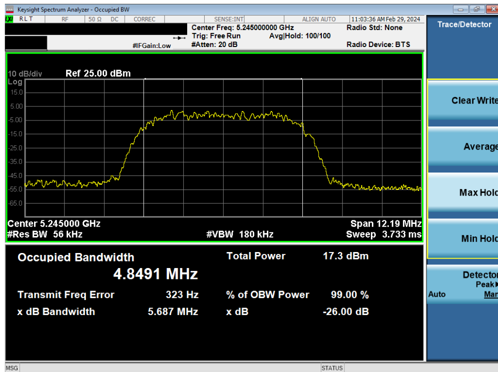
Plot 7-6. 26dB BW & 99% OBW Antenna 3c (HDR8, ePA – 5245MHz)
