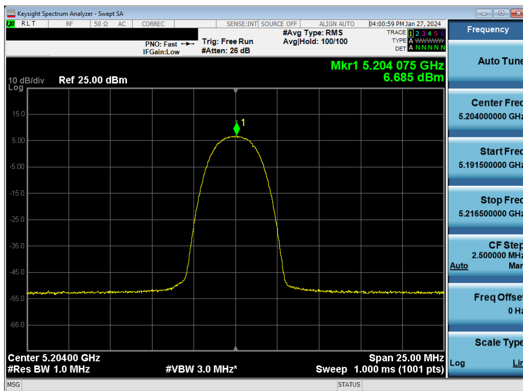
Plot 7-50. ISED PSD Antenna 3c (HDR4, ePA – 5204MHz)
