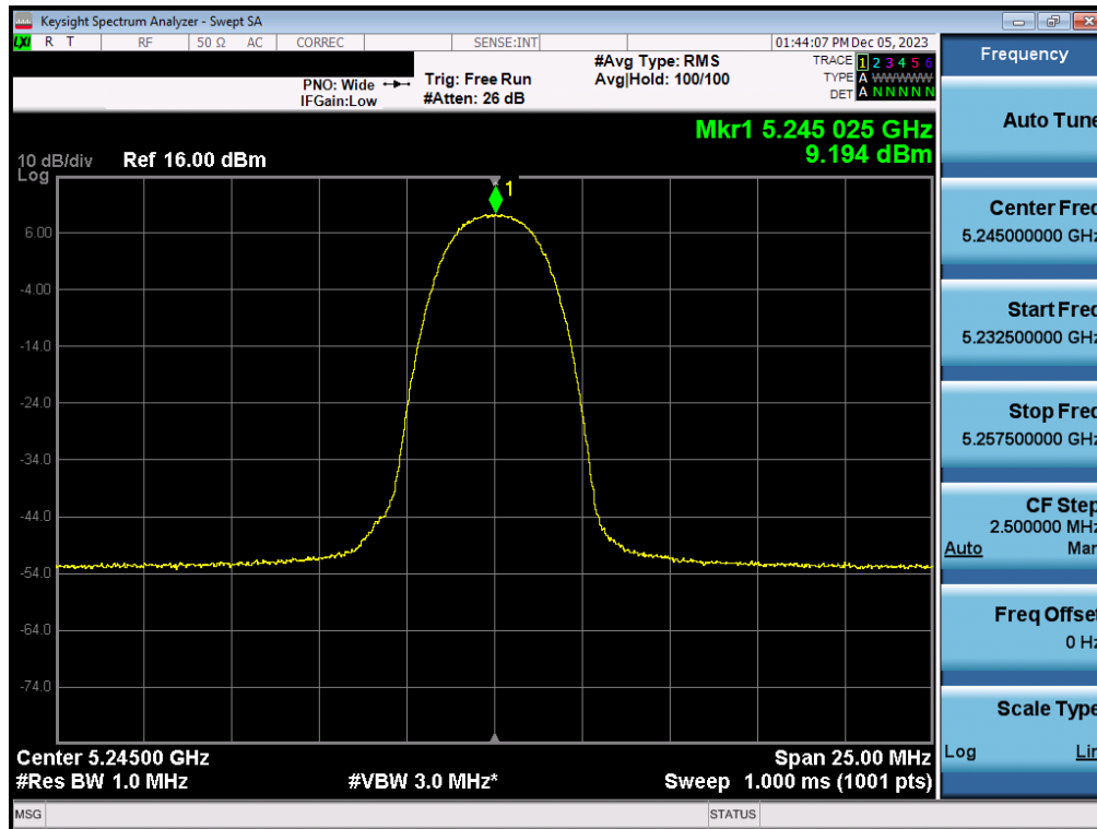
Plot 7-39. FCC PSD Antenna 3c (HDR4, ePA- 5245MHz)
