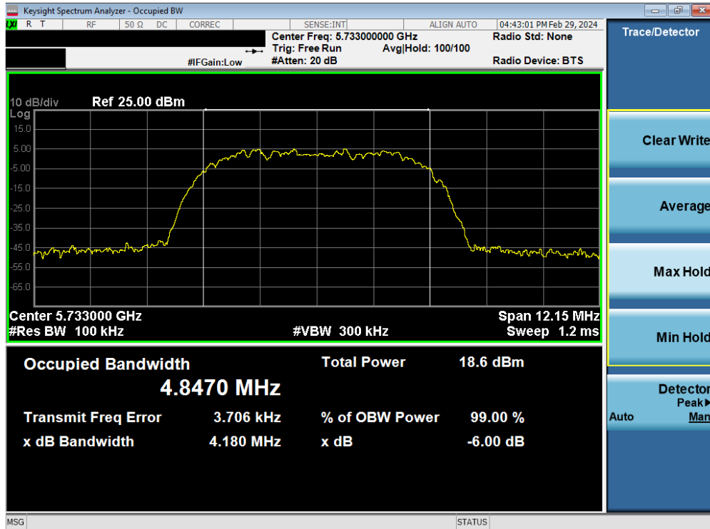
Plot 7-22. 6dB BW & 99% OBW Antenna 3c (HDR8, ePA, 5733MHz)
