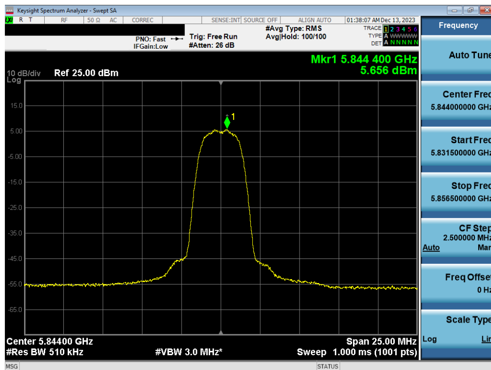
Plot 7-81. PSD Antenna 3a (HDR4, ePA 5844MHz)
