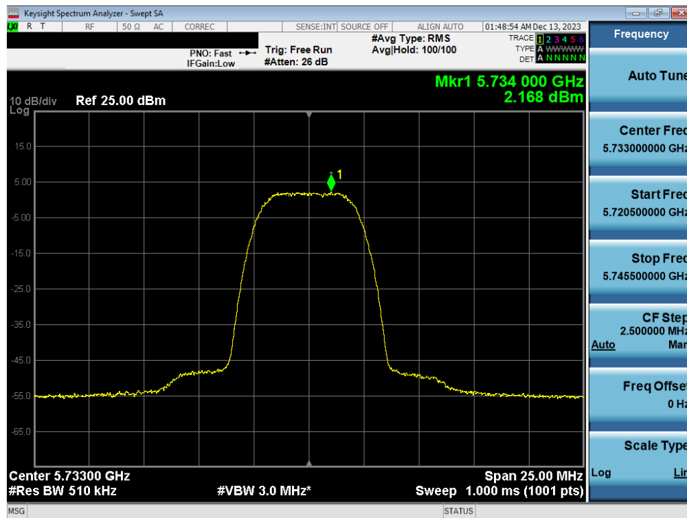
Plot 7-109. PSD Antenna 1b (HDR8, ePA 5733MHz)
