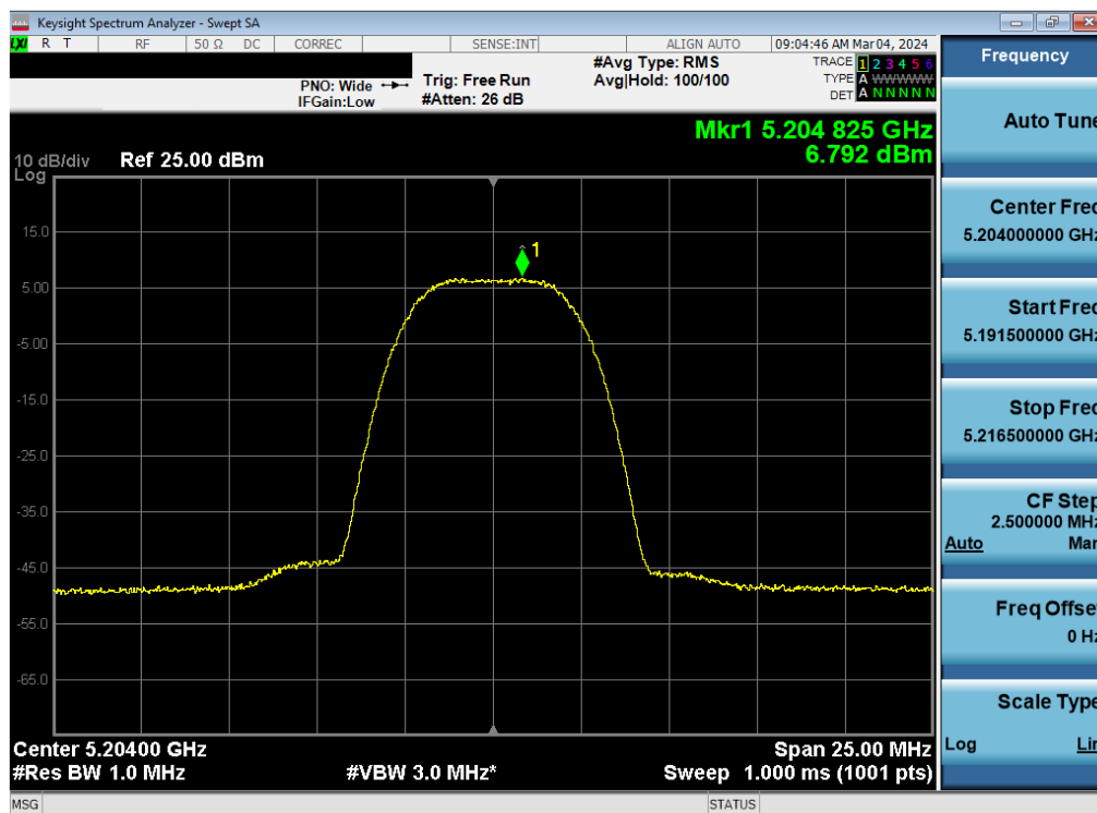
Plot 7-53. ISED PSD Antenna 3c (HDR8, ePA – 5204MHz)
