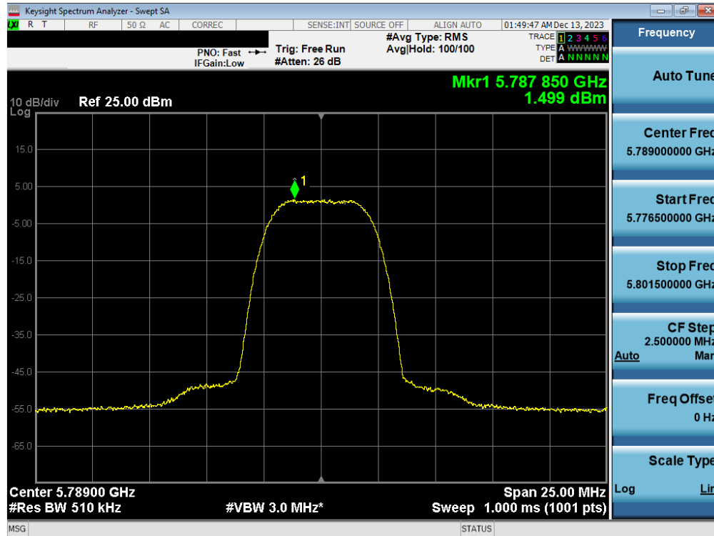
Plot 7-110. PSD Antenna 1b (HDR8, ePA 5789MHz)
