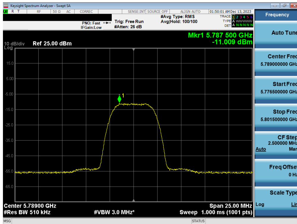
Plot 7-113. PSD Antenna 1b (HDR8, iPA 5789MHz)
