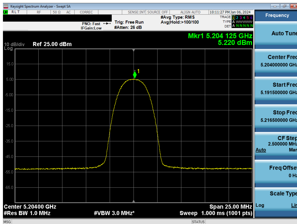
Plot 7-118. FCC PSD TxBF Antenna 3a (HDR4, ePA – 5204MHz)
