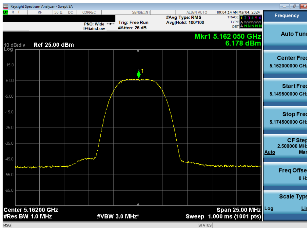
Plot 7-52. ISED PSD Antenna 3c (HDR8, ePA – 5162MHz)
