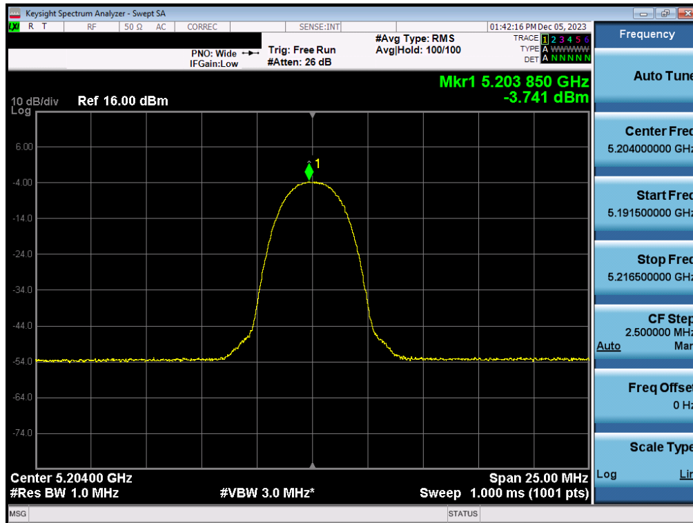
Plot 7-41. FCC/ISED PSD Antenna 3c (HDR4, iPA – 5204MHz)
