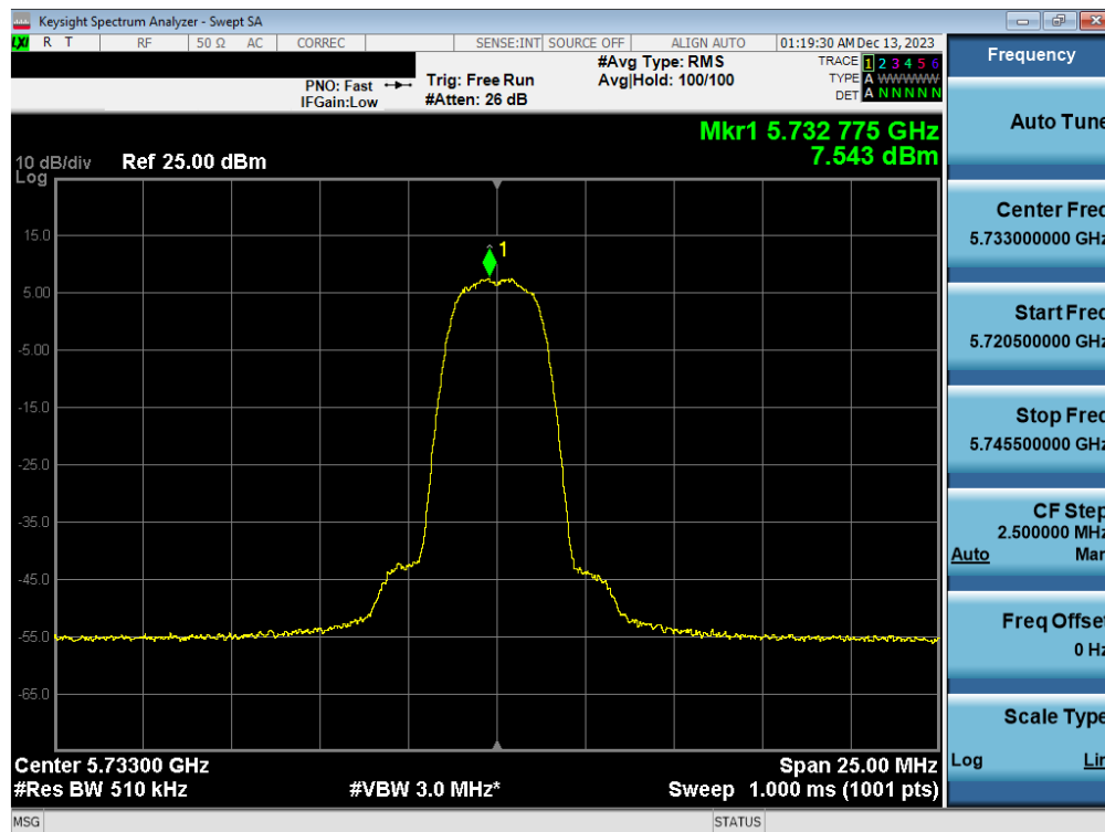
Plot 7-55. PSD Antenna 3c (HDR4, ePA 5733MHz)
