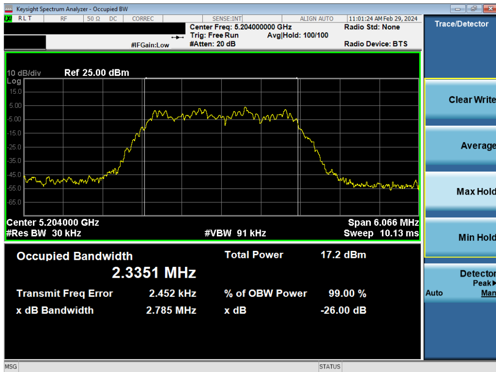
Plot 7-2. 26dB BW & 99% OBW Antenna 3c (HDR4, ePA– 5204MHz)
