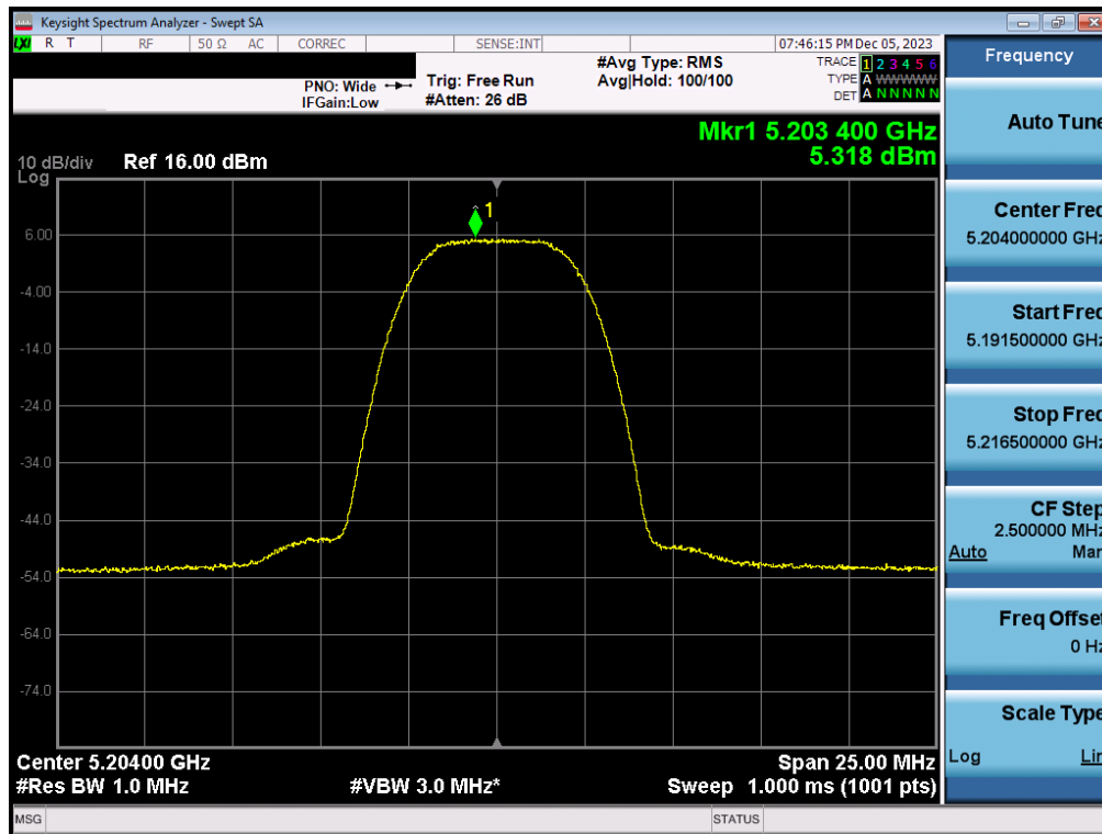
Plot 7-98. PSD Antenna 1b (HDR8, ePA – 5204MHz)
