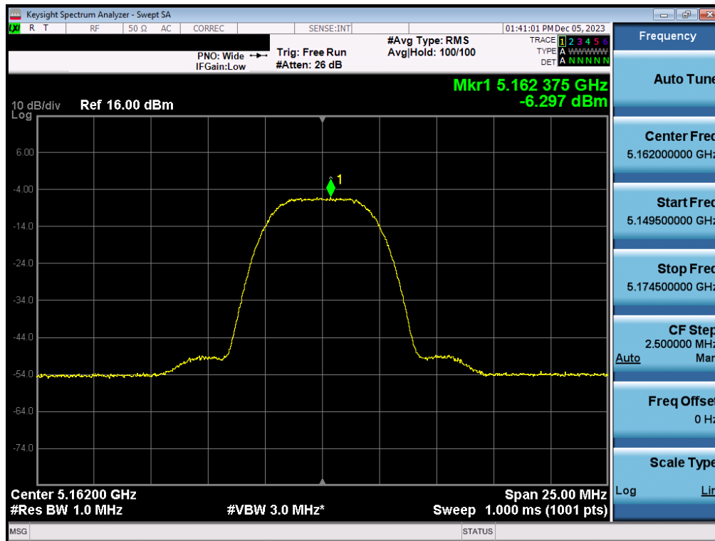
Plot 7-46. FCC/ISED PSD Antenna 3c (HDR8, iPA – 5162MHz)
