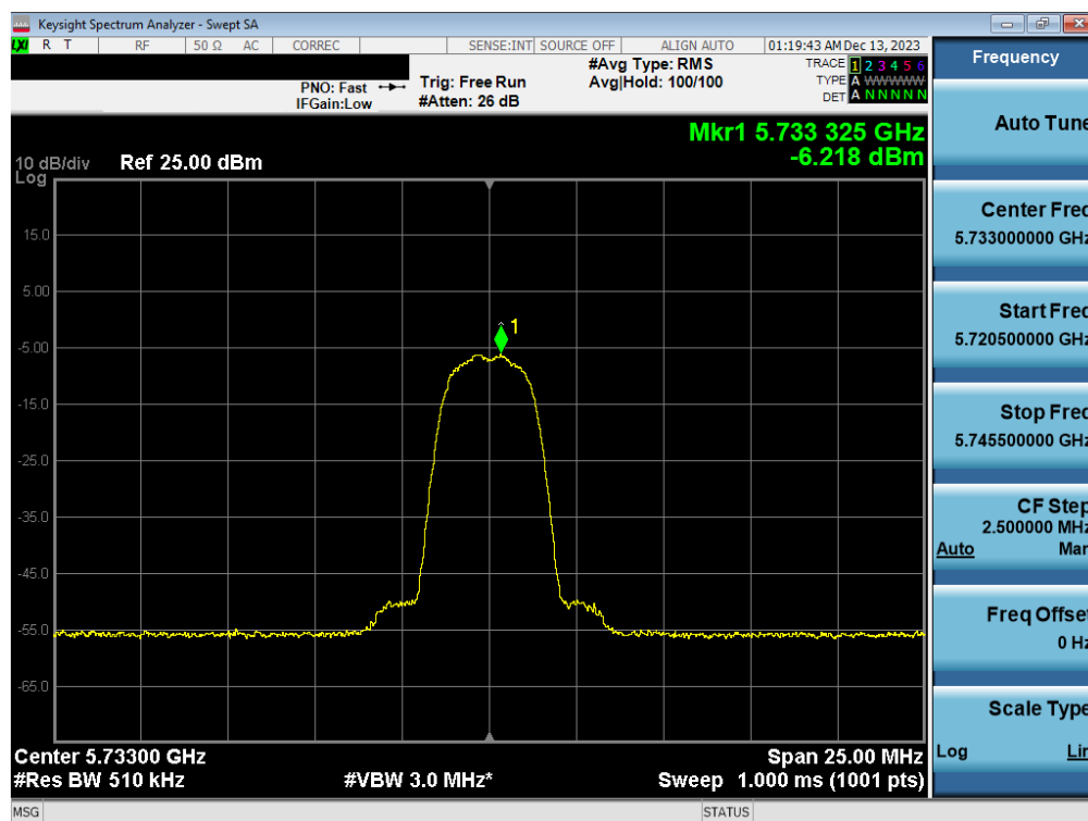
Plot 7-58. PSD Antenna 3c (HDR4, iPA 5733MHz)
