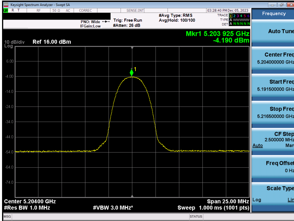
Plot 7-71. PSD Antenna 3a (HDR4, iPA - 5204MHz)
