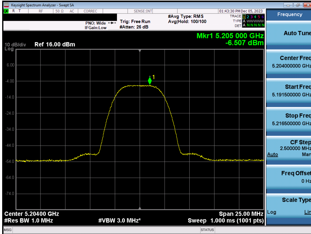
Plot 7-47. FCC/ISED PSD Antenna 3c (HDR8, iPA – 5204MHz)
