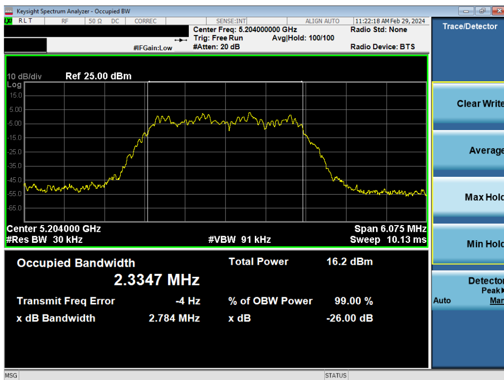
Plot 7-8. 26dB BW & 99% OBW Antenna 3a (HDR4, ePA- 5204MHz)
