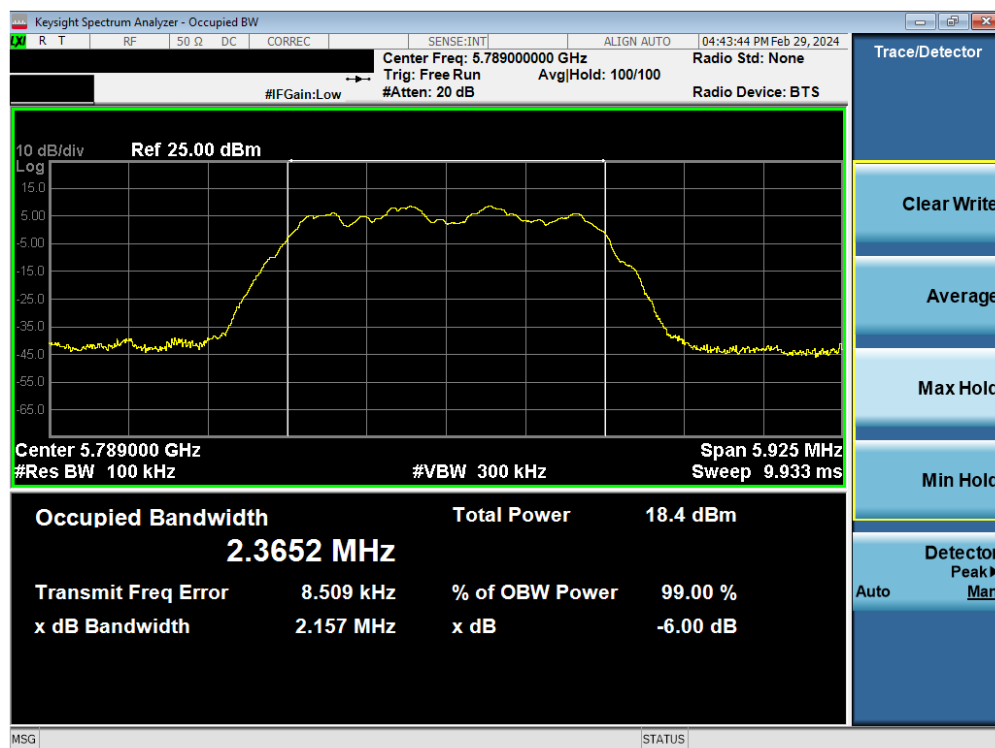
Plot 7-20. 6dB BW & 99% OBW Antenna 3c (HDR4, ePA, 5789MHz)
