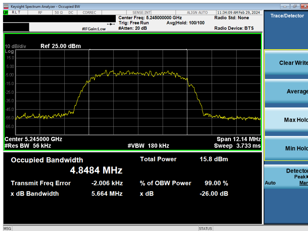
Plot 7-18. 26dB BW & 99% OBW Antenna 1b (HDR8, ePA- 5245MHz)
