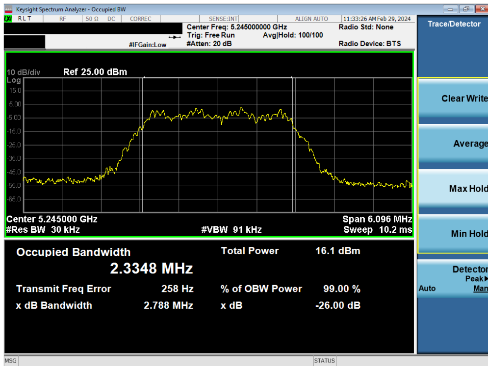
Plot 7-15. 26dB BW & 99% OBW Antenna 1b (HDR4, ePA- 5245MHz)
