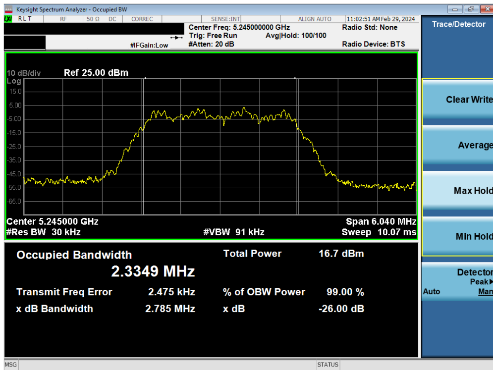
Plot 7-3. 26dB BW & 99% OBW Antenna 3c (HDR4, ePA – 5245MHz)
