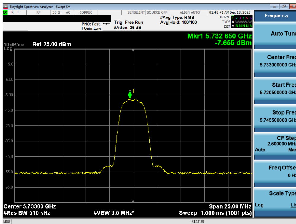
Plot 7-106. PSD Antenna 1b (HDR4, iPA 5733MHz)
