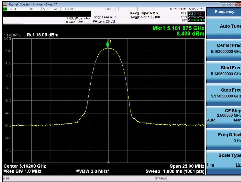
Plot 7-67. PSD Antenna 3a (HDR4, ePA – 5162MHz)
