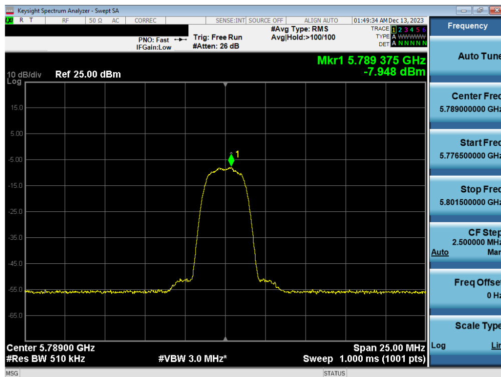
Plot 7-107. PSD Antenna 1b (HDR4, iPA 5789MHz)
