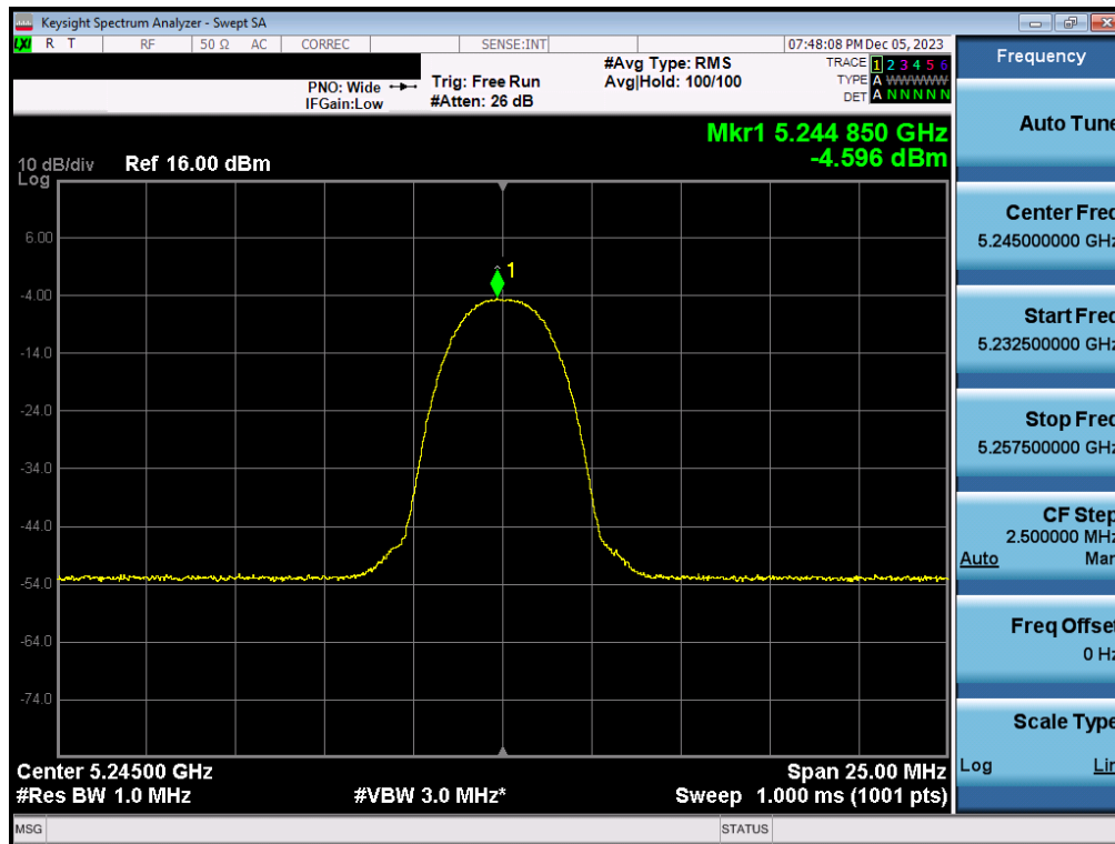
Plot 7-96. PSD Antenna 1b (HDR4, iPA- 5245MHz)
