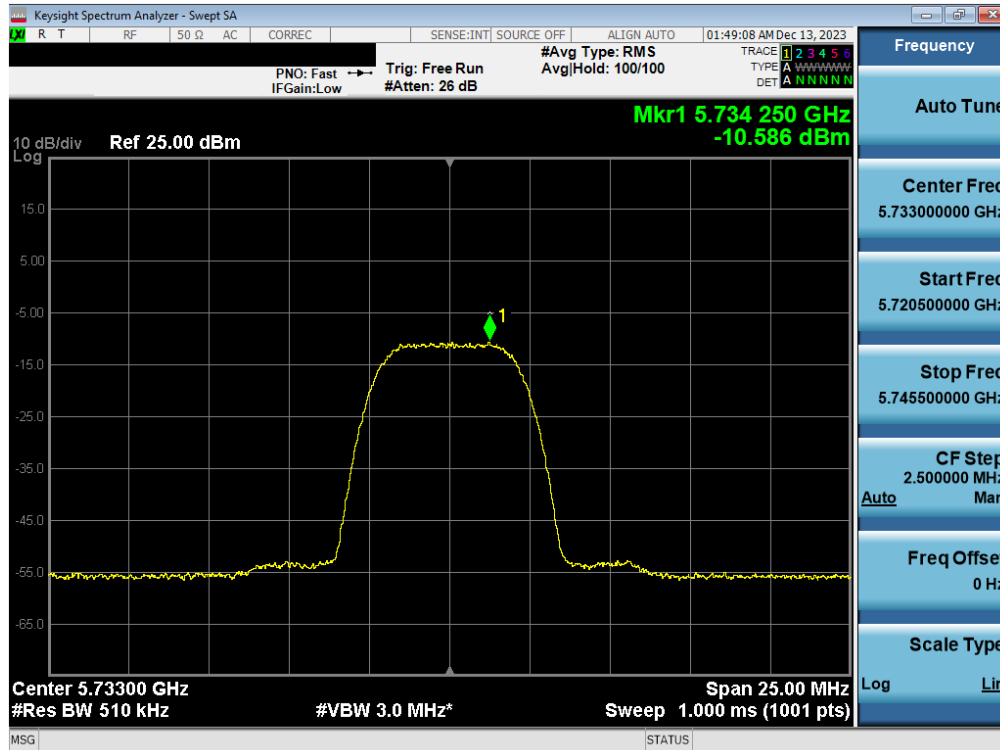
Plot 7-112. PSD Antenna 1b (HDR8, iPA 5733MHz)
