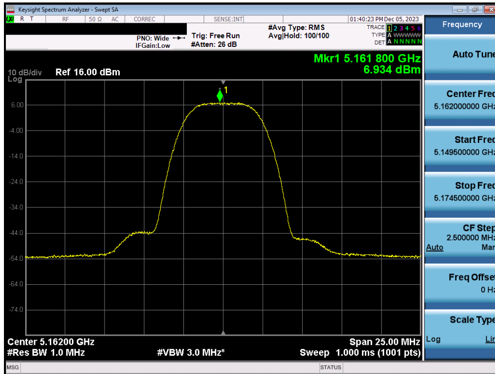
Plot 7-43. FCC PSD Antenna 3c (HDR8, ePA – 5162MHz)
