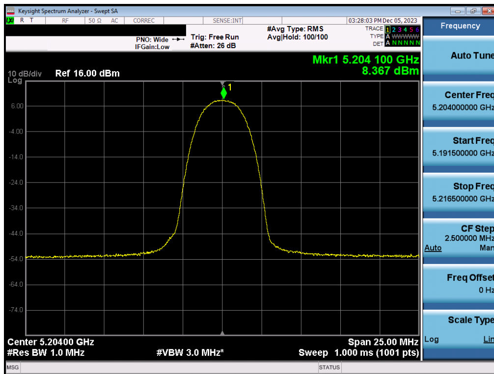
Plot 7-68. PSD Antenna 3a (HDR4, ePA – 5204MHz)
