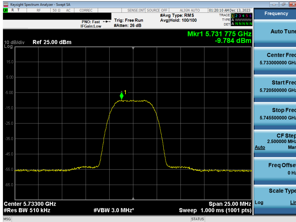
Plot 7-64. PSD Antenna 3c (HDR8, iPA 5733MHz)
