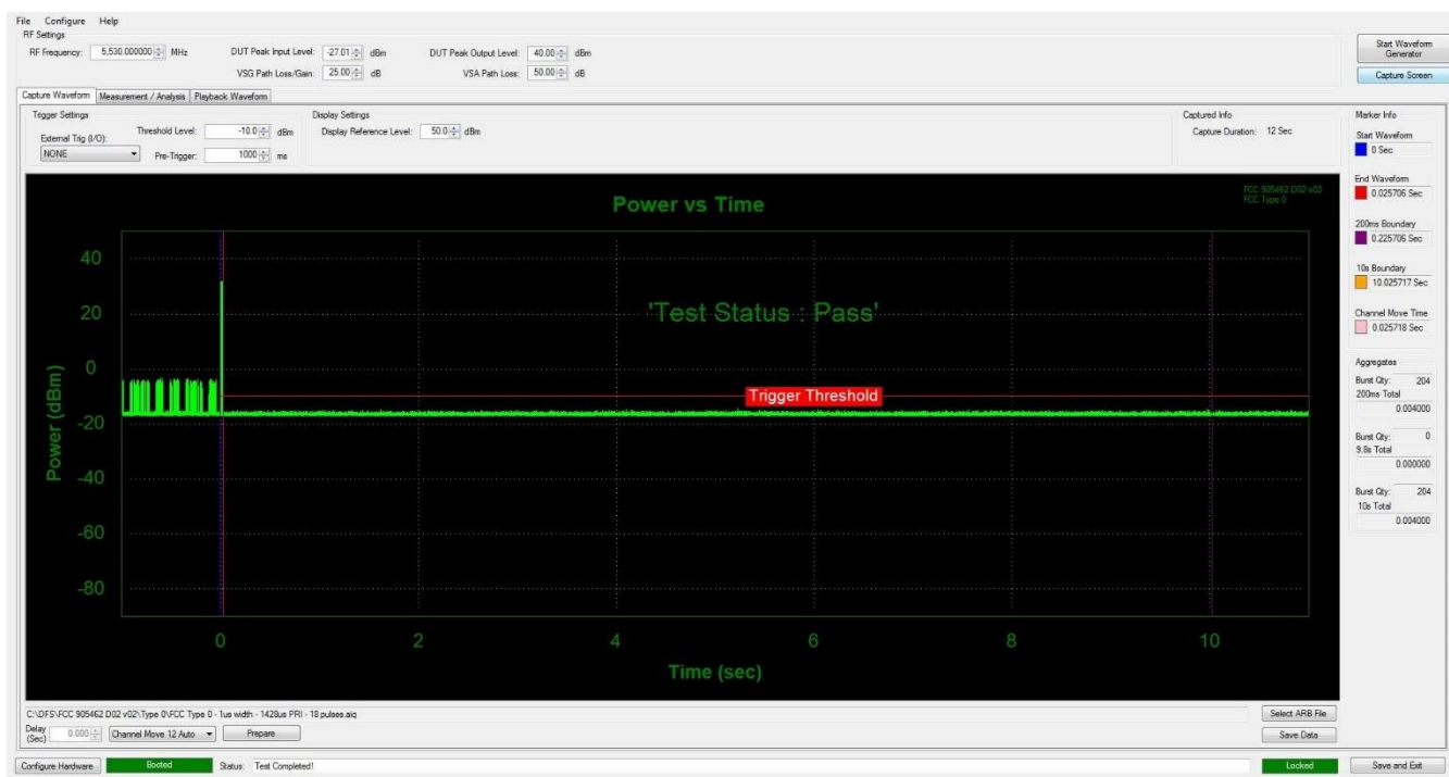
Figure 9-11. 5530MHz - Channel Move/ Closing Transmission Time - Mode 1 (80 MHz)
