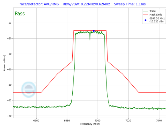
Plot 7-1511. LPI In-Band Emission Plot SDM Diversity Antenna 5T (20MHz 802.11ax RU242 (UNII Band 8) – Ch. 209)
