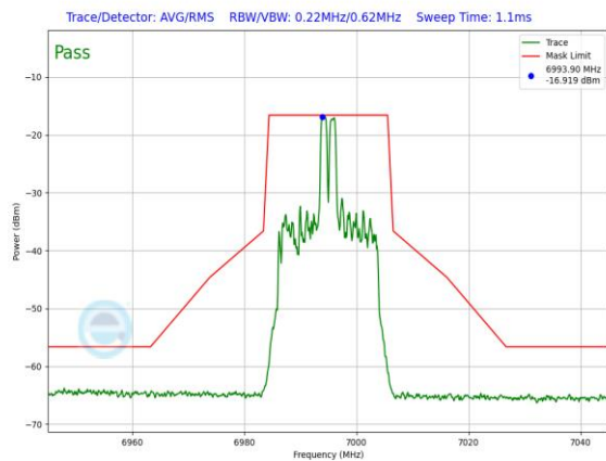
Plot 7-1507. LPI In-Band Emission Plot SDM Diversity Antenna 5T (20MHz 802.11ax RU26 (UNII Band 8) – Ch. 209)
