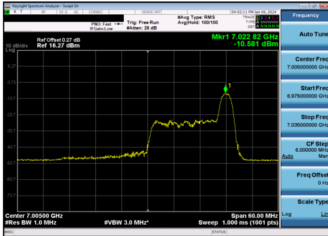
Plot 7-845. LPI Power Spectral Density Plot SDM Diversity Antenna 5T (40MHz 802.11ax RU26 (UNII Band 8) – Ch. 211)
