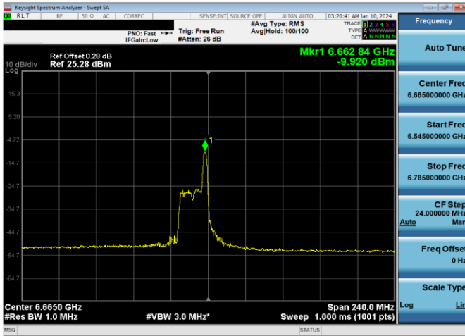
Plot 7-827. LPI Power Spectral Density Plot SDM Diversity Antenna 5T (160MHz 802.11ax RU26 (UNII Band 7) – Ch. 143)
