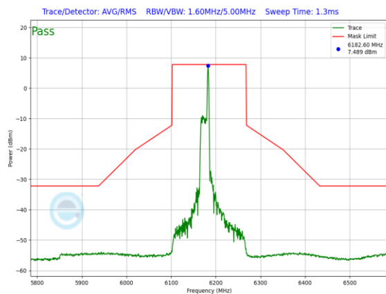
Plot 7-878. SP In-Band Emission Plot Antenna 5T (160MHz 802.11ax RU26 (UNII Band 5) – Ch. 47)
