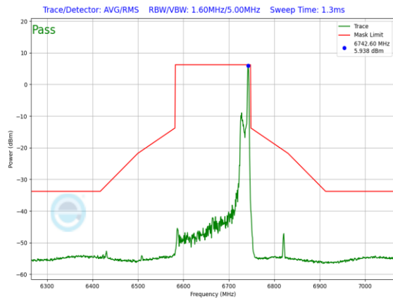
Plot 7-895. SP In-Band Emission Plot Antenna 5T (160MHz 802.11ax RU26 (UNII Band 7) – Ch. 143)
