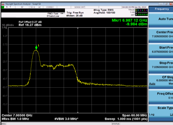
Plot 7-841. LPI Power Spectral Density Plot SDM Diversity Antenna 5T (40MHz 802.11ax RU26 (UNII Band 8) – Ch. 211)
