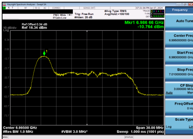
Plot 7-834. LPI Power Spectral Density Plot SDM Diversity Antenna 1b (20MHz 802.11ax RU26 (UNII Band 8) – Ch. 209)
