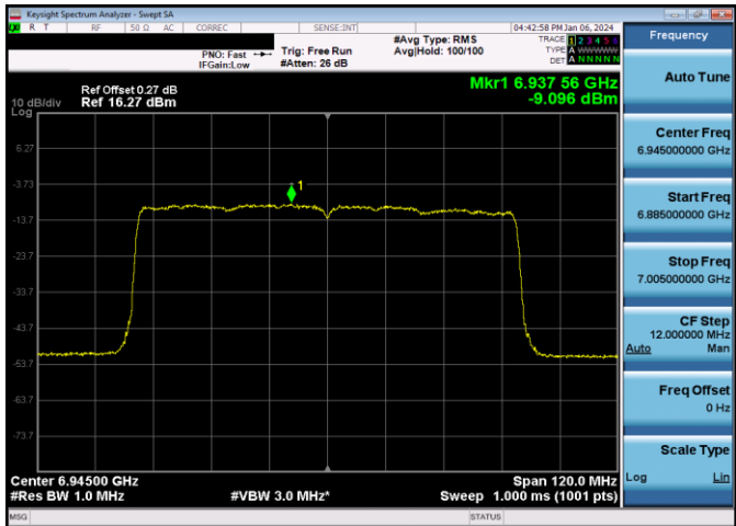
Plot 7-855. LPI Power Spectral Density Plot SDM Diversity Antenna 5T (80MHz 802.11ax RU996 (UNII Band 8) – Ch. 199)
