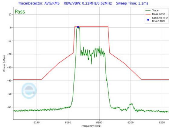
Plot 7-865. SP In-Band Emission Plot Antenna 5T (20MHz 802.11ax RU26 (UNII Band 5) – Ch. 45)
