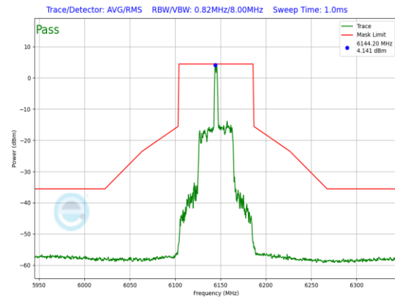
Plot 7-906. SP In-Band Emission Plot Antenna 3b (80MHz 802.11ax RU26 (UNII Band 5) – Ch. 39)
