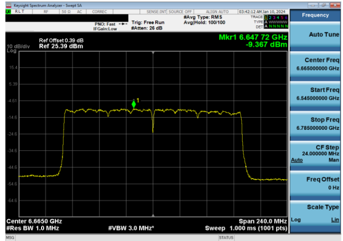
Plot 7-831. LPI Power Spectral Density Plot SDM Diversity Antenna 5T (160MHz 802.11ax RU996x2 (UNII Band 7) – Ch. 143)
