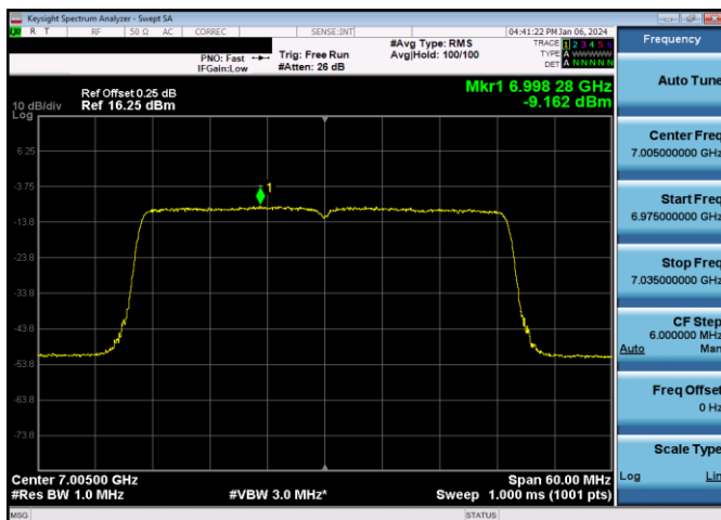
Plot 7-847. LPI Power Spectral Density Plot SDM Diversity Antenna 5T (40MHz 802.11ax RU484 (UNII Band 8) – Ch. 211)
