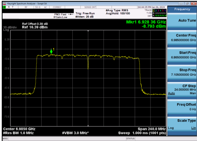
Plot 7-863. LPI Power Spectral Density Plot SDM Diversity Antenna 5T (160MHz 802.11ax RU996x2 (UNII Band 8) – Ch. 207)
