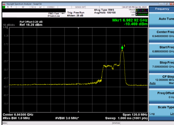
Plot 7-853. LPI Power Spectral Density Plot SDM Diversity Antenna 5T (80MHz 802.11ax RU26 (UNII Band 8) – Ch. 199)
