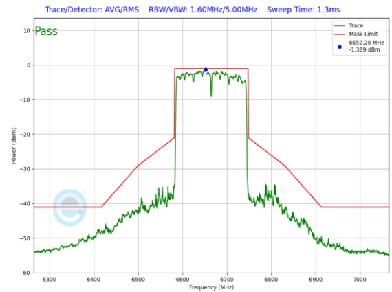
Plot 7-896. SP In-Band Emission Plot Antenna 5T (160MHz 802.11ax RU996x2 (UNII Band 7) – Ch. 143)
