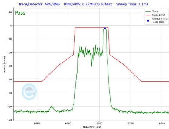
Plot 7-883. SP In-Band Emission Plot Antenna 5T (20MHz 802.11ax RU26 (UNII Band 7) – Ch. 149)
