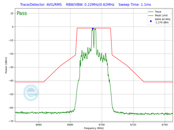
Plot 7-882. SP In-Band Emission Plot Antenna 5T (20MHz 802.11ax RU26 (UNII Band 7) – Ch. 149)
