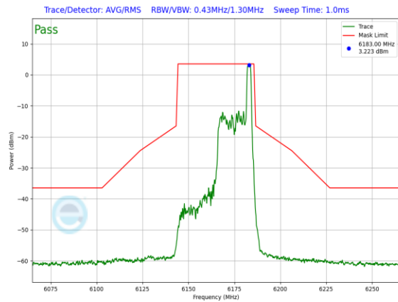
Plot 7-871. SP In-Band Emission Plot Antenna 5T (40MHz 802.11ax RU26 (UNII Band 5) – Ch. 43)
