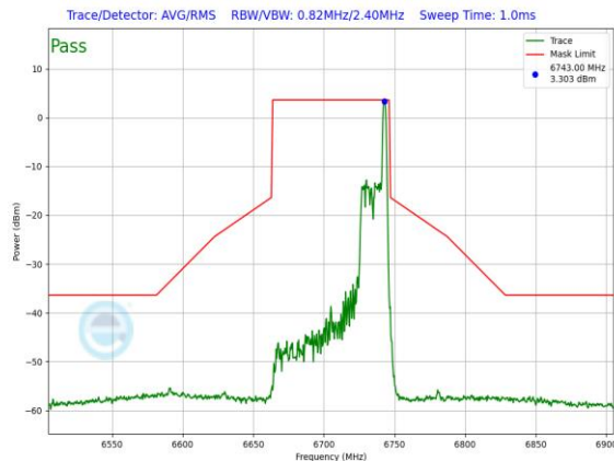
Plot 7-891. SP In-Band Emission Plot Antenna 5T (80MHz 802.11ax RU26 (UNII Band 7) – Ch. 151)
