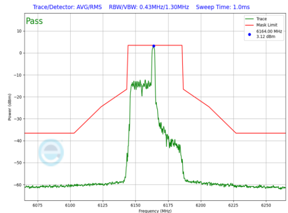
Plot 7-870. SP In-Band Emission Plot Antenna 5T (40MHz 802.11ax RU26 (UNII Band 5) – Ch. 43)
