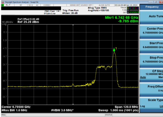
Plot 7-821. LPI Power Spectral Density Plot SDM Diversity Antenna 5T (80MHz 802.11ax RU26 (UNII Band 7) – Ch. 151)
