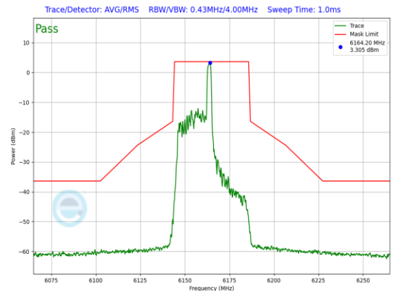
Plot 7-902. SP In-Band Emission Plot Antenna 3b (40MHz 802.11ax RU26 (UNII Band 5) – Ch. 43)
