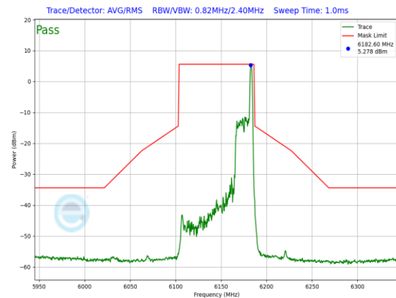
Plot 7-875. SP In-Band Emission Plot Antenna 5T (80MHz 802.11ax RU26 (UNII Band 5) – Ch. 39)
