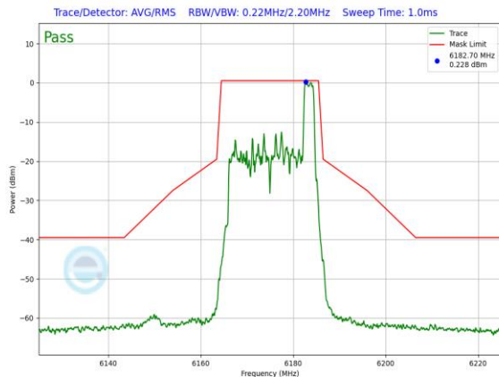
Plot 7-899. SP In-Band Emission Plot Antenna 3b (20MHz 802.11ax RU26 (UNII Band 5) – Ch. 45)
