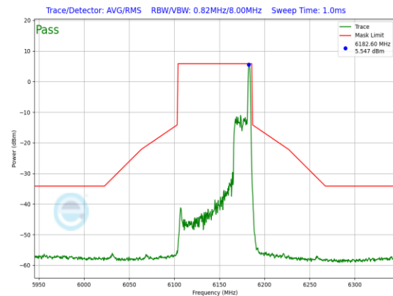
Plot 7-907. SP In-Band Emission Plot Antenna 3b (80MHz 802.11ax RU26 (UNII Band 5) – Ch. 39)
