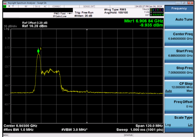
Plot 7-849. LPI Power Spectral Density Plot SDM Diversity Antenna 5T (80MHz 802.11ax RU26 (UNII Band 8) – Ch. 199)
