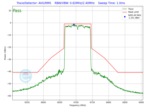
Plot 7-892. SP In-Band Emission Plot Antenna 5T (80MHz 802.11ax RU996 (UNII Band 7) – Ch. 151)
