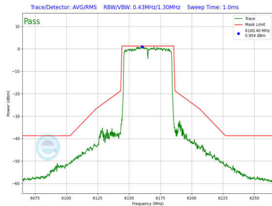
Plot 7-872. SP In-Band Emission Plot Antenna 5T (40MHz 802.11ax RU484 (UNII Band 5) – Ch. 43)
