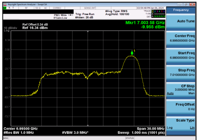
Plot 7-837. LPI Power Spectral Density Plot SDM Diversity Antenna 5T (20MHz 802.11ax RU26 (UNII Band 8) – Ch. 209)
