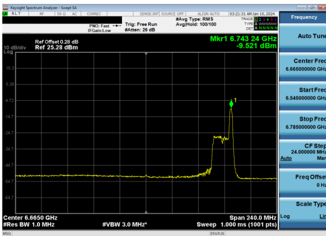
Plot 7-829. LPI Power Spectral Density Plot SDM Diversity Antenna 5T (160MHz 802.11ax RU26 (UNII Band 7) – Ch. 143)
