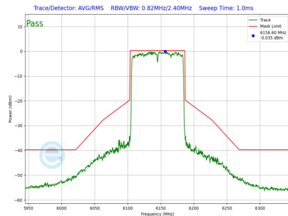
Plot 7-876. SP In-Band Emission Plot Antenna 5T (80MHz 802.11ax RU996 (UNII Band 5) – Ch. 39)
