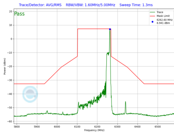
Plot 7-879. SP In-Band Emission Plot Antenna 5T (160MHz 802.11ax RU26 (UNII Band 5) – Ch. 47)
