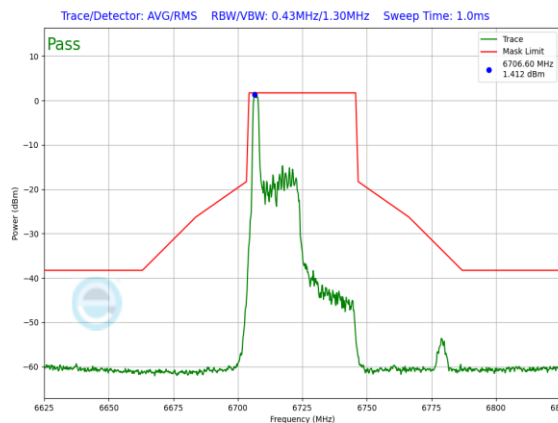
Plot 7-885. SP In-Band Emission Plot Antenna 5T (40MHz 802.11ax RU26 (UNII Band 7) – Ch. 155)
