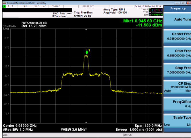
Plot 7-851. LPI Power Spectral Density Plot SDM Diversity Antenna 5T (80MHz 802.11ax RU26 (UNII Band 8) – Ch. 199)
