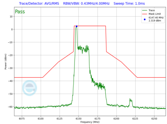
Plot 7-901. SP In-Band Emission Plot Antenna 3b (40MHz 802.11ax RU26 (UNII Band 5) – Ch. 43)
