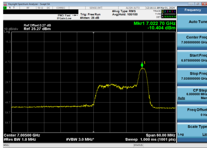
Plot 7-846. LPI Power Spectral Density Plot SDM Diversity Antenna 1b (40MHz 802.11ax RU26 (UNII Band 8) – Ch. 211)
