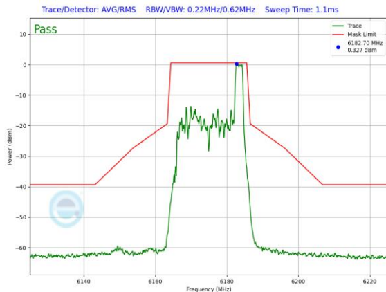
Plot 7-867. SP In-Band Emission Plot Antenna 5T (20MHz 802.11ax RU26 (UNII Band 5) – Ch. 45)
