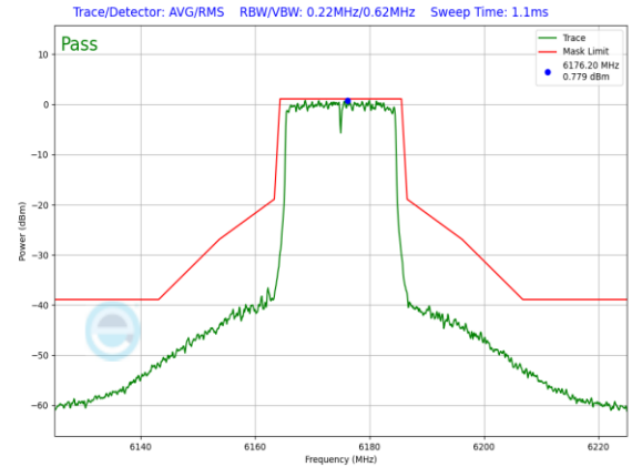
Plot 7-868. SP In-Band Emission Plot Antenna 5T (20MHz 802.11ax RU242 (UNII Band 5) – Ch. 45)
