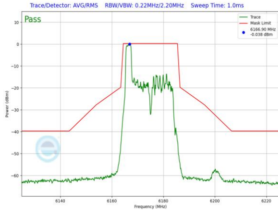
Plot 7-897. SP In-Band Emission Plot Antenna 3b (20MHz 802.11ax RU26 (UNII Band 5) – Ch. 45)
