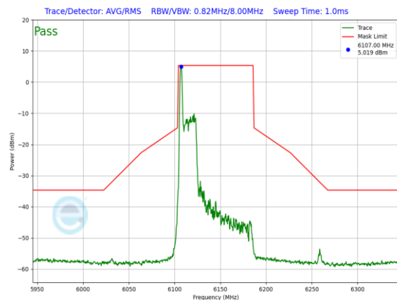
Plot 7-905. SP In-Band Emission Plot Antenna 3b (80MHz 802.11ax RU26 (UNII Band 5) – Ch. 39)
