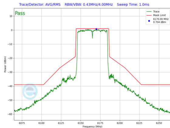
Plot 7-904. SP In-Band Emission Plot Antenna 3b (40MHz 802.11ax RU484 (UNII Band 5) – Ch. 43)
