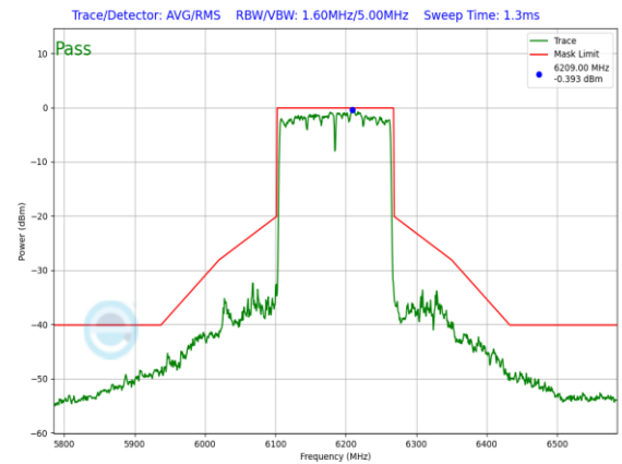
Plot 7-880. SP In-Band Emission Plot Antenna 5T (160MHz 802.11ax RU996x2 (UNII Band 5) – Ch. 47)
