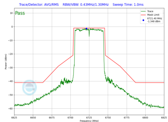
Plot 7-888. SP In-Band Emission Plot Antenna 5T (40MHz 802.11ax RU484 (UNII Band 7) – Ch. 155)
