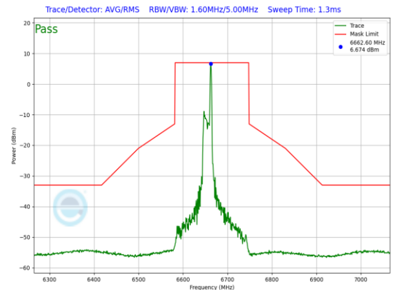
Plot 7-894. SP In-Band Emission Plot Antenna 5T (160MHz 802.11ax RU26 (UNII Band 7) – Ch. 143)
