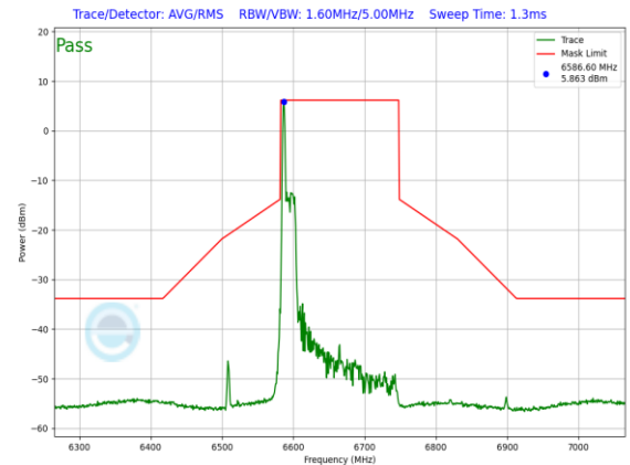
Plot 7-893. SP In-Band Emission Plot Antenna 5T (160MHz 802.11ax RU26 (UNII Band 7) – Ch. 143)
