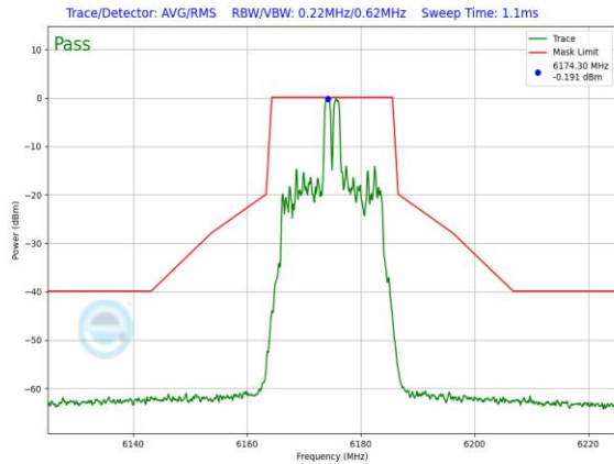
Plot 7-866. SP In-Band Emission Plot Antenna 5T (20MHz 802.11ax RU26 (UNII Band 5) – Ch. 45)
