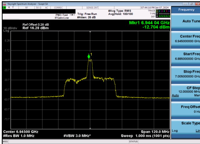
Plot 7-852. LPI Power Spectral Density Plot SDM Diversity Antenna 1b (80MHz 802.11ax RU26 (UNII Band 8) – Ch. 199)
