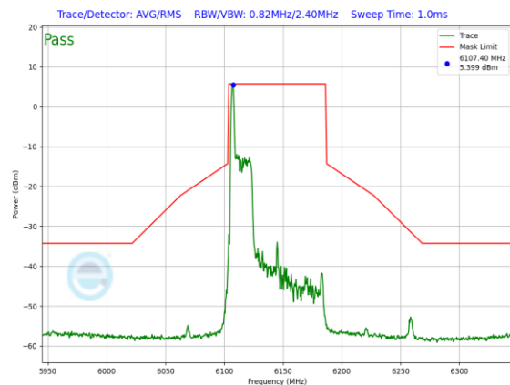
Plot 7-873. SP In-Band Emission Plot Antenna 5T (80MHz 802.11ax RU26 (UNII Band 5) – Ch. 39)
