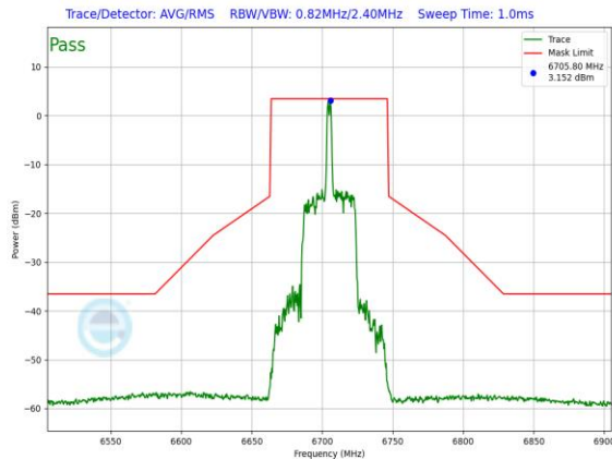
Plot 7-890. SP In-Band Emission Plot Antenna 5T (80MHz 802.11ax RU26 (UNII Band 7) – Ch. 151)
