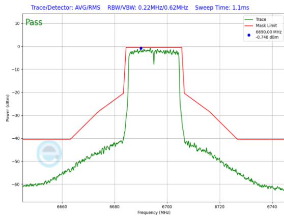
Plot 7-884. SP In-Band Emission Plot Antenna 5T (20MHz 802.11ax RU242 (UNII Band 7) – Ch. 149)
