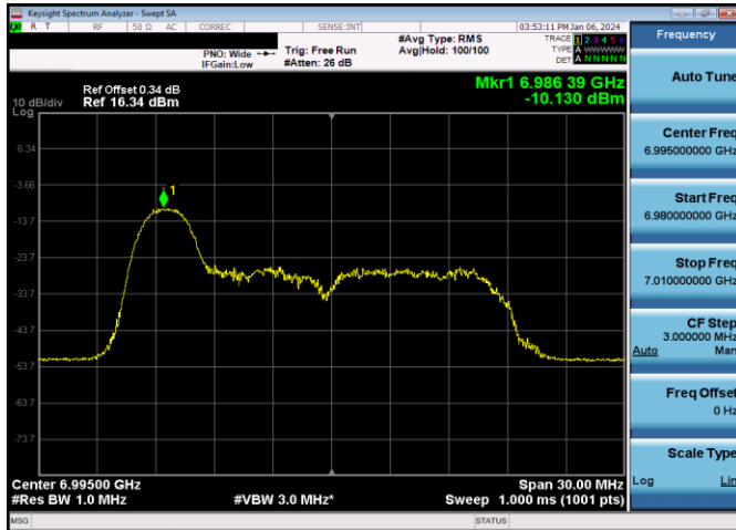
Plot 7-833. LPI Power Spectral Density Plot SDM Diversity Antenna 5T (20MHz 802.11ax RU26 (UNII Band 8) – Ch. 209)
