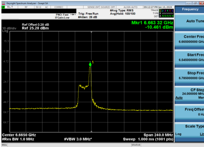
Plot 7-828. LPI Power Spectral Density Plot SDM Diversity Antenna 1b (160MHz 802.11ax RU26 (UNII Band 7) – Ch. 143)
