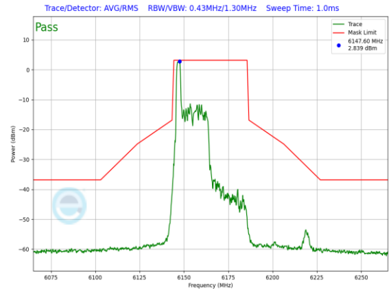
Plot 7-869. SP In-Band Emission Plot Antenna 5T (40MHz 802.11ax RU26 (UNII Band 5) – Ch. 43)
