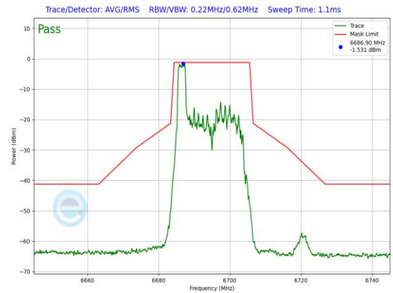
Plot 7-881. SP In-Band Emission Plot Antenna 5T (20MHz 802.11ax RU26 (UNII Band 7) – Ch. 149)
