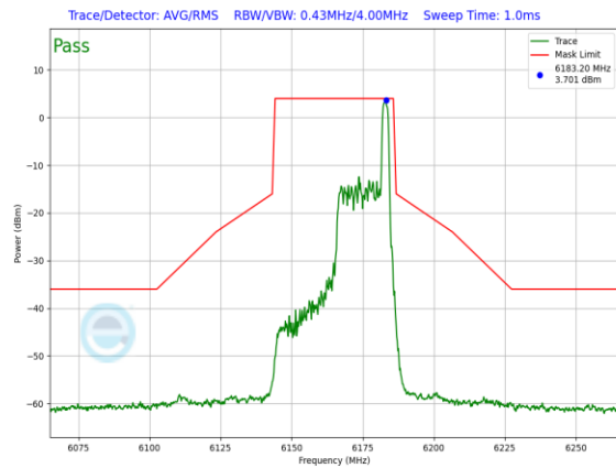
Plot 7-903. SP In-Band Emission Plot Antenna 3b (40MHz 802.11ax RU26 (UNII Band 5) – Ch. 43)
