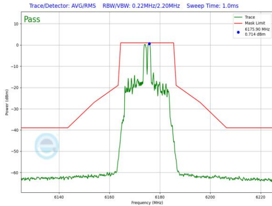
Plot 7-898. SP In-Band Emission Plot Antenna 3b (20MHz 802.11ax RU26 (UNII Band 5) – Ch. 45)
