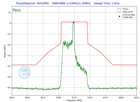
Plot 7-886. SP In-Band Emission Plot Antenna 5T (40MHz 802.11ax RU26 (UNII Band 7) – Ch. 155)
