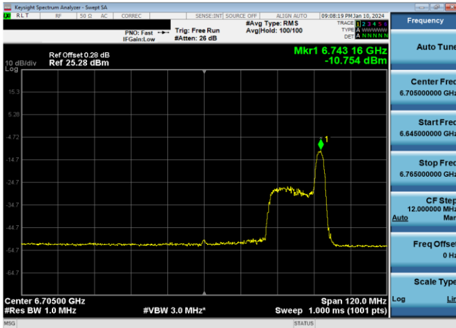
Plot 7-822. LPI Power Spectral Density Plot SDM Diversity Antenna 1b (80MHz 802.11ax RU26 (UNII Band 7) – Ch. 151)
