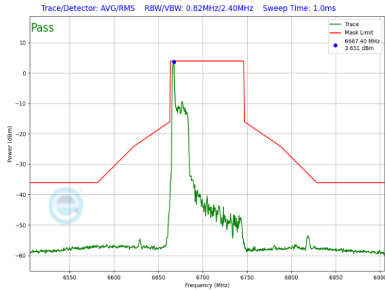
Plot 7-889. SP In-Band Emission Plot Antenna 5T (80MHz 802.11ax RU26 (UNII Band 7) – Ch. 151)
