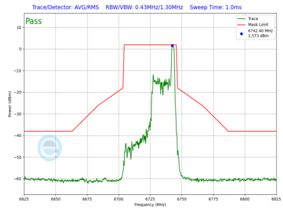
Plot 7-887. SP In-Band Emission Plot Antenna 5T (40MHz 802.11ax RU26 (UNII Band 7) – Ch. 155)
