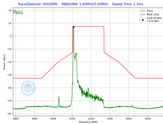
Plot 7-877. SP In-Band Emission Plot Antenna 5T (160MHz 802.11ax RU26 (UNII Band 5) – Ch. 47)
