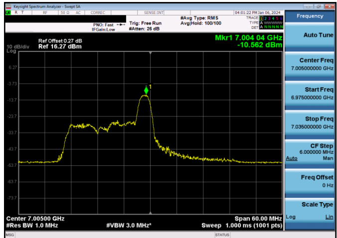
Plot 7-843. LPI Power Spectral Density Plot SDM Diversity Antenna 5T (40MHz 802.11ax RU26 (UNII Band 8) – Ch. 211)
