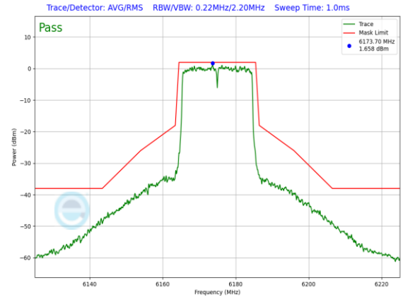
Plot 7-900. SP In-Band Emission Plot Antenna 3b (20MHz 802.11ax RU242 (UNII Band 5) – Ch. 45)
