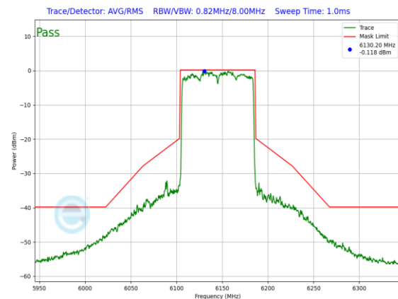
Plot 7-908. SP In-Band Emission Plot Antenna 3b (80MHz 802.11ax RU996 (UNII Band 5) – Ch. 39)
