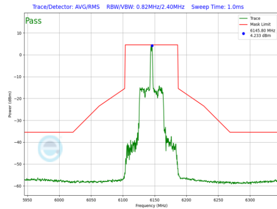
Plot 7-874. SP In-Band Emission Plot Antenna 5T (80MHz 802.11ax RU26 (UNII Band 5) – Ch. 39)
