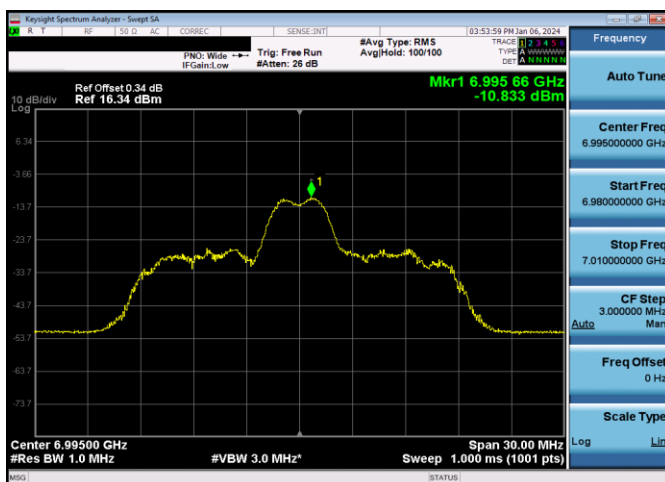
Plot 7-835. LPI Power Spectral Density Plot SDM Diversity Antenna 5T (20MHz 802.11ax RU26 (UNII Band 8) – Ch. 209)
