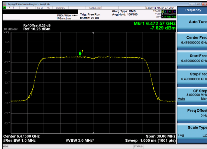
Plot 7-500. LPI Power Spectral Density Plot Antenna 3b (20MHz 802.11ax RU242 (UNII Band 6) – Ch. 105)
