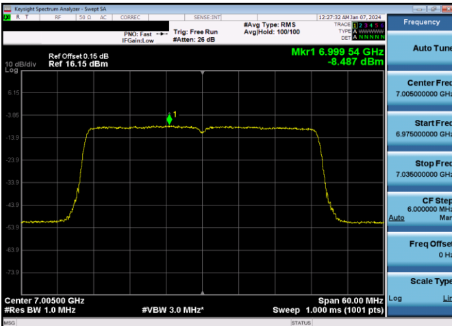
Plot 7-536. LPI Power Spectral Density Plot Antenna 3b (40MHz 802.11ax RU484 (UNII Band 8) – Ch. 211)
