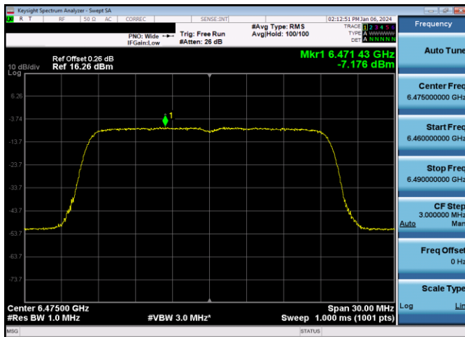
Plot 7-436. LPI Power Spectral Density Plot Antenna 5T (20MHz 802.11ax RU242 (UNII Band 6) – Ch. 105)
