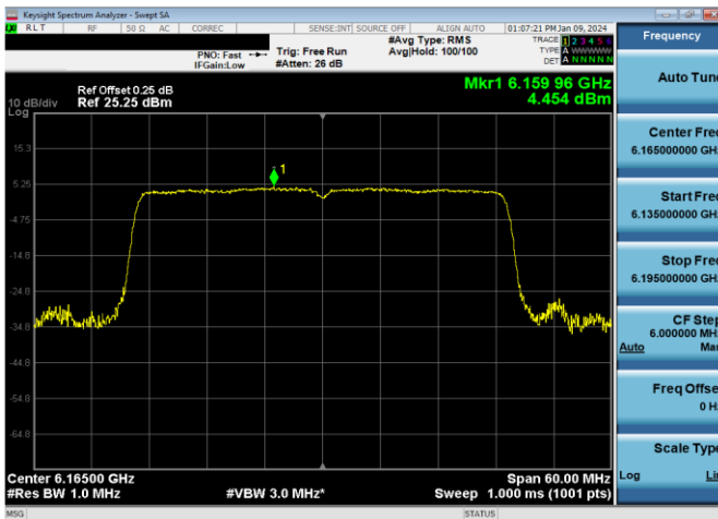
Plot 7-303. SP Power Spectral Density Plot CDD Primary Antenna 5T (40MHz 802.11ax RU484 (UNII Band 5) – Ch. 43)
