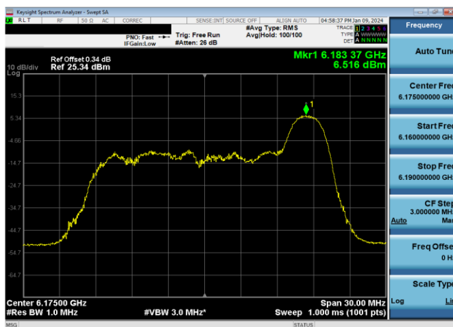
Plot 7-294. SP Power Spectral Density Plot CDD Primary Antenna 3b (20MHz 802.11ax RU26 (UNII Band 5) – Ch. 45)
