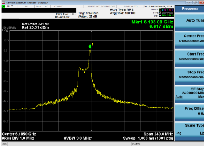
Plot 7-238. SP Power Spectral Density Plot Antenna 3b (160MHz 802.11ax RU26 (UNII Band 5) – Ch. 47)
