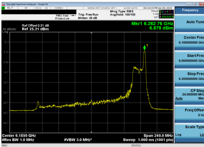
Plot 7-239. SP Power Spectral Density Plot Antenna 3b (160MHz 802.11ax RU26 (UNII Band 5) – Ch. 47)
