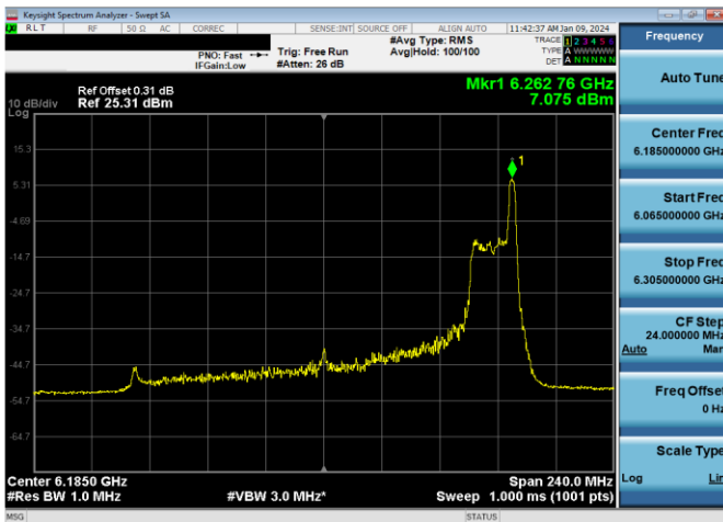
Plot 7-207. SP Power Spectral Density Plot Antenna 5T (160MHz 802.11ax RU26 (UNII Band 5) – Ch. 47)
