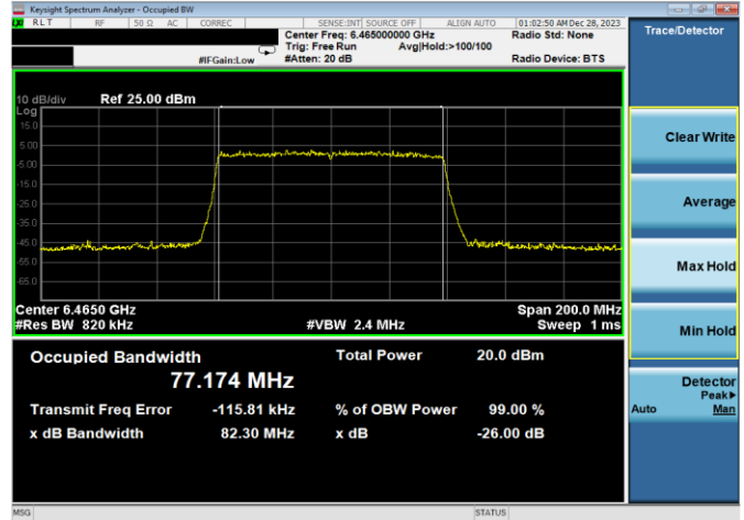
Plot 7-28. 26dB & 99% Bandwidth Plot Antenna 5T (80MHz 802.11ax RU96 (UNII Band 6) – Ch. 103)
