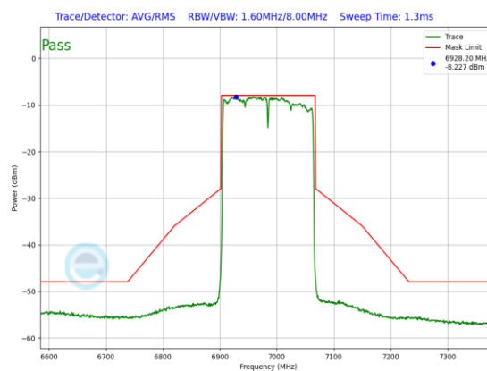
Plot 7-1040. LPI In-Band Emission Plot SDM Primary Antenna 3b (160MHz 802.11ax (UNII Band 8) – Ch. 207, MCS2)
