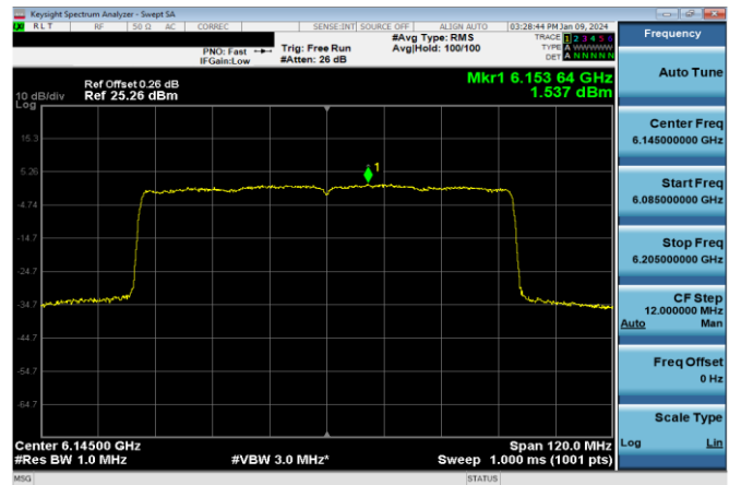
Plot 7-711. Power Spectral Density Plot CDD Diversity Antenna 3b Standard Power (40MHz 802.11ax (UNII Band 5) – Ch. 39, MCS4)
