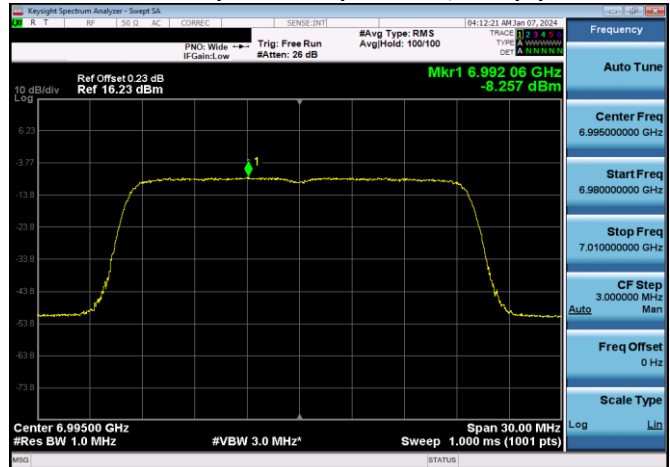
Plot 7-397. Power Spectral Density Plot Antenna 1b LPI (20MHz 802.11ax (UNII Band 8) – Ch. 209, MCS4)
