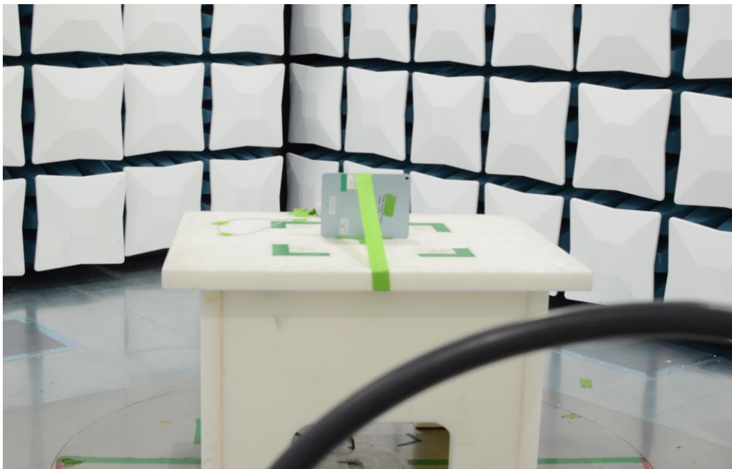
Figure 20: 9kHz-30MHz Test Setup (Front View)
