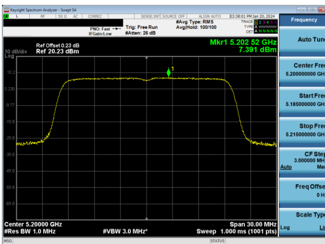
Plot 7-172. PSD Antenna WF7a (20MHz BW 11ax- RU242 - Ch.40)
