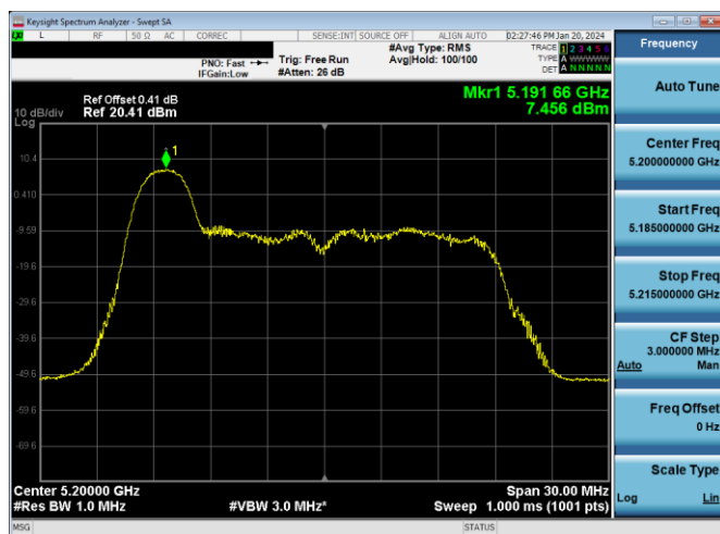
Plot 7-169. PSD Antenna WF7a (20MHz BW 11ax Index 0 - RU26 - Ch.40)
