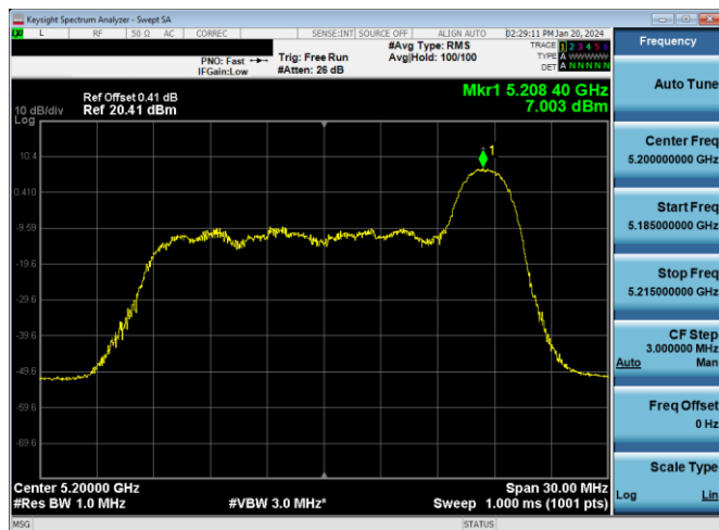
Plot 7-171. PSD Antenna WF7a (20MHz BW 11ax Index 8 - RU26 - Ch.40)
