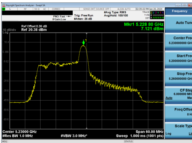
Plot 7-174. PSD Antenna WF7a (40MHz BW 11ax Index 8 - RU26 - Ch.46)
