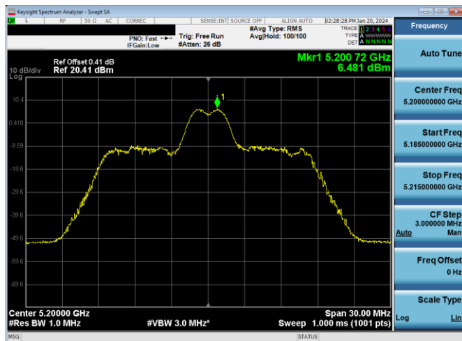
Plot 7-170. PSD Antenna WF7a (20MHz BW 11ax Index 4 - RU26 - Ch.40)
