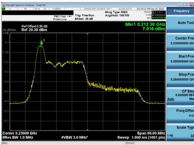
Plot 7-173. PSD Antenna WF7a (40MHz BW 11ax Index 0 - RU26 - Ch.46)
