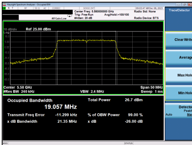
Plot 7-32. 26dB BW & 99% OBW Antenna WF7a (20MHz BW 11ax– RU242 – Ch.116)
