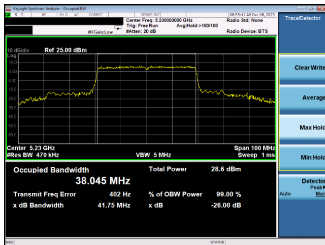
Plot 7-8. 26dB BW & 99% OBW Antenna WF7a (40MHz BW 11ax - RU484 - Ch.46)
